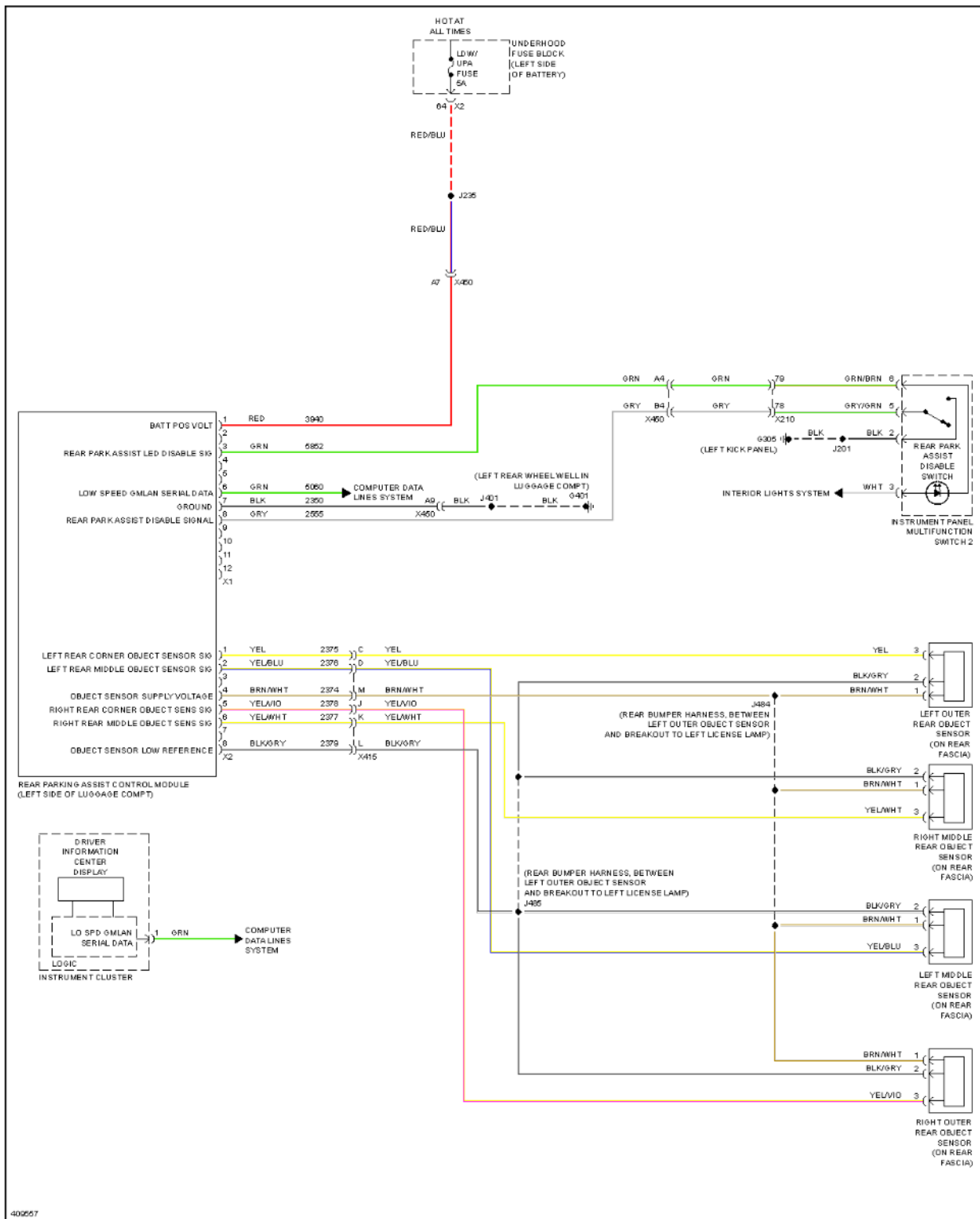
Fig. 86: Parking Assistant Circuit
