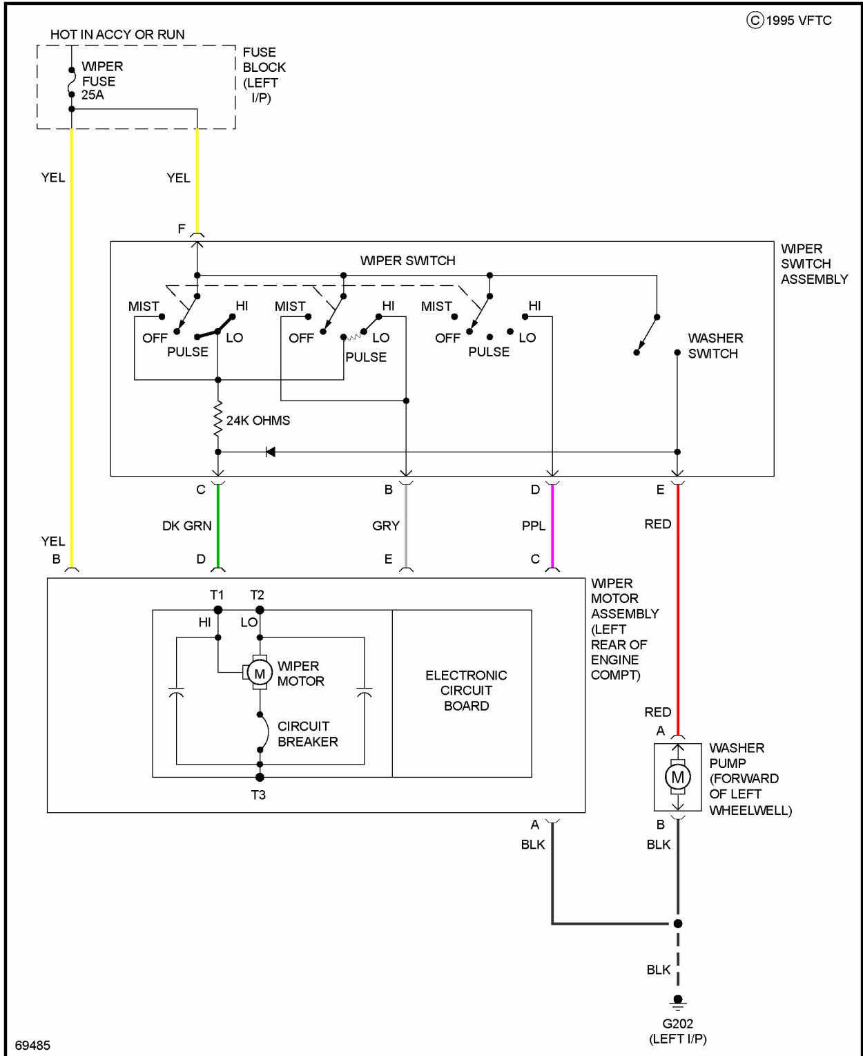
Fig. 46: Wiper/Washer Circuit
