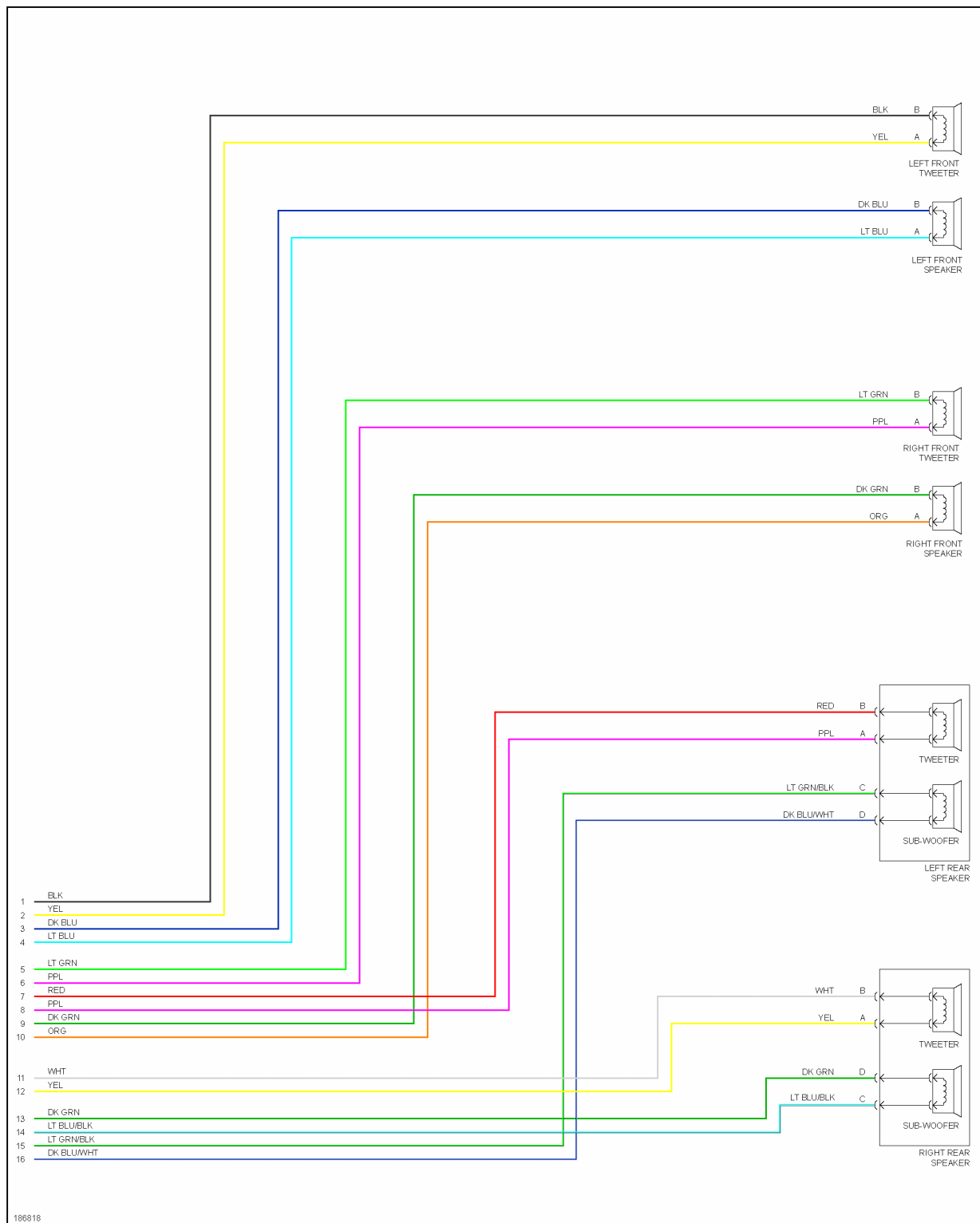
Fig. 32: Radio Circuit, U85 (2 of 2)
