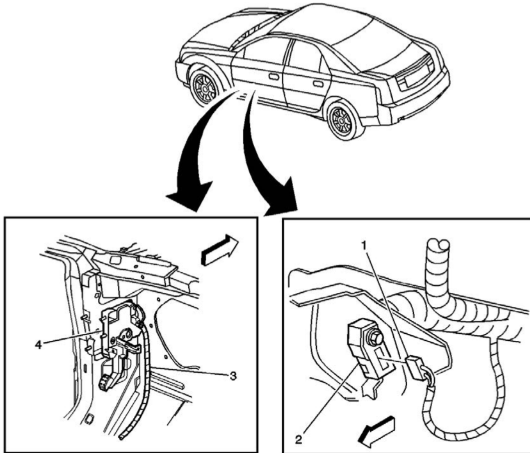
Fig. 2: Park Brake Subsystem Components Courtesy of GENERAL MOTORS CORP.
