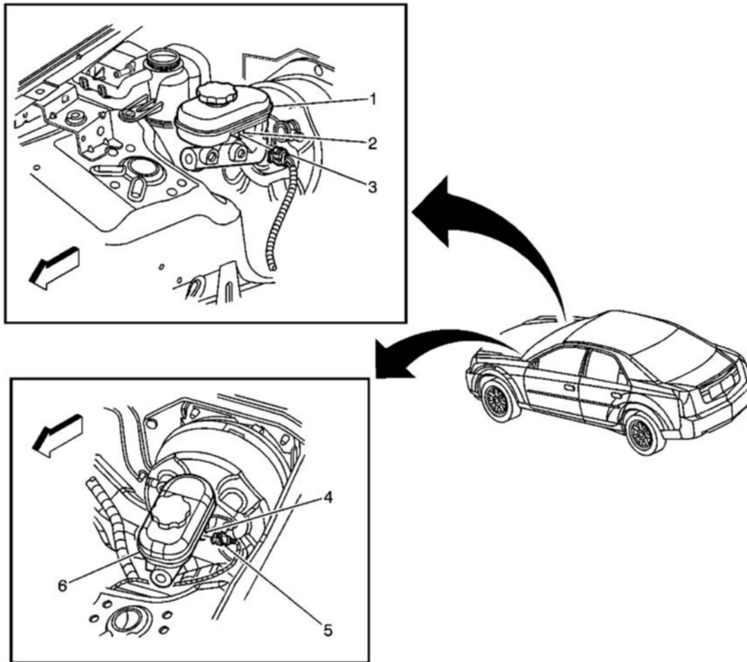
Fig. 3: Brake Fluid Level Switch Courtesy of GENERAL MOTORS CORP.
