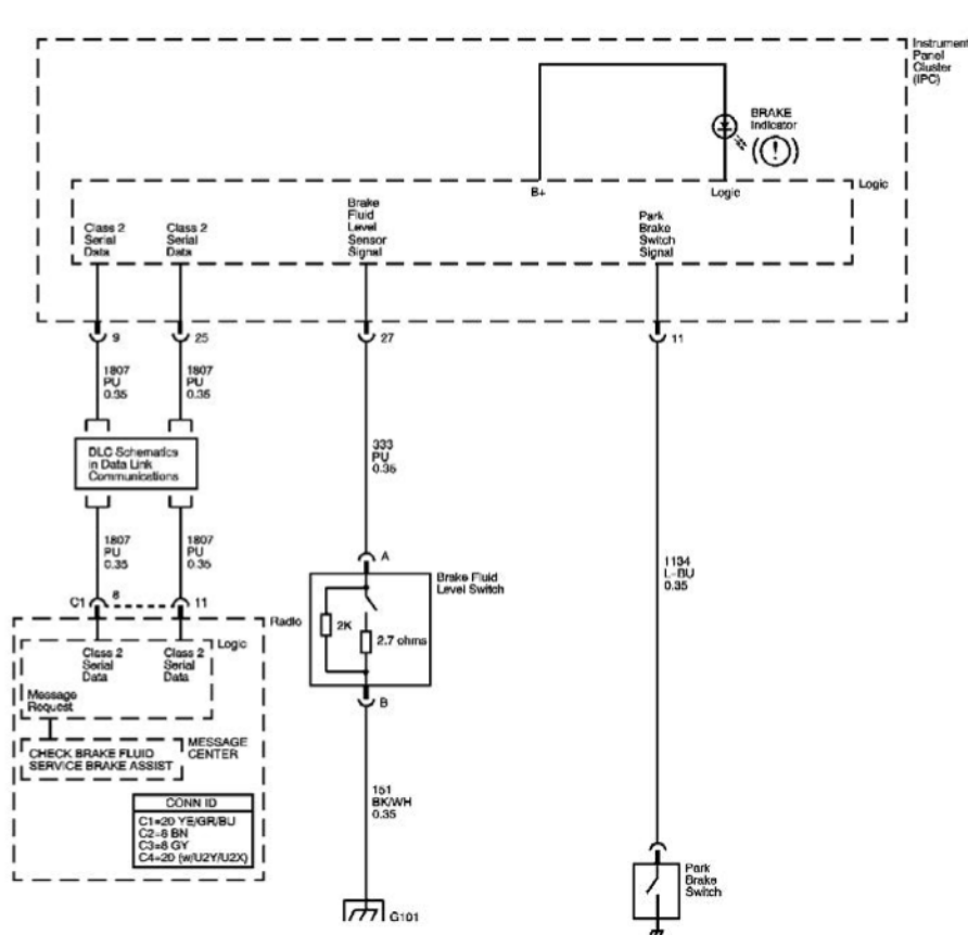
Fig. 1: Brake Warning System Schematic Courtesy of GENERAL MOTORS CORP.
