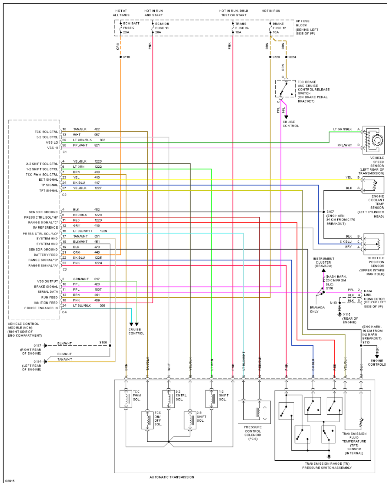
Fig. 36: 4.3L (VIN W), Transmission Circuit
