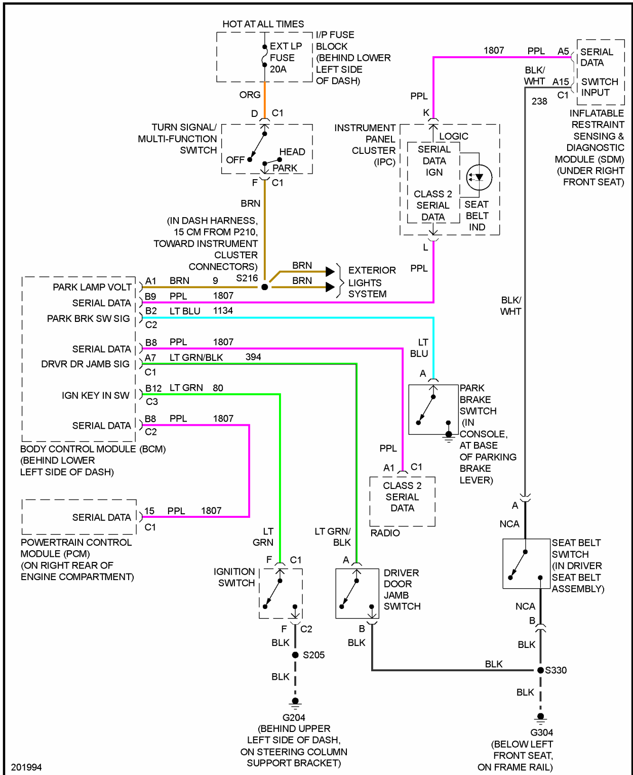
Fig. 41: Warning Systems Circuit
