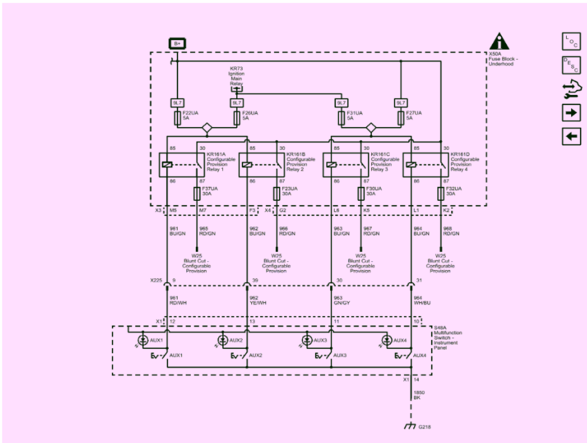
Fig. 2: Upfitter Provisions (E29) Courtesy of GENERAL MOTORS COMPANY
