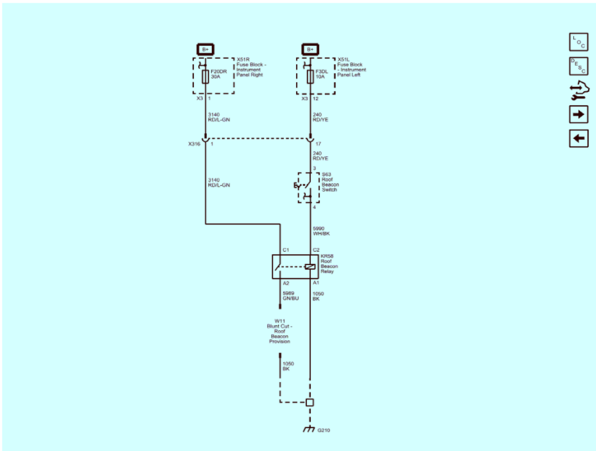
Fig. 3: Roof Beacon Provisions (TRW) Courtesy of GENERAL MOTORS COMPANY
