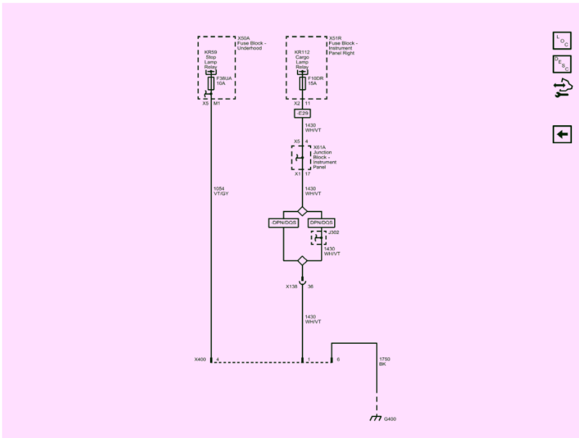
Fig. 4: Lighting Provisions - Rear of Frame Courtesy of GENERAL MOTORS COMPANY
