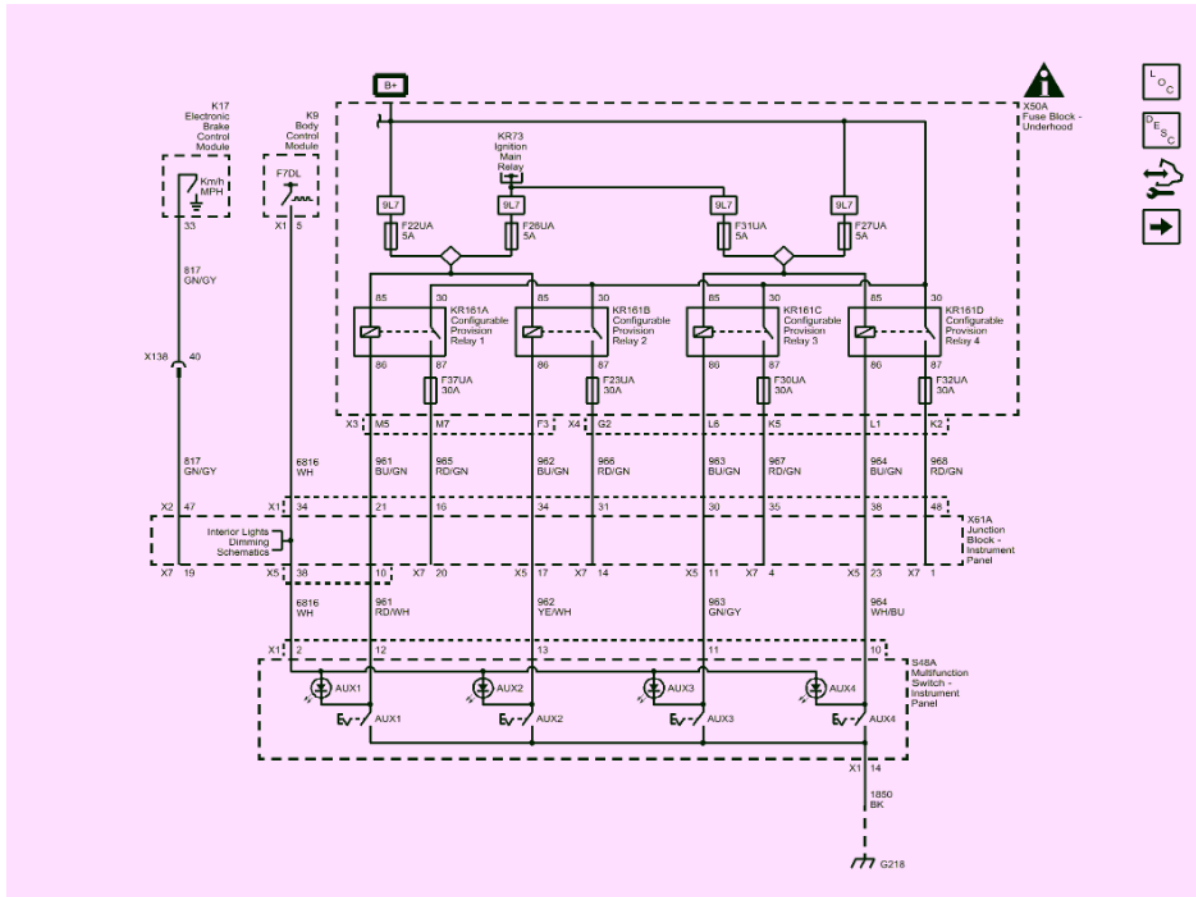
Fig. 1: Upfitter Provisions (except E29)
