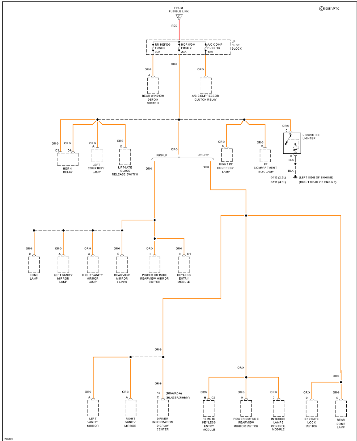
Fig. 22: Power Distribution Circuit (4 of 4)
