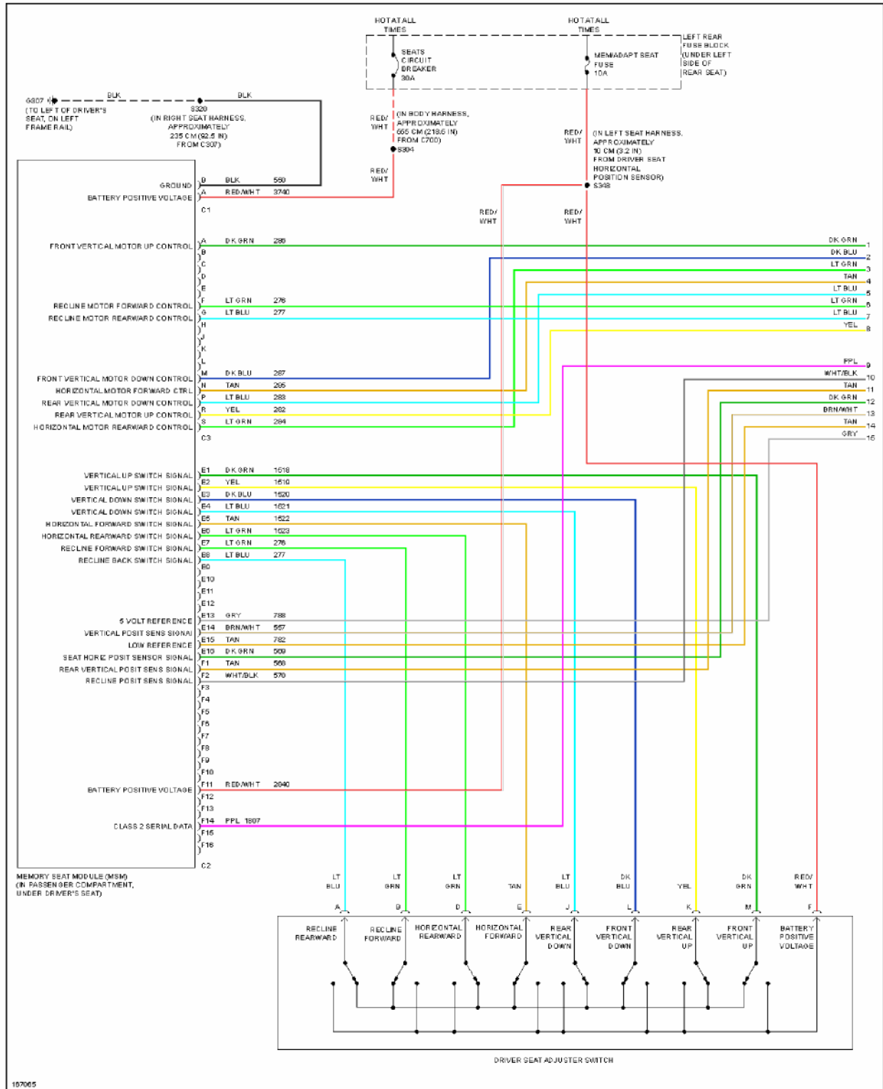
Fig. 36: Memory Seat Circuit (1 of 2)
