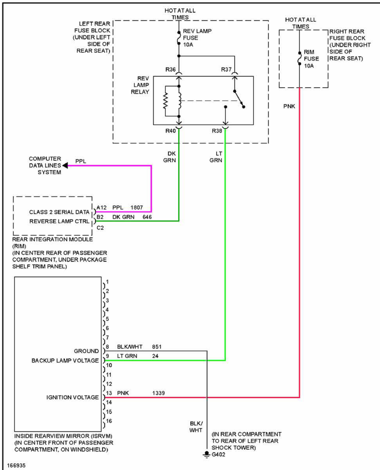
Fig. 48: Automatic Day/Night Mirror Circuit
