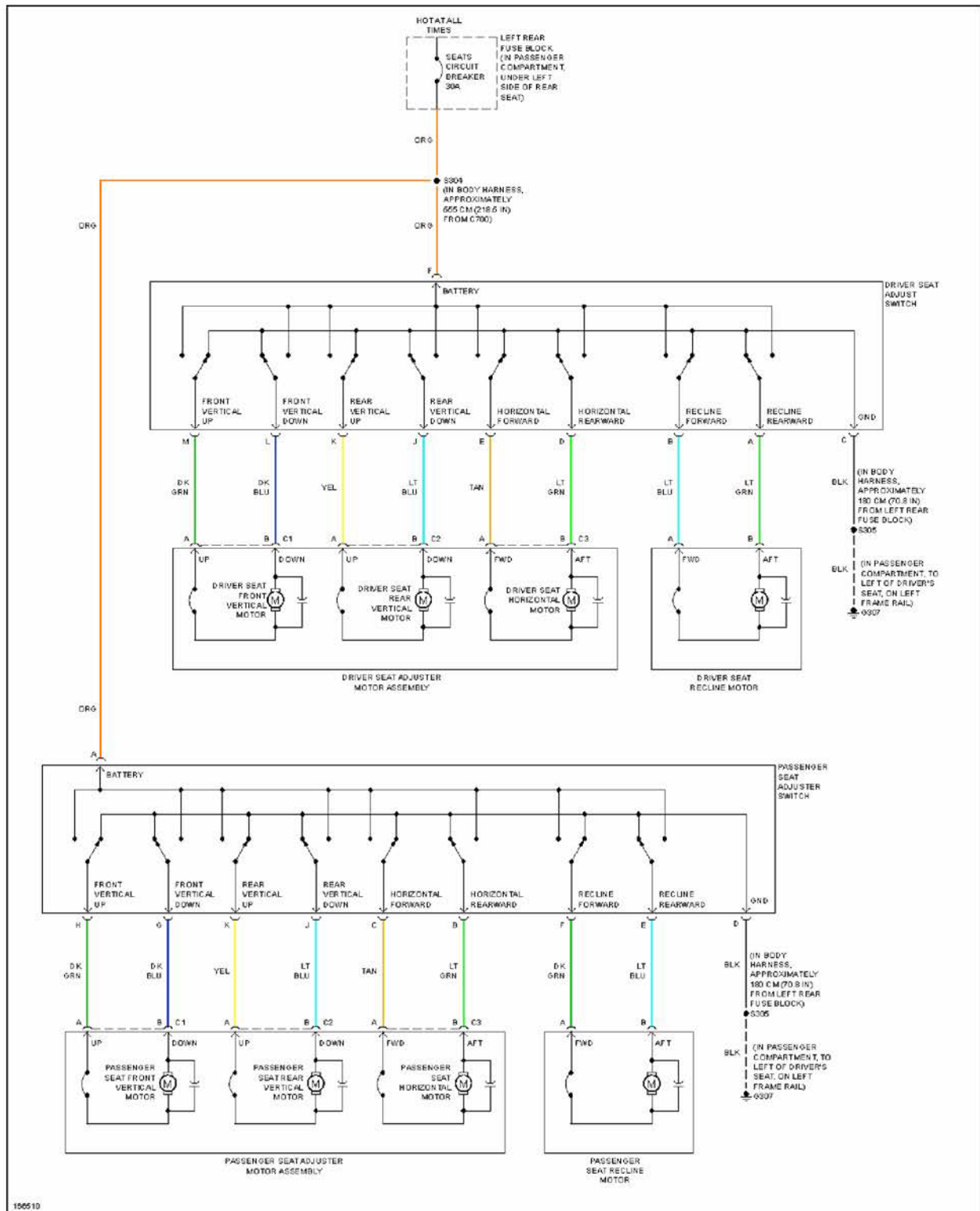
Fig. 51: Power Seats Circuit
