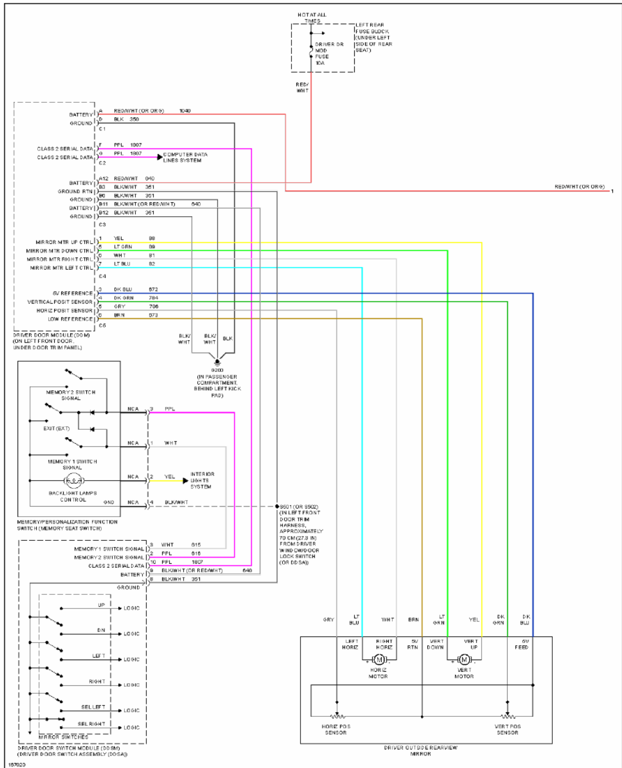
Fig. 34: Memory Mirrors Circuit (1 of 2)
