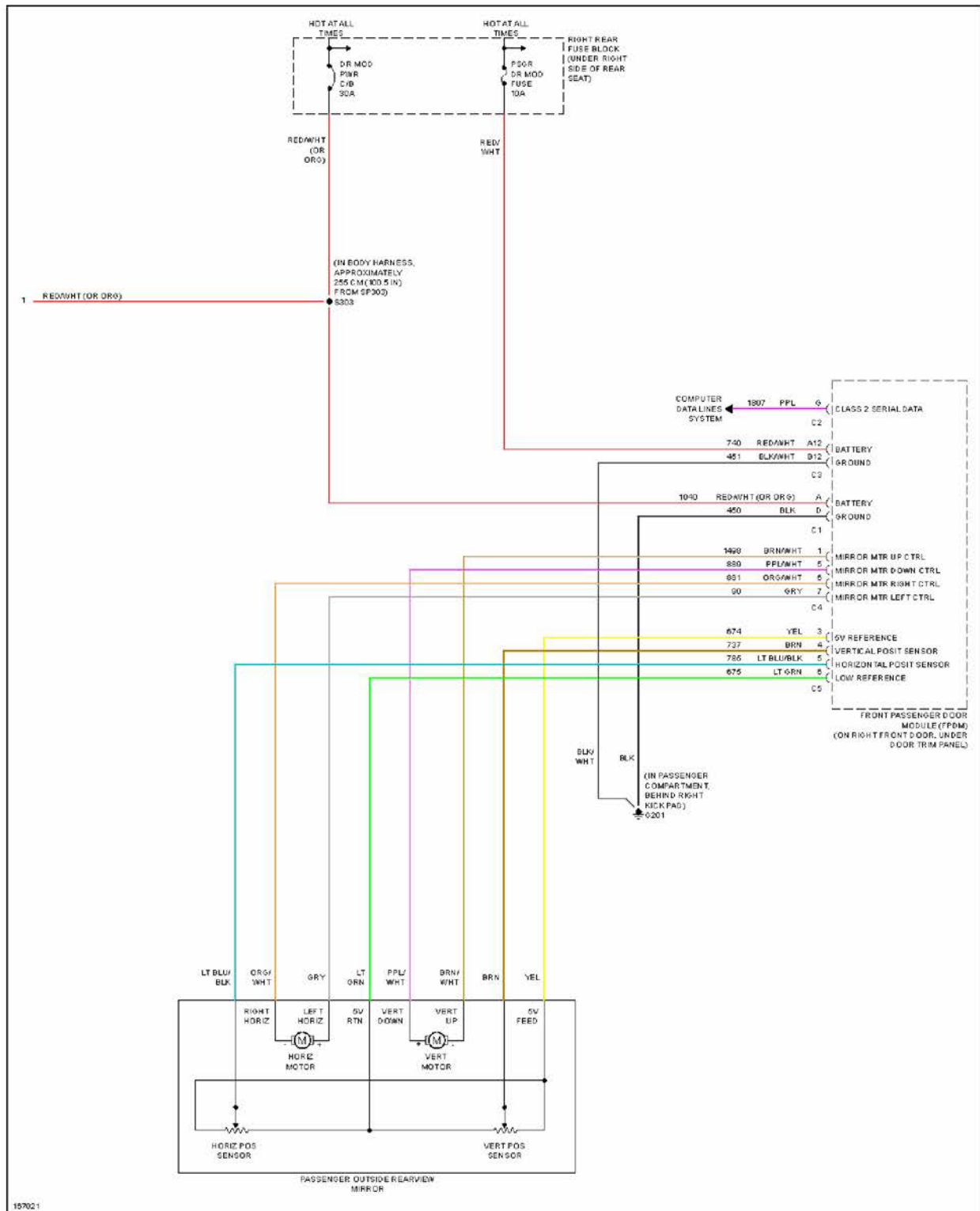
Fig. 35: Memory Mirrors Circuit (2 of 2)
