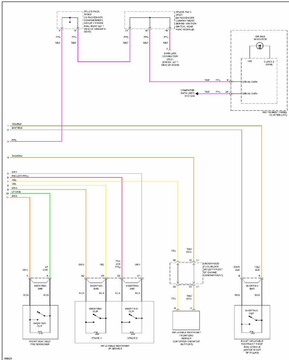
Fig. 64: Supplemental Restraints Circuit (2 of 2)
