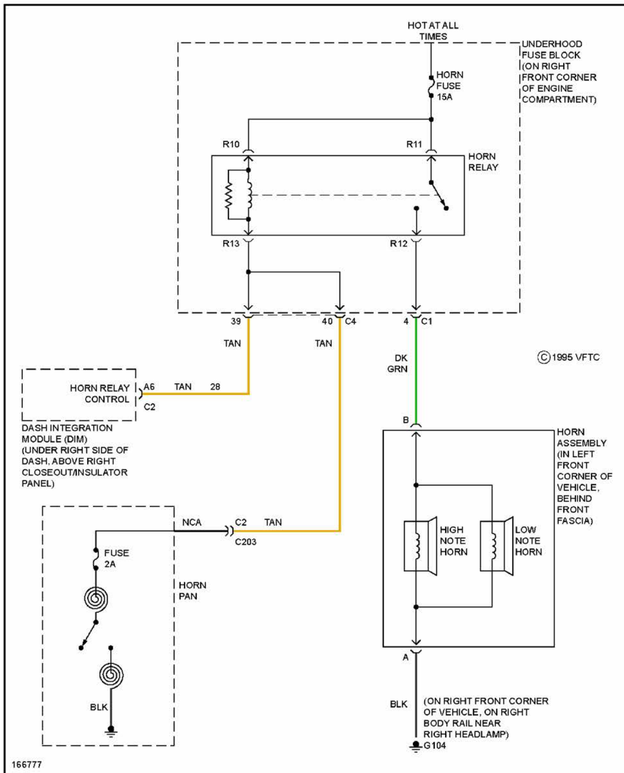
Fig. 28: Horn Circuit
