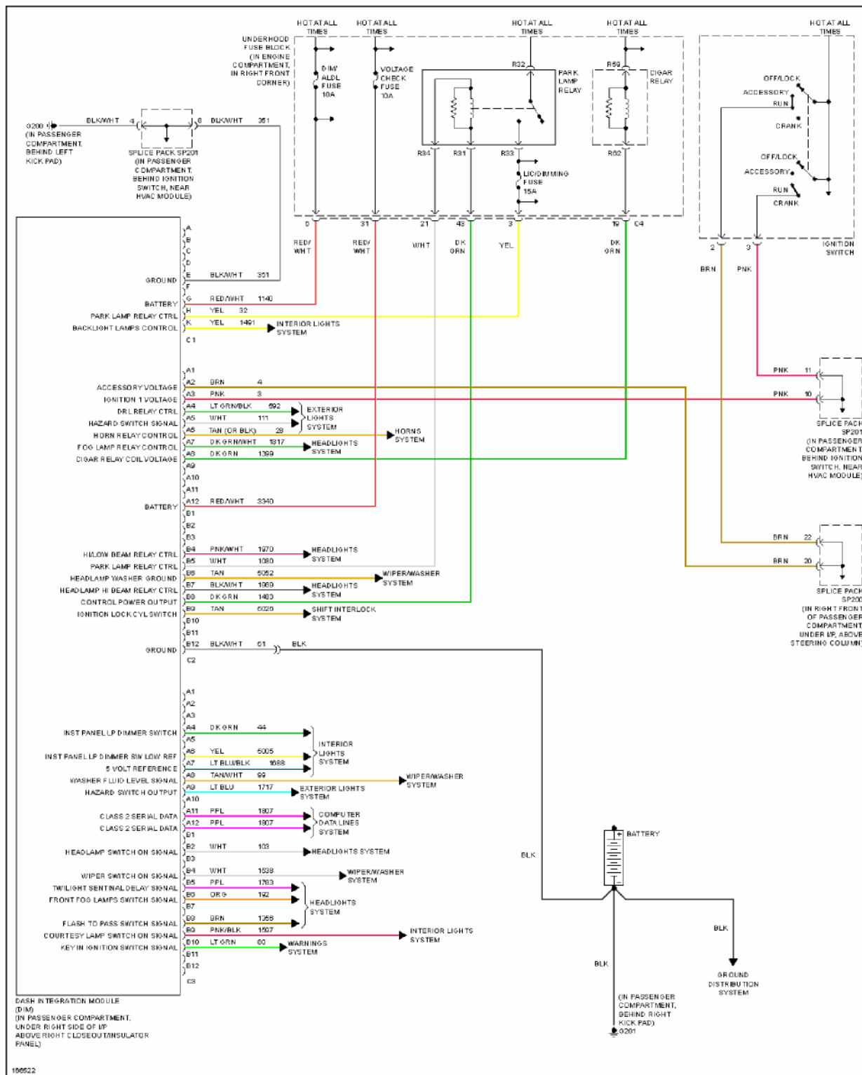
Fig. 9: Dash Integration Module Circuit
