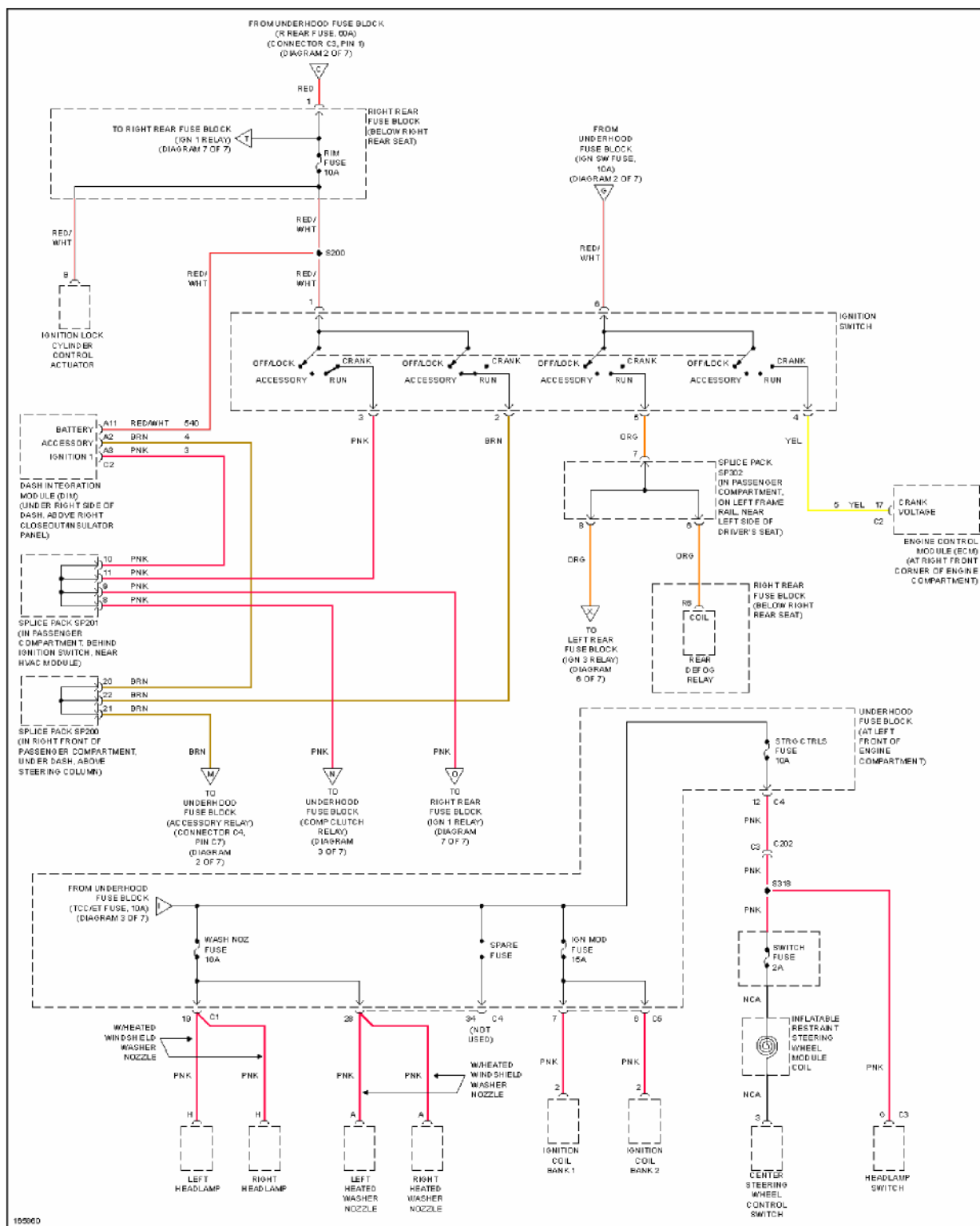
Fig. 42: Power Distribution Circuit (4 of 7)
