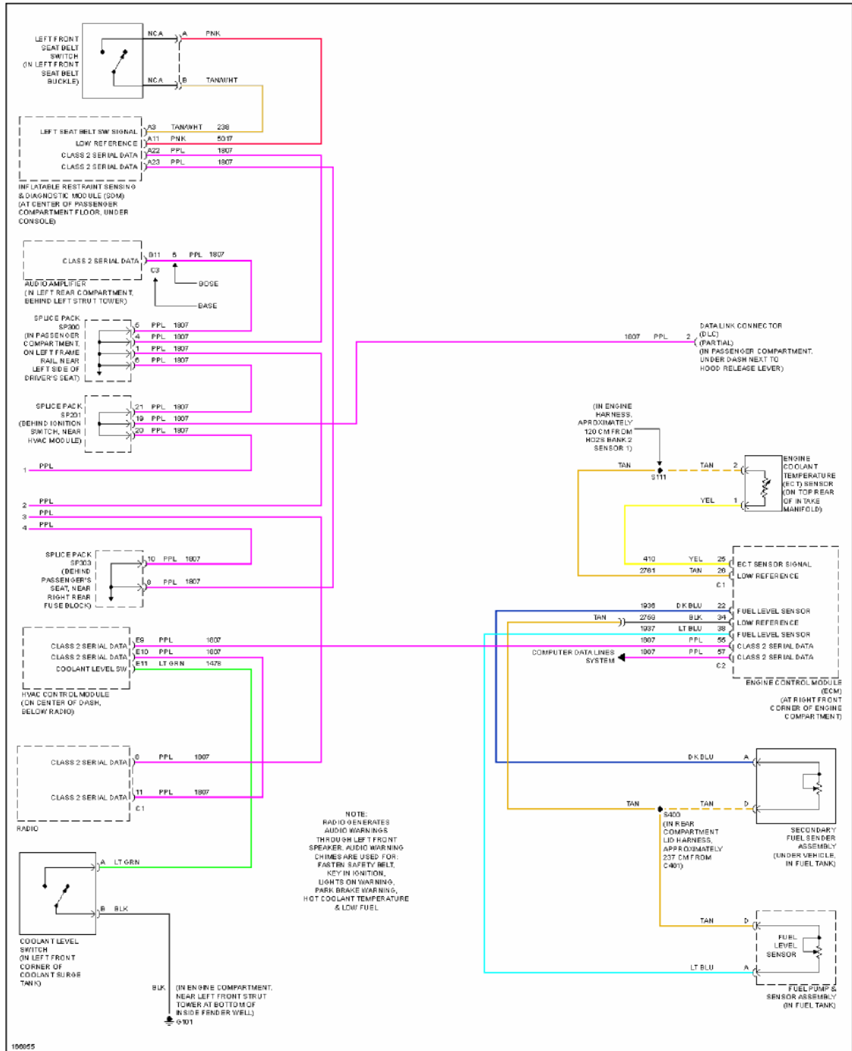
Fig. 69: Warning Systems Circuit (2 of 2)
