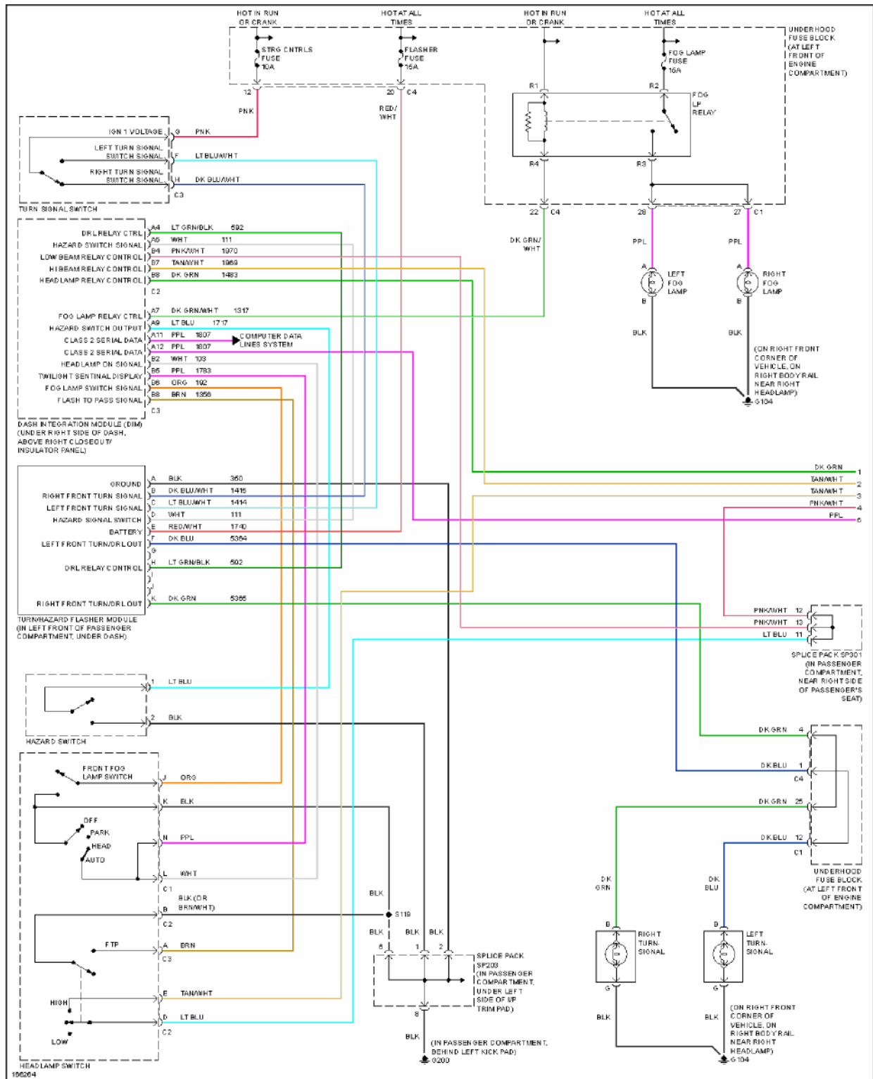
Fig. 26: Headlights Circuit (1 of 2)
