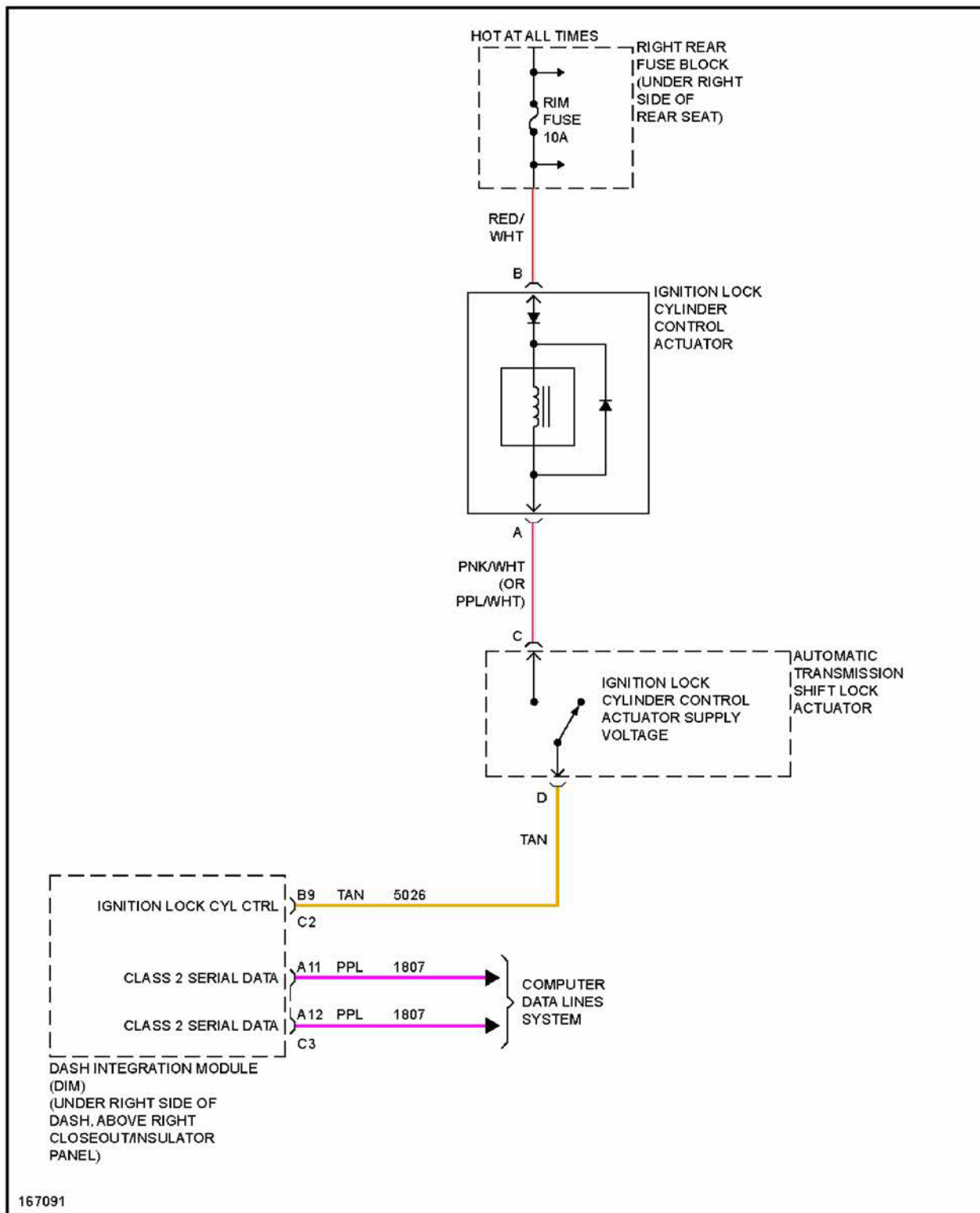
Fig. 59: Ignition Lock Solenoid Circuit
