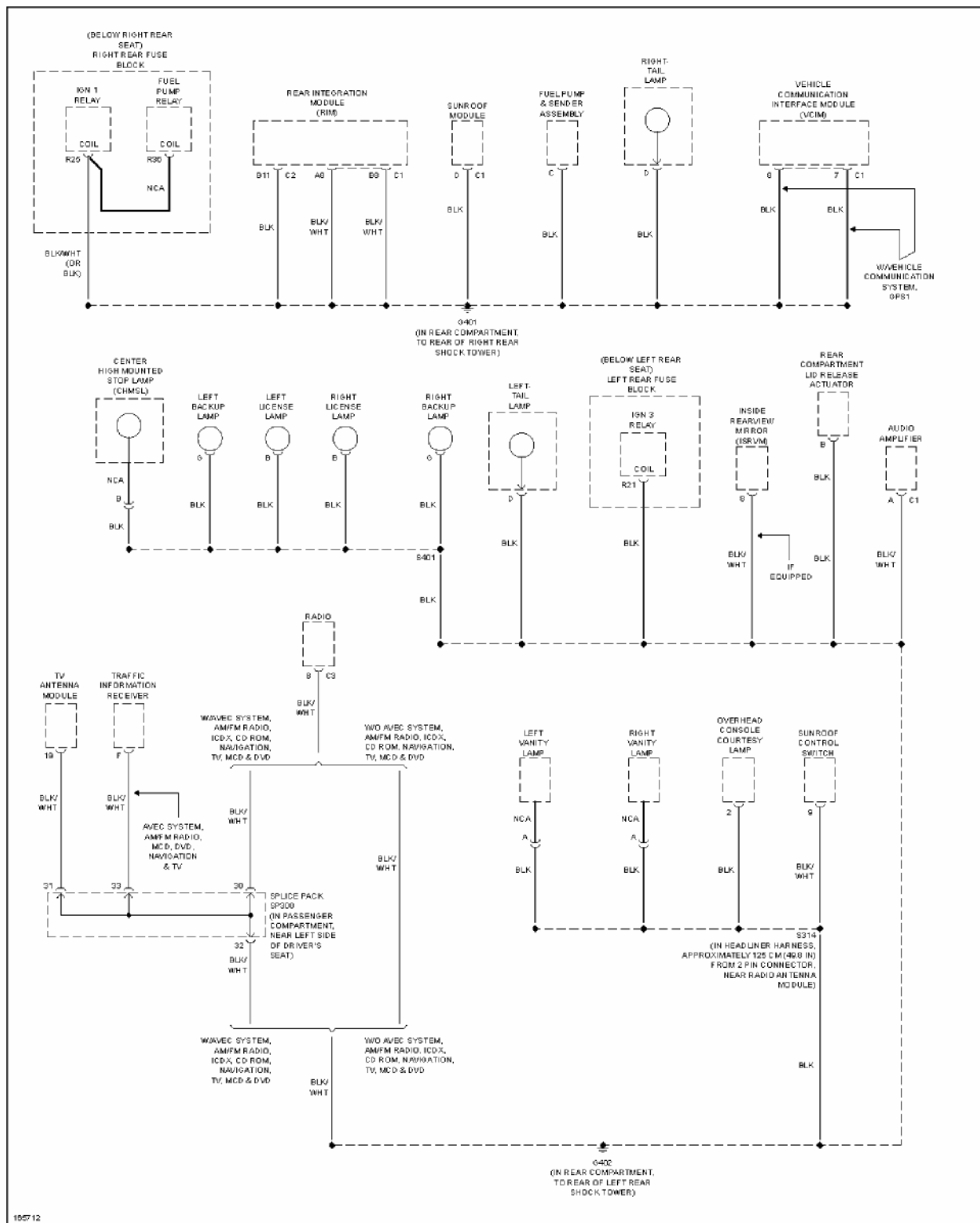
Fig. 25: Ground Distribution Circuit (4 of 4)
