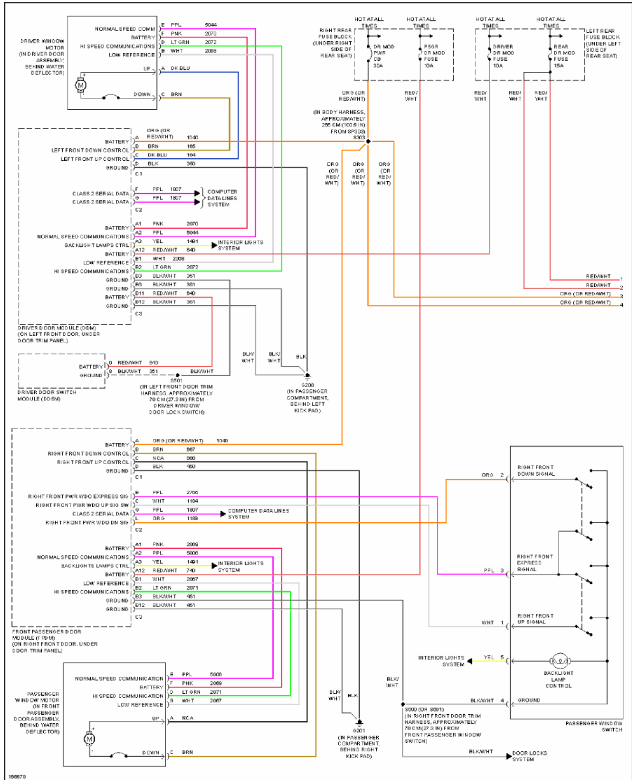
Fig. 53: Power Windows Circuit (1 of 2)
