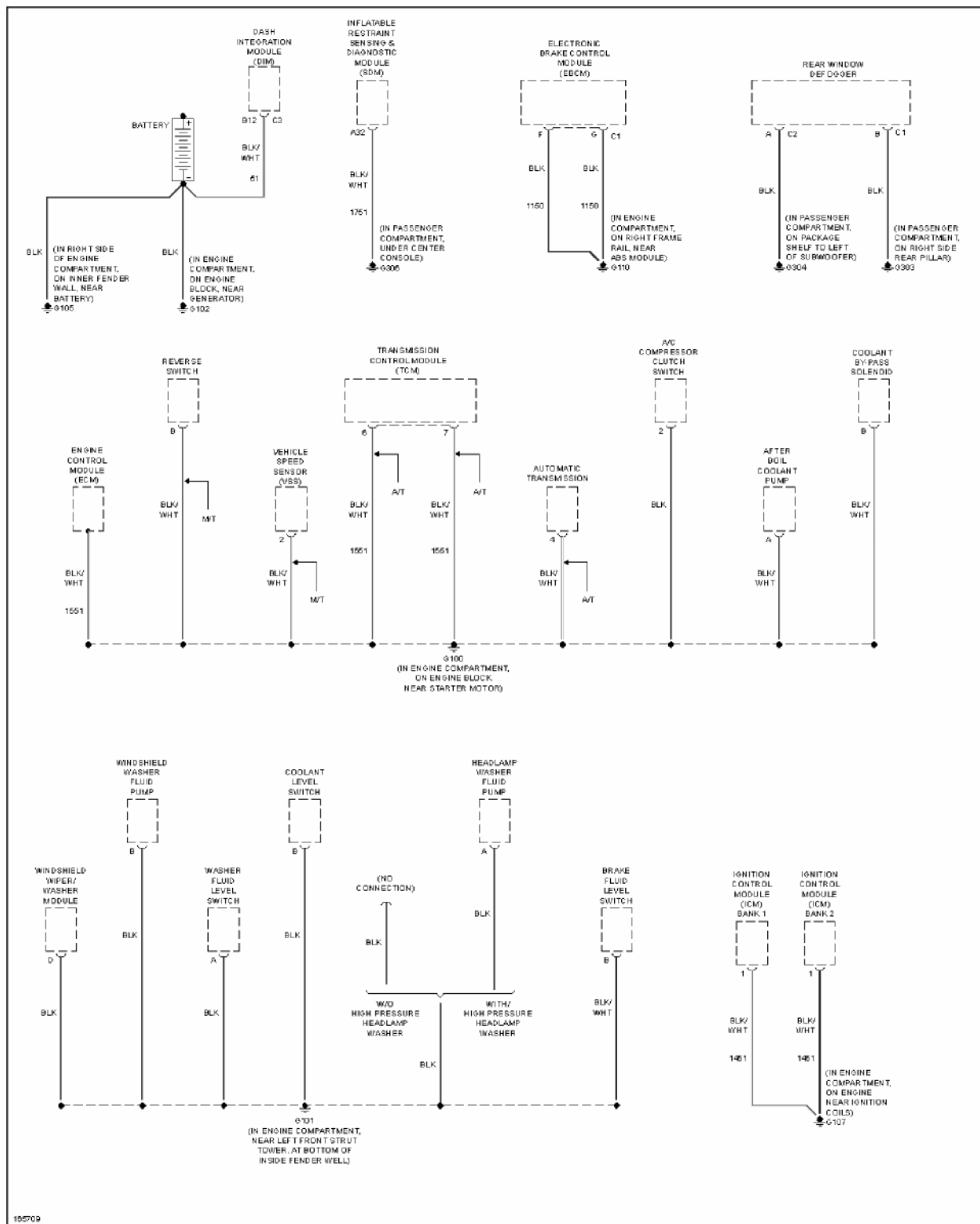
Fig. 22: Ground Distribution Circuit (1 of 4)
