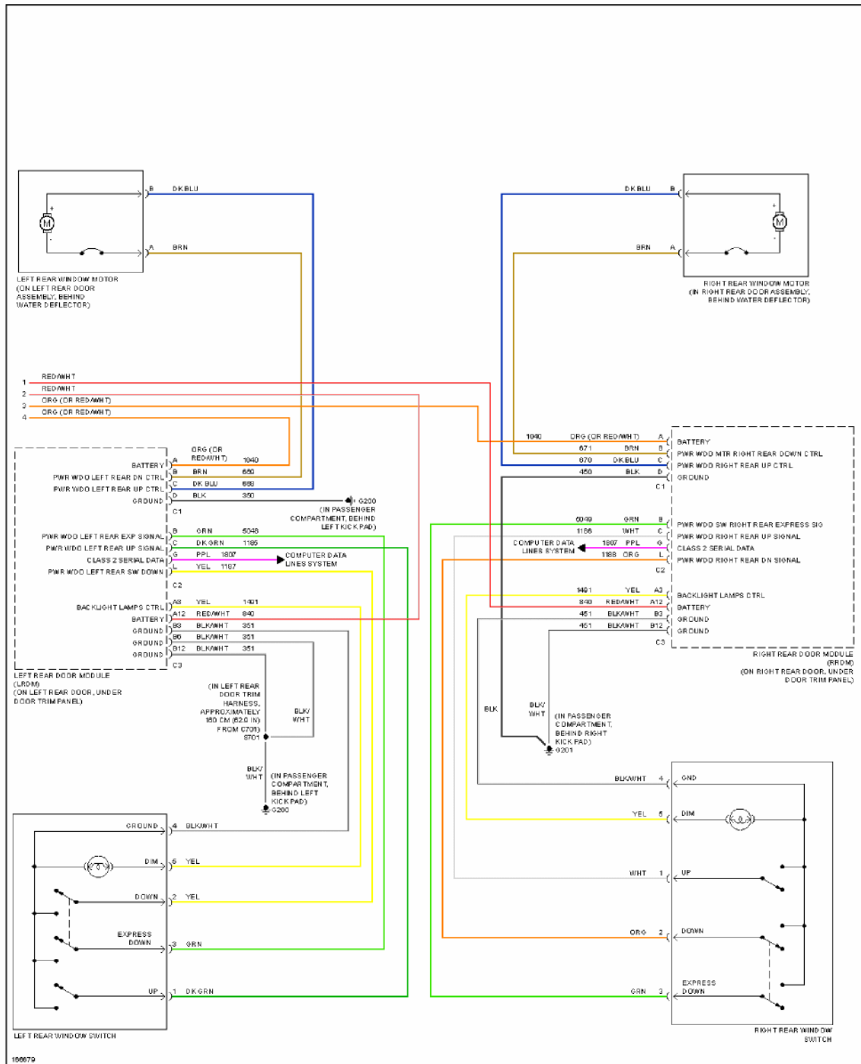
Fig. 54: Power Windows Circuit (2 of 2)
