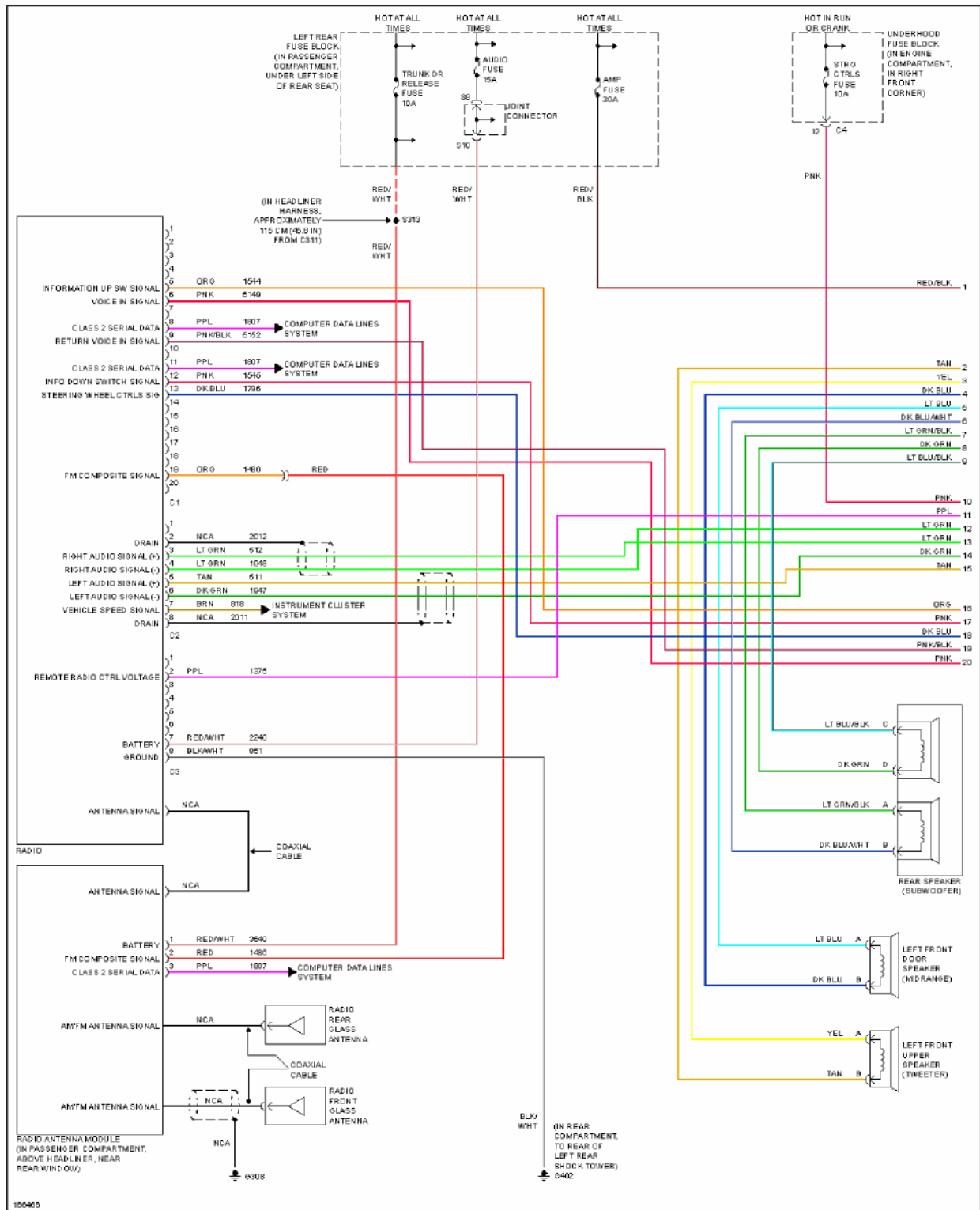
Fig. 55: Radio Circuit, Base (1 of 2)
