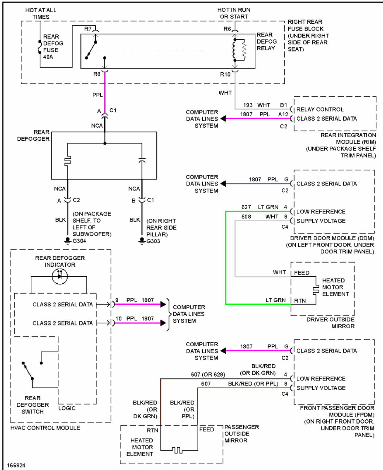
Fig. 14: Defoggers Circuit
