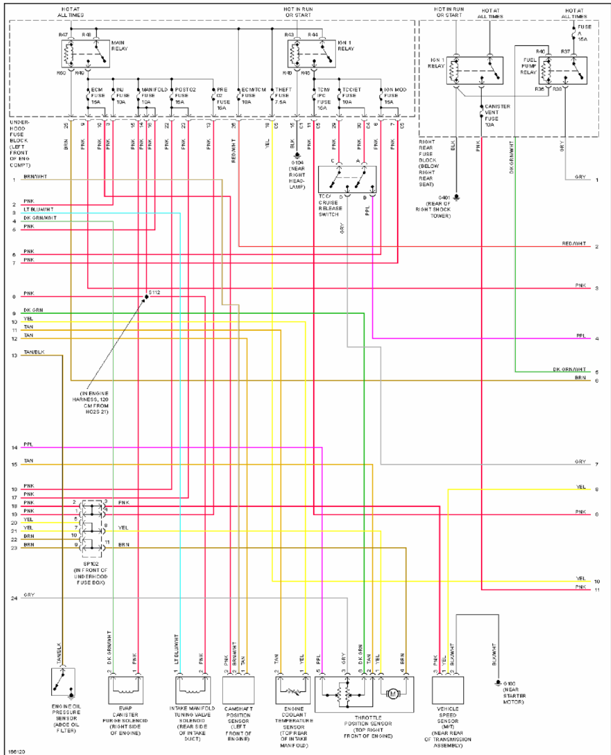
Fig. 17: 3.2L VIN N, Engine Performance Circuit (2 of 3)
