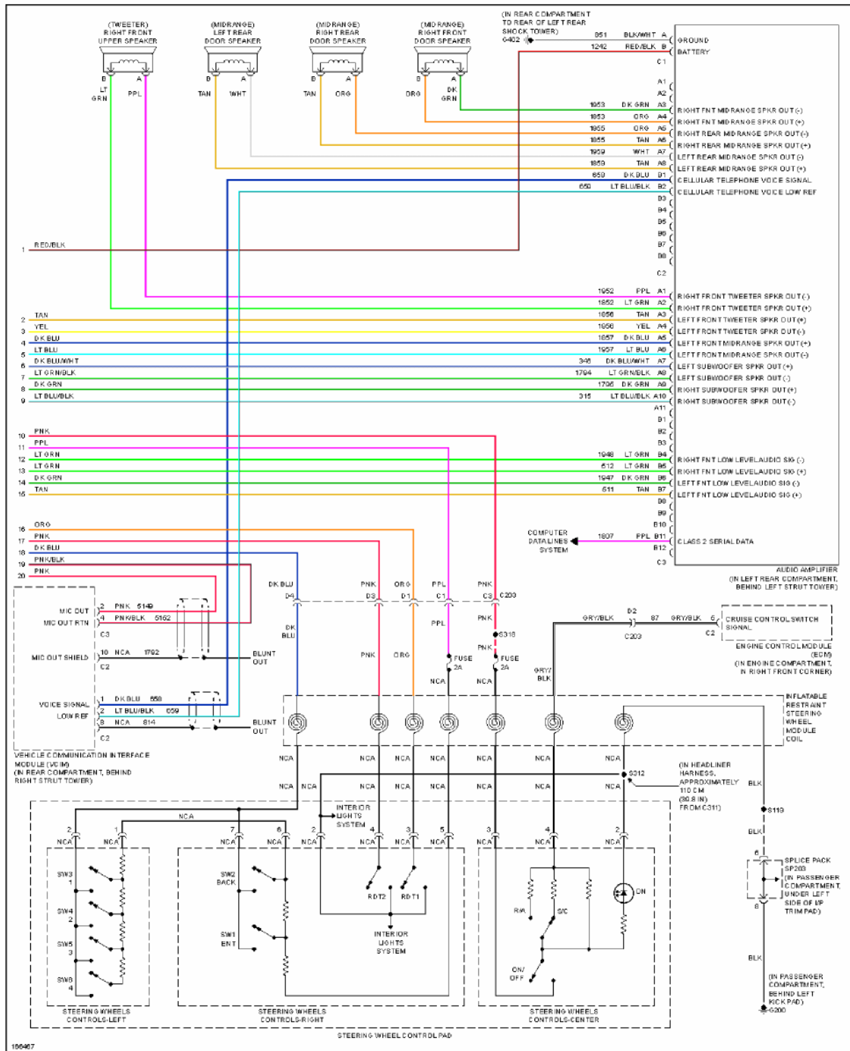
Fig. 56: Radio Circuit, Base (2 of 2)
