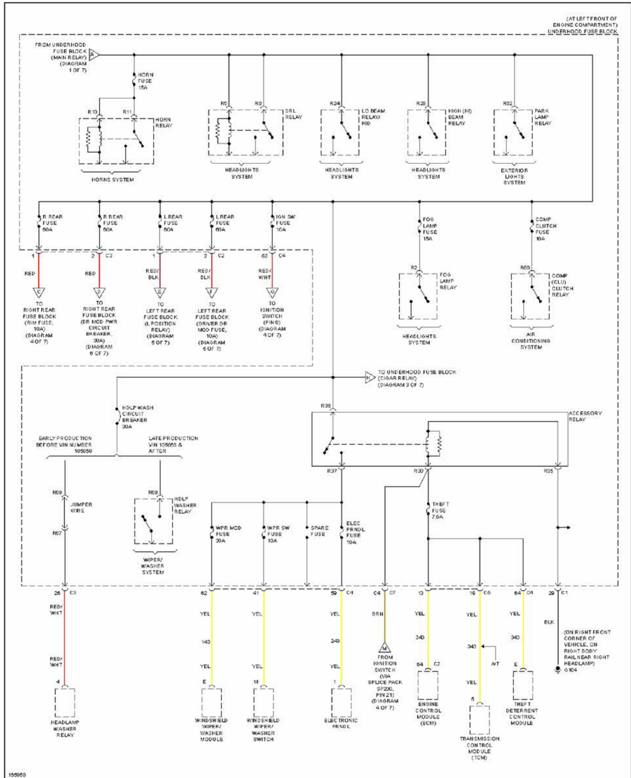
Fig. 40: Power Distribution Circuit (2 of 7)
