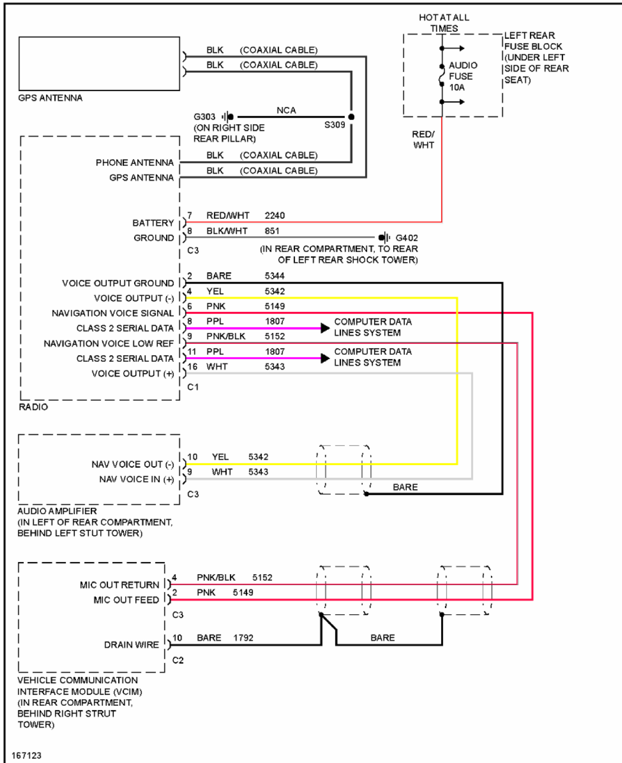
Fig. 38: Navigation Circuit
