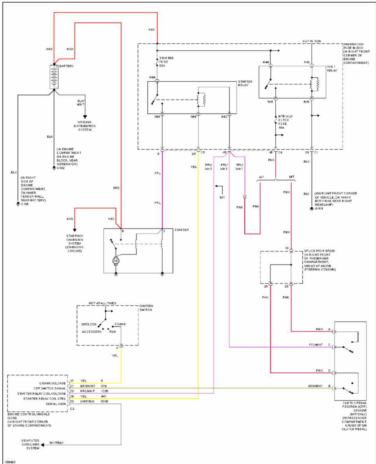
Fig. 62: Starting Circuit
