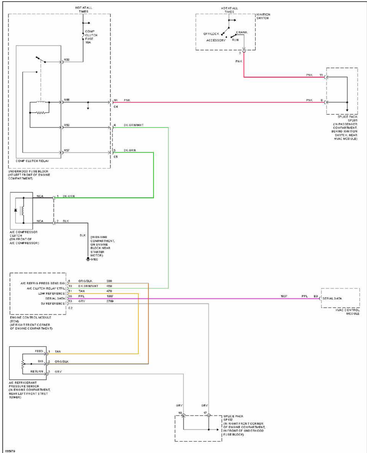
Fig. 4: Compressor Circuit
