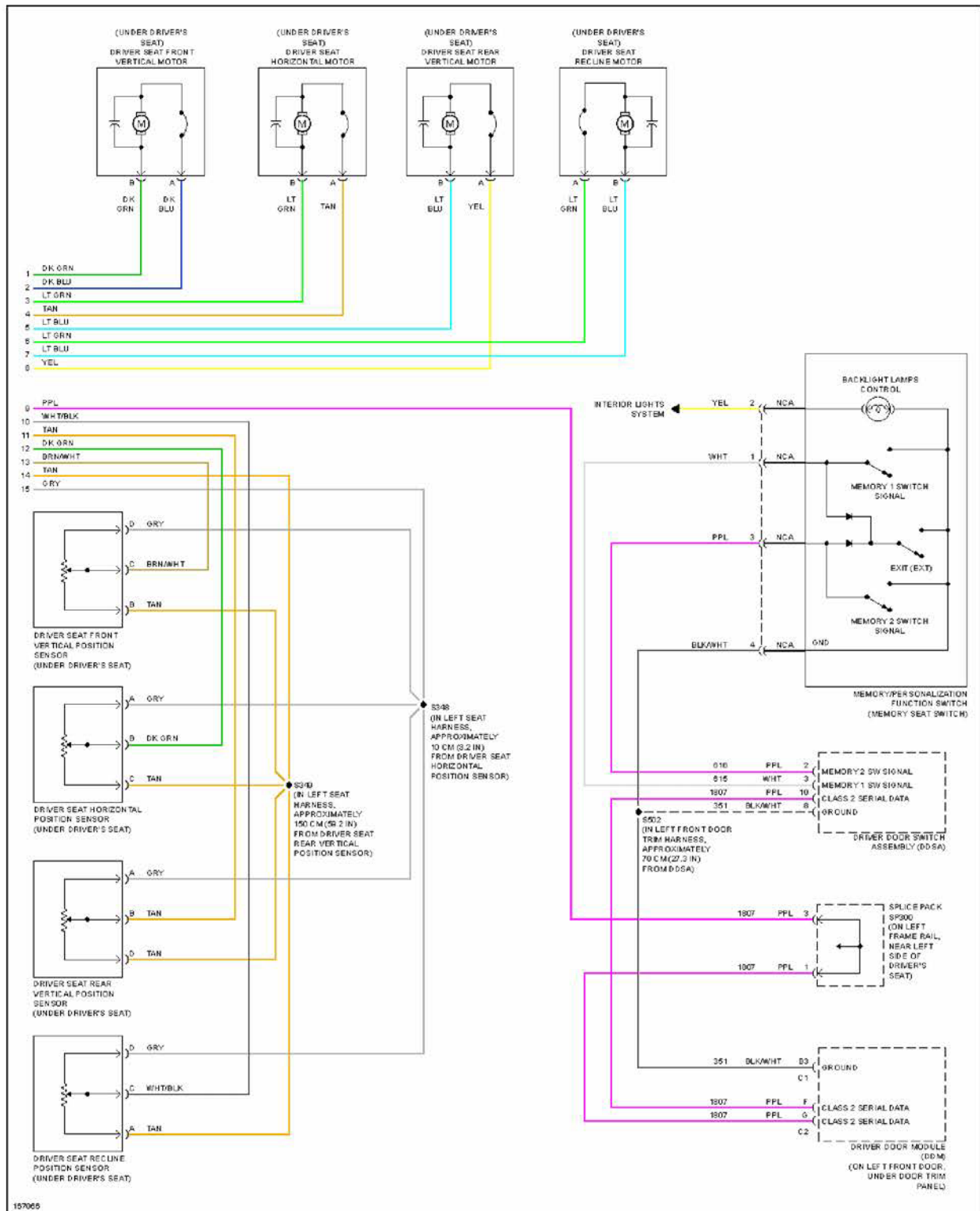
Fig. 37: Memory Seat Circuit (2 of 2)
