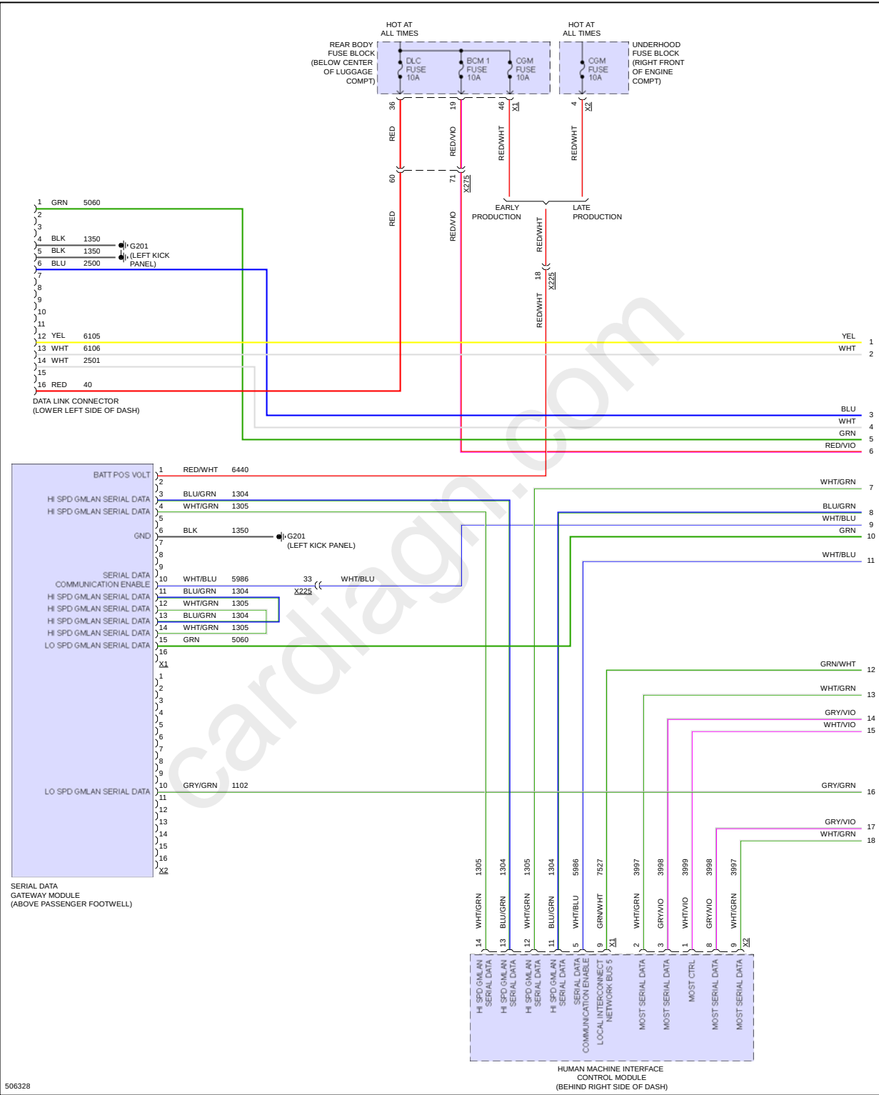
Fig 1: Computer Data Lines Circuit (1 of 6)
