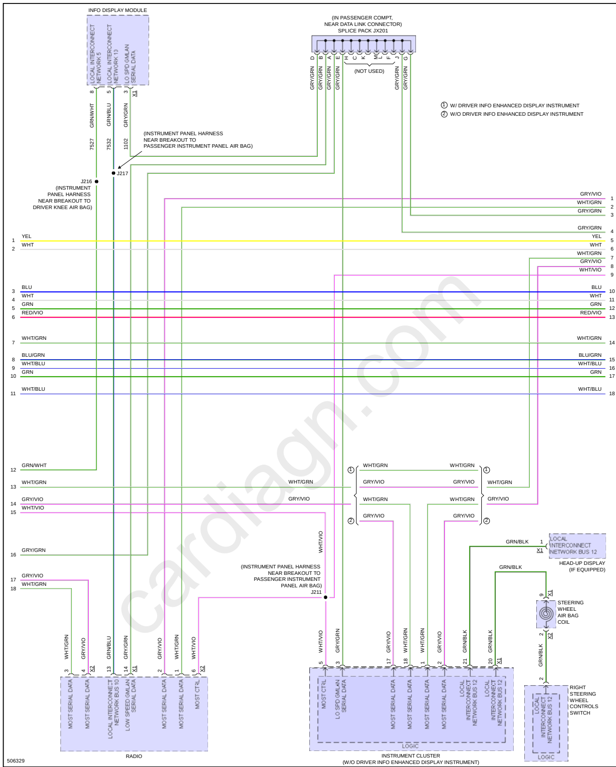
Fig 2: Computer Data Lines Circuit (2 of 6)
