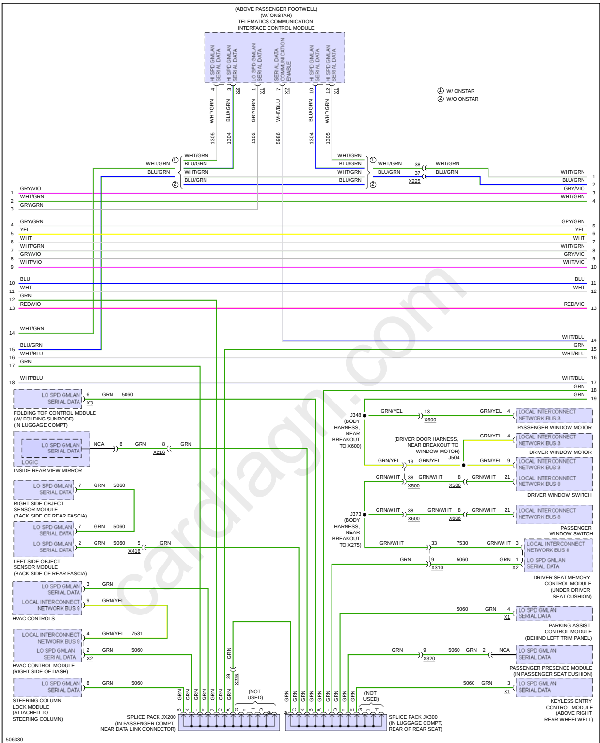
Fig 3: Computer Data Lines Circuit (3 of 6)
