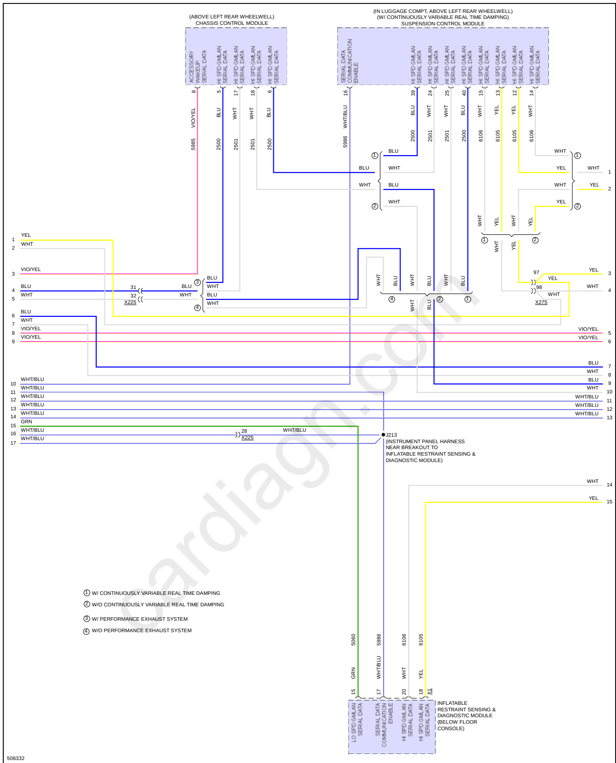
Fig 5: Computer Data Lines Circuit (5 of 6)
