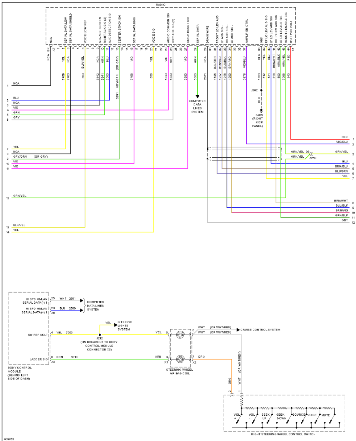
Fig. 115: Radio Circuit, W/ Amplifier (3 of 4)
