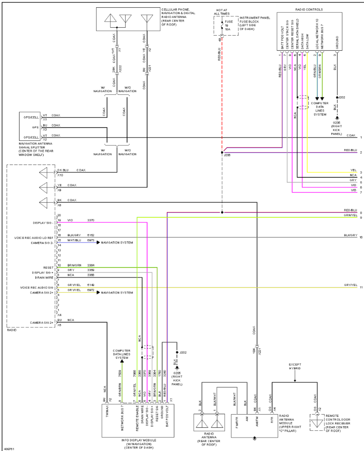
Fig. 113: Radio Circuit, W/ Amplifier (1 of 4)
