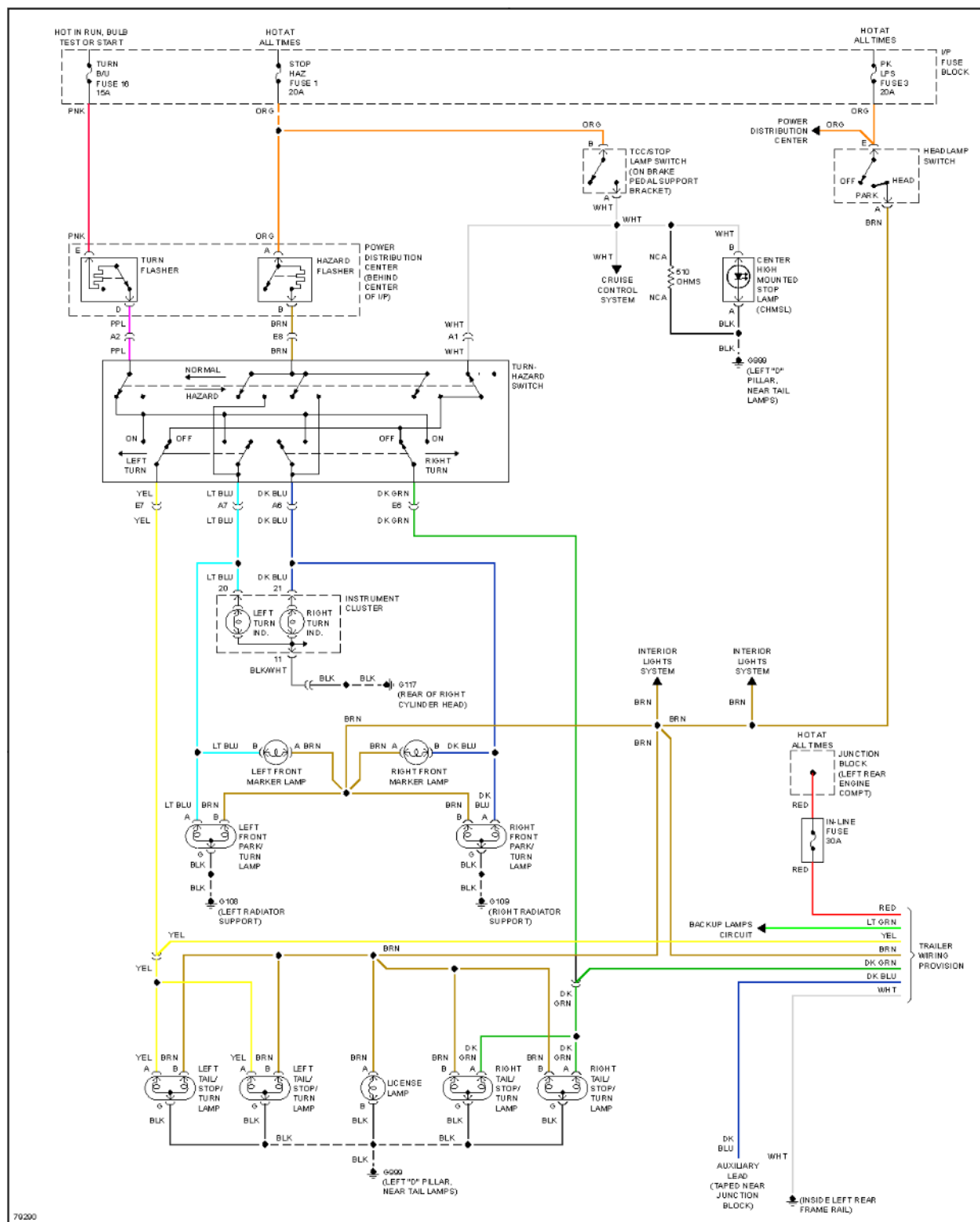
Fig. 11: Exterior Lamps Circuit
