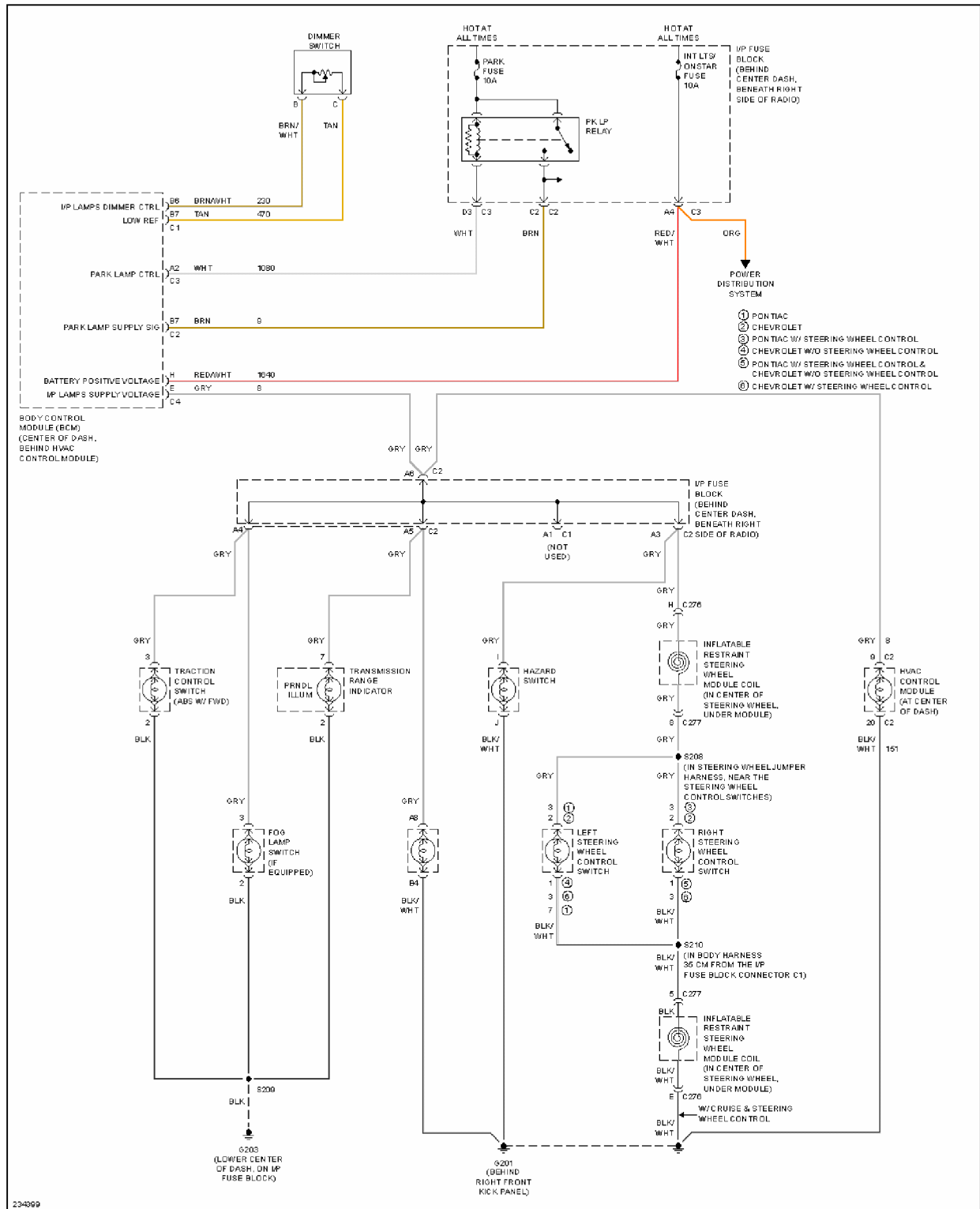
Fig. 26: Instrument Illumination Circuit
