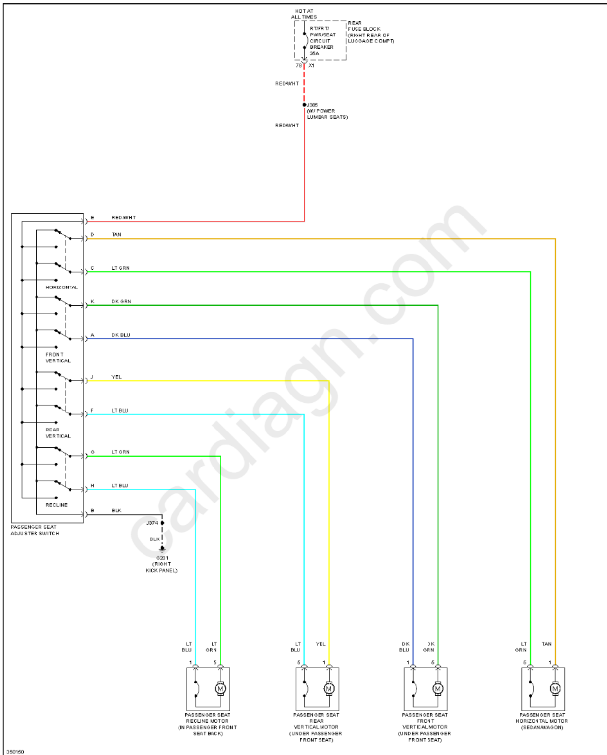
Fig. 93: Passenger Power Seat Circuit
