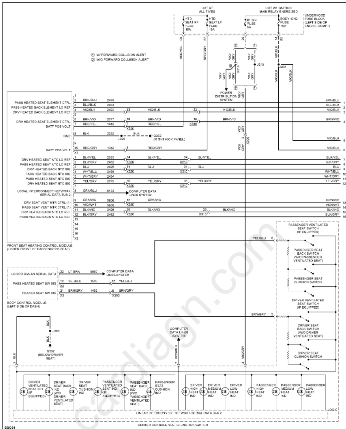
Fig. 102: Front Heated Seats Circuit (1 of 3)
