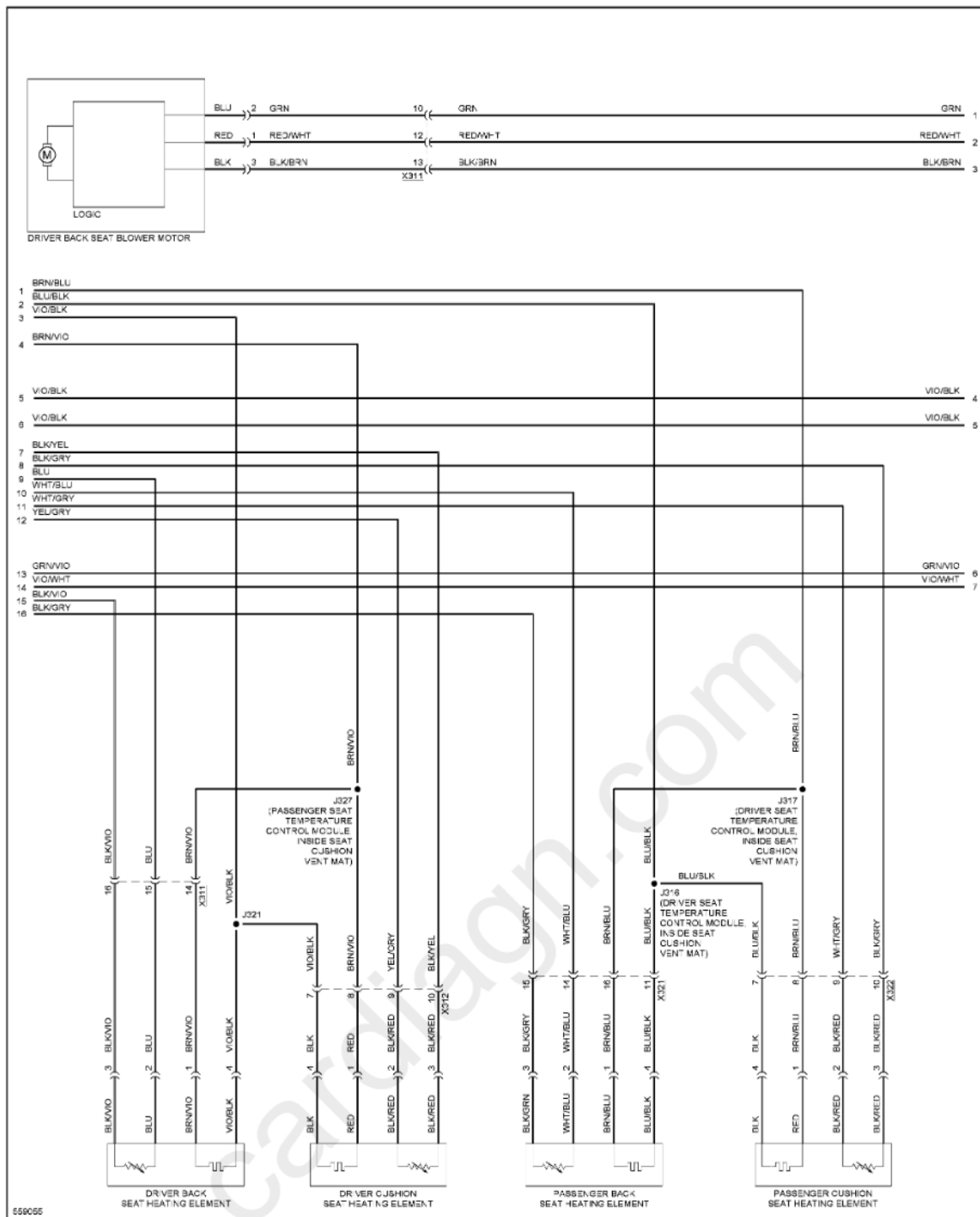
Fig. 103: Front Heated Seats Circuit (2 of 3)
