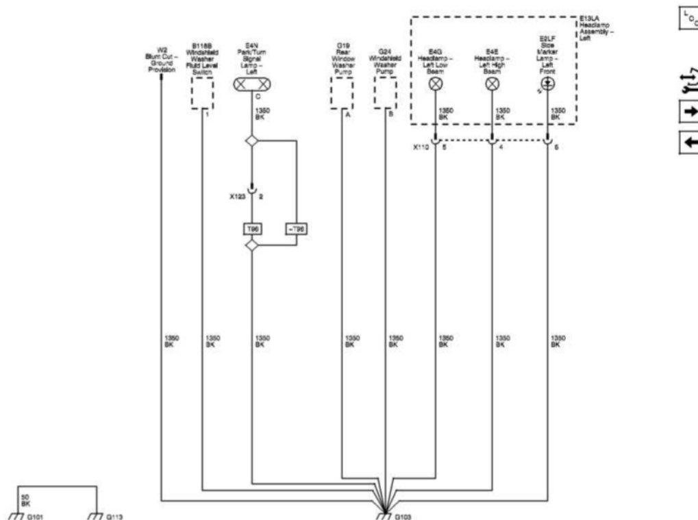
Fig. 52: G101, G103 And G113 (X88) Wiring Schematics Courtesy of GENERAL MOTORS COMPANY
