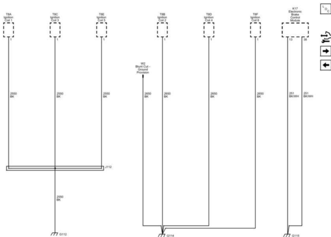
Fig. 58: G112, G114 and G115 Wiring Schematics Courtesy of GENERAL MOTORS COMPANY
