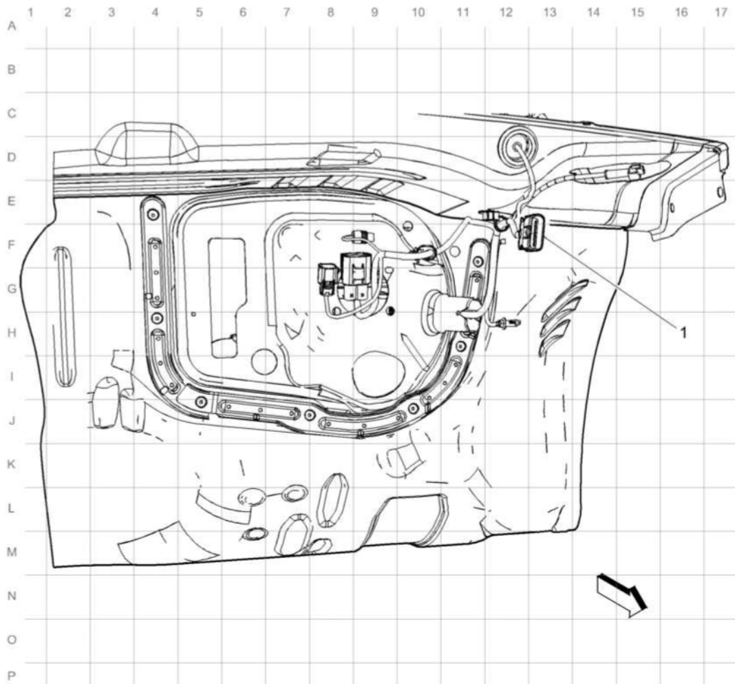
Fig. 4: Instrument Panel Harness Routing - Engine Compartment Courtesy of GENERAL MOTORS COMPANY
