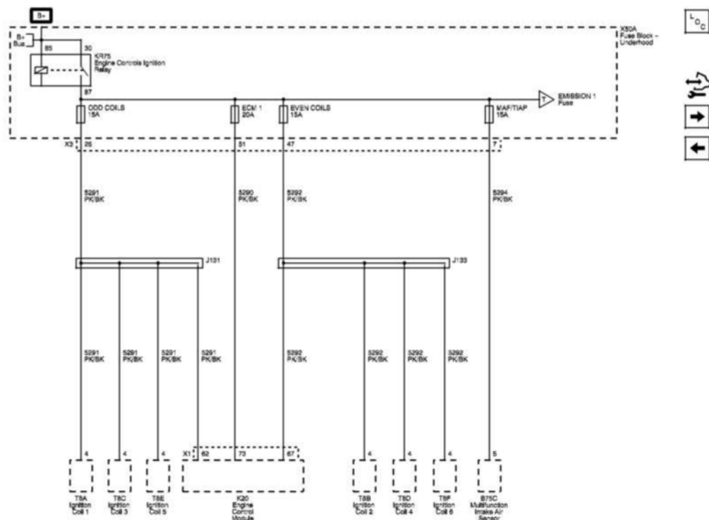
Fig. 40: ECM 1, EVEN COILS, MAF/TIAP And ODD COILS Wiring Schematics Courtesy of GENERAL MOTORS COMPANY
