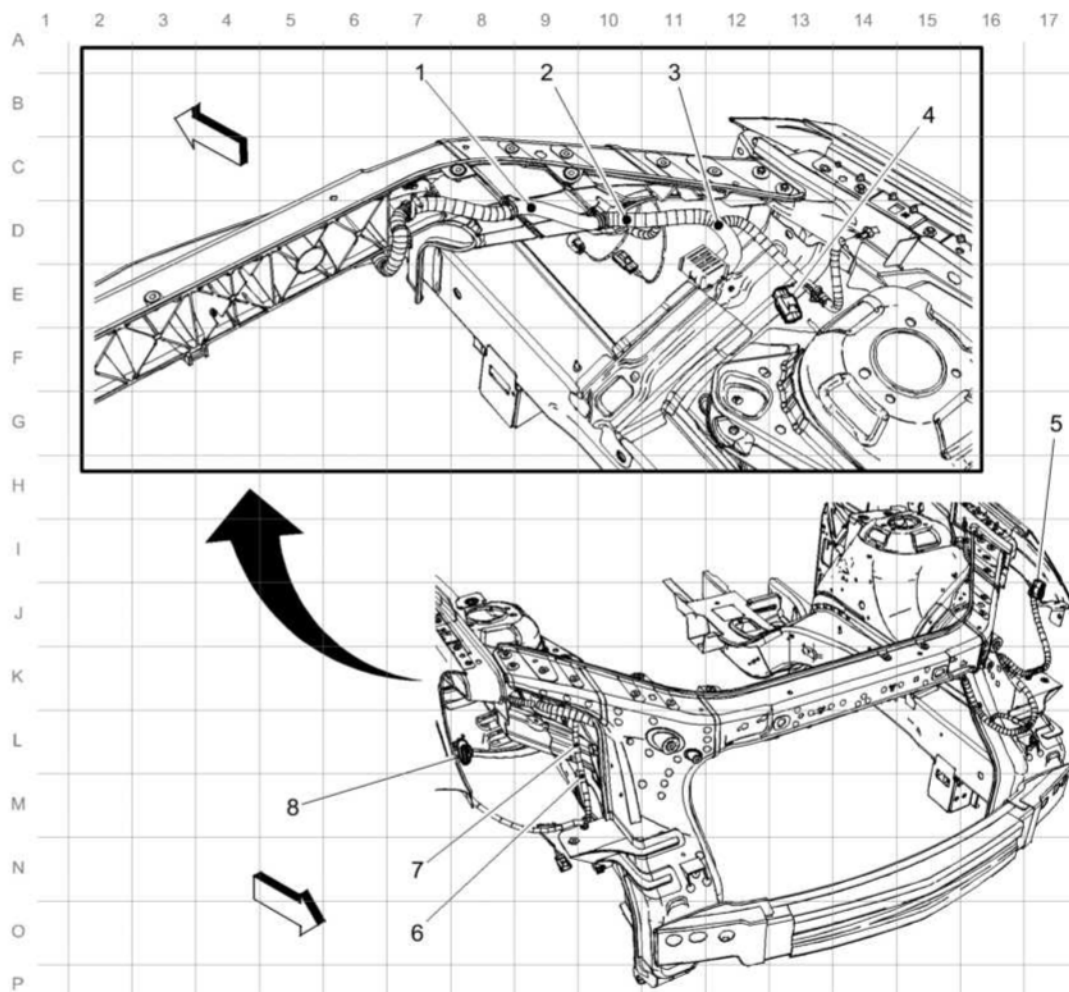
Fig. 24: Forward Lamp Harness Routing
