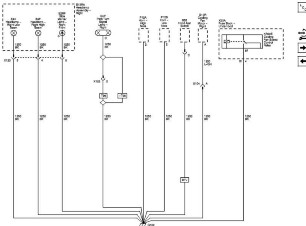
Fig. 55: G102 (X88) Wiring Schematics Courtesy of GENERAL MOTORS COMPANY
