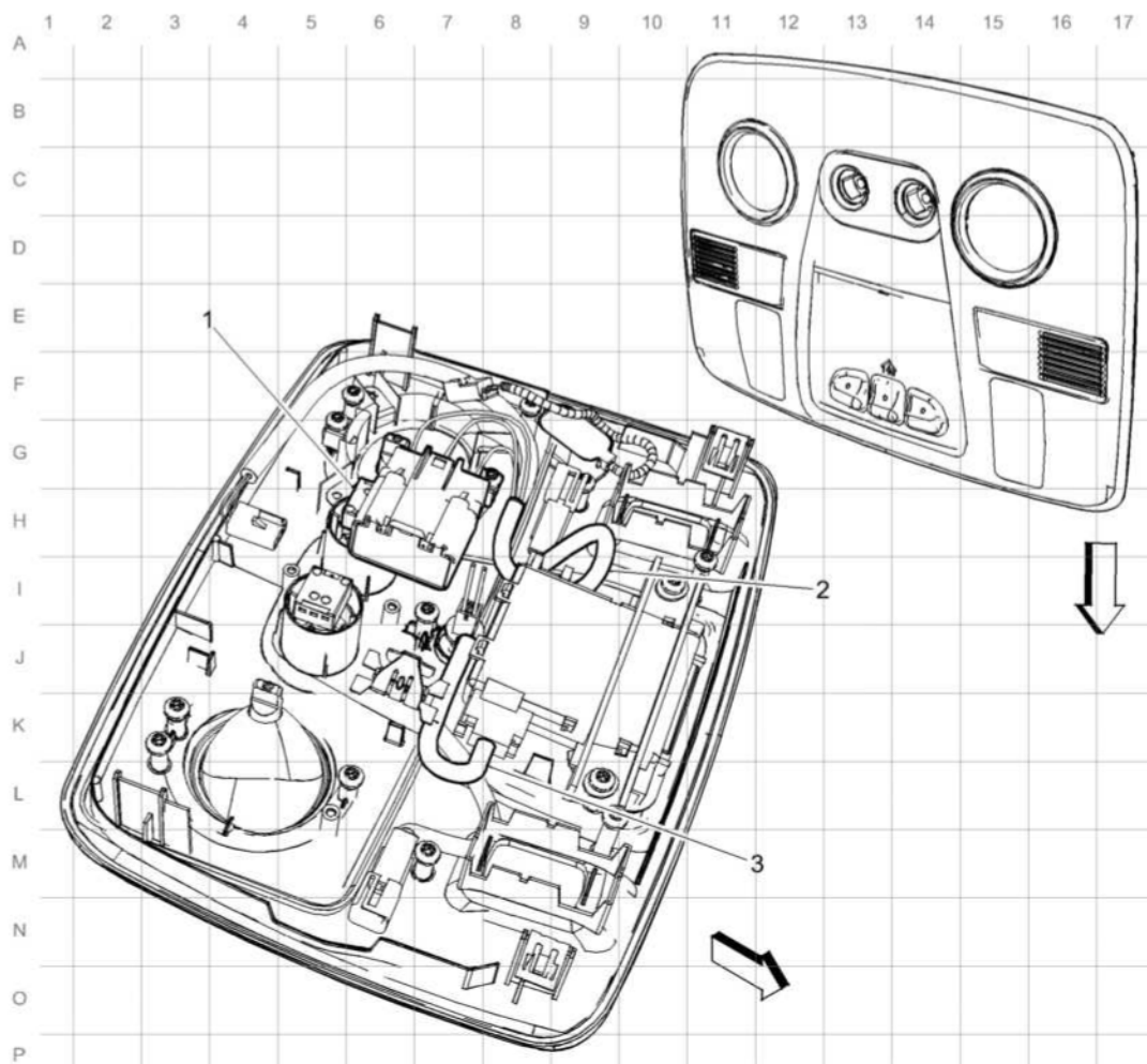
Fig. 7: Overhead Console Harness Routing Courtesy of GENERAL MOTORS COMPANY
