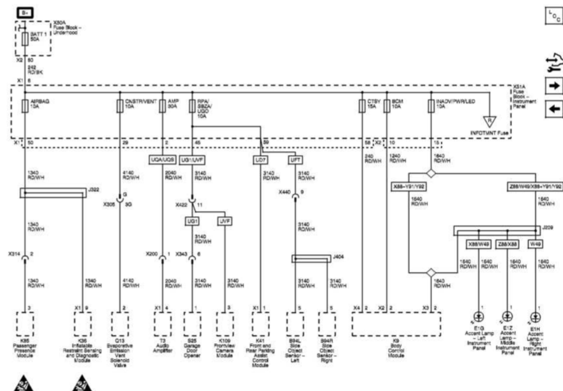
Fig. 32: AIRBAG, AMP, BATT 1, BCM, CNSTR/VENT, CTSY, INADV/PWR/LED And RPA/SBZA/UGO Wiring Schematics
