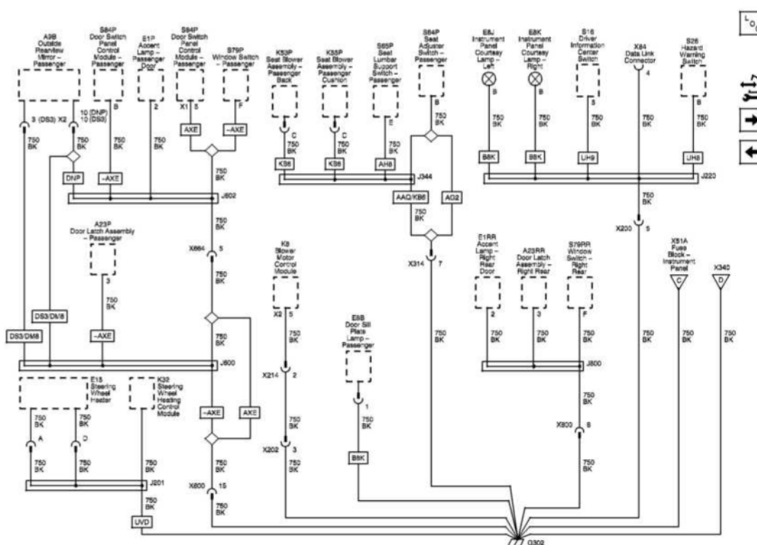
Fig. 62: G302 (1 Of 3) Wiring Schematics Courtesy of GENERAL MOTORS COMPANY
