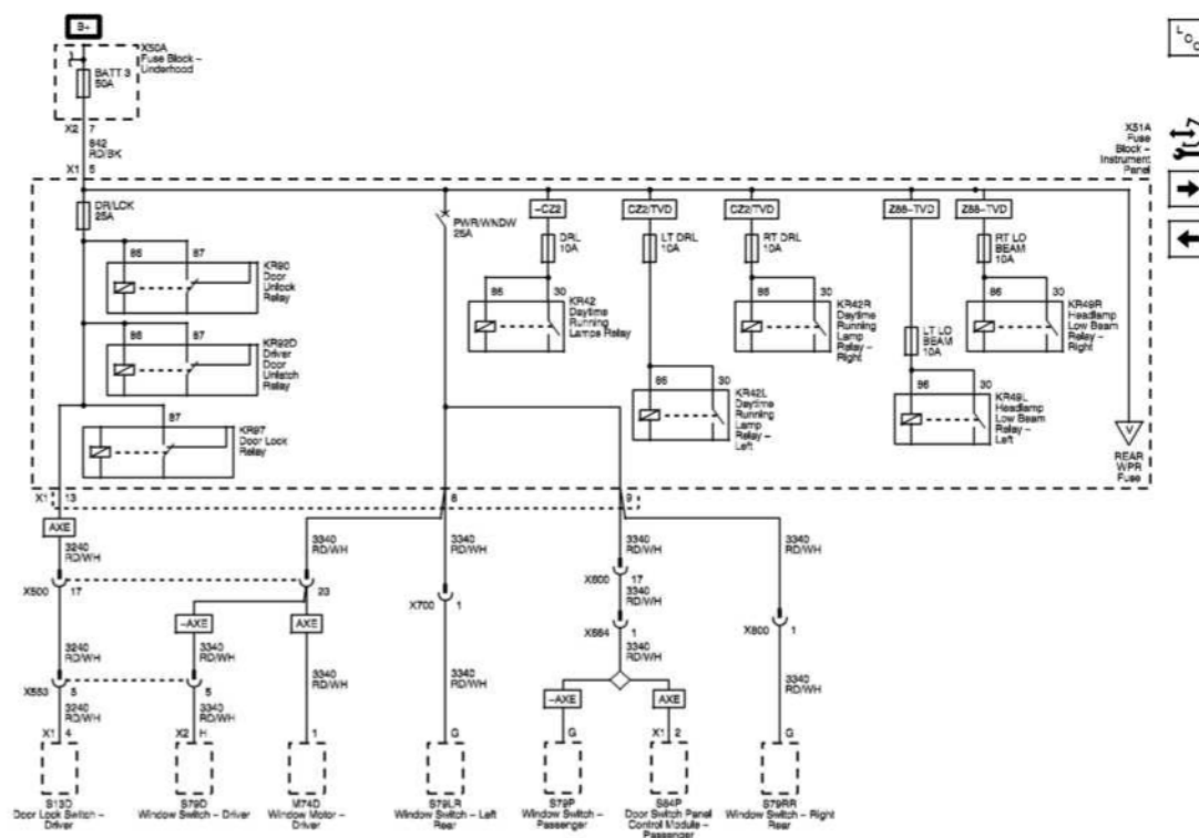
Fig. 34: BATT 3, DRL, DR/LCK, LT LO BEAM And RT LO BEAM Fuses And PWR/WNDW Wiring Schematics
