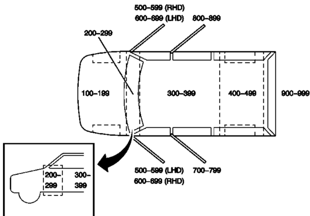
Fig. 29: View Of Utility/Van Zoning
