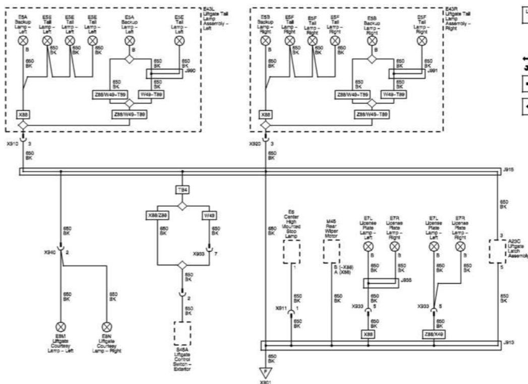
Fig. 68: G401 (2 Of 2) Wiring Schematics Courtesy of GENERAL MOTORS COMPANY
