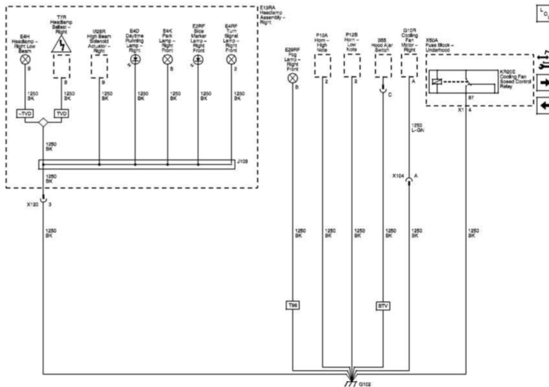
Fig. 56: G102 (Z88) Wiring Schematics Courtesy of GENERAL MOTORS COMPANY
