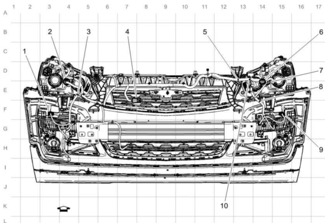
Fig. 20: Front Fascia Harness Routing (X88) Courtesy of GENERAL MOTORS COMPANY
