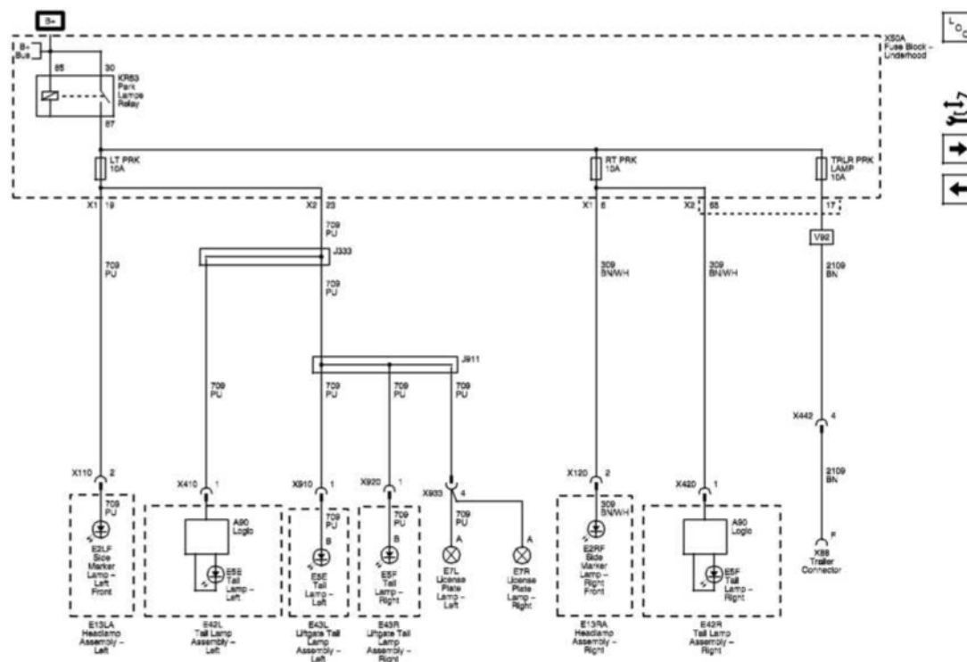
Fig. 45: LT PRK, RT PRK And TRLR PRK LAMP (Z88) Wiring Schematics Courtesy of GENERAL MOTORS COMPANY
