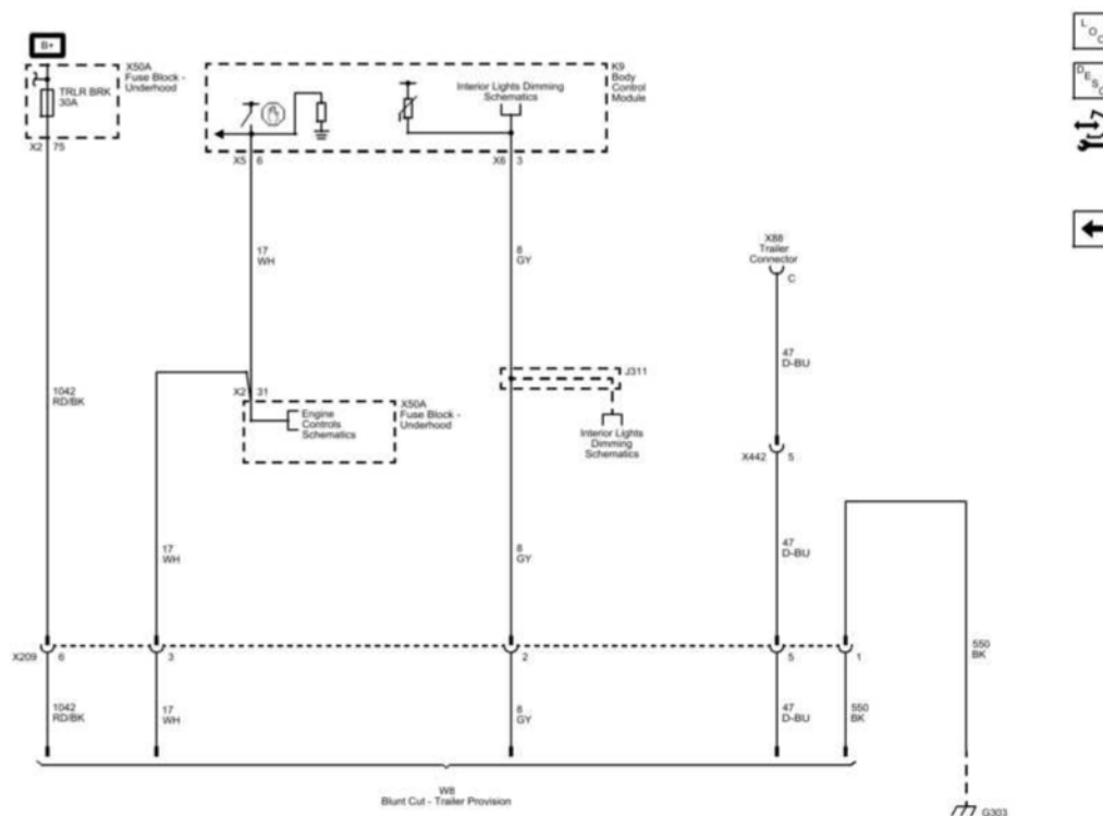
Fig. 72: Trailer Brake Provisions (V92) Wiring Schematics Courtesy of GENERAL MOTORS COMPANY
