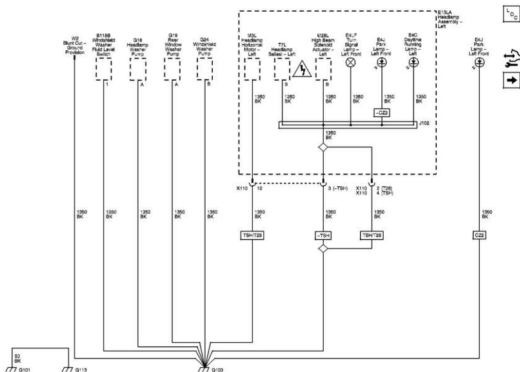
Fig. 51: G101, G103 And G113 (W49) Wiring Schematics Courtesy of GENERAL MOTORS COMPANY
