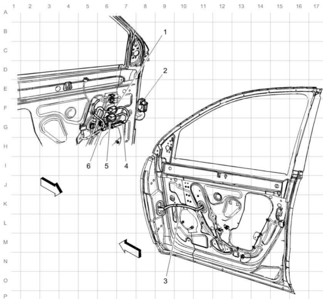
Fig. 6: Driver Door Harness Routing
