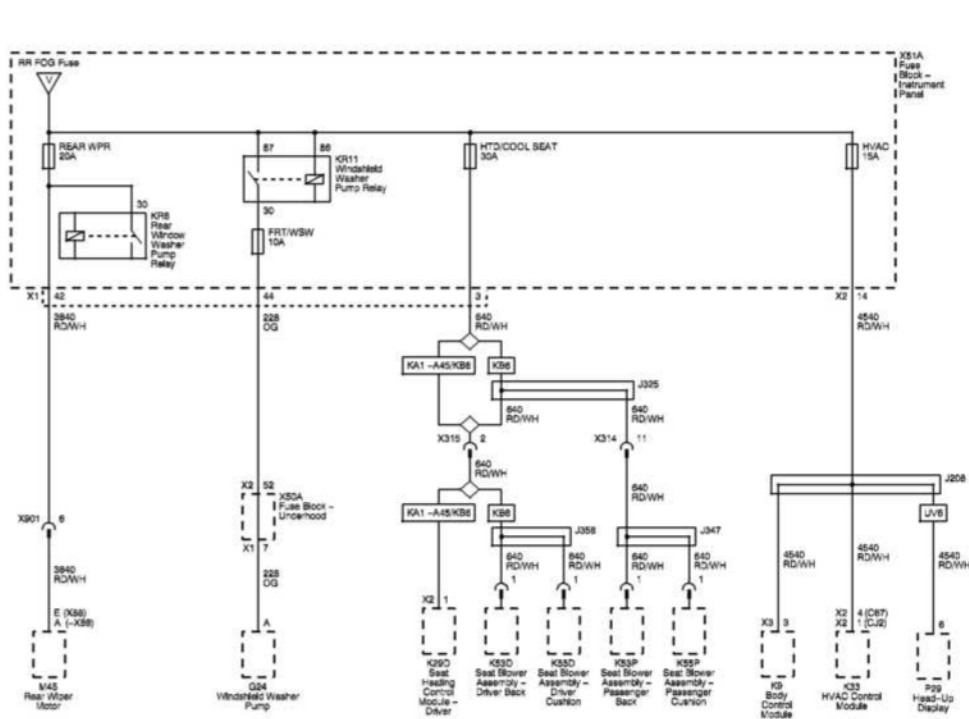
Fig. 36: FRT/WSW, HVAC, HTD/COOL SEAT And REAR WPR Wiring Schematics Courtesy of GENERAL MOTORS COMPANY
