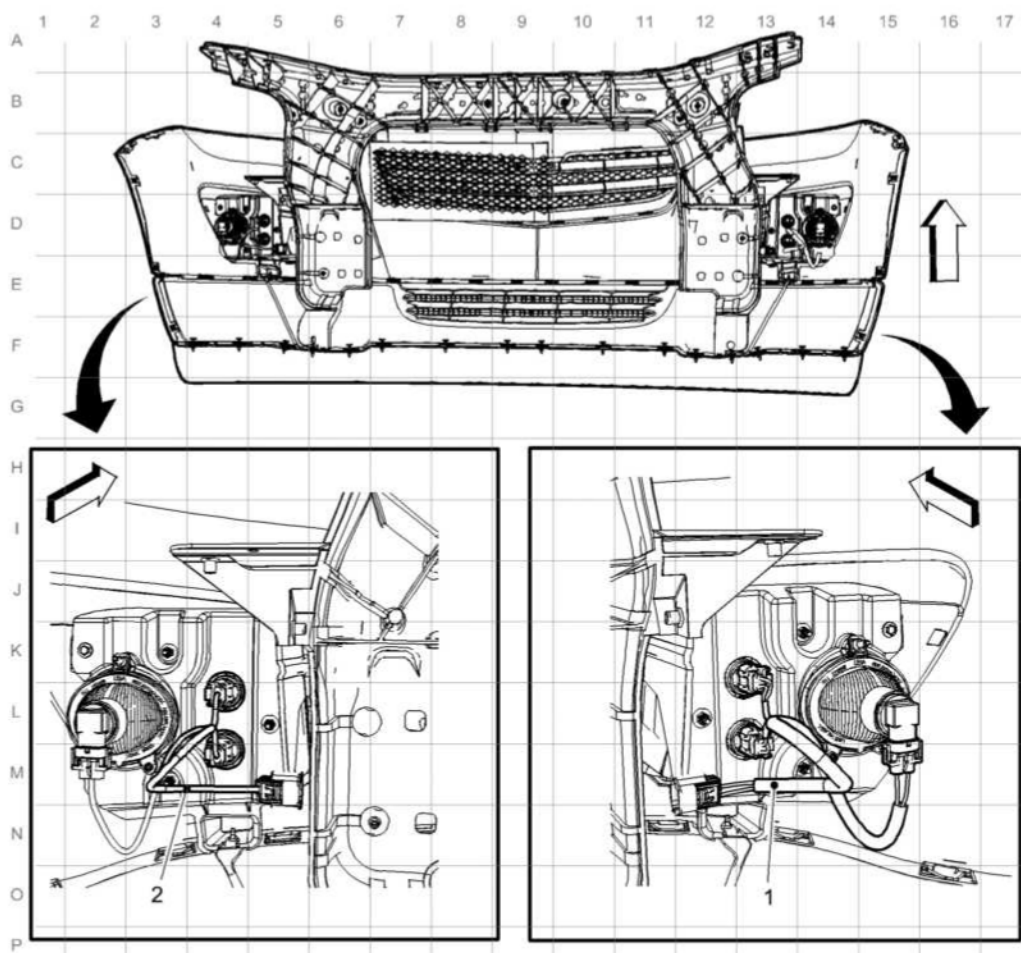
Fig. 25: Fog Lamp Extension Harness Routing Courtesy of GENERAL MOTORS COMPANY
