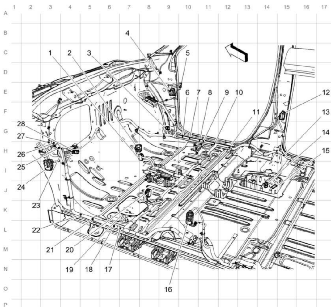
Fig. 17: Body Harness Routing - Front Passenger Compartment Courtesy of GENERAL MOTORS COMPANY
