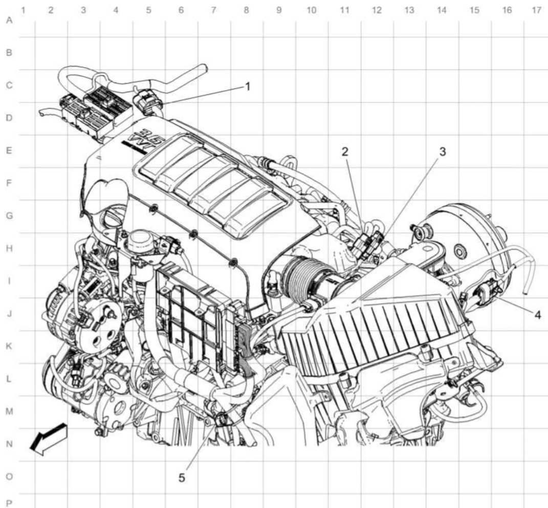
Fig. 28: Engine Compartment Harness Routing Courtesy of GENERAL MOTORS COMPANY
