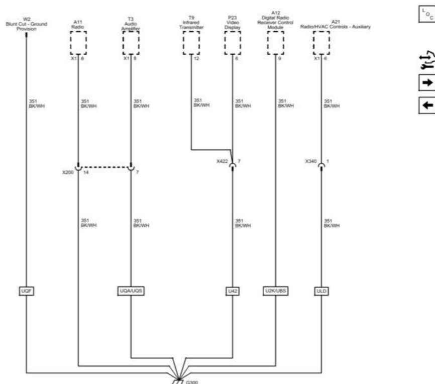
Fig. 59: G300 Wiring Schematics Courtesy of GENERAL MOTORS COMPANY
