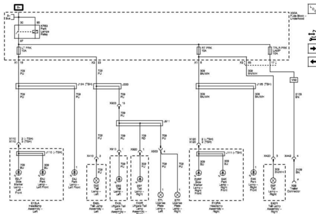
Fig. 46: LT PRK, RT PRK And TRLR PRK LAMP (W49) Wiring Schematics Courtesy of GENERAL MOTORS COMPANY
