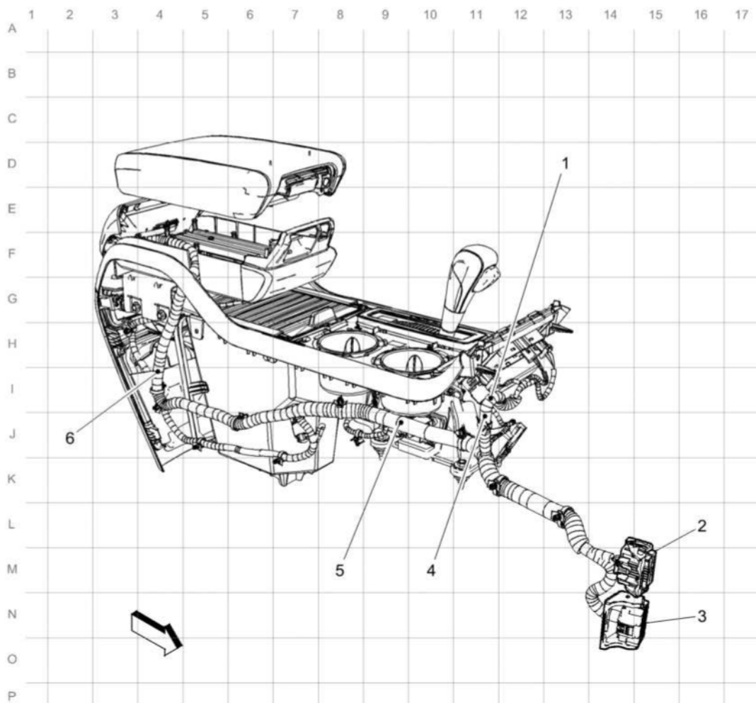
Fig. 2: Front Floor Console Harness Routing Courtesy of GENERAL MOTORS COMPANY
