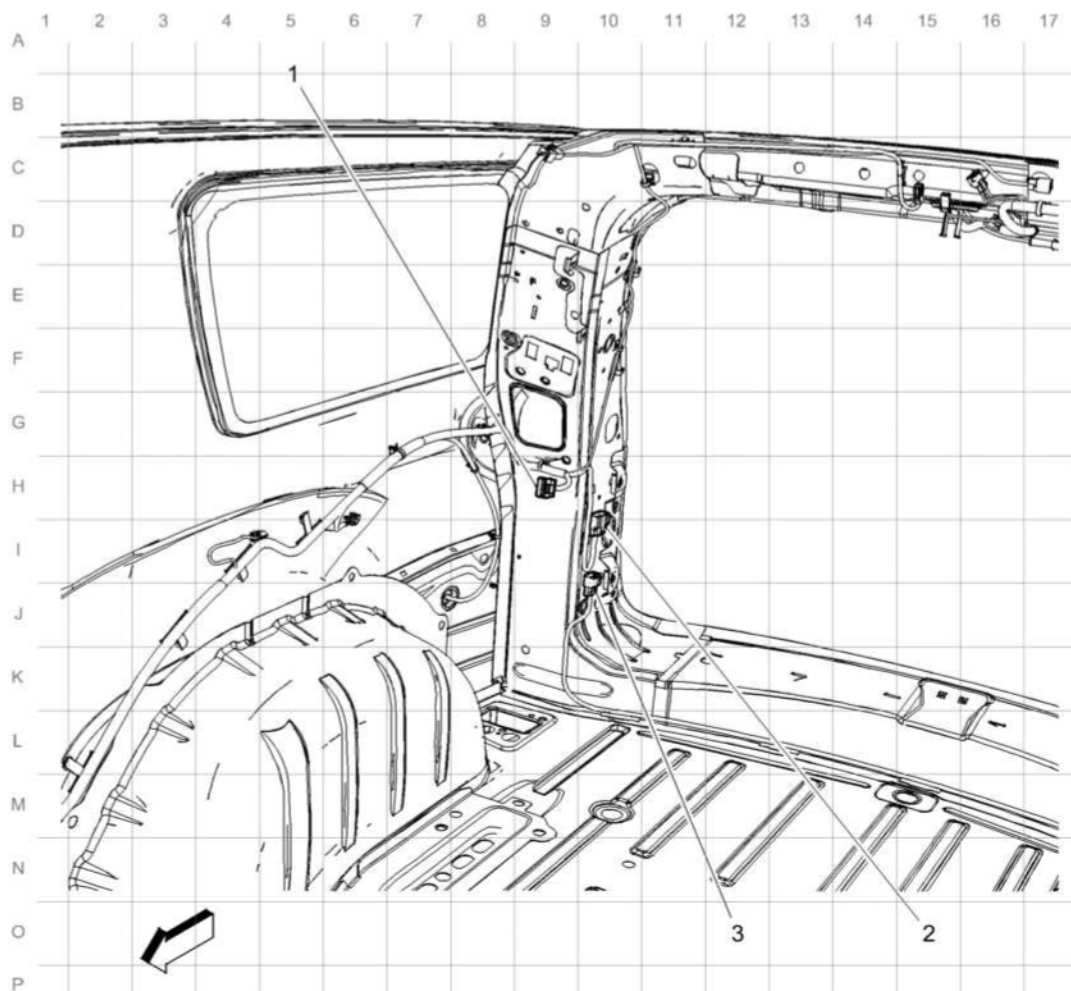
Fig. 16: Body Harness Routing - Right Rear Passenger Compartment Courtesy of GENERAL MOTORS COMPANY
