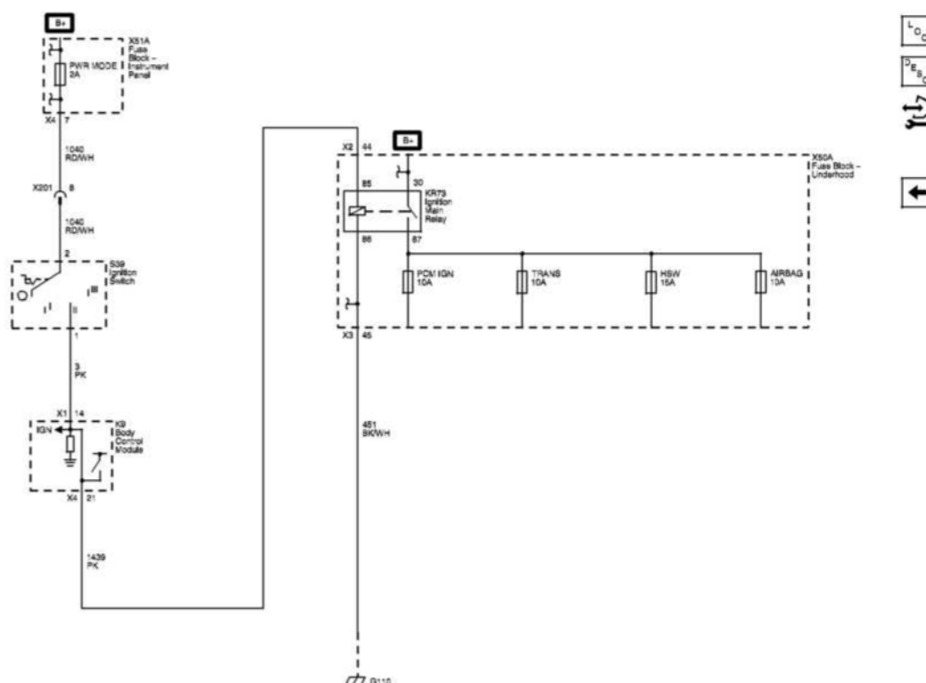
Fig. 49: IGN II/III Wiring Schematics Courtesy of GENERAL MOTORS COMPANY
