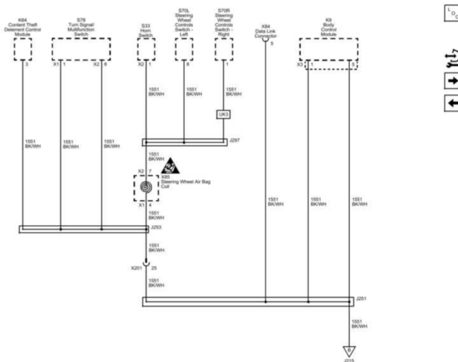
Fig. 61: G301 (2 Of 2) Wiring Schematics
