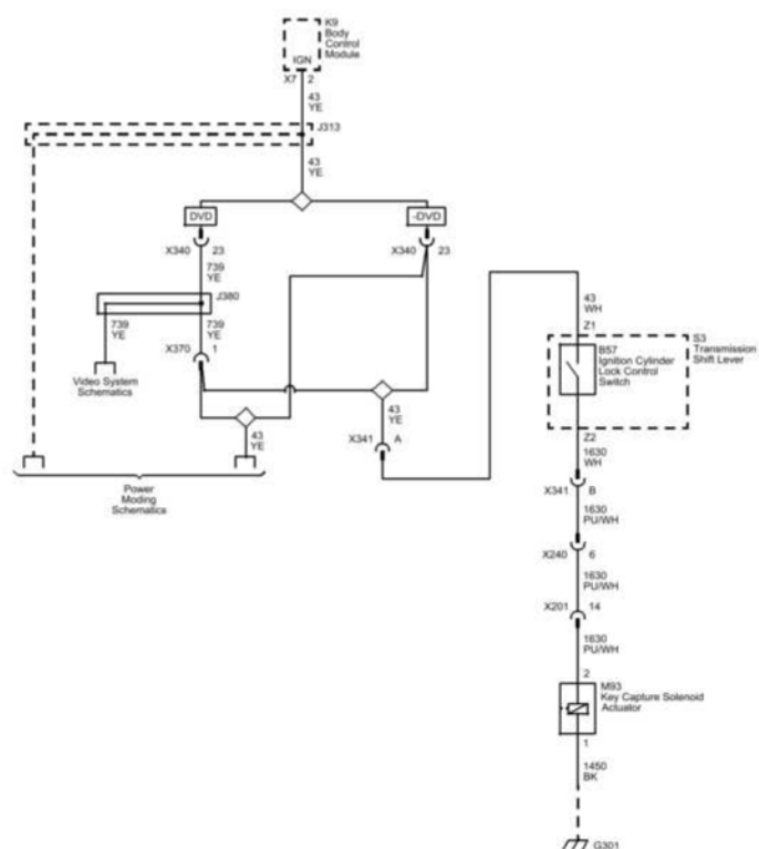
Fig. 50: Ignition Lock Wiring Schematics Courtesy of GENERAL MOTORS COMPANY
