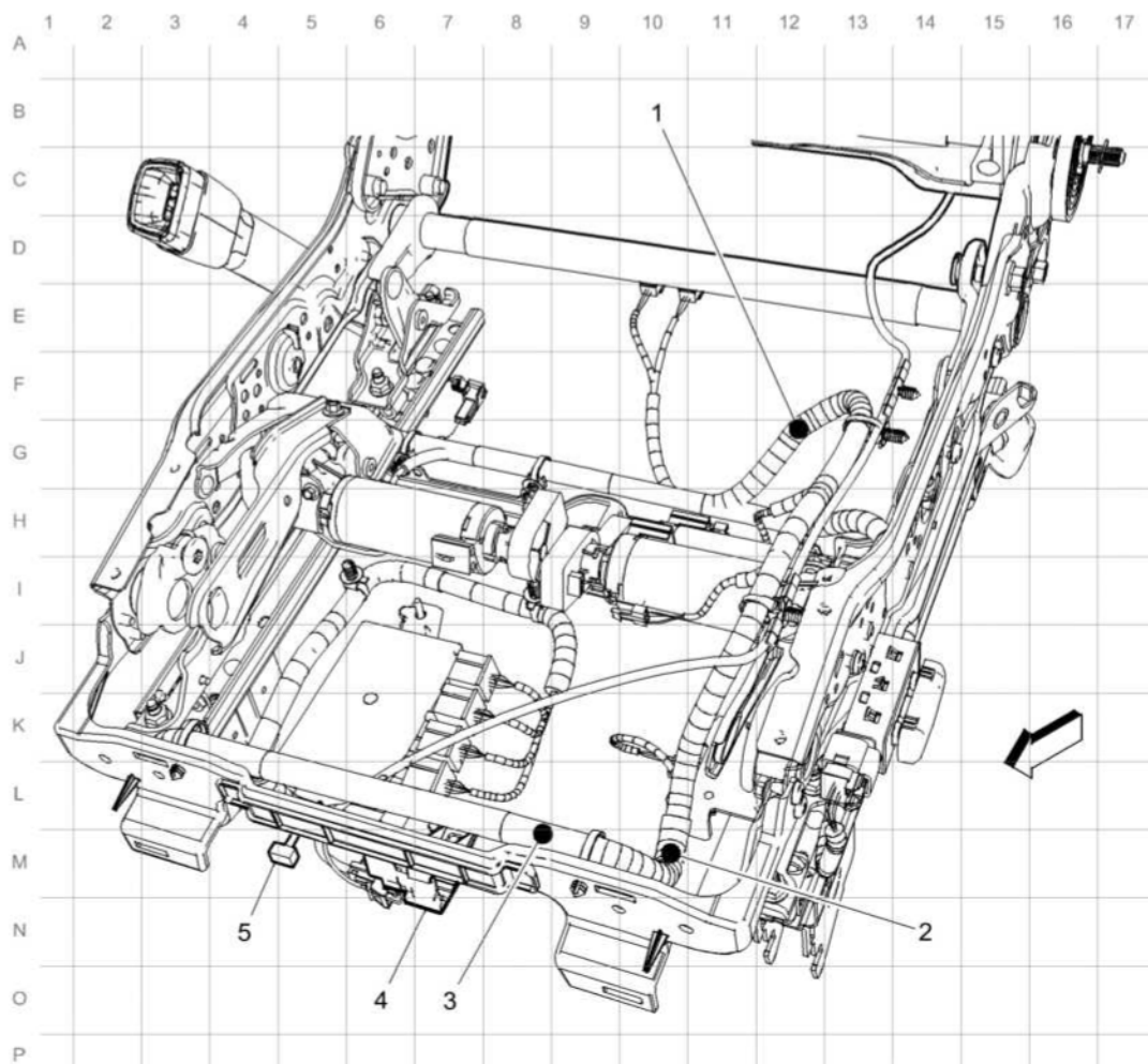
Fig. 14: Driver Seat Harness Routing (Without AG3) Courtesy of GENERAL MOTORS COMPANY
