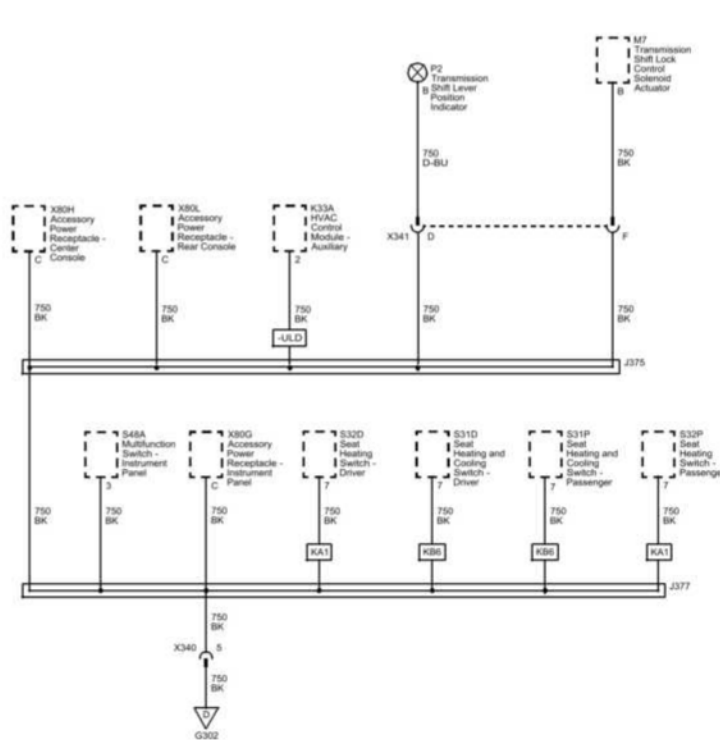
Fig. 64: G302 (3 Of 3) Wiring Schematics Courtesy of GENERAL MOTORS COMPANY
