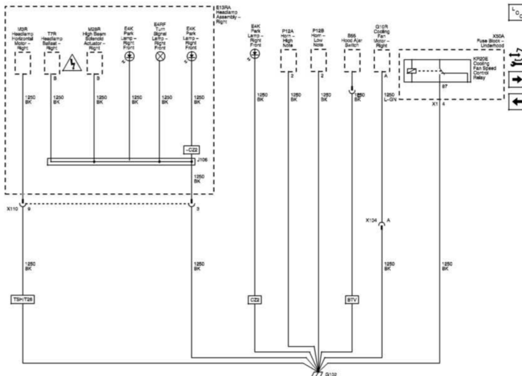
Fig. 54: G102 (W49) Wiring Schematics Courtesy of GENERAL MOTORS COMPANY
