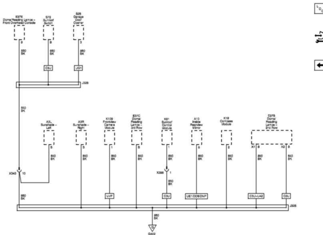
Fig. 70: G402 (2 Of 2) Wiring Schematics Courtesy of GENERAL MOTORS COMPANY
