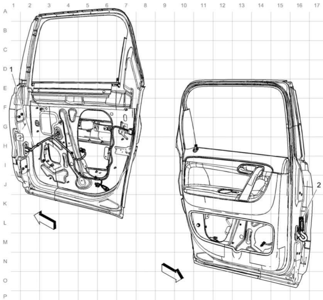
Fig. 8: Left Rear Door Harness Routing Courtesy of GENERAL MOTORS COMPANY
