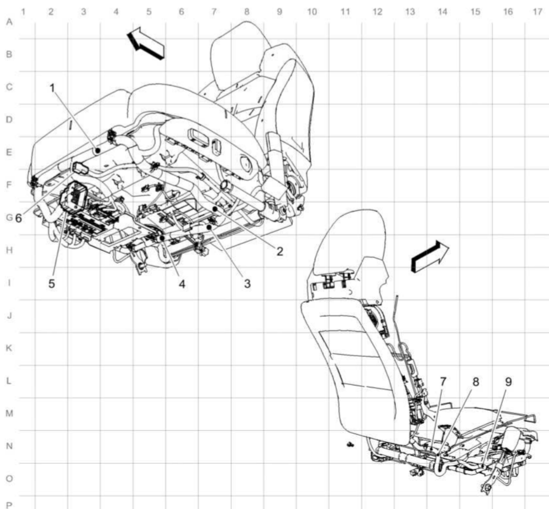
Fig. 13: Driver Seat Harness Routing (AG3) Courtesy of GENERAL MOTORS COMPANY
