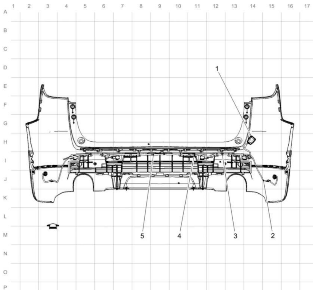
Fig. 18: Rear Bumper Harness Routing Courtesy of GENERAL MOTORS COMPANY
