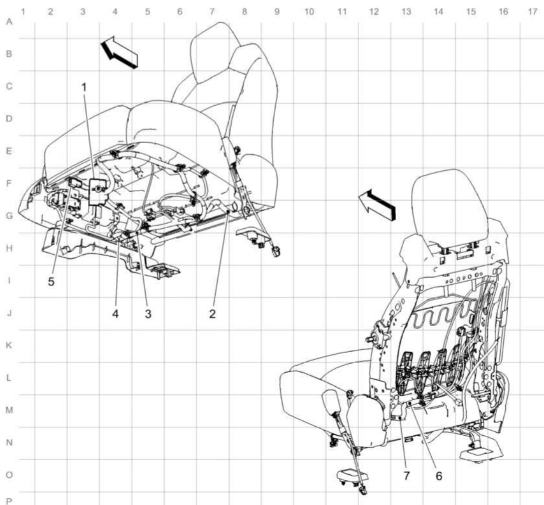
Fig. 15: Passenger Seat Harness Routing Courtesy of GENERAL MOTORS COMPANY
