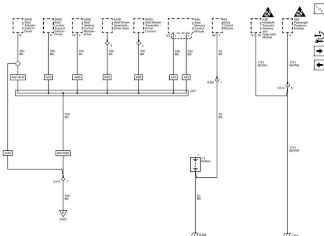
Fig. 66: G303 (2 Of 2), G304 And G305 Wiring Schematics Courtesy of GENERAL MOTORS COMPANY
