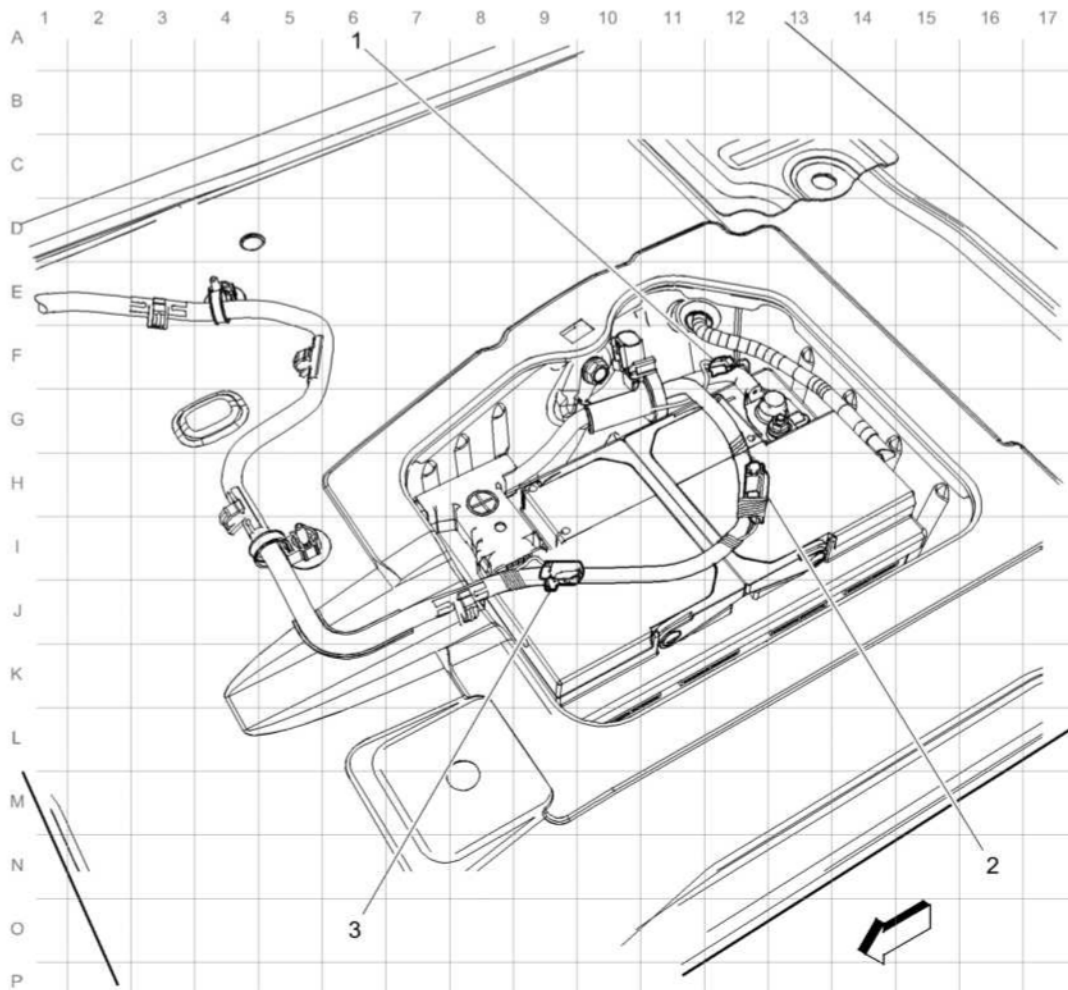
Fig. 22: Second Row Seat Area Floor Harness Routing Courtesy of GENERAL MOTORS COMPANY
