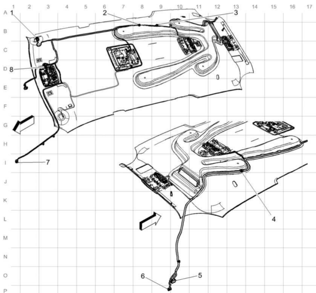
Fig. 21: Headlining Harness Routing Courtesy of GENERAL MOTORS COMPANY
