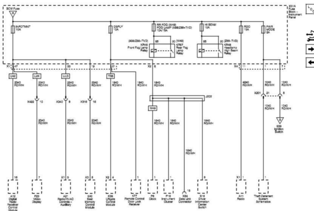
Fig. 35: DSPLY, FOG LAMP, HI BEAM, INFOTMNT, PWR MODE, RDO And RR FOG Wiring Schematics
