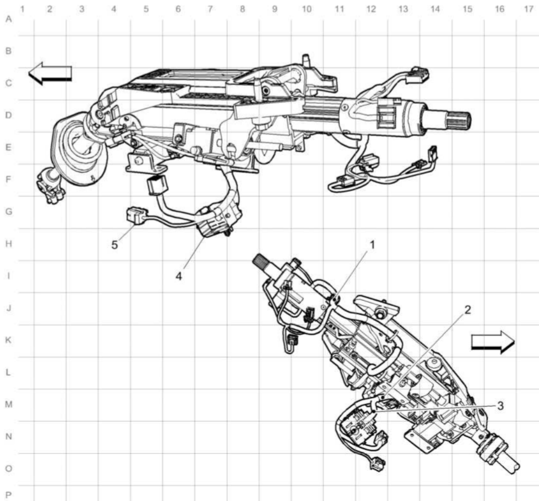
Fig. 5: Steering Column Harness Routing Courtesy of GENERAL MOTORS COMPANY
