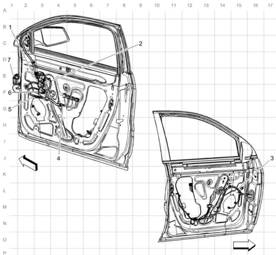
Fig. 9: Passenger Door Harness Routing Courtesy of GENERAL MOTORS COMPANY
