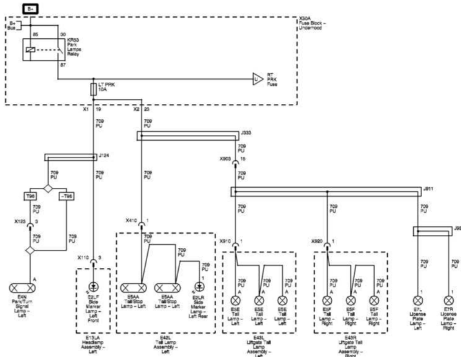
Fig. 43: LT PRK (X88) Wiring Schematics Courtesy of GENERAL MOTORS COMPANY
