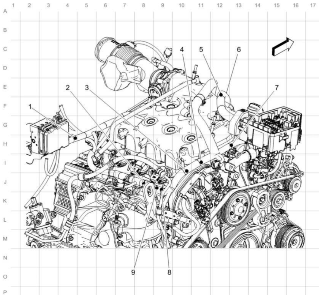
Fig. 11: Engine Harness Splice Routing - Rear Courtesy of GENERAL MOTORS COMPANY
