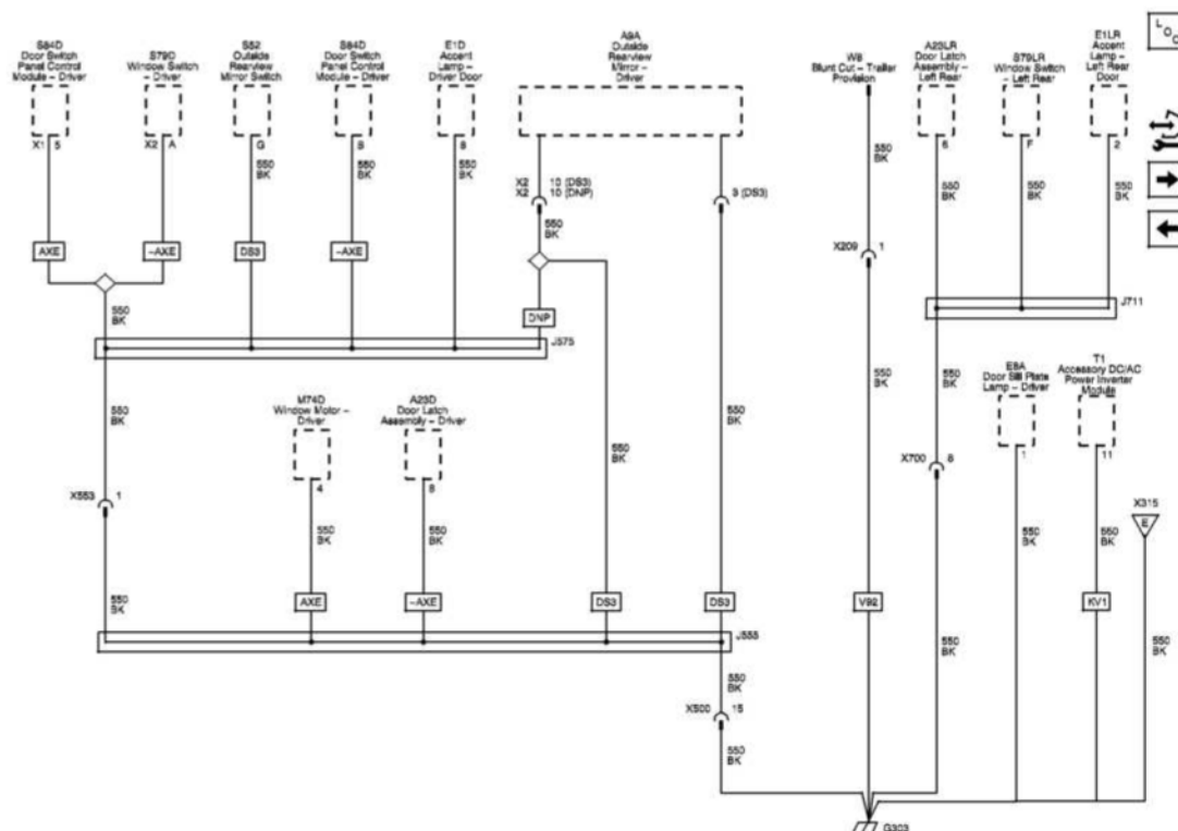
Fig. 65: G303 (1 Of 2) Wiring Schematics Courtesy of GENERAL MOTORS COMPANY
