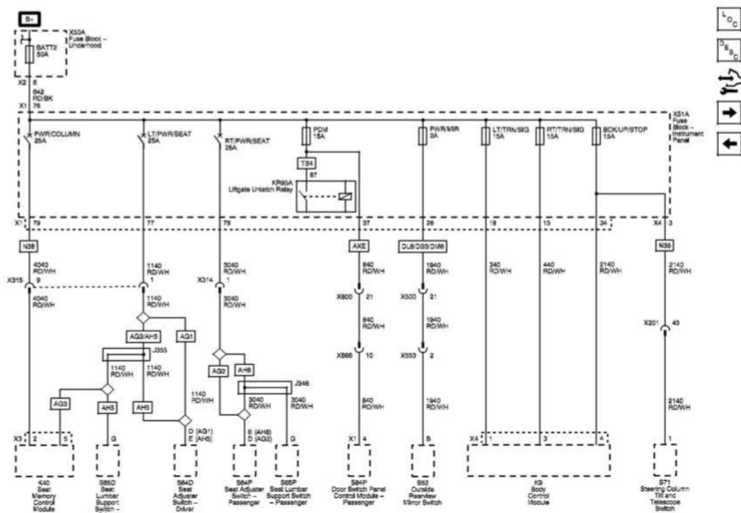
Fig. 33: BATT 2, BCK/UP/STOP, LT/TRN/SIG, PDM, PWR/MIR And RT/TRN/SIG Fuses, LT/PWR/SEAT, PWR/COLUMN And RT/PWR/SEAT Wiring Schematics Courtesy of GENERAL MOTORS COMPANY
