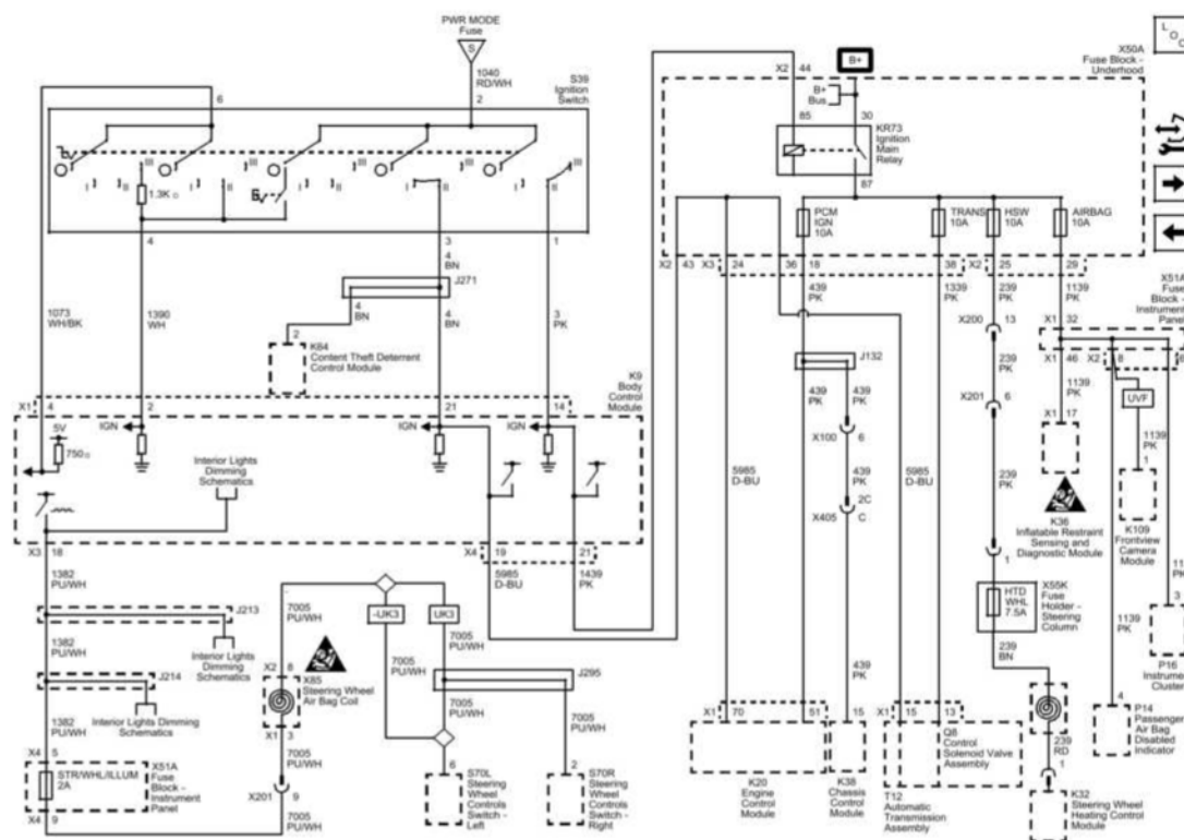
Fig. 39: Ignition Switch And AIRBAG, HSW, PCM IGN And TRANS Fuses Wiring Schematics Courtesy of GENERAL MOTORS COMPANY
