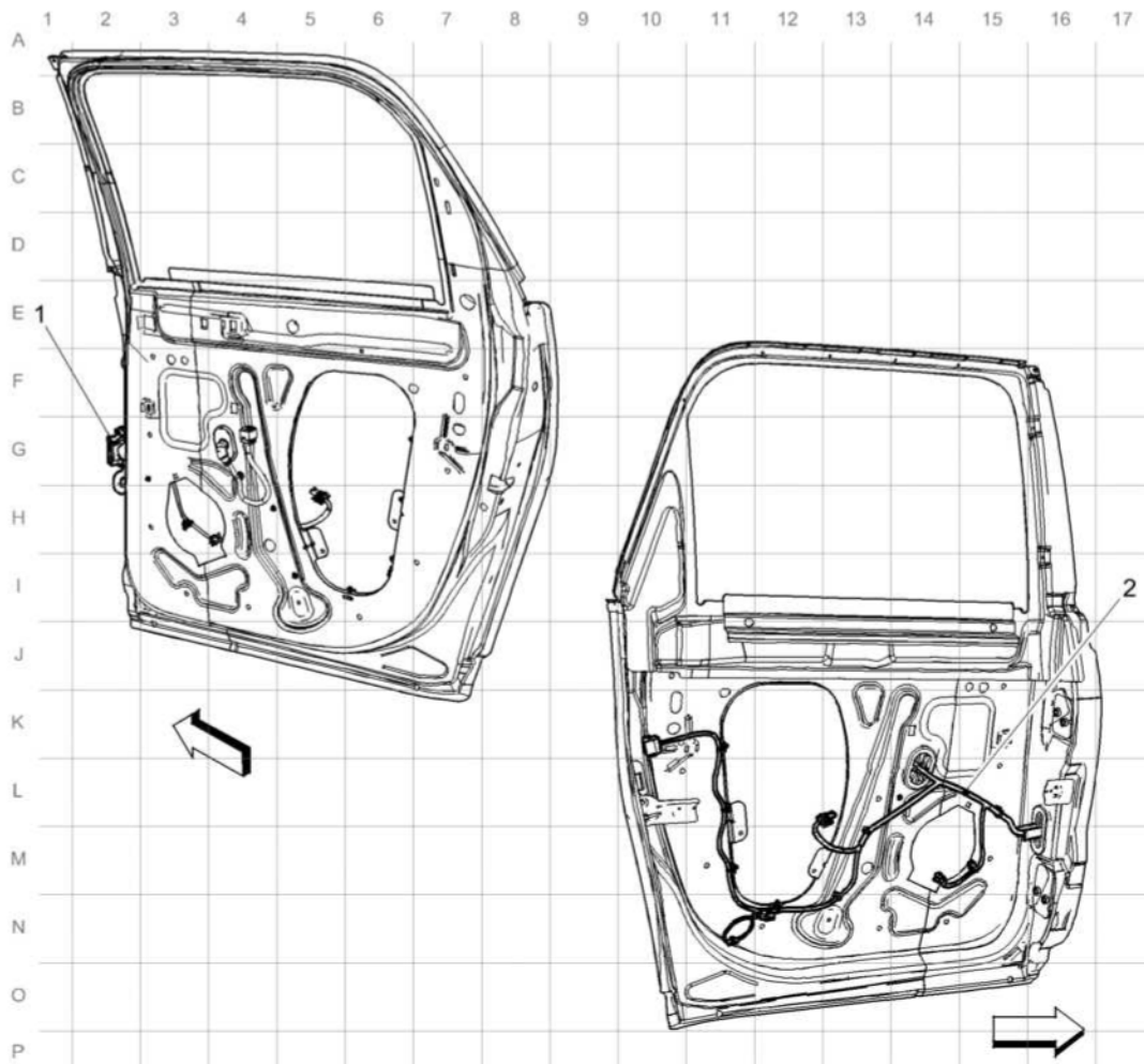
Fig. 10: Right Rear Door Harness Routing Courtesy of GENERAL MOTORS COMPANY
