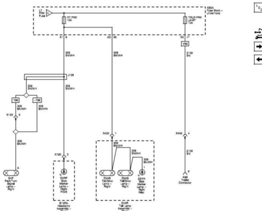
Fig. 44: RT PRK And TRLR LAMP (X88) Wiring Schematics
