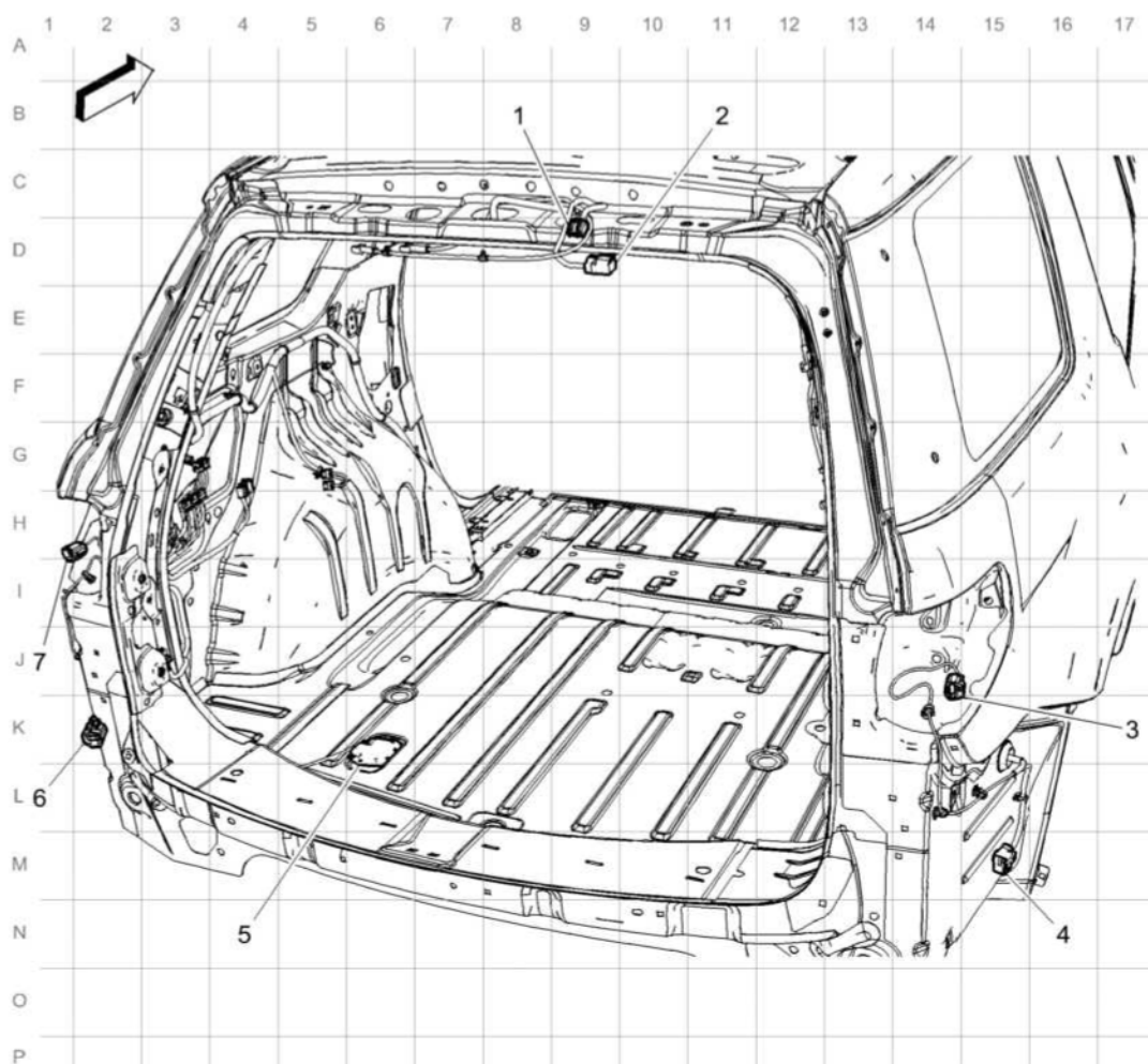
Fig. 26: Body Harness Routing - Near Liftgate Courtesy of GENERAL MOTORS COMPANY
