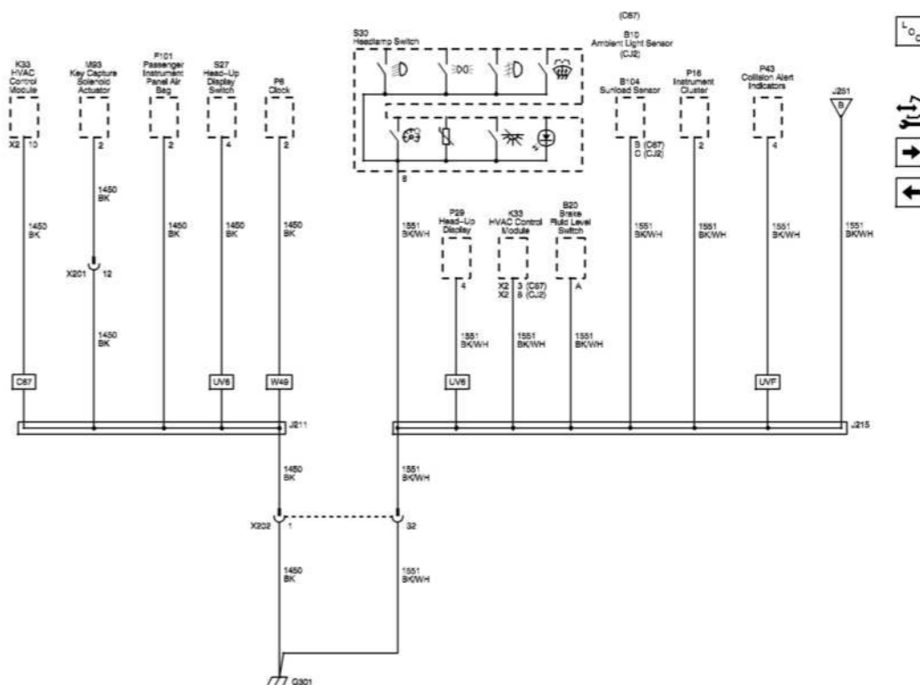
Fig. 60: G301 (1 Of 2) Wiring Schematics
