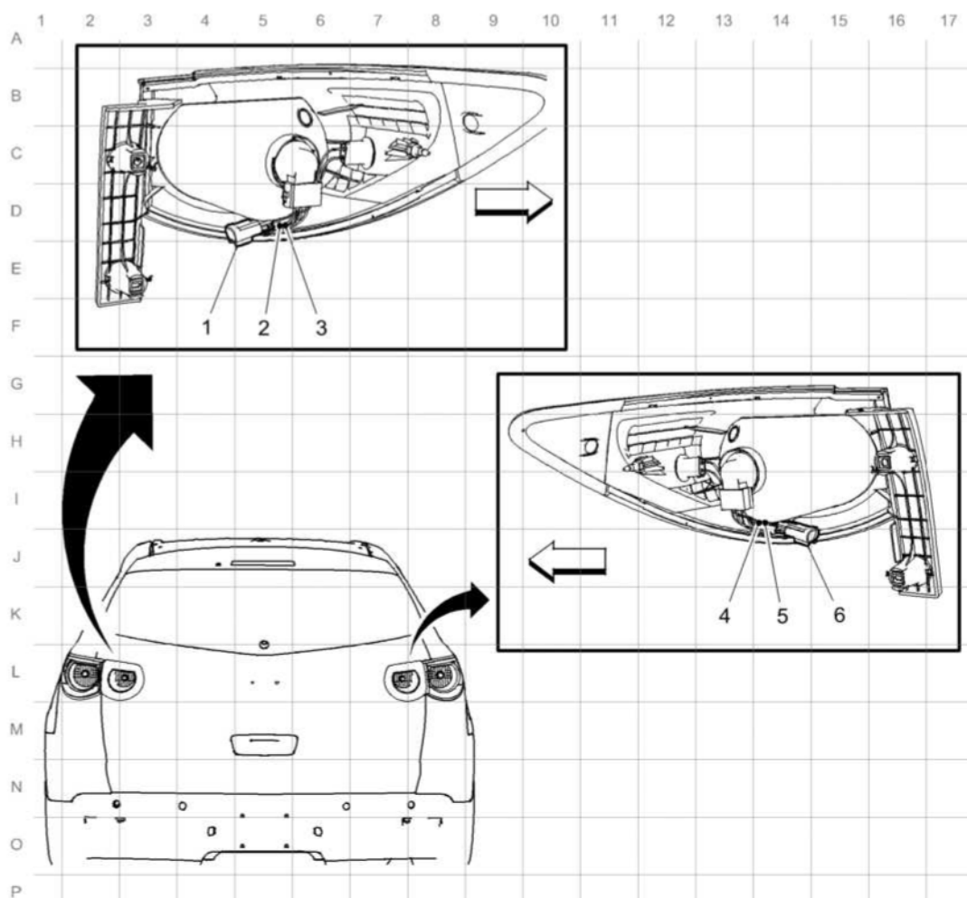
Fig. 19: Tail Lamp Harness Routing (X88) Courtesy of GENERAL MOTORS COMPANY
