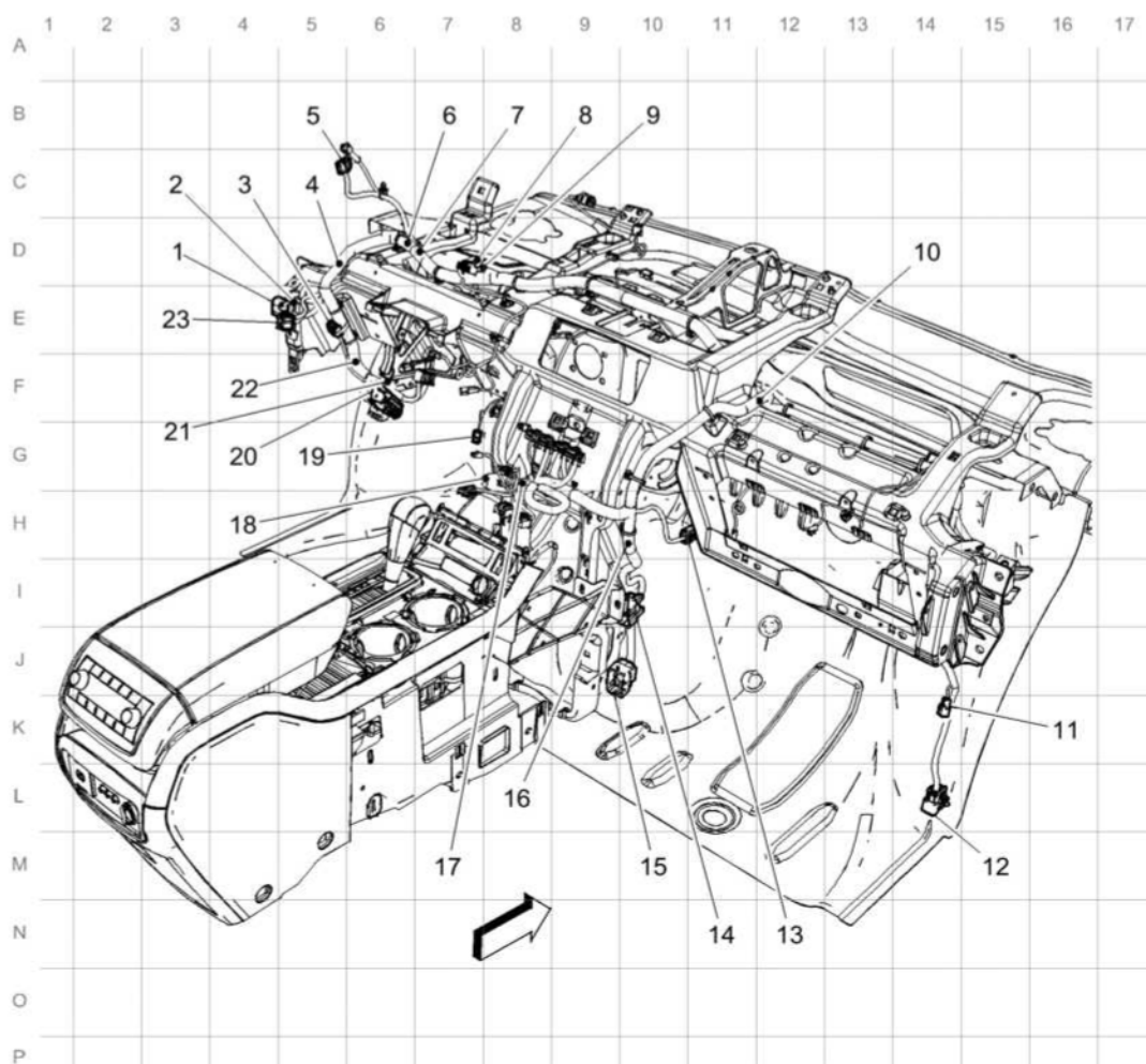
Fig. 23: Instrument Panel Harness Routing - Passenger Compartment Courtesy of GENERAL MOTORS COMPANY
