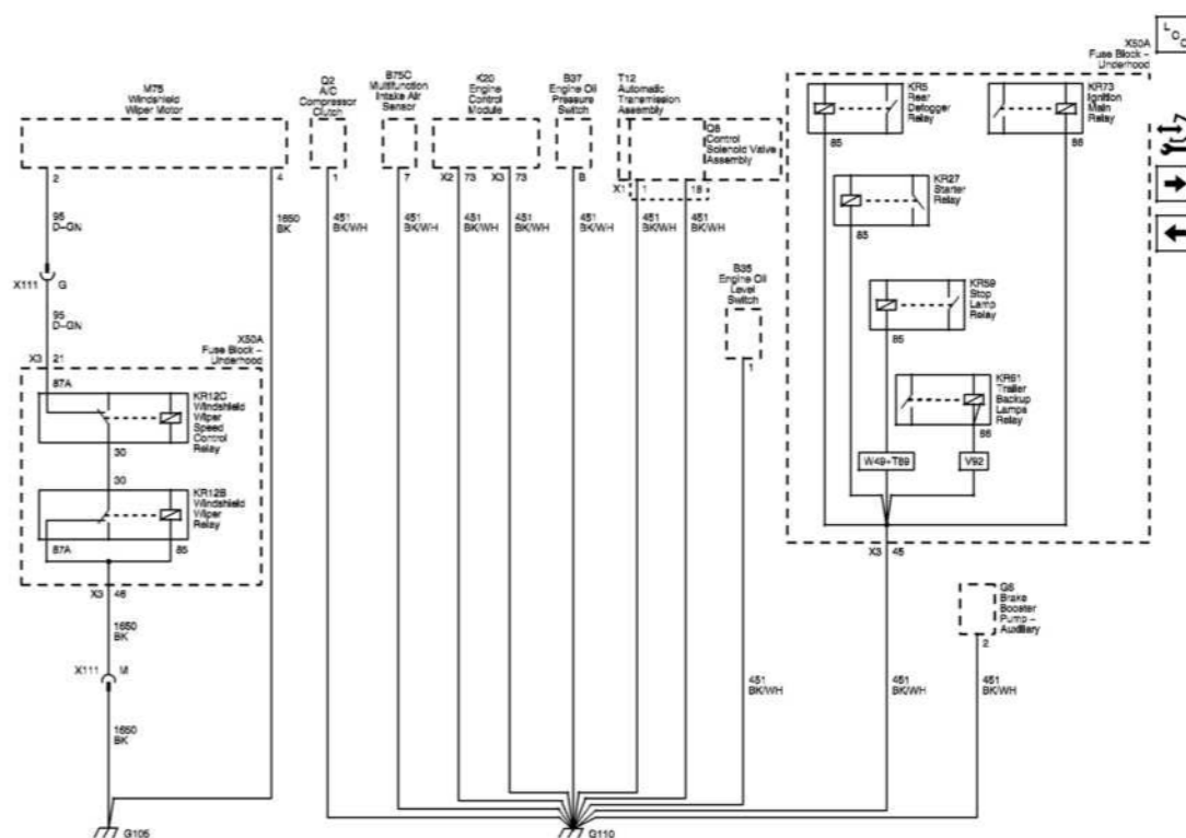
Fig. 57: G105 and G110 Wiring Schematics Courtesy of GENERAL MOTORS COMPANY
