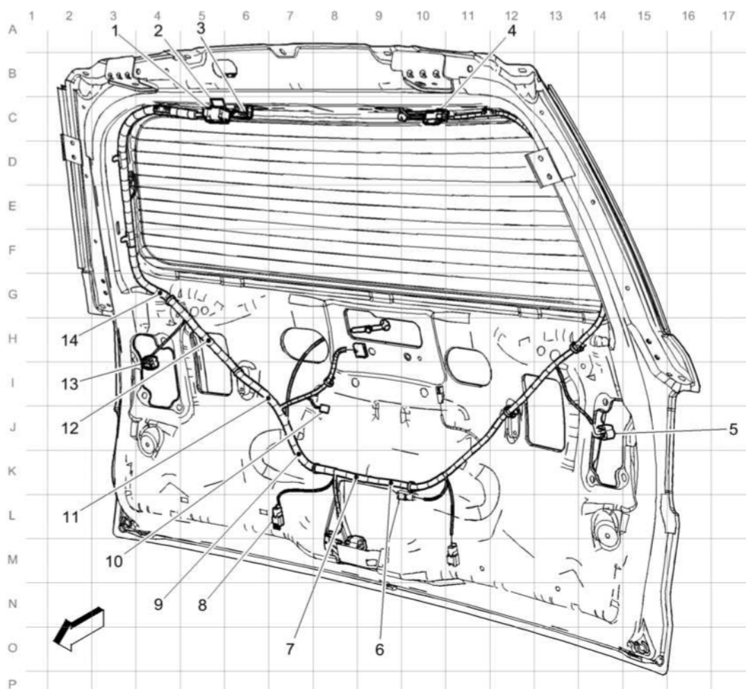
Fig. 27: Liftgate Harness Routing
