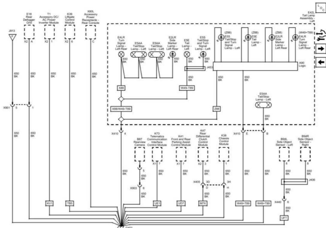
Fig. 67: G401 (1 Of 2) Wiring Schematics Courtesy of GENERAL MOTORS COMPANY
