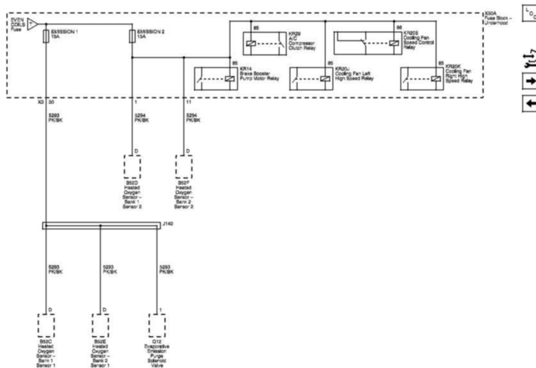
Fig. 41: EMISSION 1 And EMISSION 2 Wiring Schematics Courtesy of GENERAL MOTORS COMPANY
