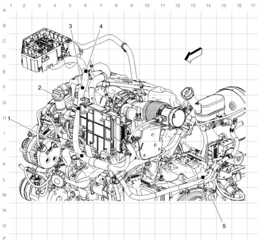
Fig. 12: Engine Harness Splice Routing - Front Courtesy of GENERAL MOTORS COMPANY
