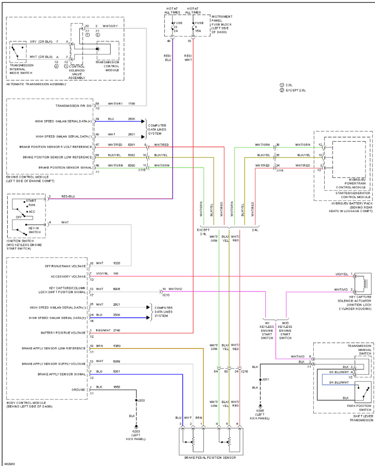
Fig. 121: Ignition Lock Solenoid Circuit
