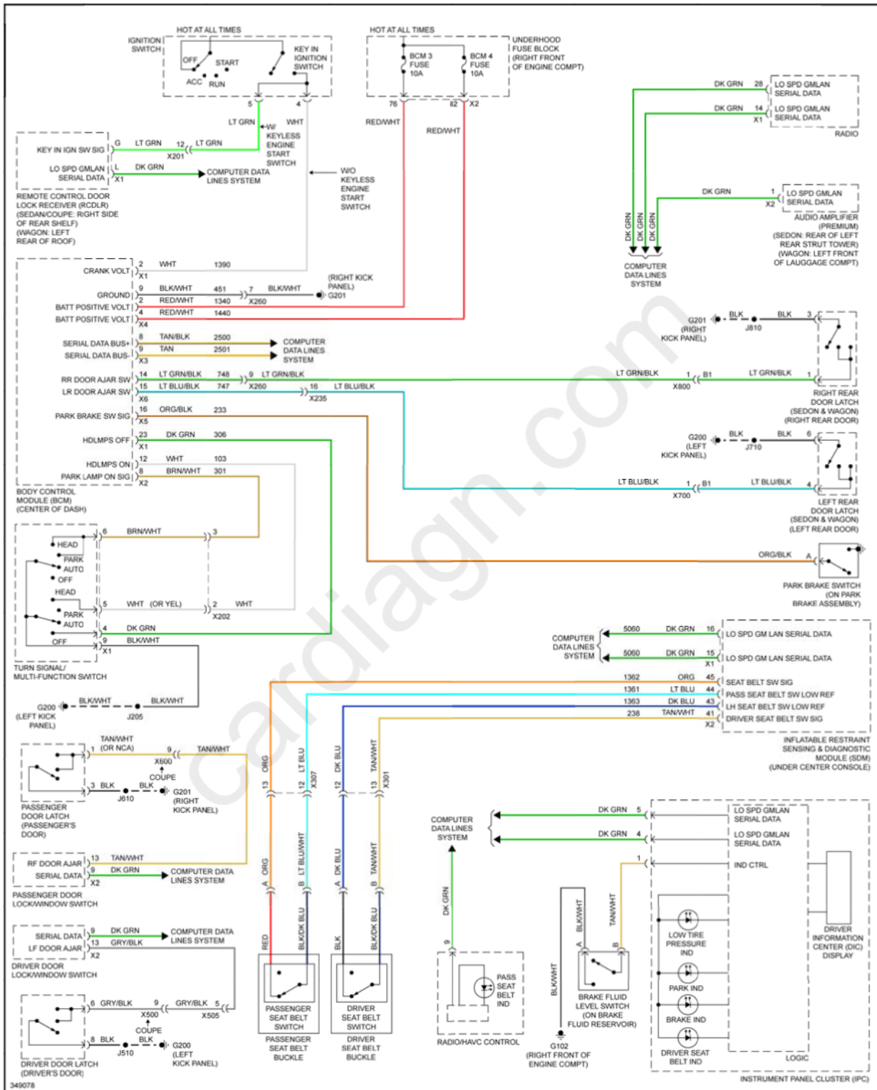
Fig. 120: Warning Systems Circuit
