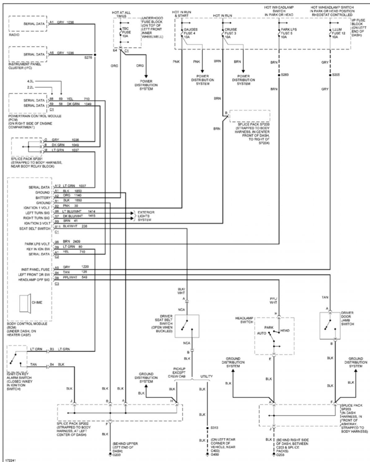
Fig. 53: Warning Systems Circuit
