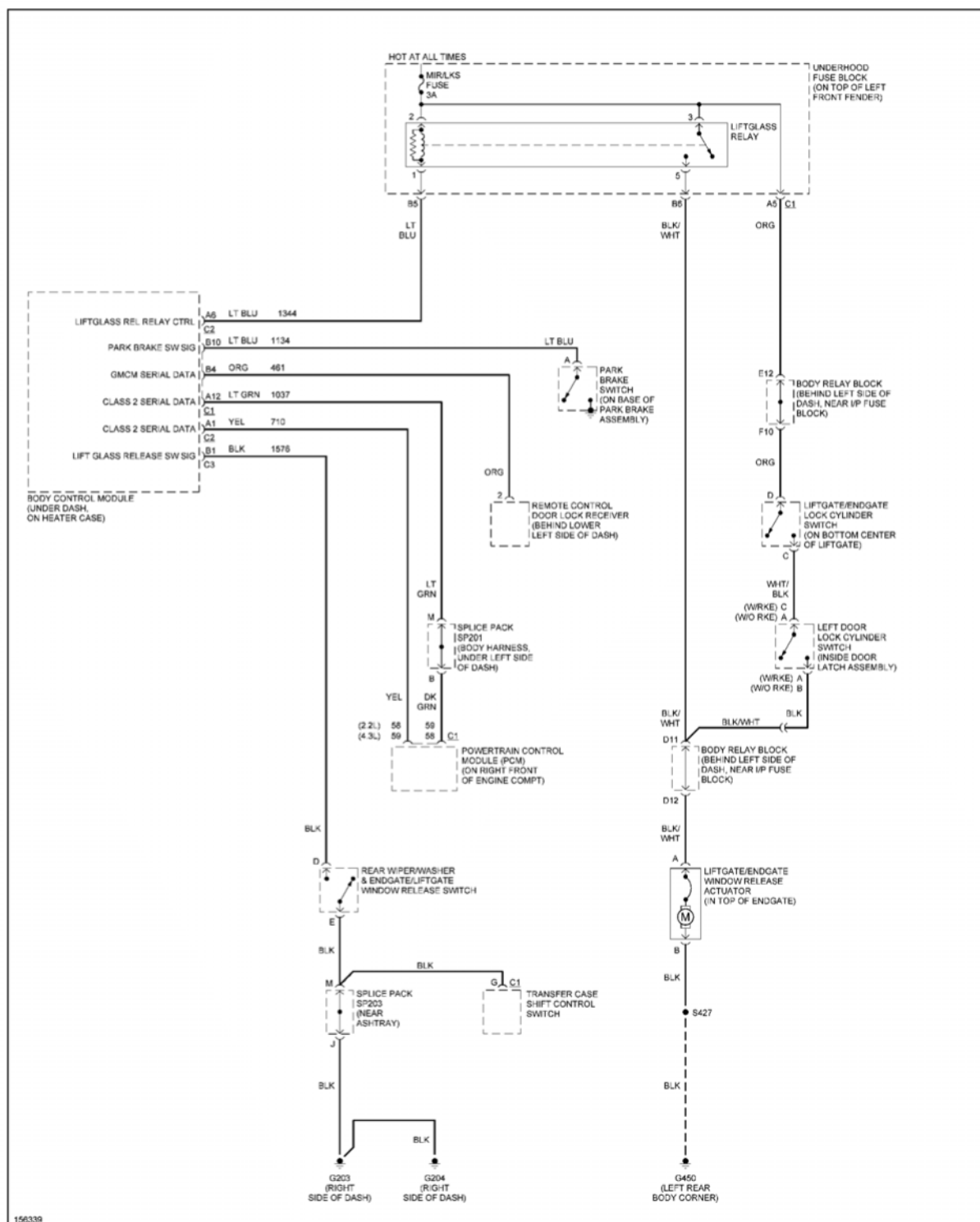
Fig. 52: Liftgate/Endgate Release Circuit
