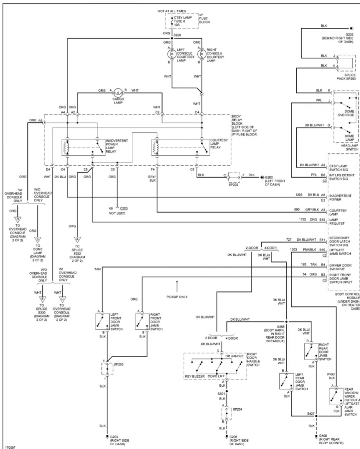
Fig. 24: Courtesy Lamps Circuit (1 of 2)
