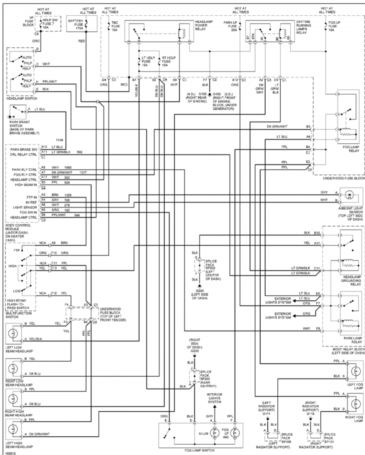
Fig. 20: Headlights Circuit, W/O ZR2
