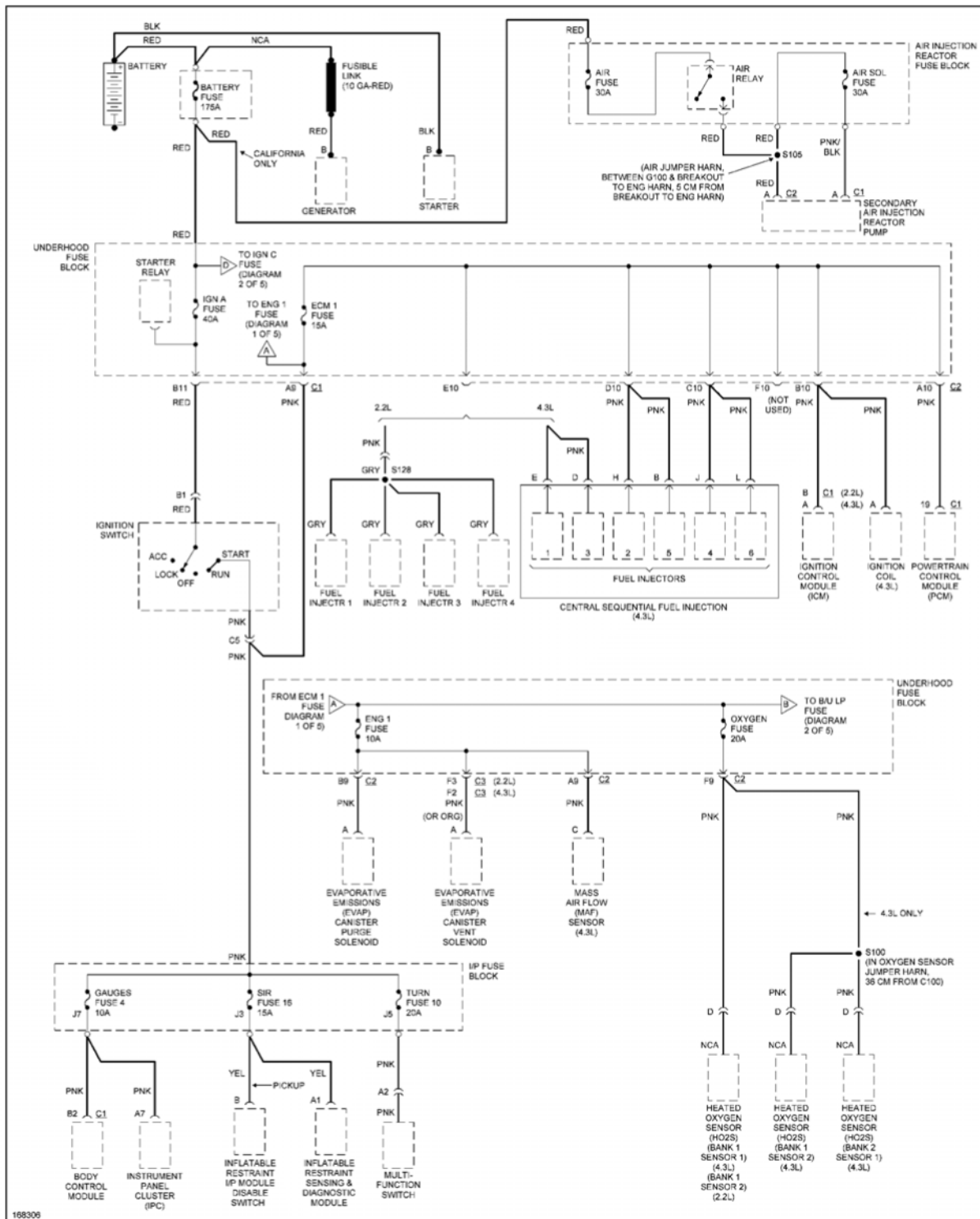
Fig. 27: Power Distribution Circuit (1 of 5)
