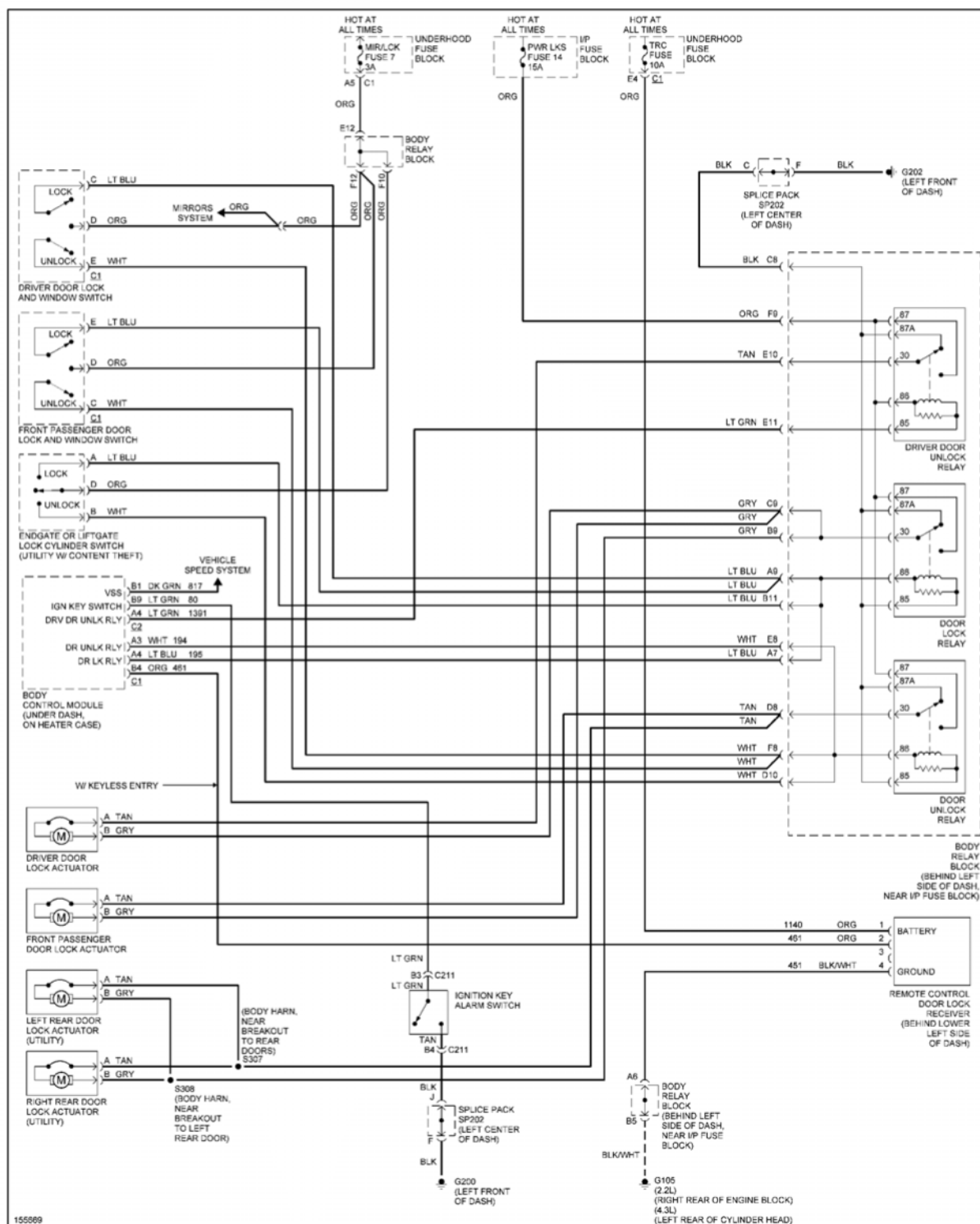
Fig. 32: Power Door Locks Circuit
