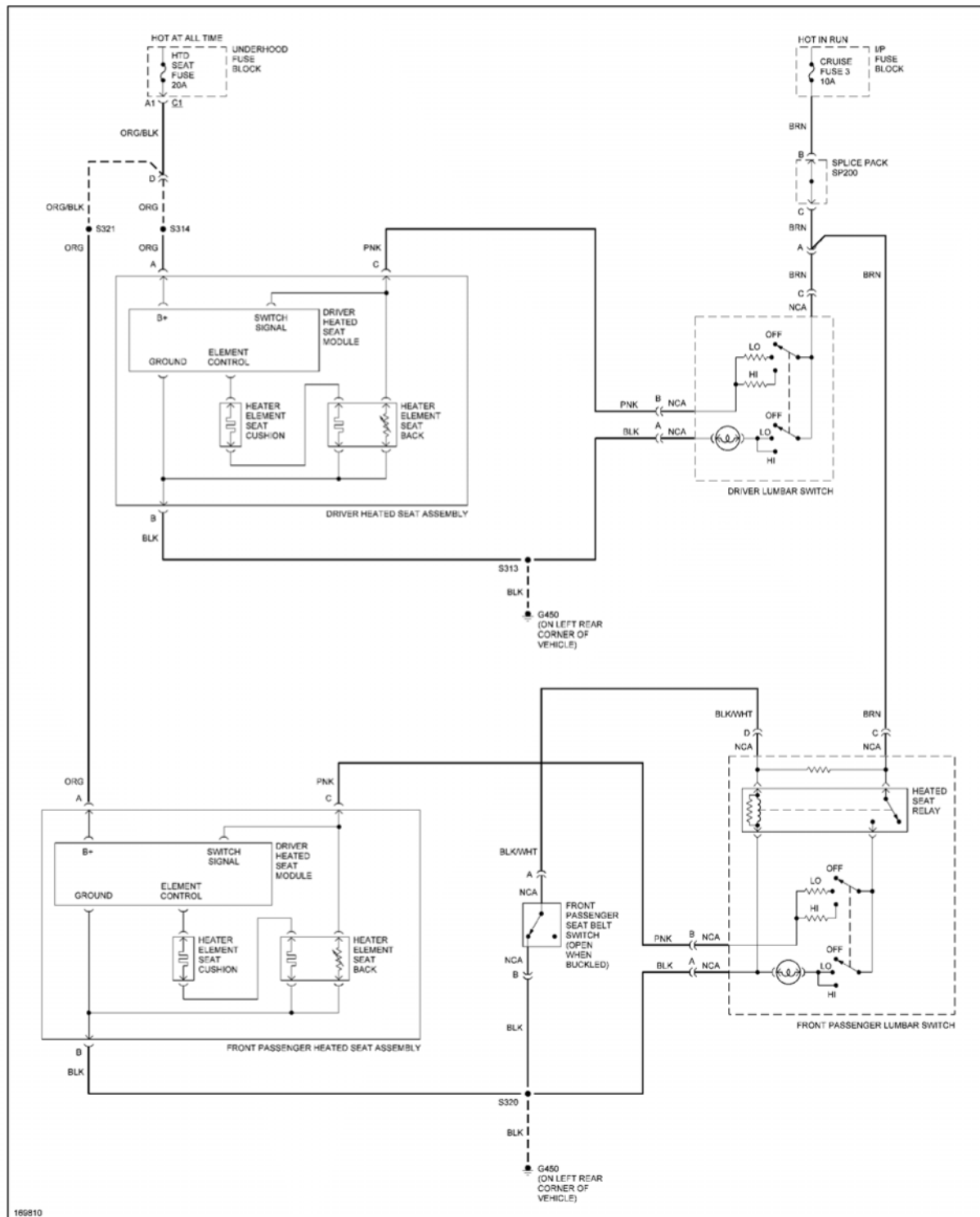
Fig. 37: Heated Seats Circuit
