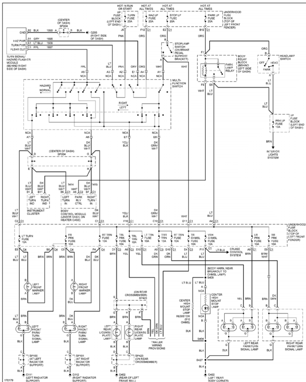
Fig. 15: Exterior Lamps Circuit
