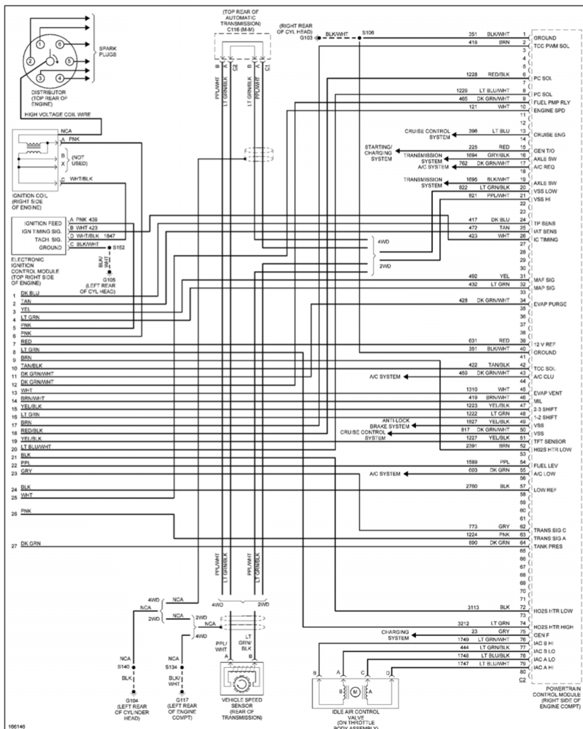
Fig. 13: 4.3L VIN W, Engine Performance Circuit (4 of 4)
