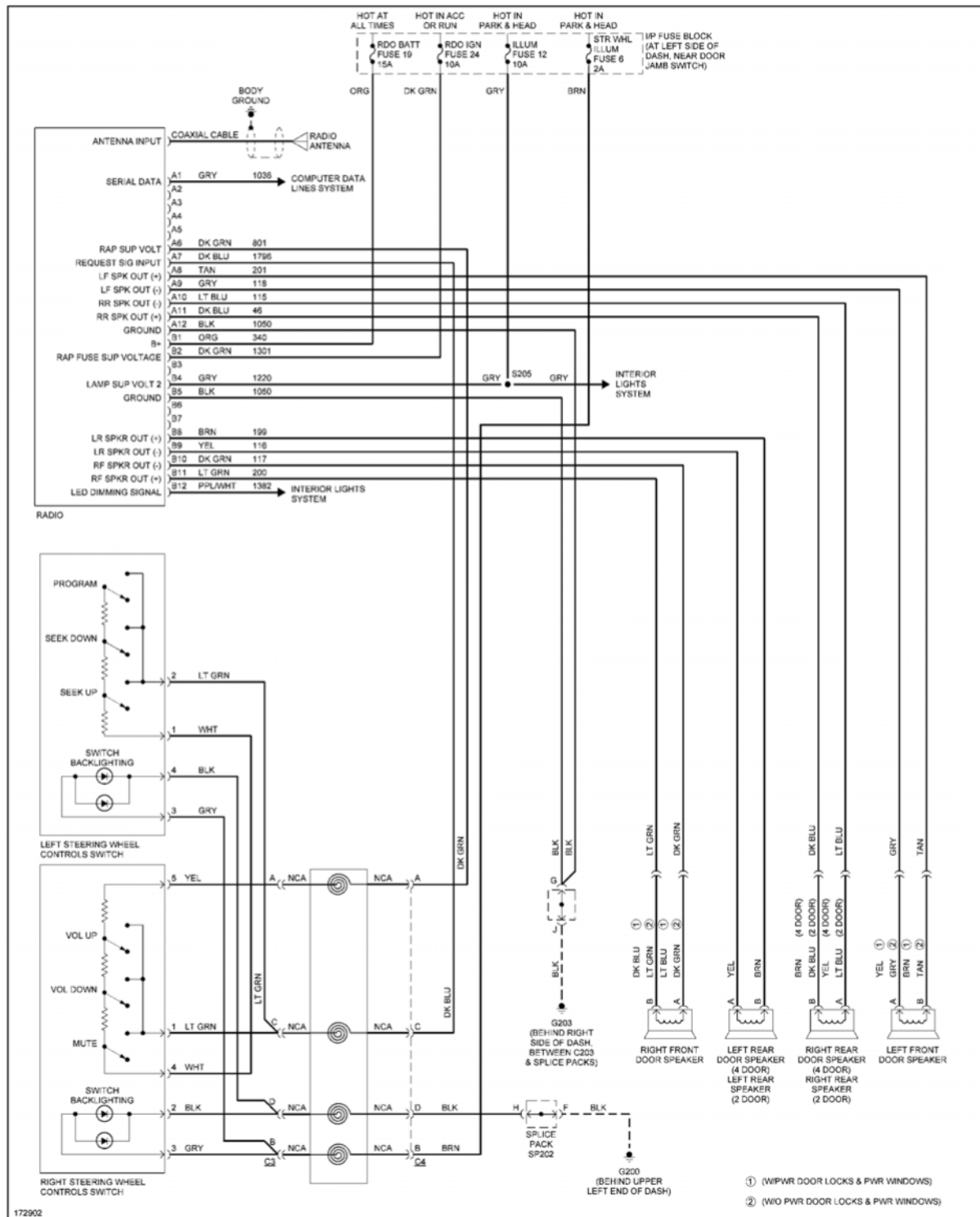
Fig. 43: Radio Circuit
