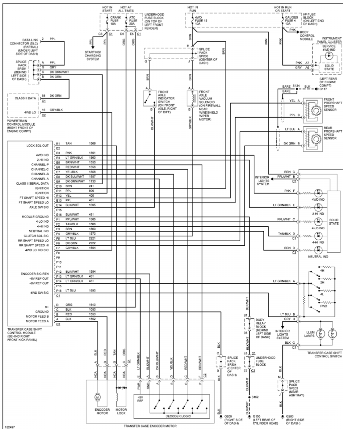
Fig. 50: 4.3L VIN W, Transfer Case Circuit, W/ 2-Speed Automatic Transfer Case
