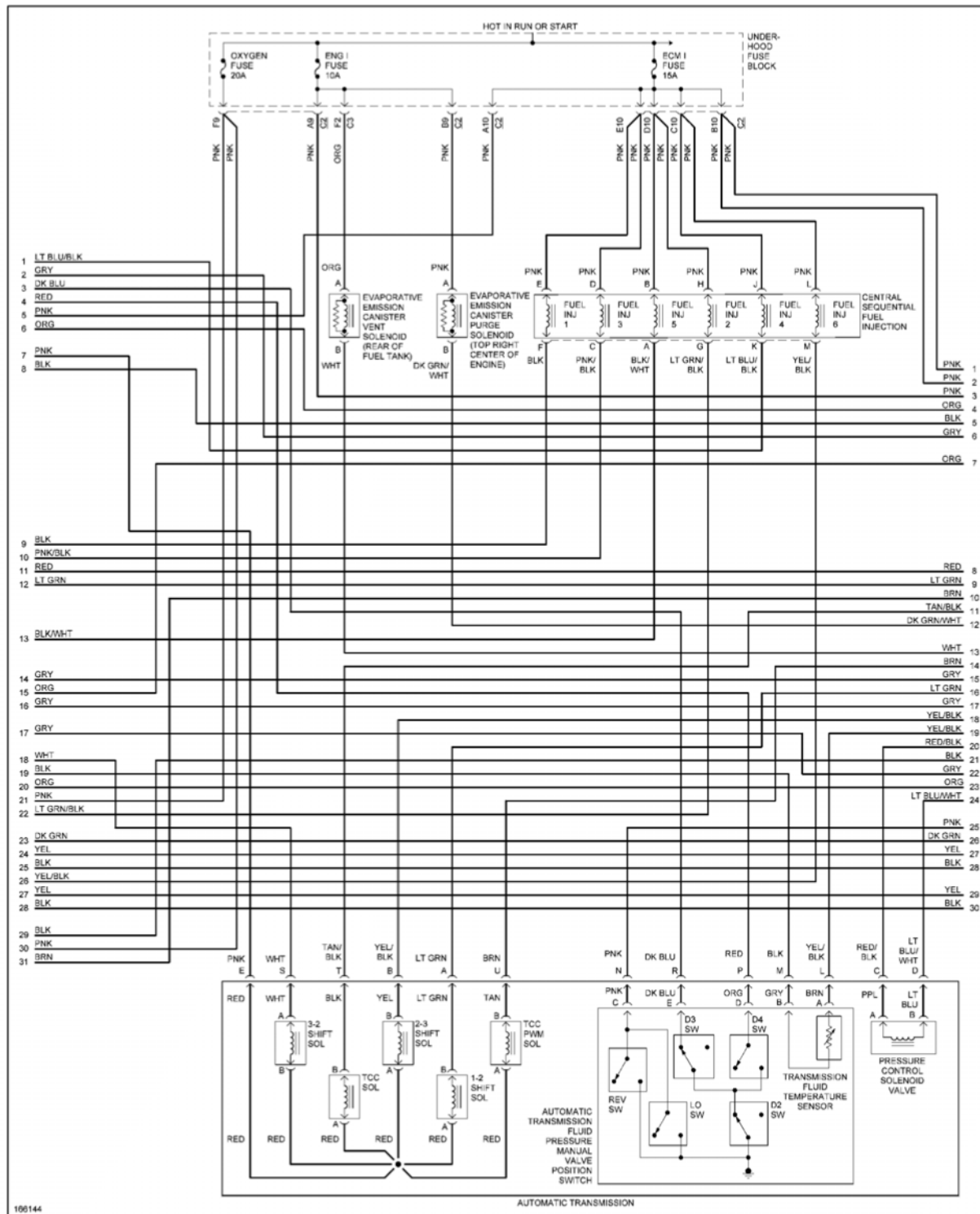
Fig. 11: 4.3L VIN W, Engine Performance Circuit (2 of 4)
