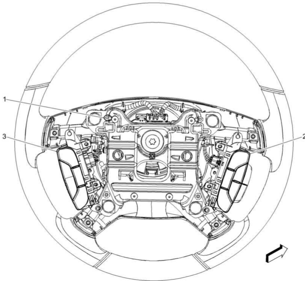
Fig. 7: Identifying Steering Wheel Components Courtesy of GENERAL MOTORS COMPANY
