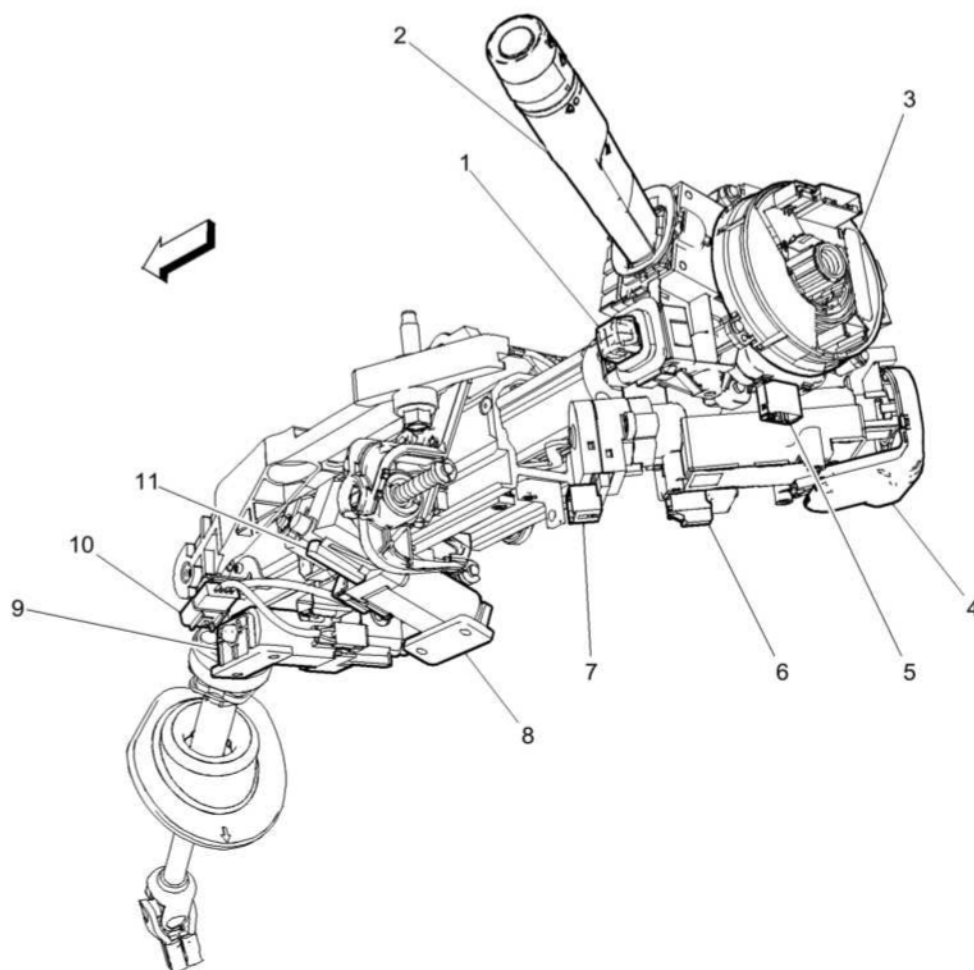
Fig. 11: View Of Steering Column Components Courtesy of GENERAL MOTORS COMPANY
