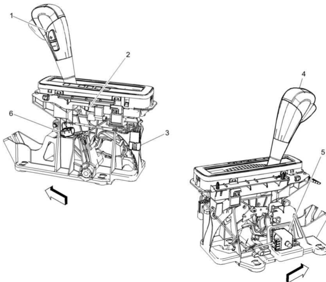
Fig. 12: View Of Automatic Transmission Floor Shifter Courtesy of GENERAL MOTORS COMPANY
