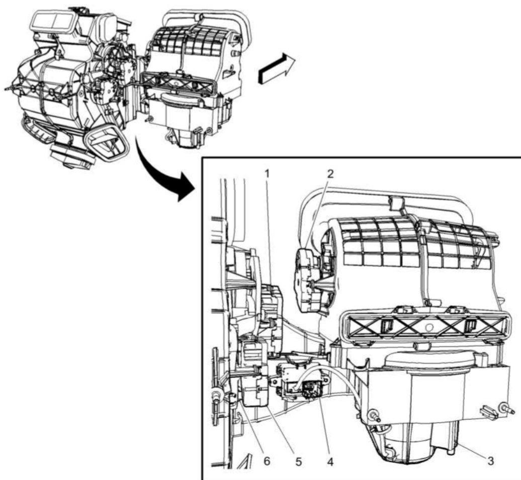
Fig. 5: View Of Front HVAC Module (C67) Courtesy of GENERAL MOTORS COMPANY
