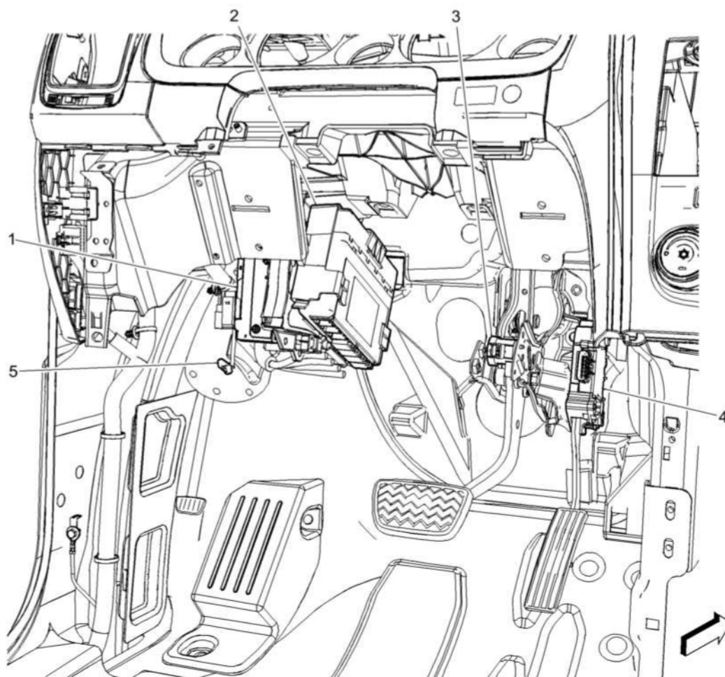
Fig. 15: Identifying Components Below Driver Side Instrument Panel Courtesy of GENERAL MOTORS COMPANY
