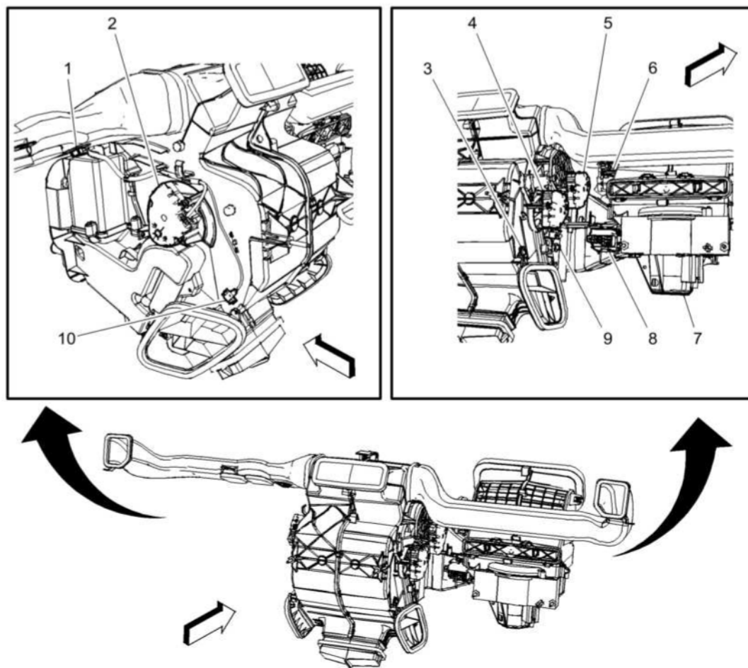
Fig. 2: View Of Air Temperature Sensors Courtesy of GENERAL MOTORS COMPANY
