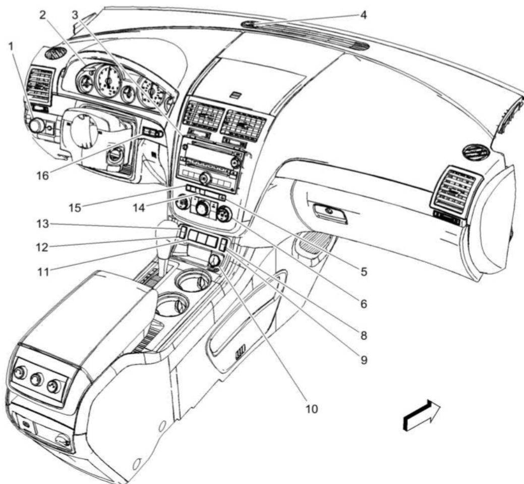
Fig. 16: Locating Instrument Panel Components Courtesy of GENERAL MOTORS COMPANY
