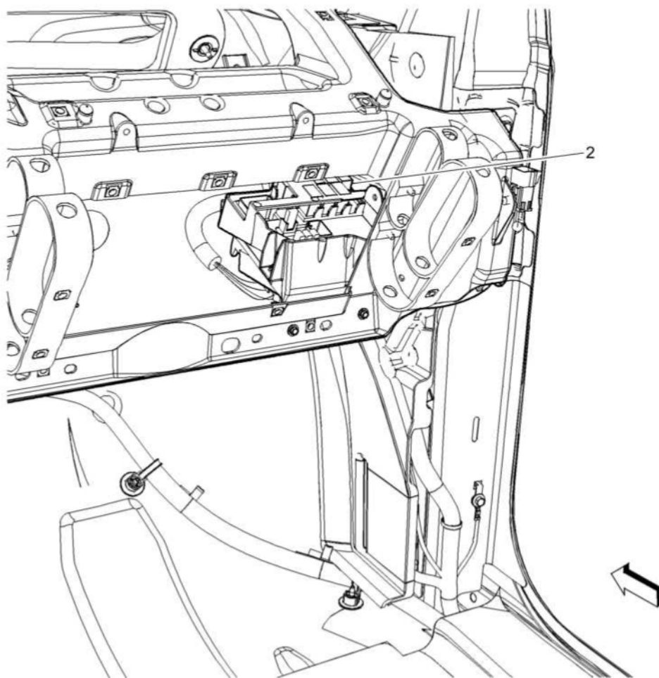
Fig. 13: Instrument Panel Fuse Block Courtesy of GENERAL MOTORS COMPANY
