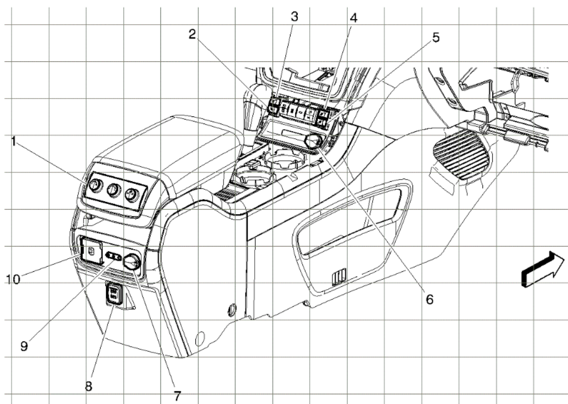
Fig. 18: Locating Console Components
