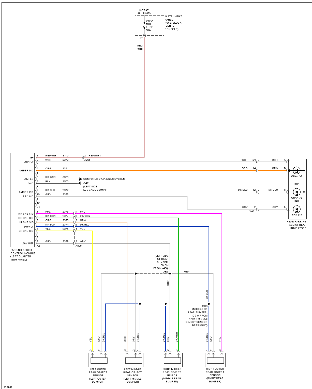
Fig. 47: Parking Assistant Circuit
