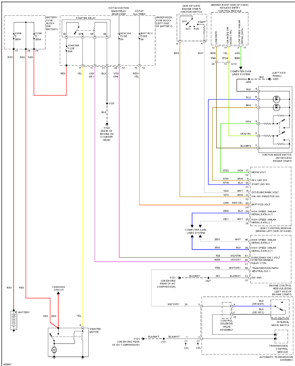
Fig. 125: Starting Circuit, Except Hybrid
