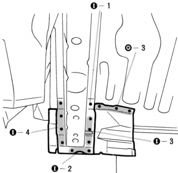
Rear Floor Inner Crossmember
