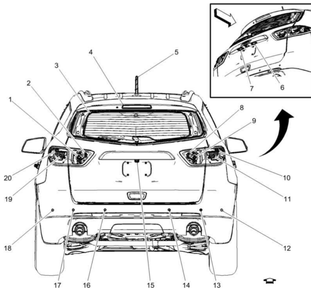
Fig. 5: Rear Of Vehicle Components (X88)
