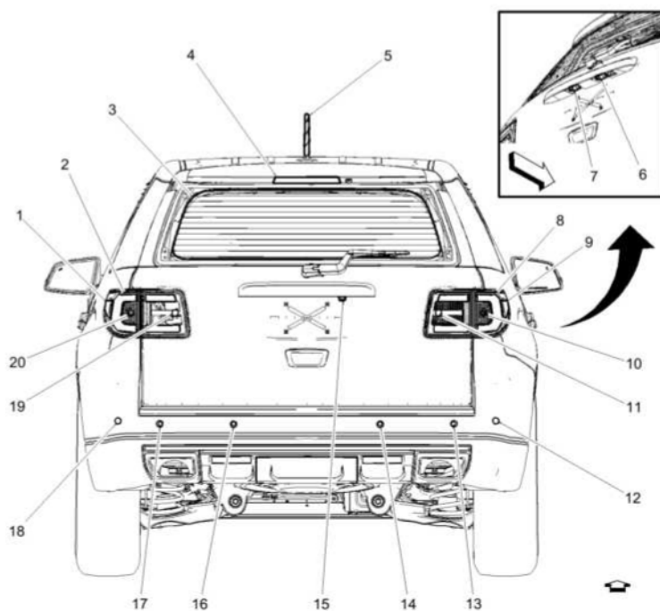
Fig. 7: Rear Of Vehicle Components (Z88)
