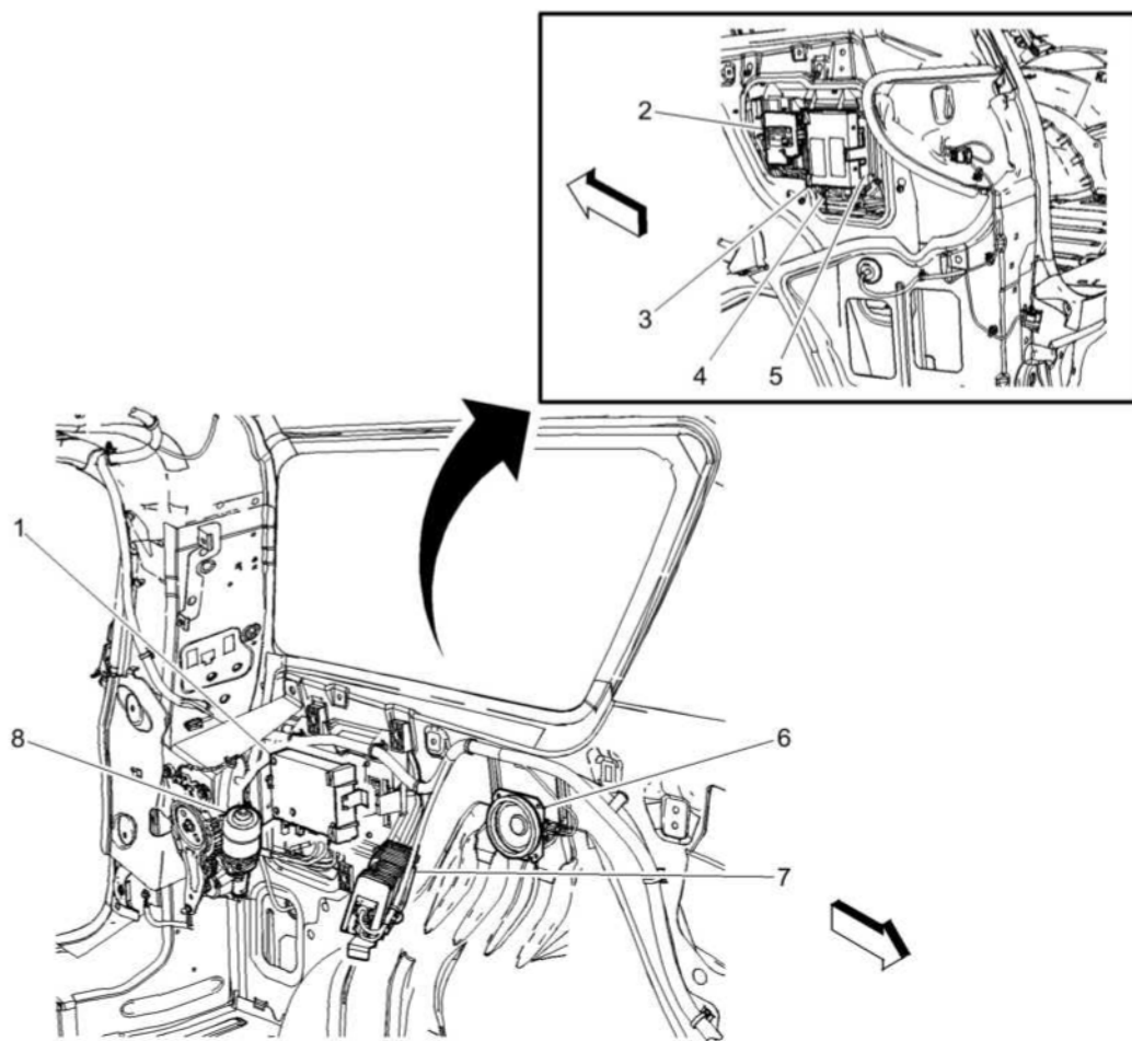
Fig. 10: Left Rear Of Passenger Compartment
