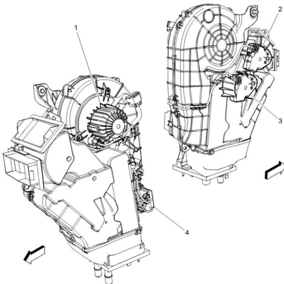
Fig. 1: Identifying Interior HVAC Module - Rear Courtesy of GENERAL MOTORS COMPANY
