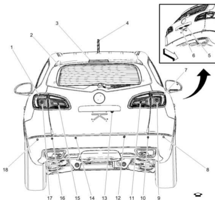
Fig. 6: Rear Of Vehicle Components (W49)
