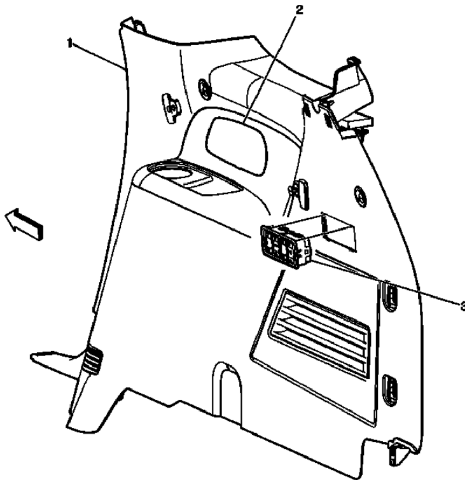
Fig. 3: Identifying Right Rear Trim Panel Courtesy of GENERAL MOTORS COMPANY
