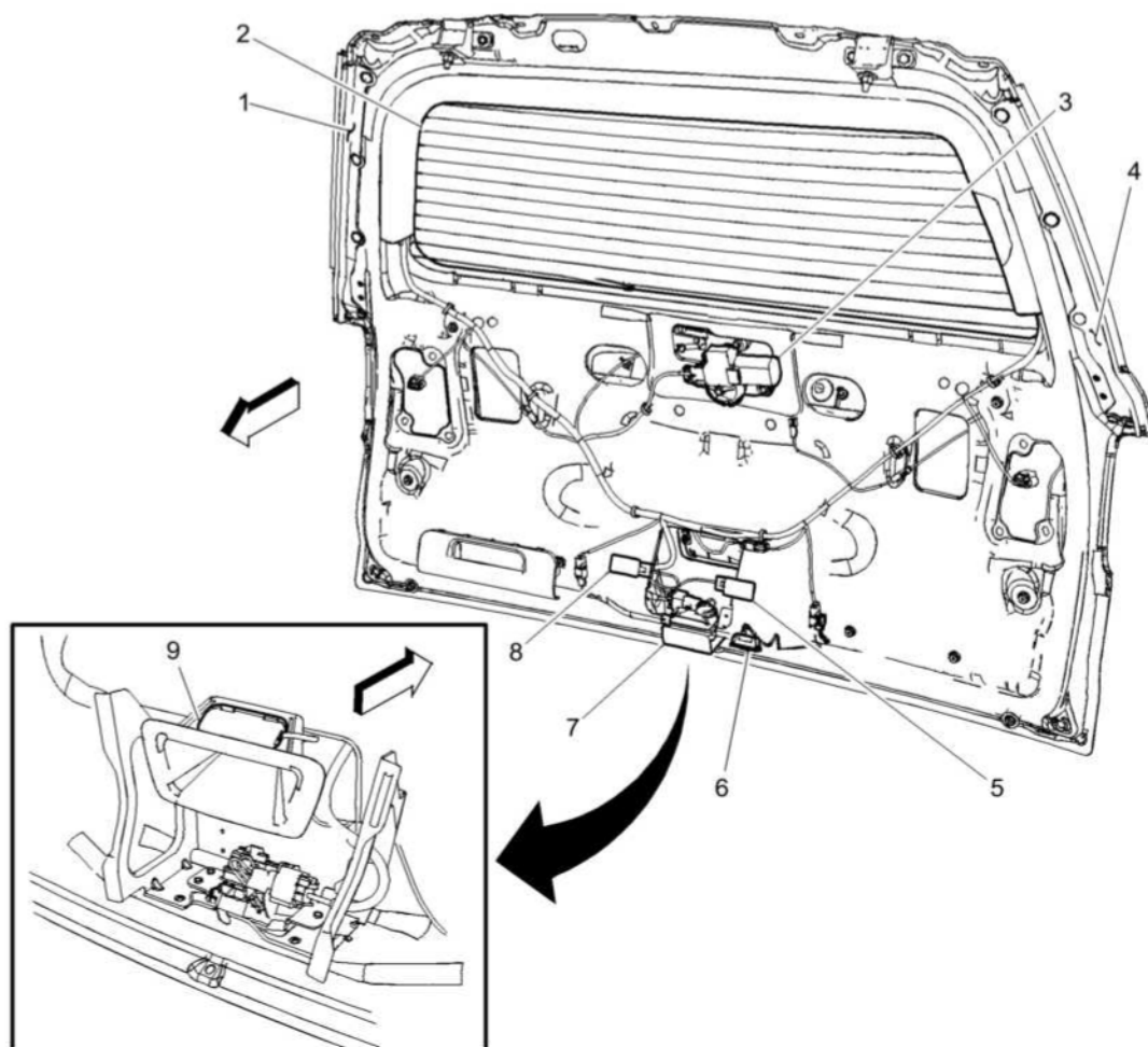
Fig. 4: Identifying Liftgate Components Courtesy of GENERAL MOTORS COMPANY
