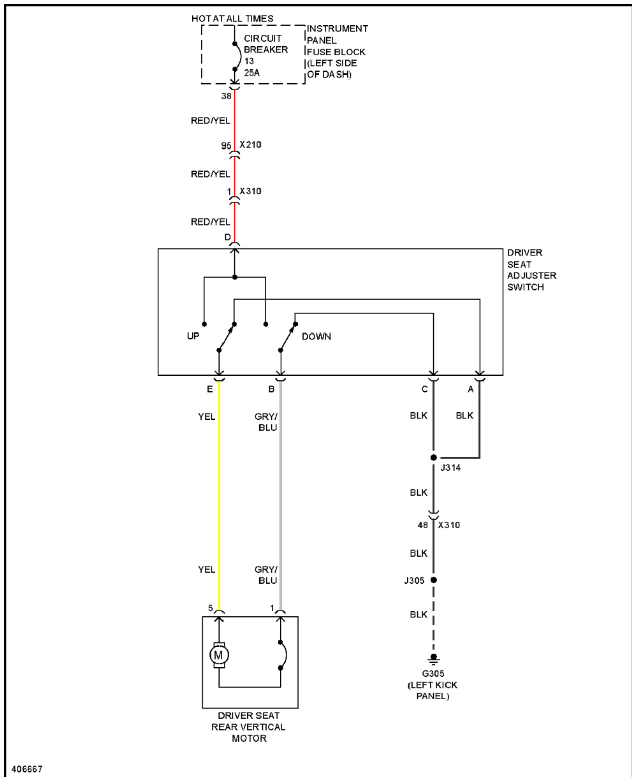
Fig. 102: Driver Power Seat Circuit, 2-Way Power Seat
