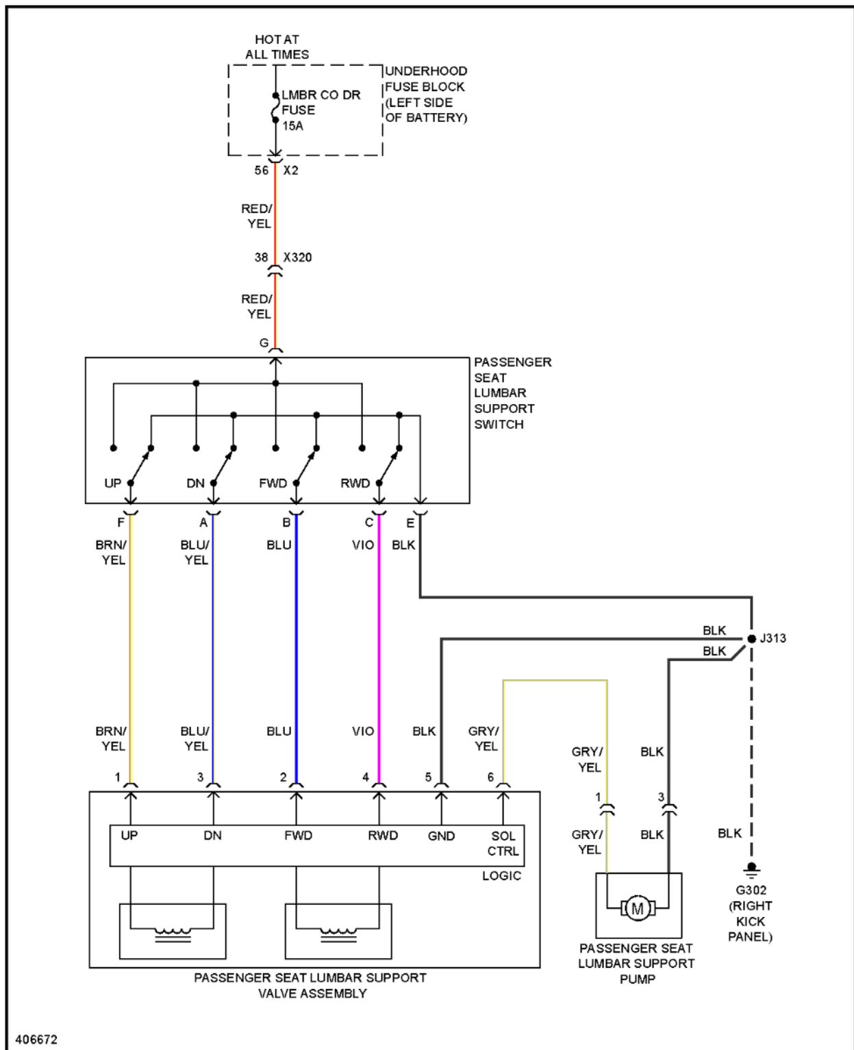
Fig. 109: Passenger's Lumbar Circuit
