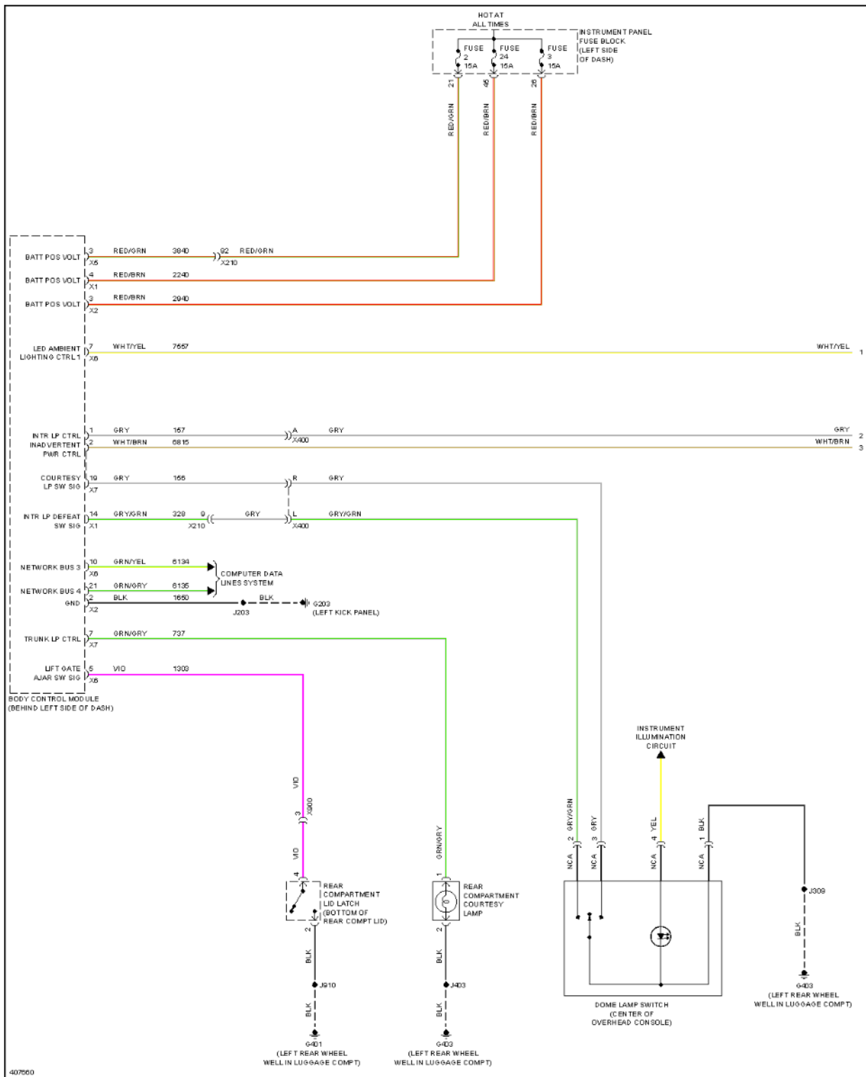
Fig. 68: Courtesy Lamps Circuit (1 of 3)
