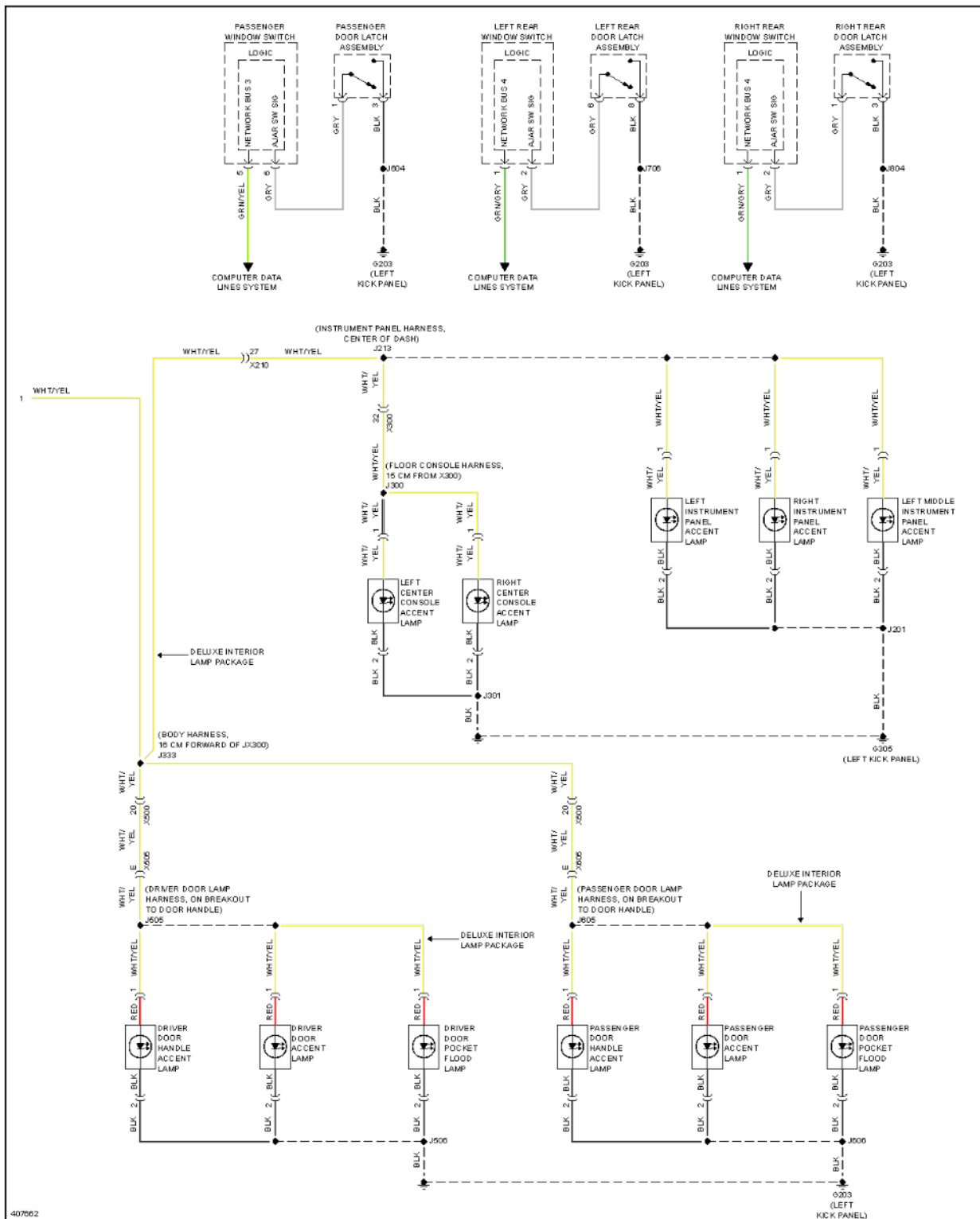
Fig. 70: Courtesy Lamps Circuit (3 of 3)
