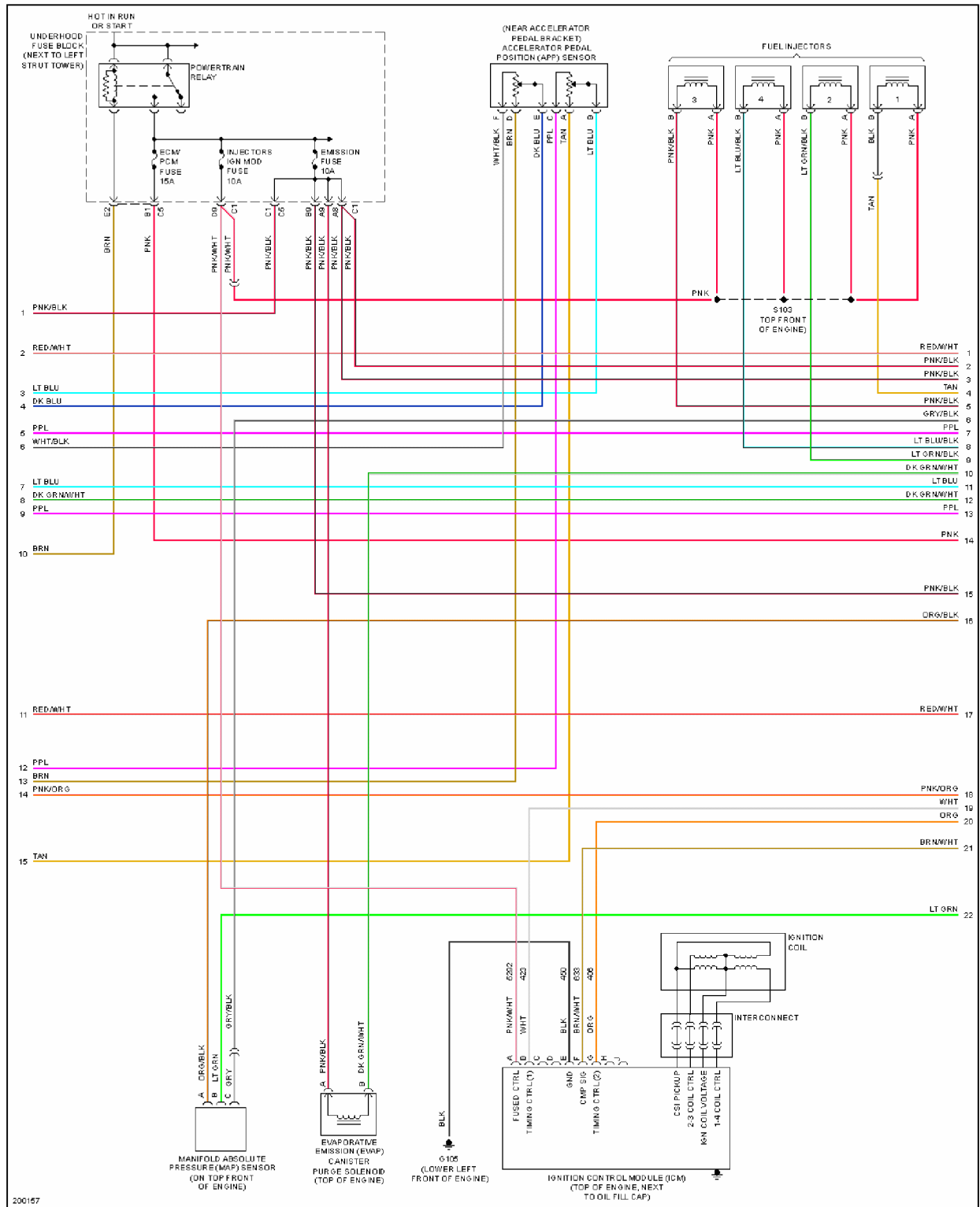
Fig. 26: 2.2L VIN F, Engine Performance Circuit (2 of 4)
