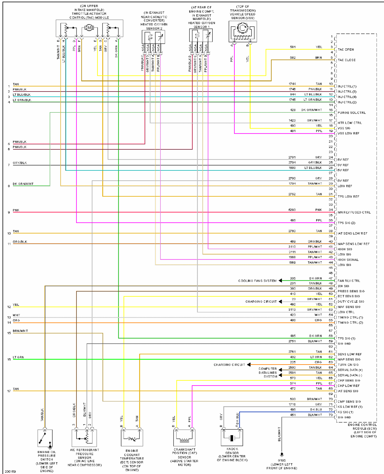
Fig. 28: 2.2L VIN F, Engine Performance Circuit (4 of 4)
