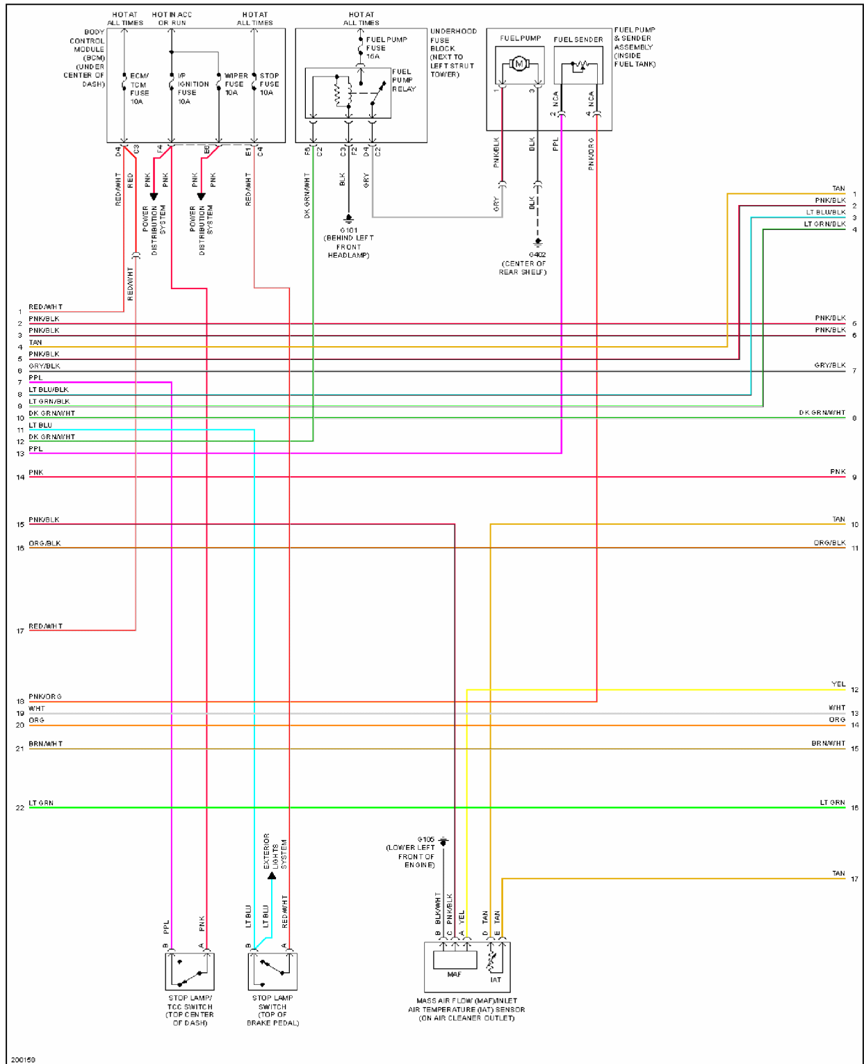
Fig. 27: 2.2L VIN F, Engine Performance Circuit (3 of 4)
