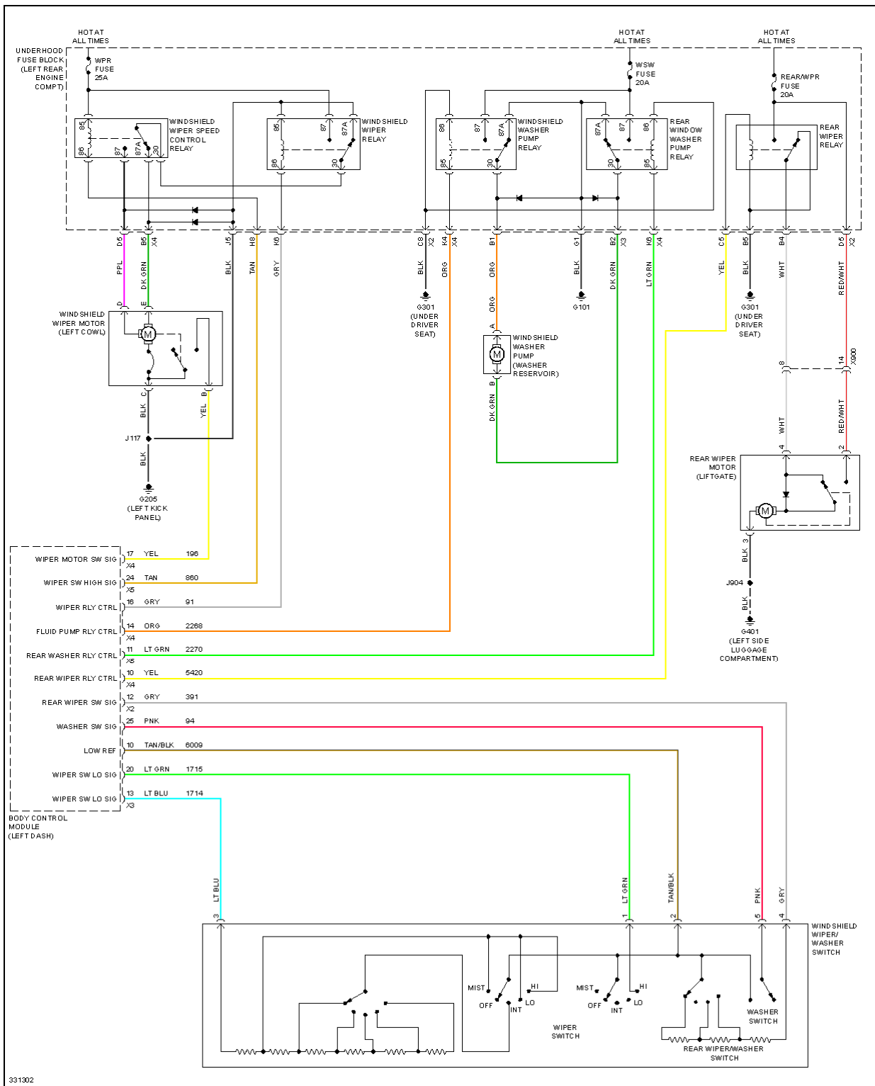
Fig. 82: Wiper/Washer Circuit
