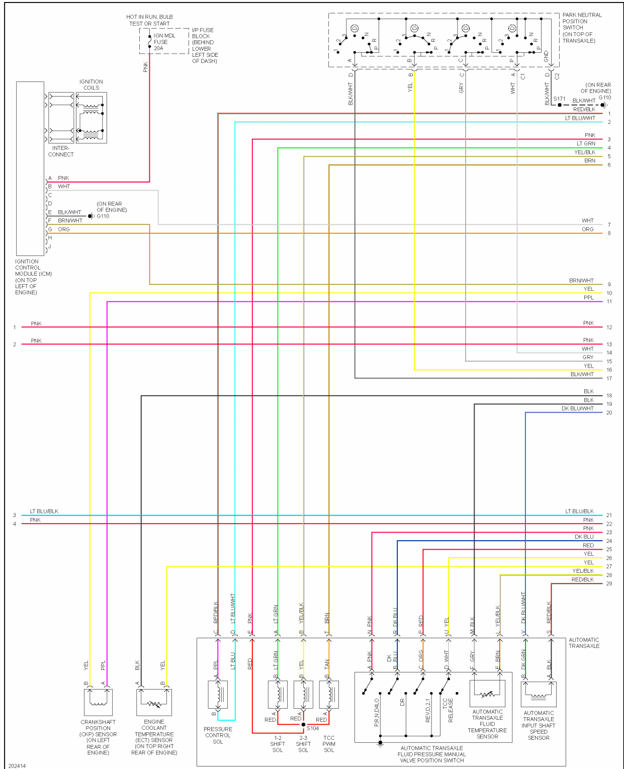
Fig. 11: 2.2L VIN F, Engine Performance Circuit (2 of 3)
