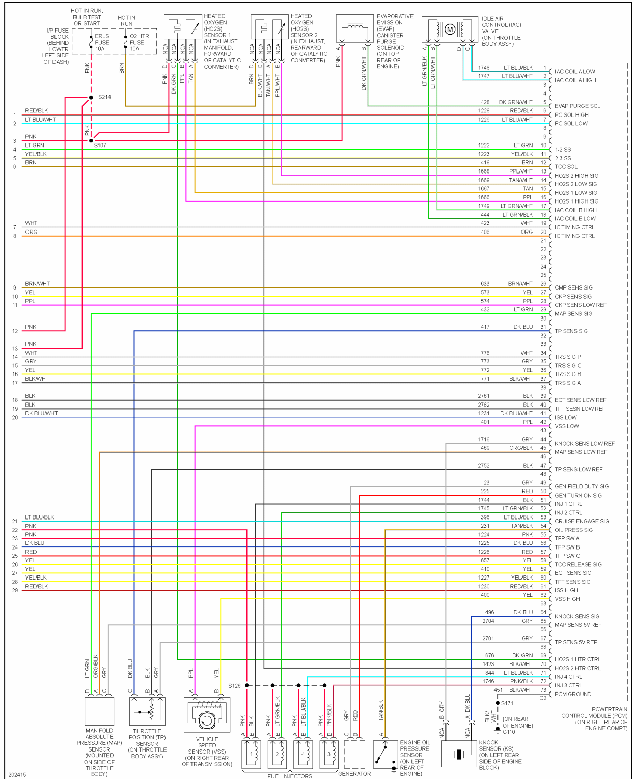
Fig. 12: 2.2L VIN F, Engine Performance Circuit (3 of 3)
