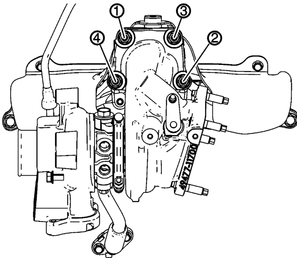
Fig. 26: Turbocharger Nuts In Sequence Courtesy of GENERAL MOTORS COMPANY
