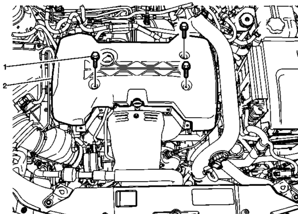
Fig. 2: Intake Manifold Cover (LTG)
