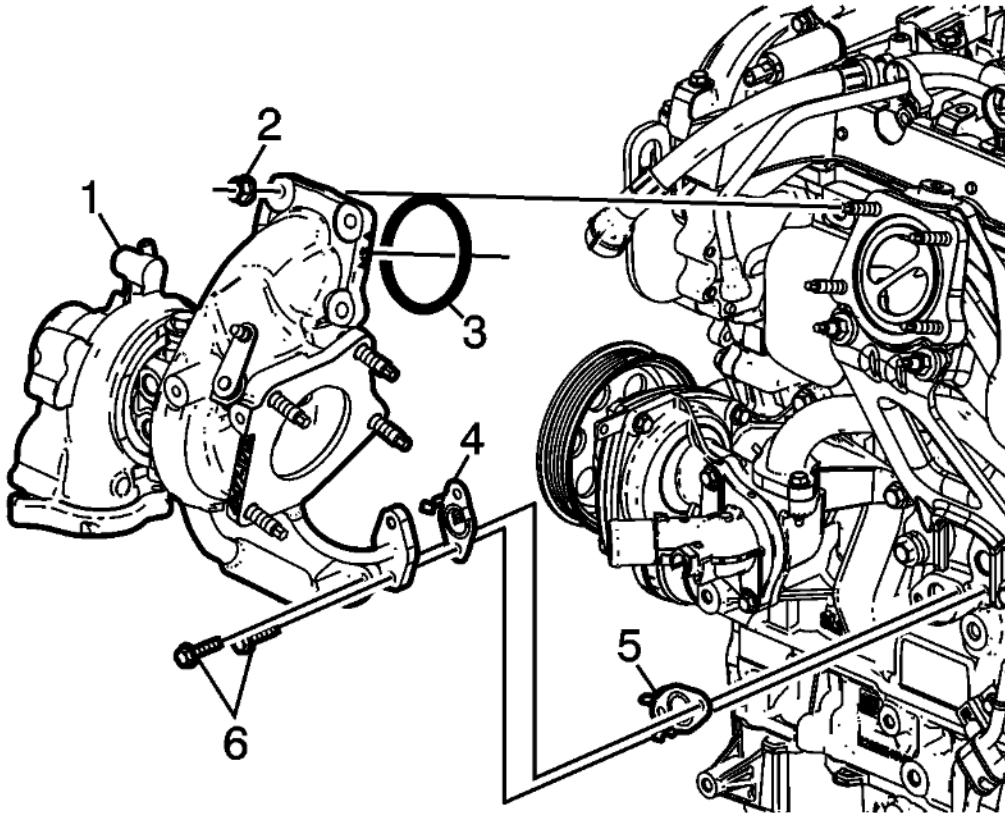
Fig. 25: NEW Turbocharger Gasket And Turbocharger Courtesy of GENERAL MOTORS COMPANY
