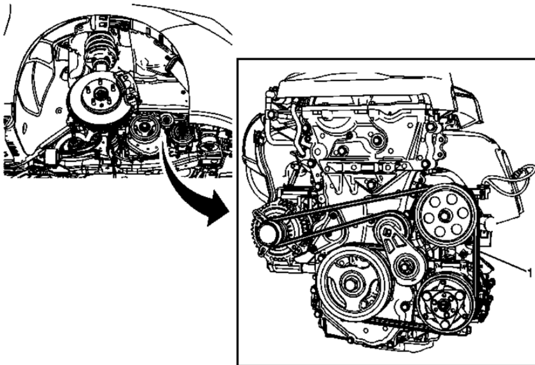
Fig. 3: Drive Belt Routing Courtesy of GENERAL MOTORS COMPANY
