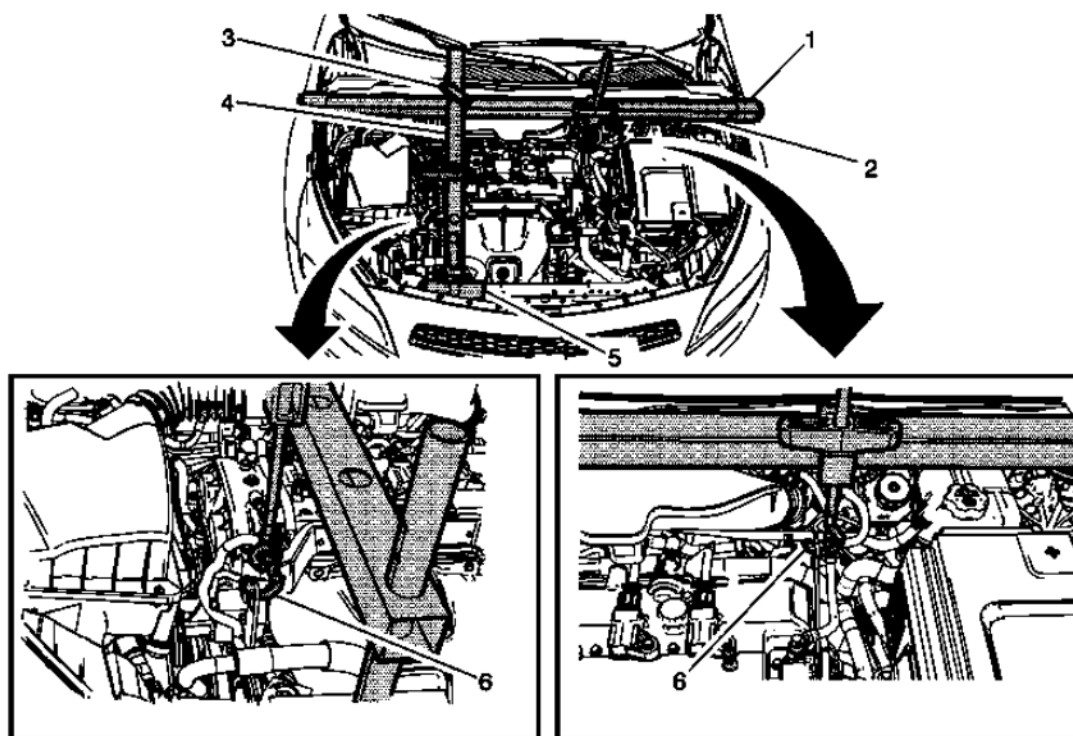
Fig. 18: Engine Support
