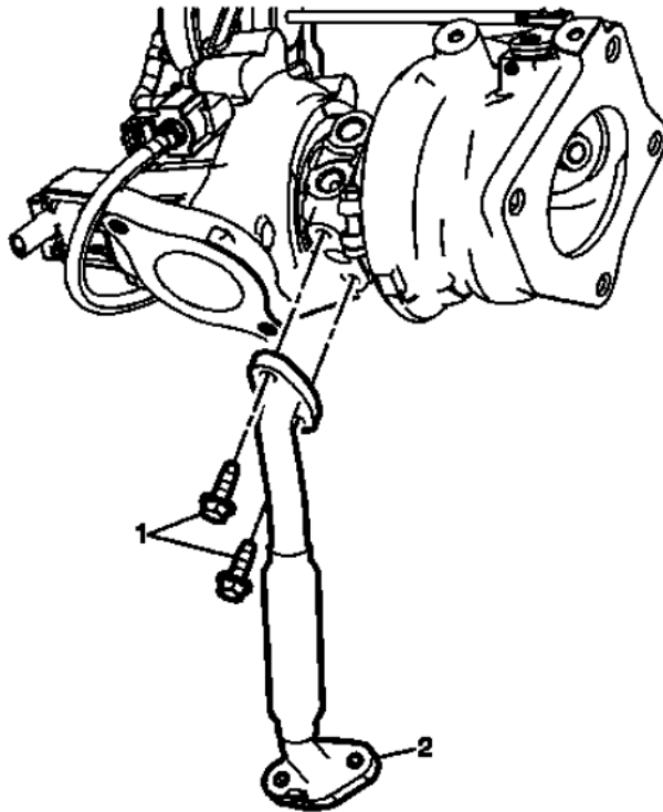
Fig. 29: Turbocharger Oil Return Pipe Courtesy of GENERAL MOTORS COMPANY
