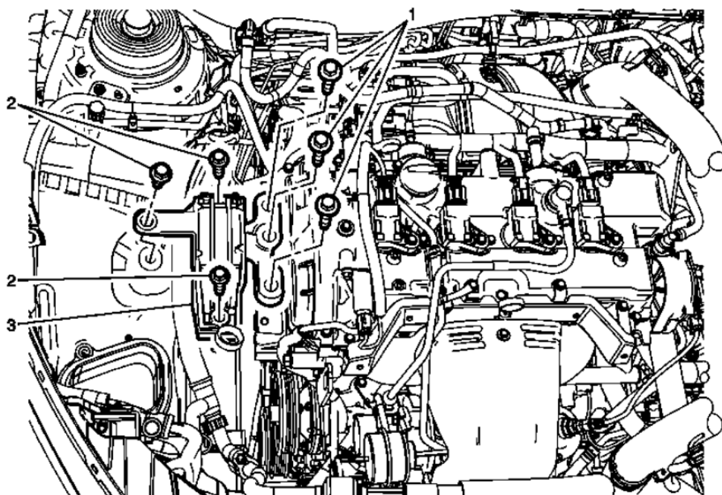
Fig. 17: Engine Mount (LTG)
