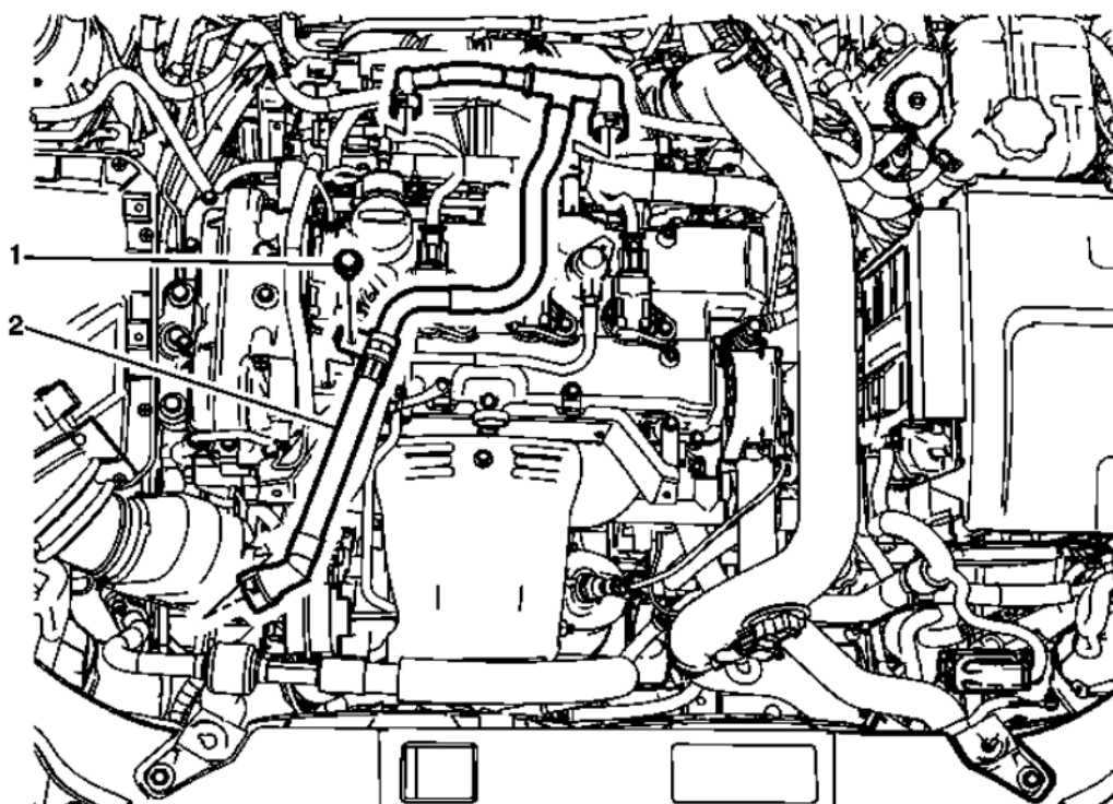
Fig. 35: Positive Crankcase Ventilation Hose/Pipe/Tube Courtesy of GENERAL MOTORS COMPANY
