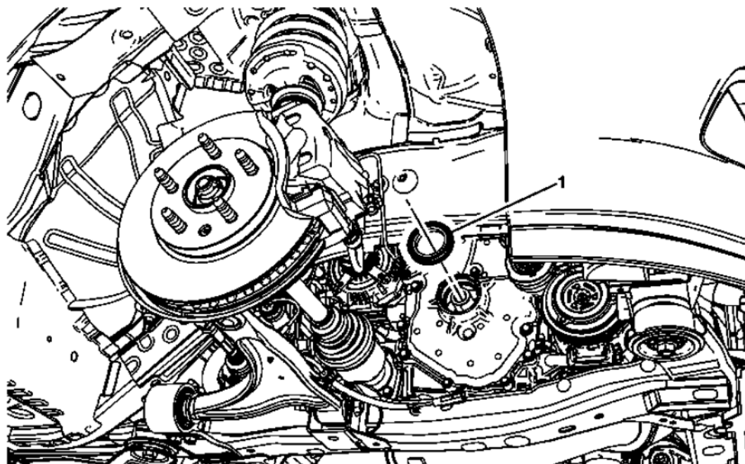
Fig. 69: Crankshaft Front Oil Seal Courtesy of GENERAL MOTORS COMPANY
