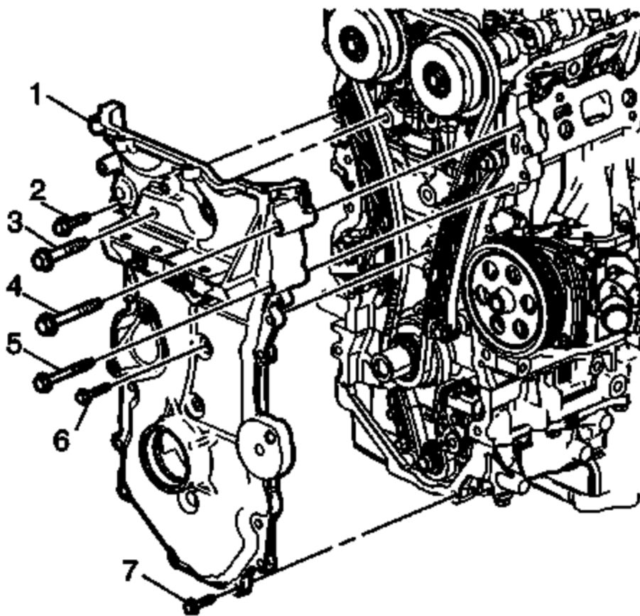
Fig. 84: Engine Front Cover
