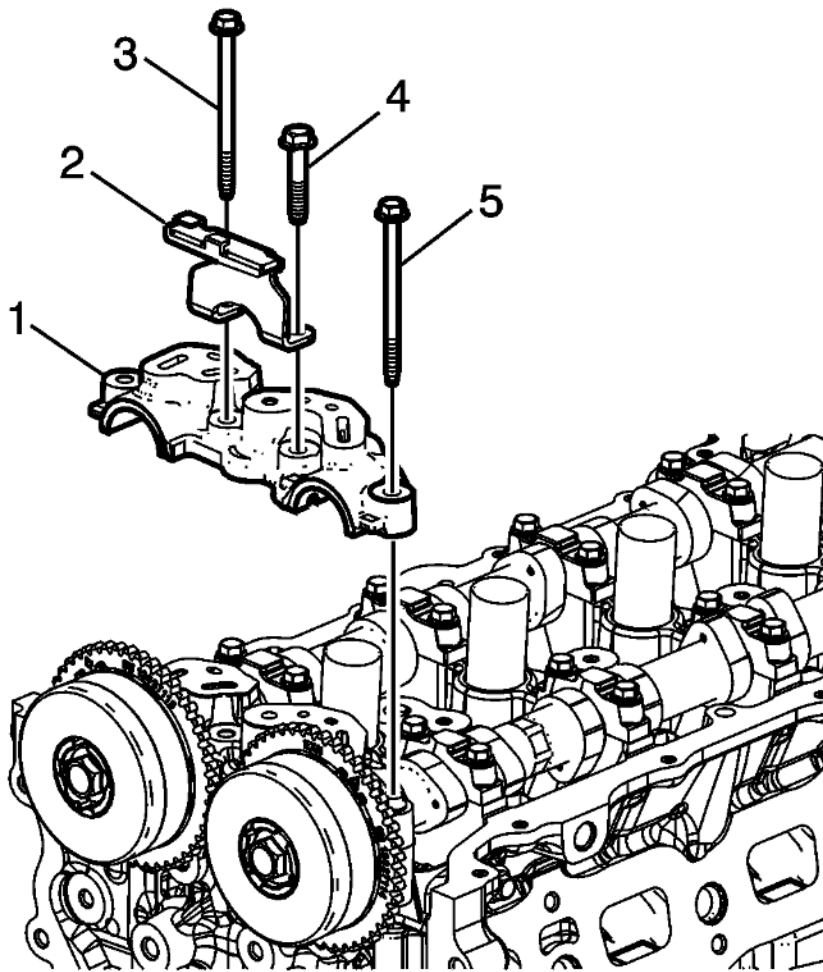
Fig. 188: Front Camshaft Bearing Cap Courtesy of GENERAL MOTORS COMPANY
