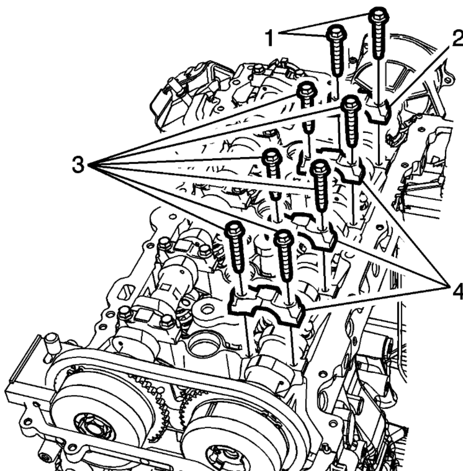
Fig. 158: Exhaust Camshaft Bearing Rear Cap Bolts And Cap Courtesy of GENERAL MOTORS COMPANY
