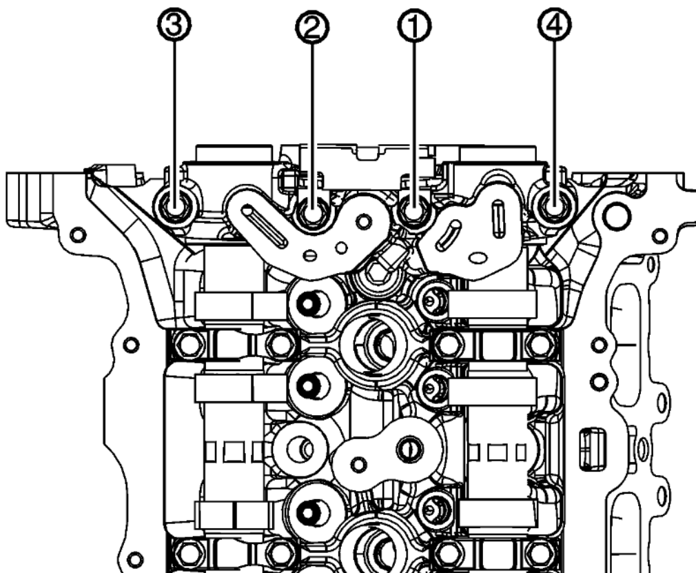
Fig. 108: Front Camshaft Cap Bolts In Sequence Courtesy of GENERAL MOTORS COMPANY
