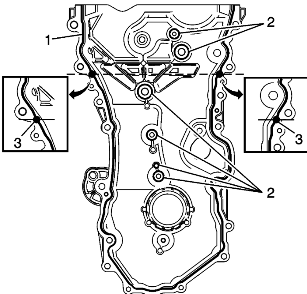
Fig. 83: Applying Bead Of Sealer Directly In Flange Courtesy of GENERAL MOTORS COMPANY
