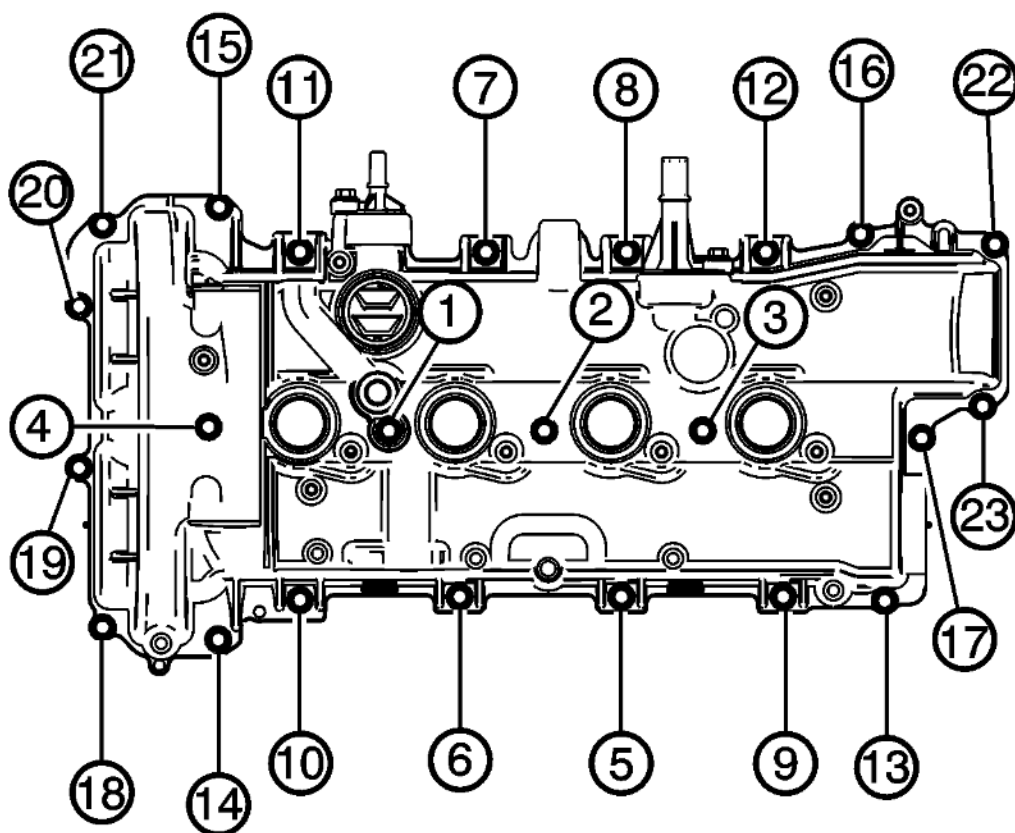
Fig. 120: Camshaft Cover Bolts In Sequence Courtesy of GENERAL MOTORS COMPANY
