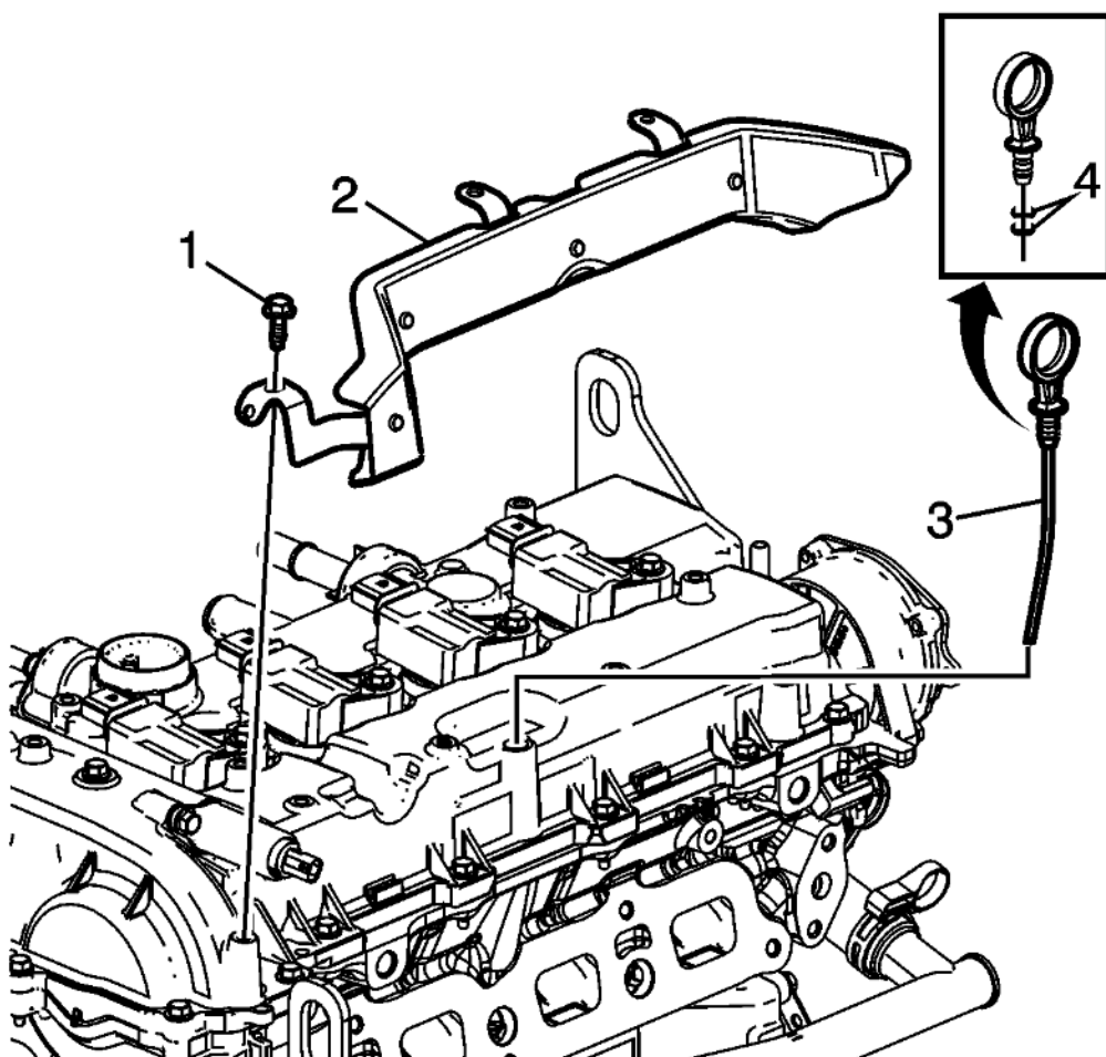
Fig. 126: Oil Level Indicator
