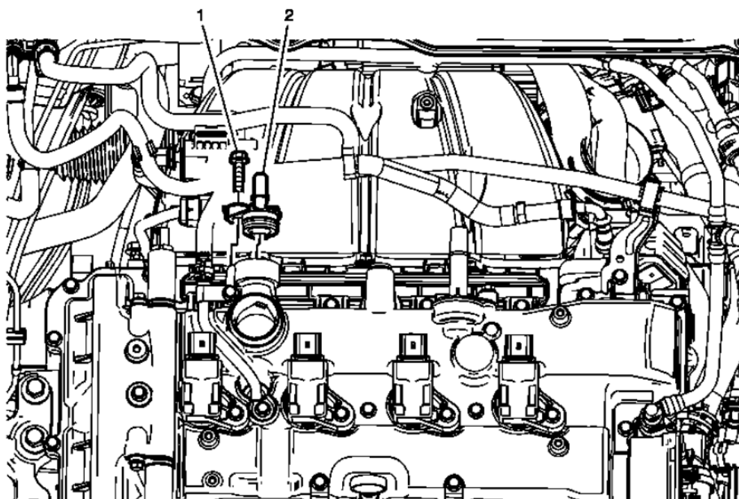
Fig. 32: Positive Crankcase Ventilation Valve (Front)
