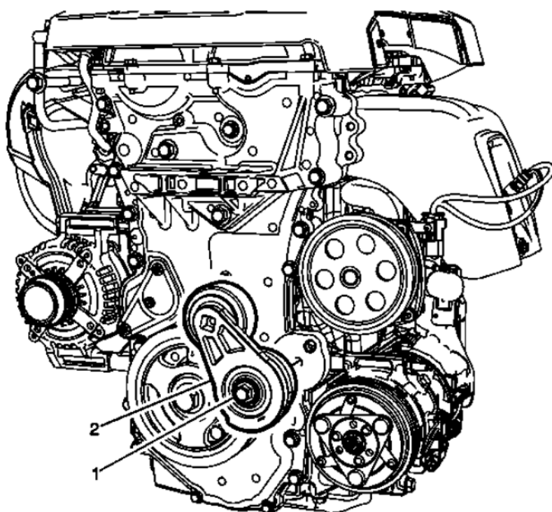
Fig. 4: Drive Belt Tensioner
