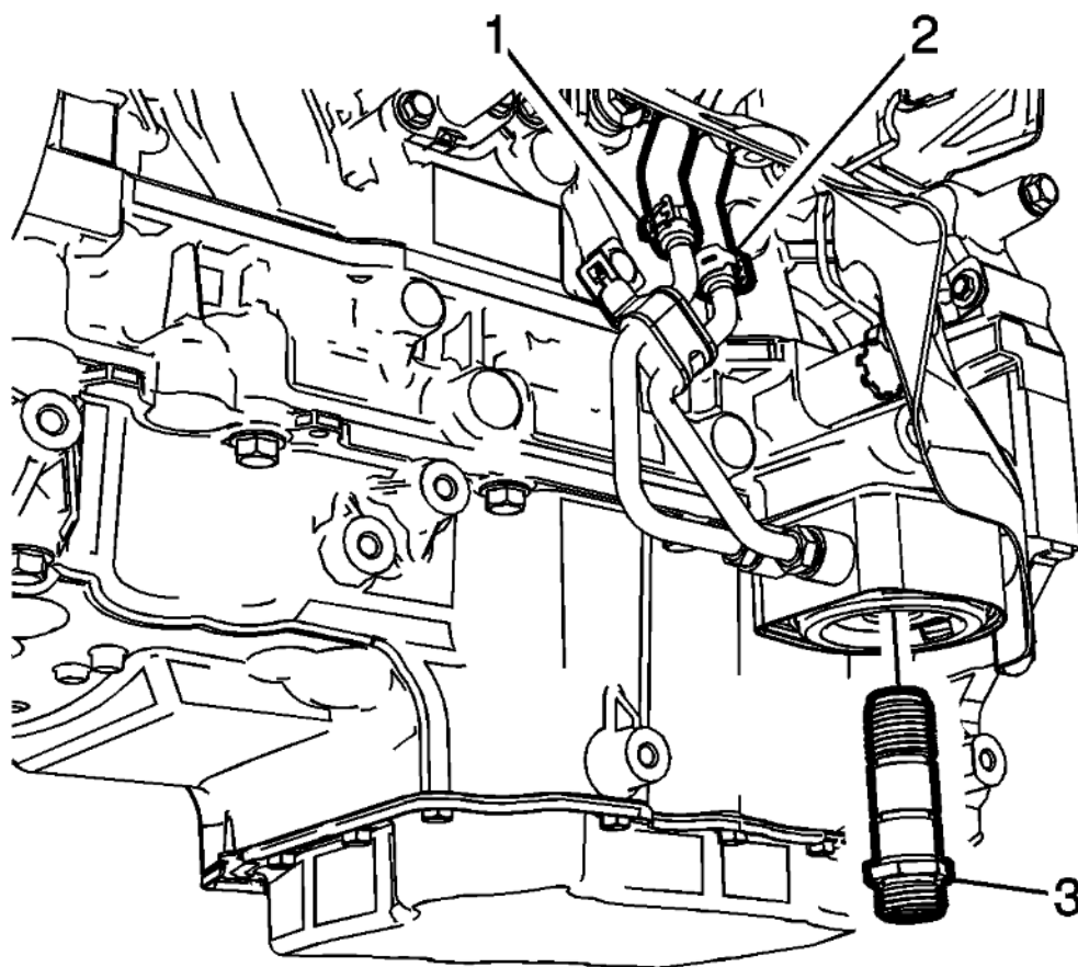
Fig. 204: Engine Oil Cooler Connector Courtesy of GENERAL MOTORS COMPANY
