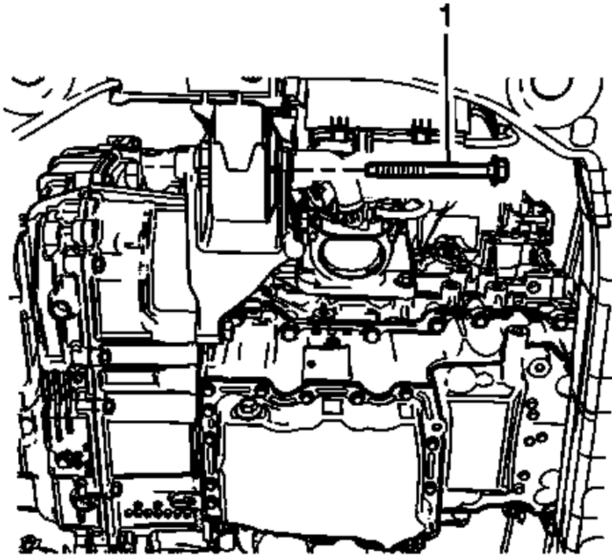
Fig. 6: Rear Transaxle Mount Through Bolt Courtesy of GENERAL MOTORS COMPANY
