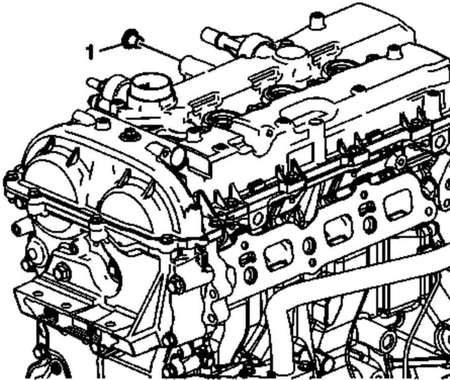
Fig. 121: Camshaft Cover Plug
