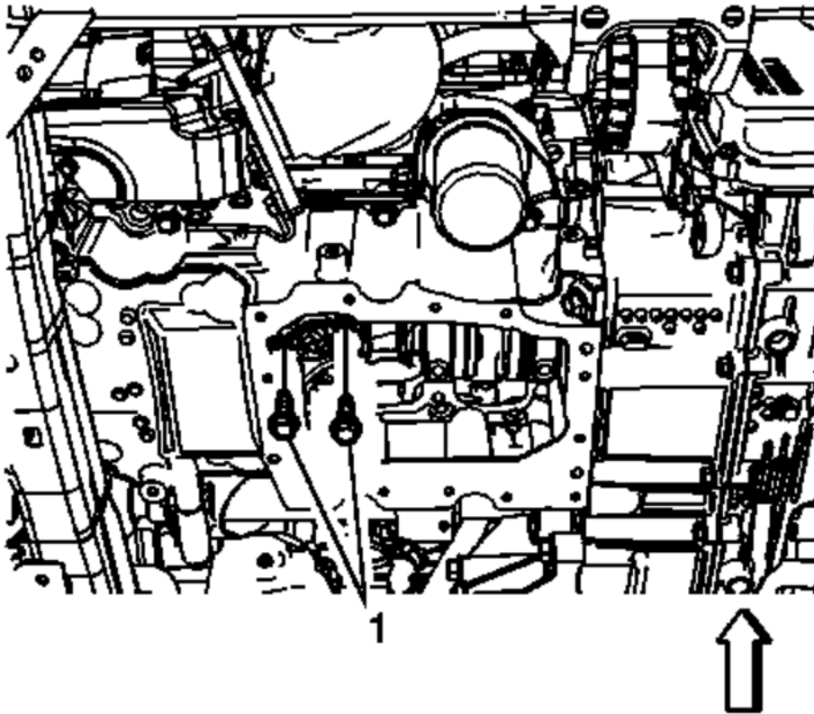
Fig. 213: Engine Oil Level Sensor Fasteners Courtesy of GENERAL MOTORS COMPANY
