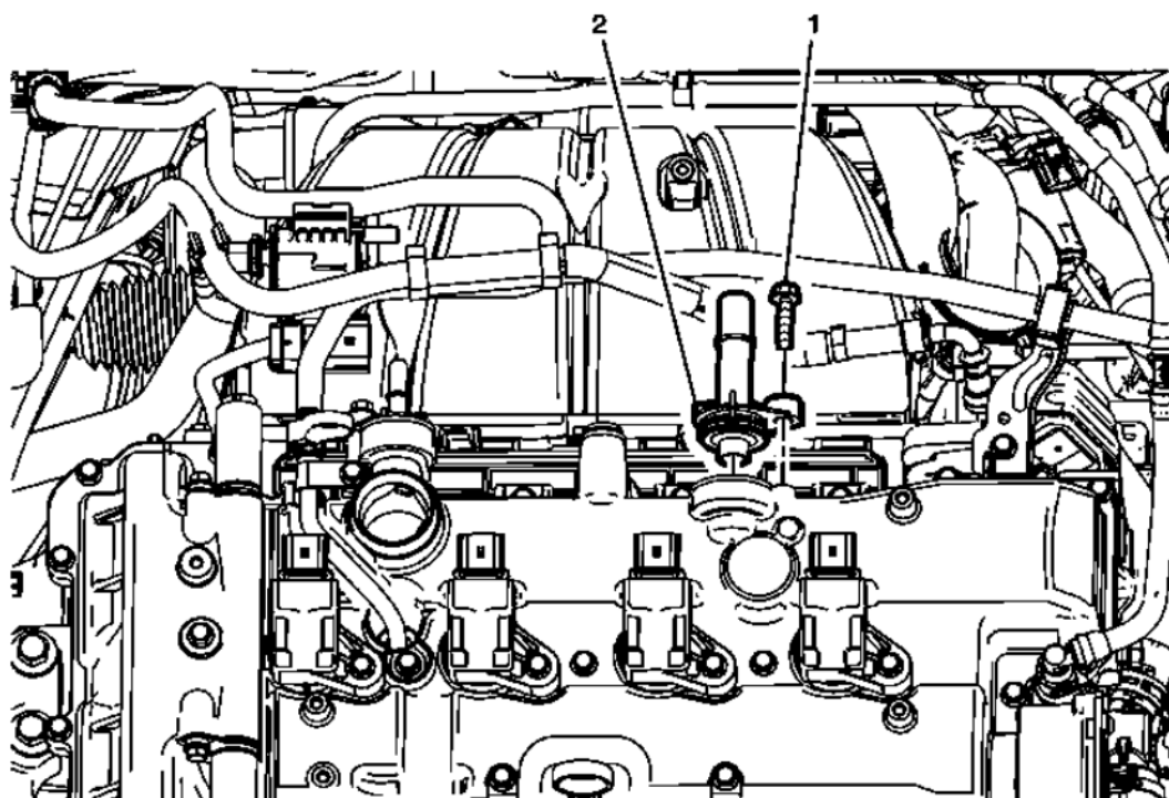
Fig. 31: Positive Crankcase Ventilation Valve (Rear)
