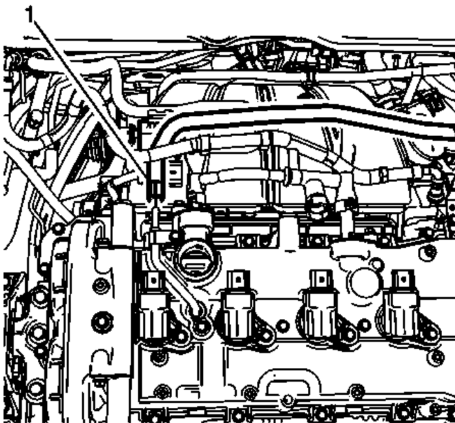
Fig. 147: Surge Tank Hose
