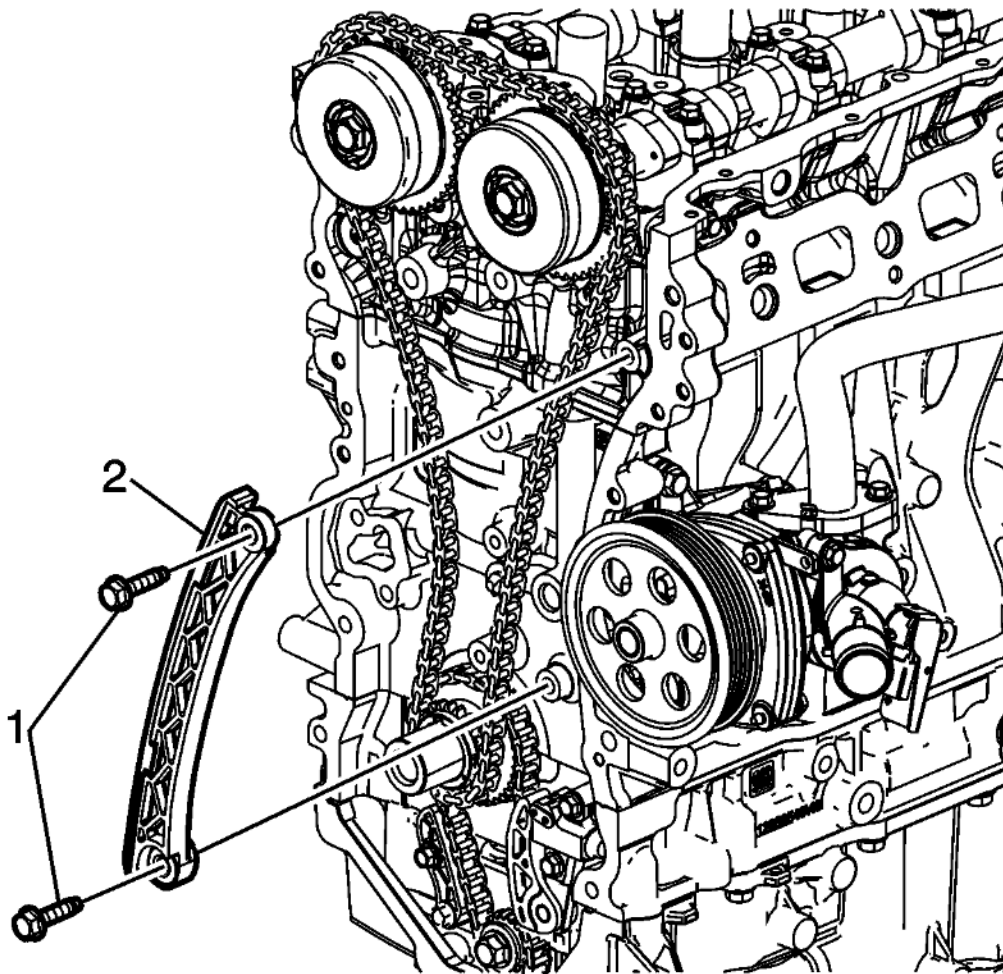
Fig. 97: Timing Chain Guide Bolts Courtesy of GENERAL MOTORS COMPANY
