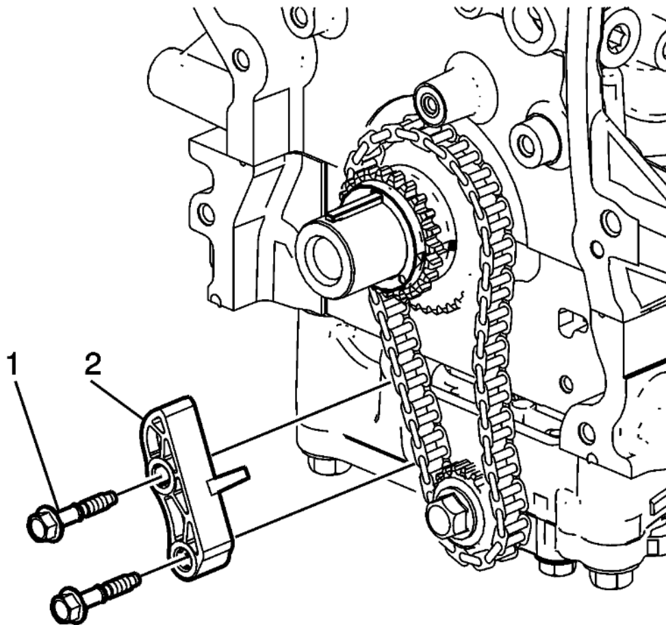
Fig. 60: Balancer Chain Guide Bolt Courtesy of GENERAL MOTORS COMPANY
