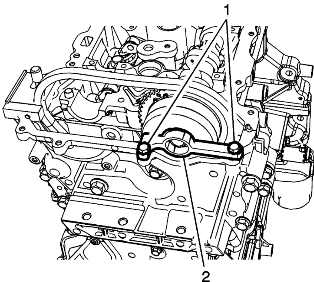
Fig. 166: Camshaft Actuator Locking Tool EN 50793 Courtesy of GENERAL MOTORS COMPANY
