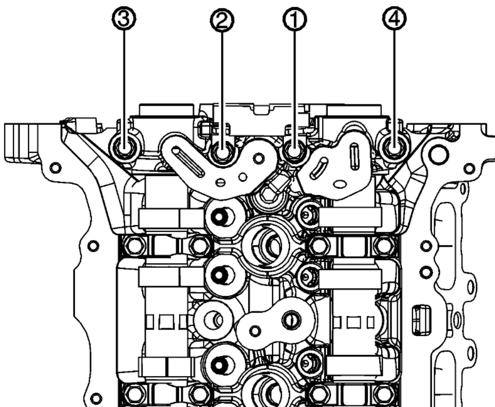
Fig. 175: Front Camshaft Cap Bolts In Sequence Courtesy of GENERAL MOTORS COMPANY
