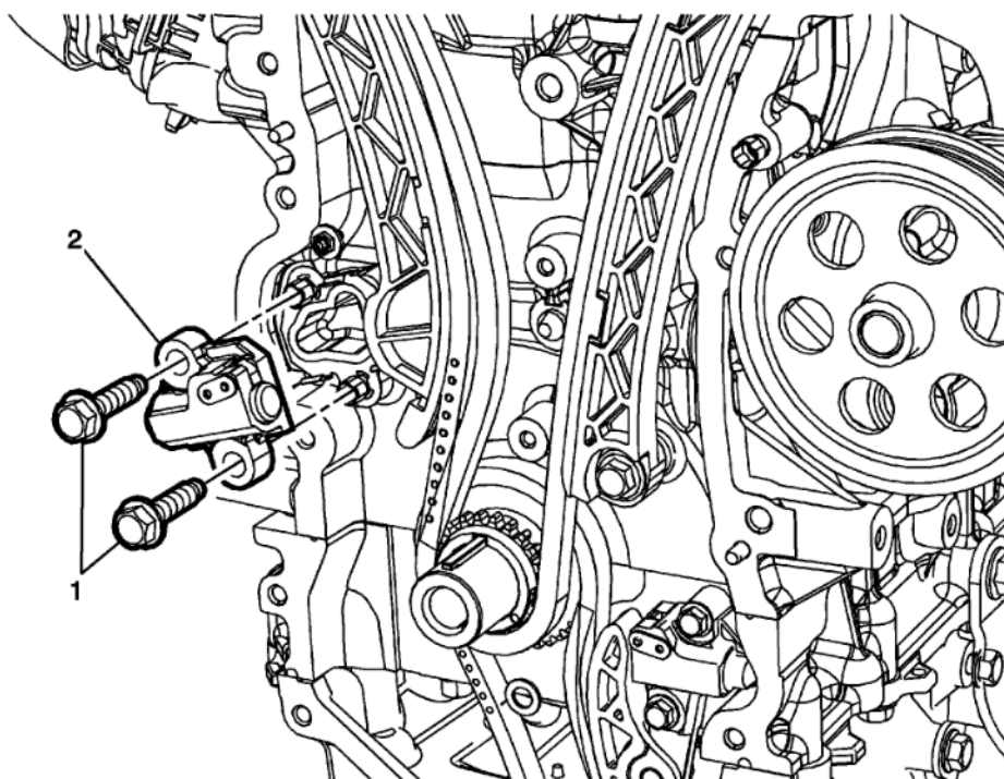
Fig. 105: Timing Chain Tensioner Bolts And Timing Chain Tensioner Courtesy of GENERAL MOTORS COMPANY
