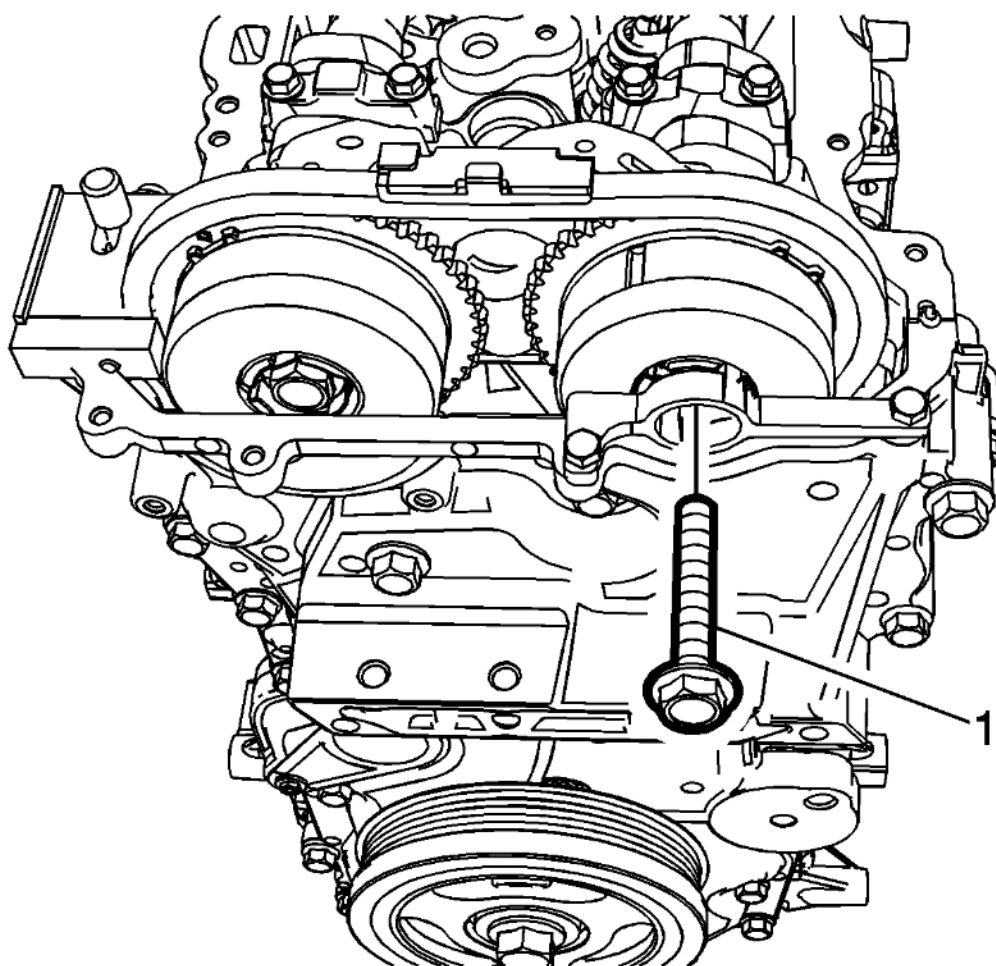
Fig. 179: Camshaft Actuator Bolt Courtesy of GENERAL MOTORS COMPANY
