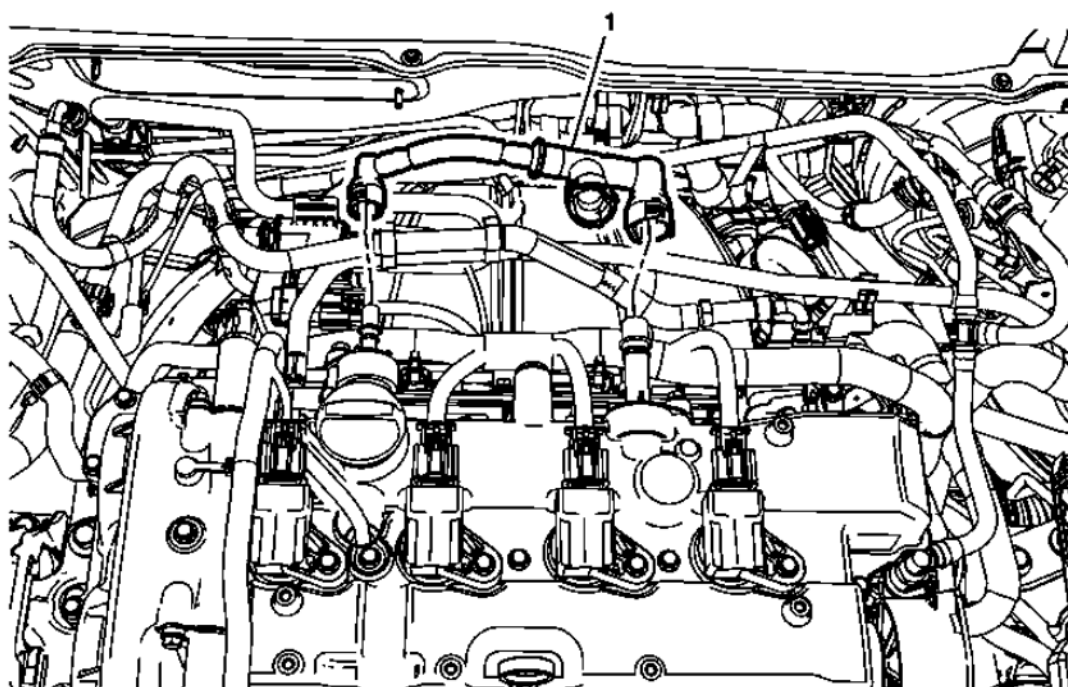
Fig. 34: Positive Crankcase Ventilation Hose/Pipe/Tube (LCV) Courtesy of GENERAL MOTORS COMPANY
