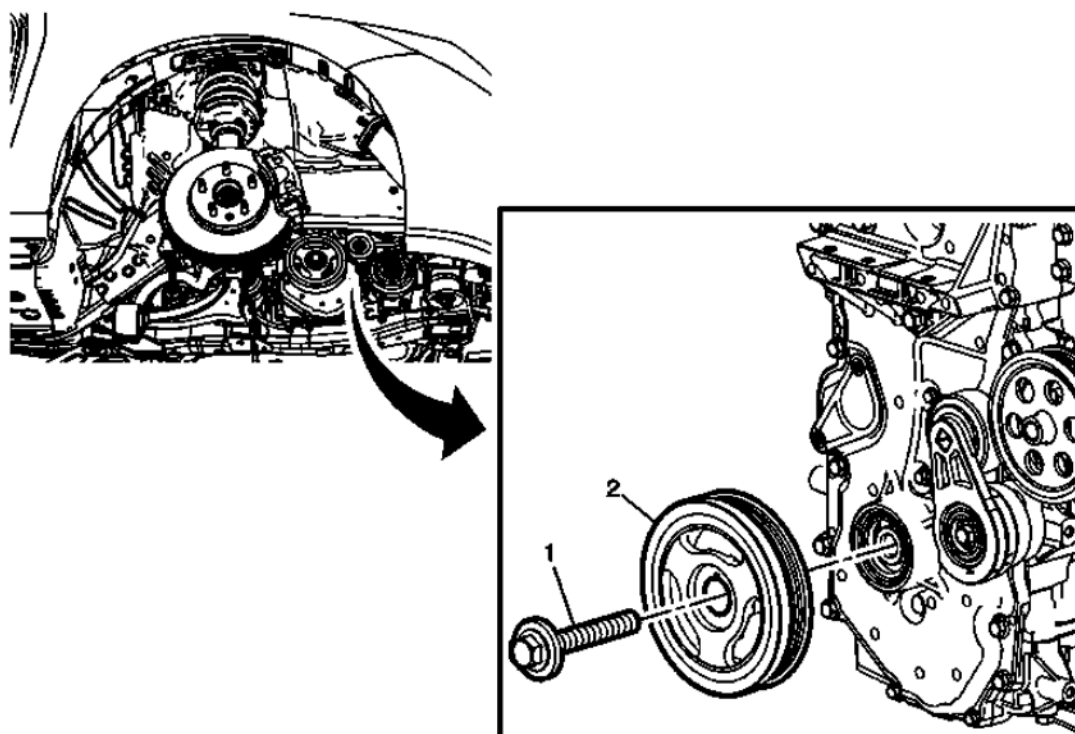
Fig. 58: Crankshaft Balancer Courtesy of GENERAL MOTORS COMPANY
