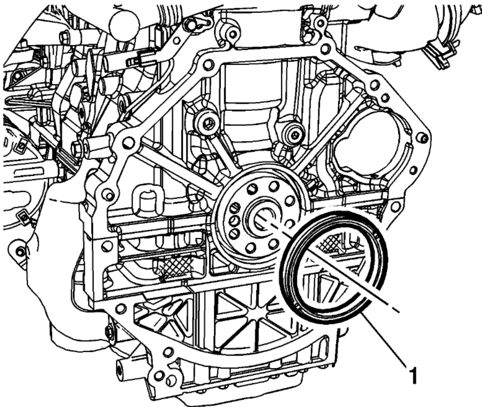
Fig. 220: Crankshaft Rear Oil Seal Courtesy of GENERAL MOTORS COMPANY
