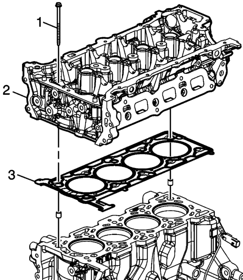
Fig. 200: Cylinder Head Gasket
