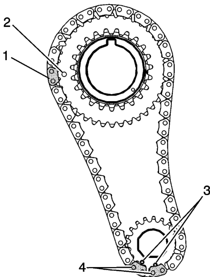
Fig. 63: Timing Link And Timing Mark Courtesy of GENERAL MOTORS COMPANY
