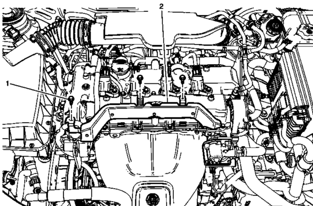
Fig. 192: Camshaft Cover Heat Shield Courtesy of GENERAL MOTORS COMPANY
