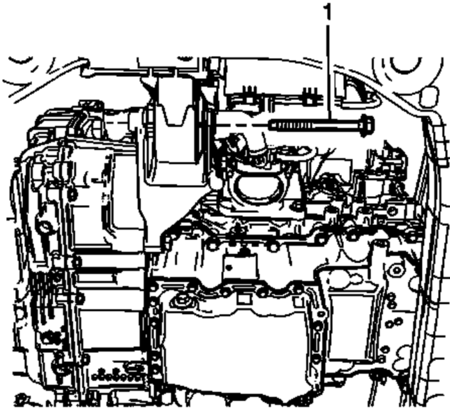
Fig. 14: Rear Transaxle Mount Through Bolt Courtesy of GENERAL MOTORS COMPANY
