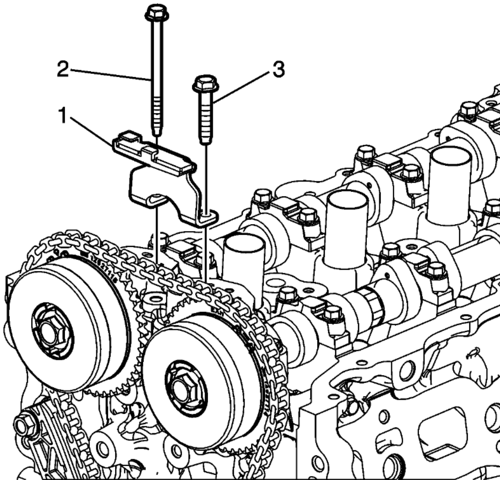
Fig. 94: Upper Timing Chain Guide Bolts Courtesy of GENERAL MOTORS COMPANY
