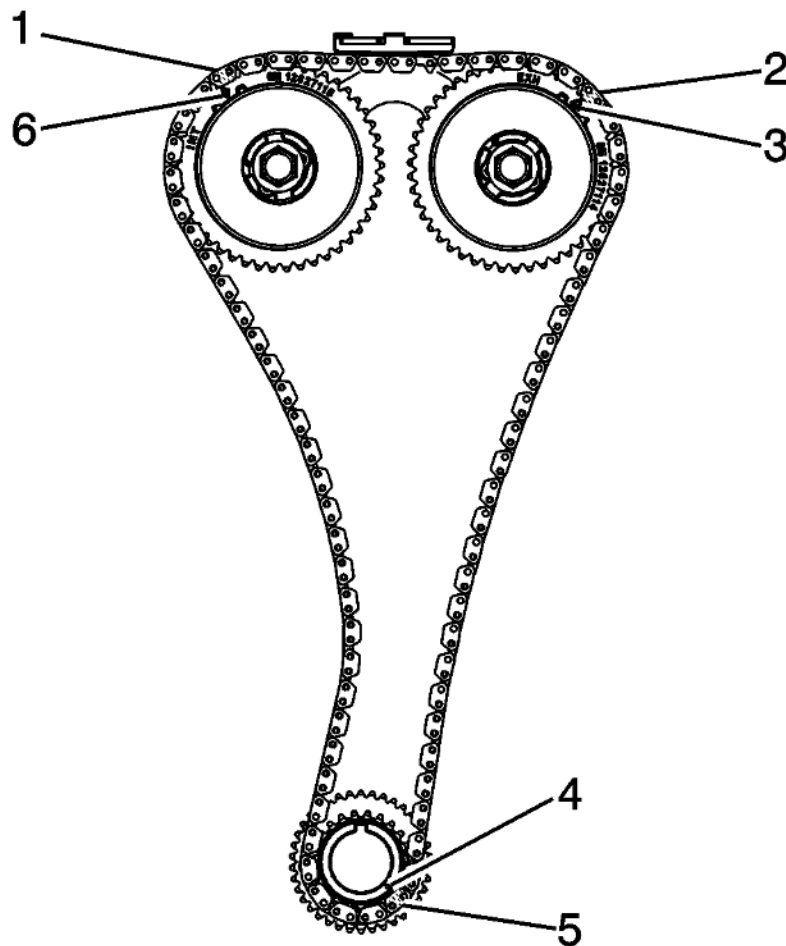
Fig. 106: Timing Chain Oil Nozzle Courtesy of GENERAL MOTORS COMPANY
