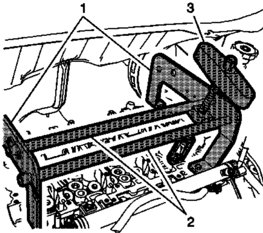
Fig. 193: View Of Valve Spring Compressor Adaptor Set Courtesy of GENERAL MOTORS COMPANY
