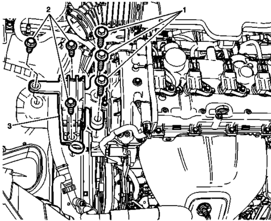
Fig. 16: Engine Mount (LCV)
