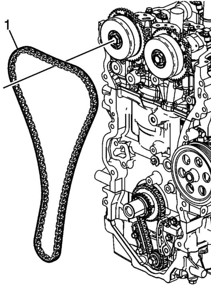
Fig. 98: Timing Chain Courtesy of GENERAL MOTORS COMPANY
