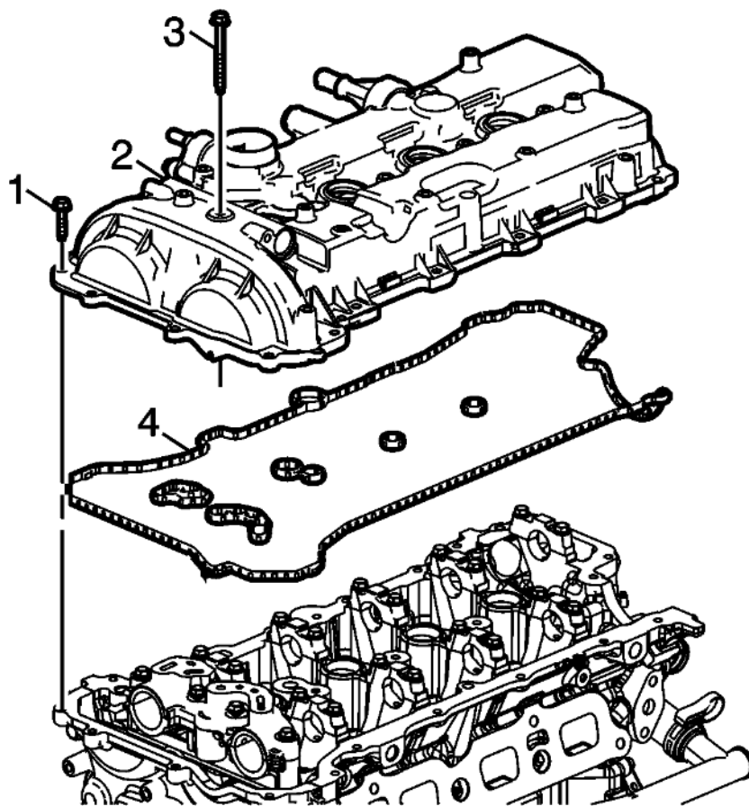
Fig. 138: Camshaft Cover
