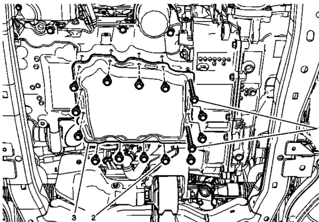
Fig. 208: Oil Pan
