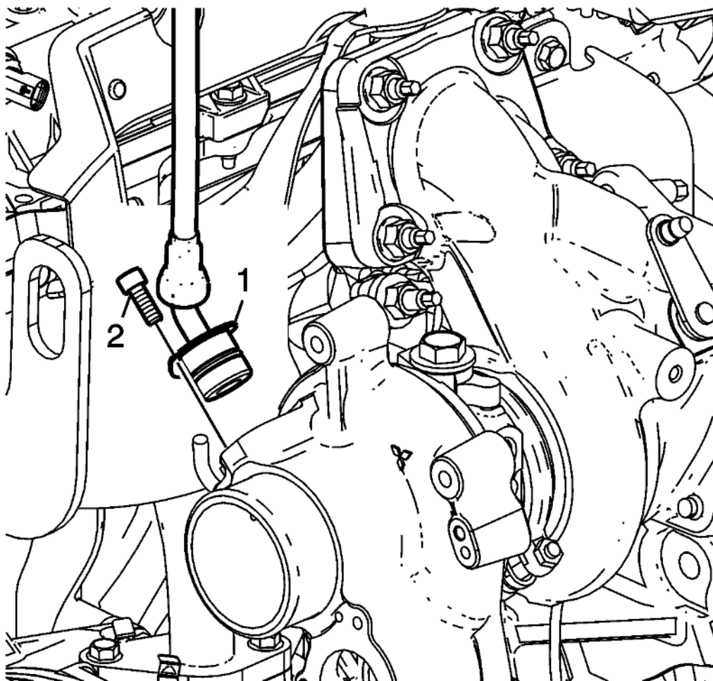
Fig. 134: PCV Hose Fitting Bolt
