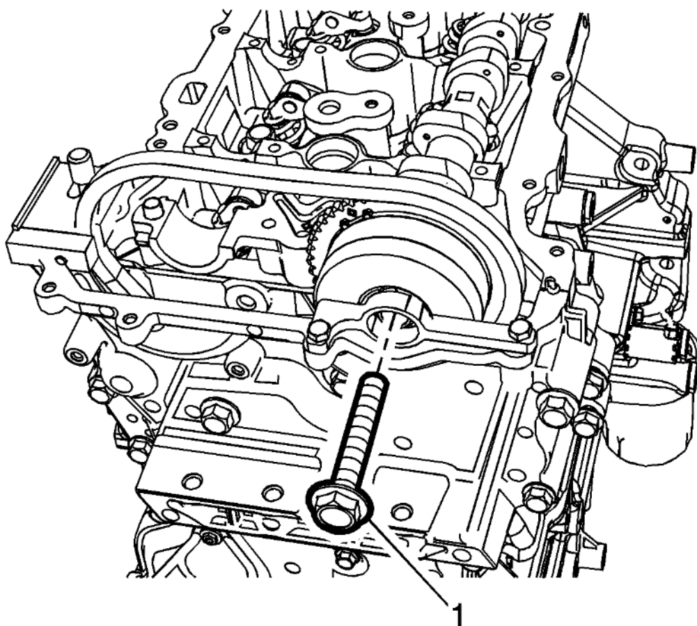
Fig. 167: Camshaft Actuator Bolt Courtesy of GENERAL MOTORS COMPANY
