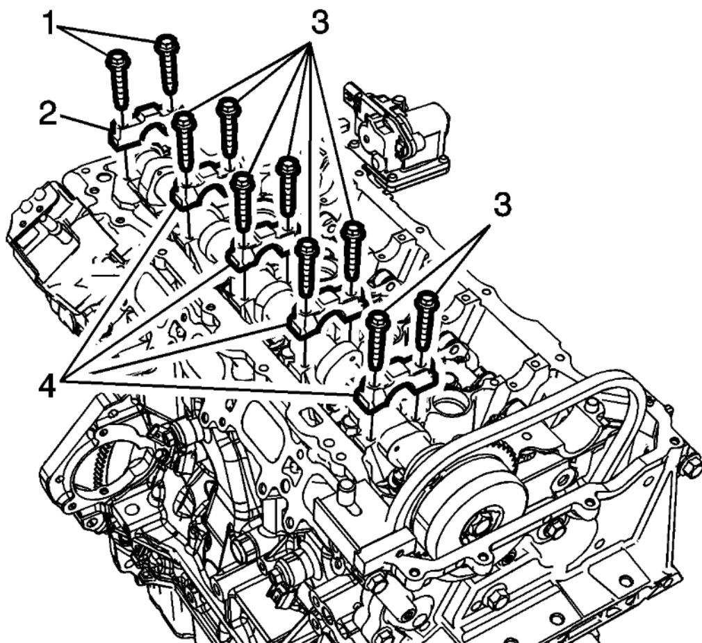
Fig. 168: Intake Camshaft Bearing Rear Cap Bolts And Cap Courtesy of GENERAL MOTORS COMPANY
