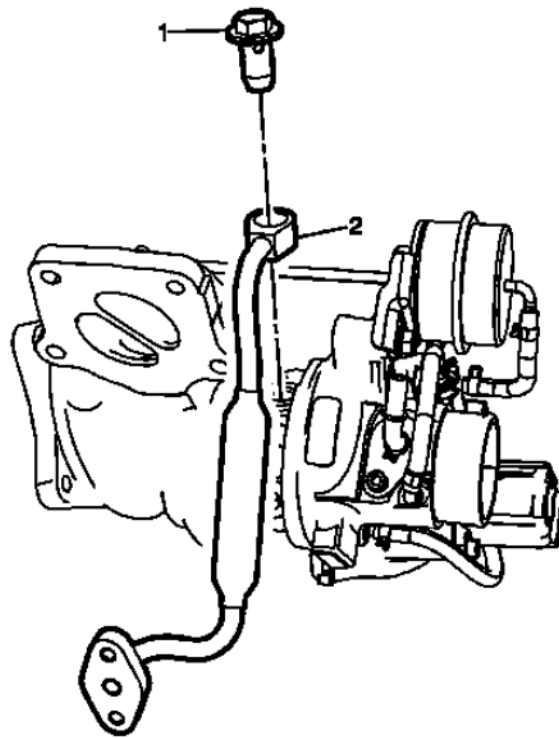
Fig. 30: Turbocharger Oil Feed Pipe Courtesy of GENERAL MOTORS COMPANY
