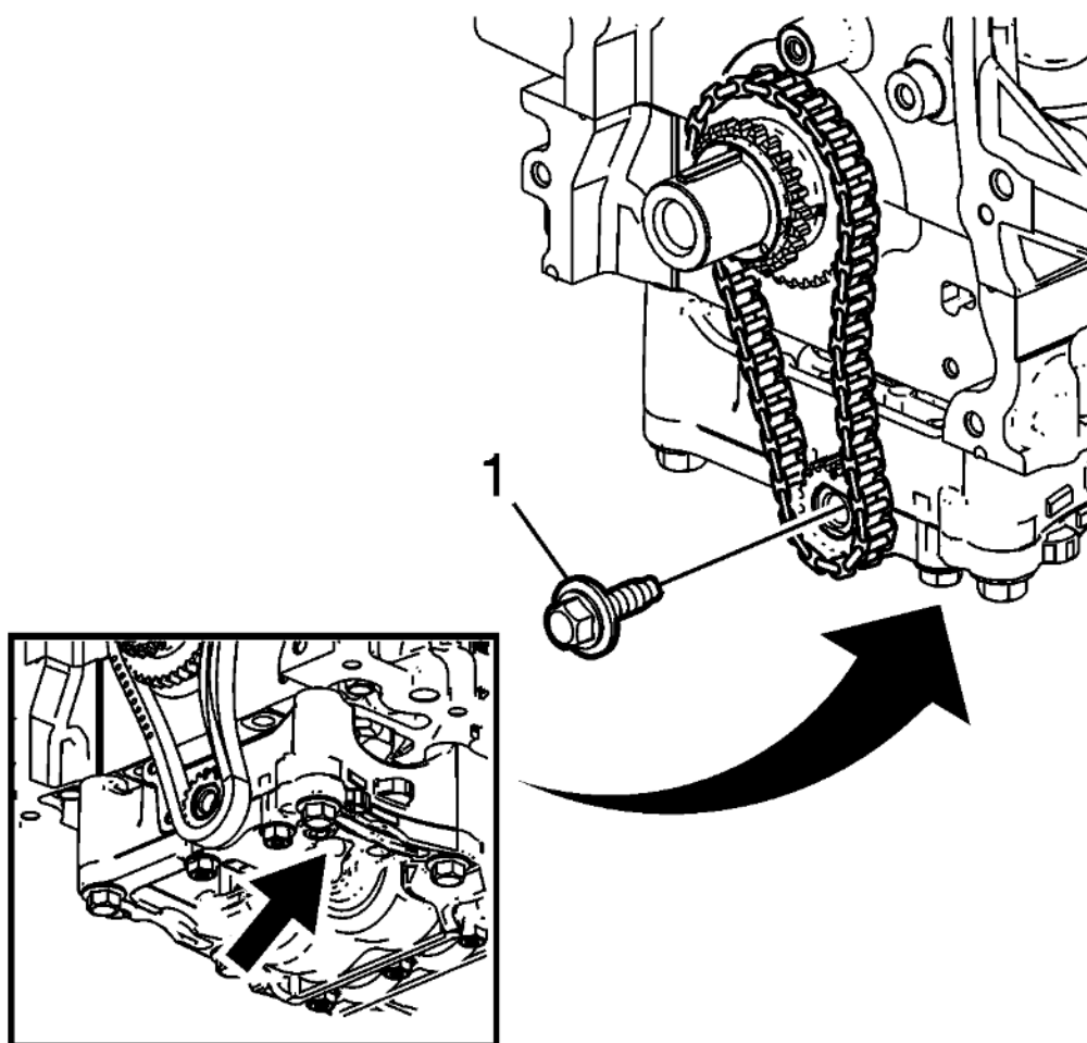
Fig. 61: Balancer Shaft Driven Sprocket Bolt Courtesy of GENERAL MOTORS COMPANY
