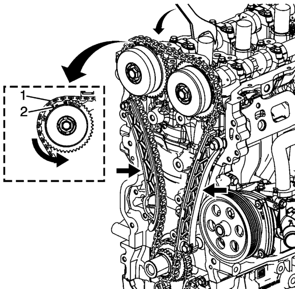
Fig. 104: Timing Mark On Intake Actuator Courtesy of GENERAL MOTORS COMPANY
