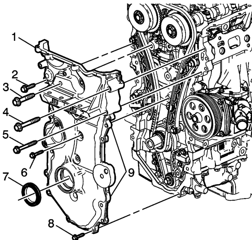
Fig. 81: Front Oil Seal Courtesy of GENERAL MOTORS COMPANY
