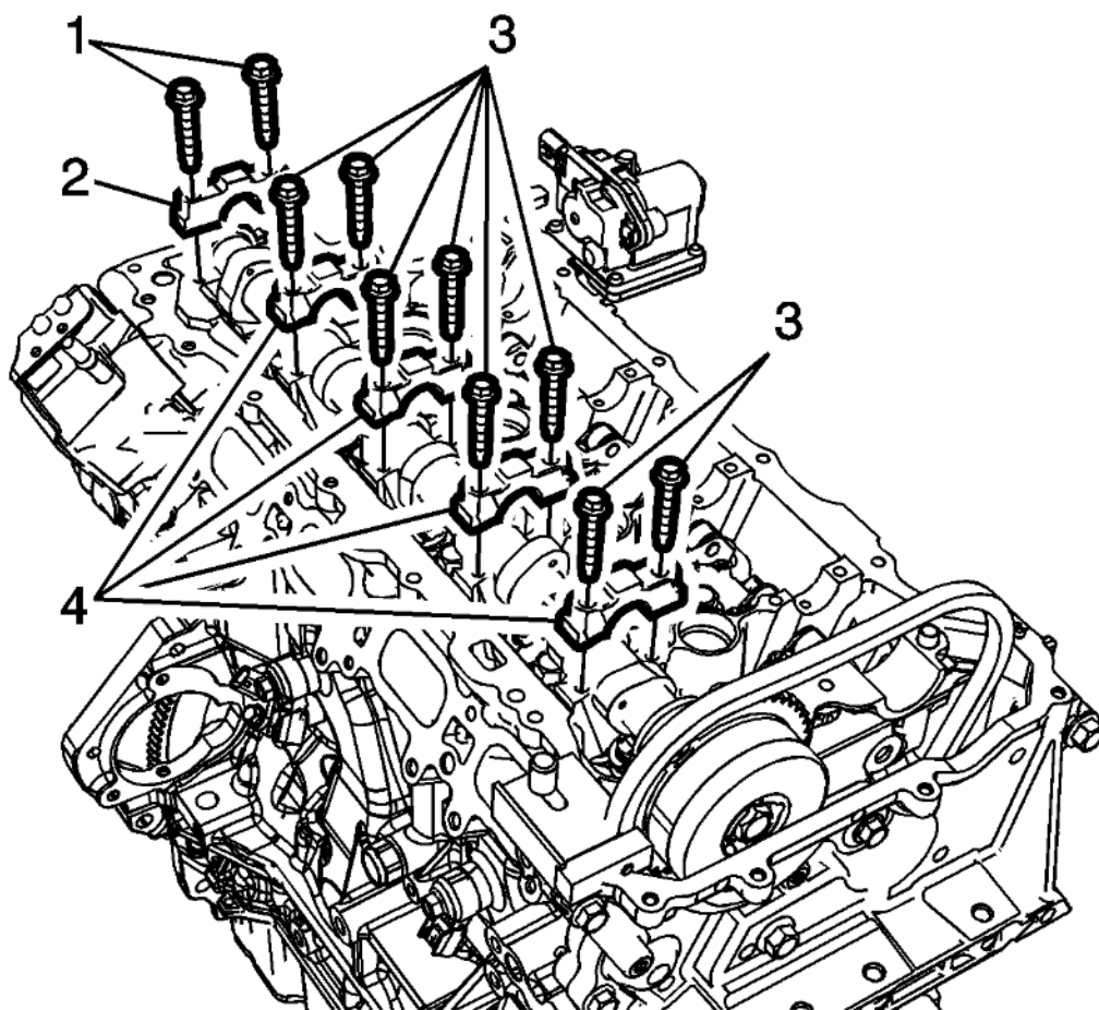
Fig. 160: Intake Camshaft Bearing Rear Cap Bolts And Cap Courtesy of GENERAL MOTORS COMPANY
