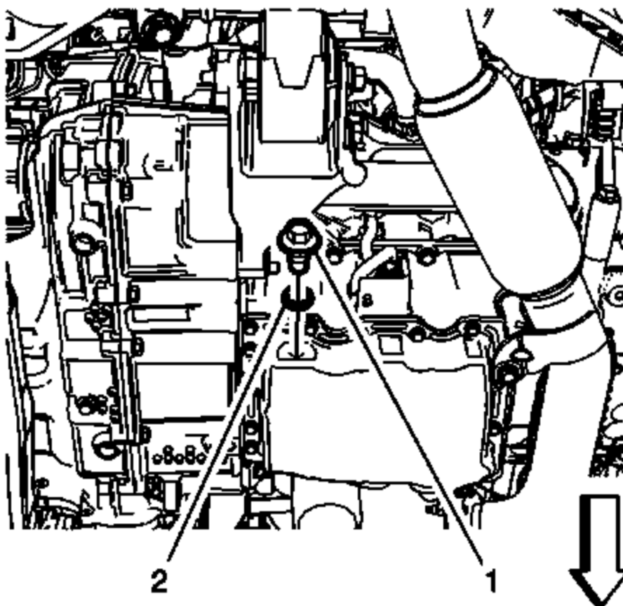
Fig. 262: Oil Pan Drain Plug
