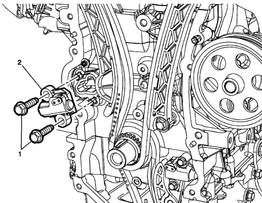
Fig. 148: Timing Chain Tensioner Bolts And Timing Chain Tensioner Courtesy of GENERAL MOTORS COMPANY
