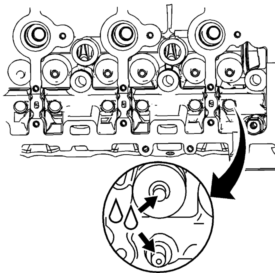
Fig. 92: Valve Tips
