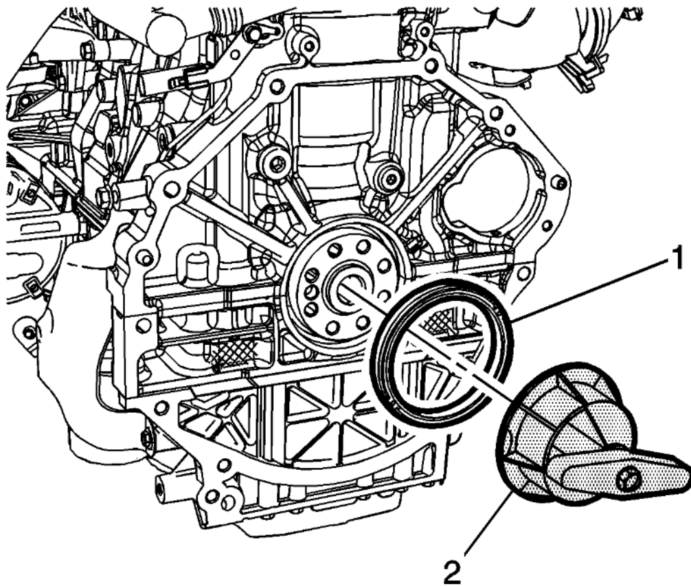
Fig. 221: Crankshaft Real Oil Seal Courtesy of GENERAL MOTORS COMPANY
