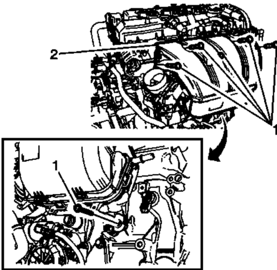
Fig. 39: Intake Bolts
