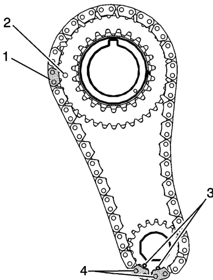
Fig. 109: Timing Link And Timing Mark Courtesy of GENERAL MOTORS COMPANY
