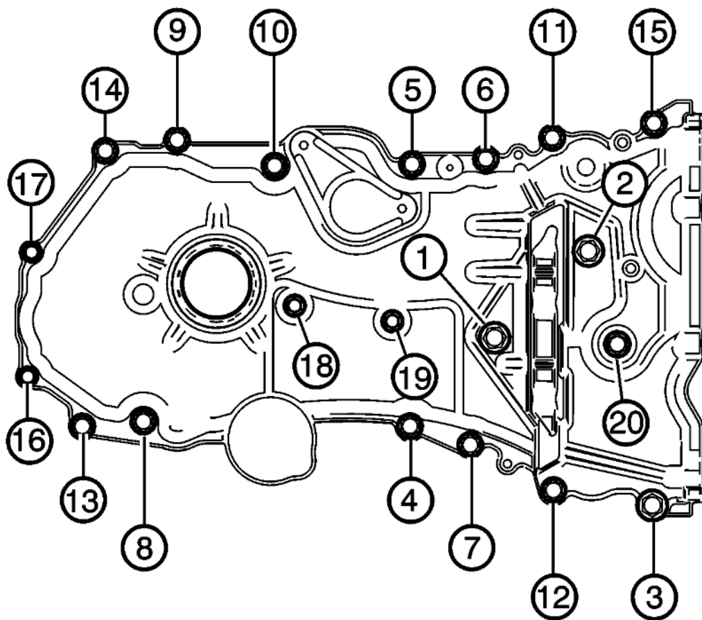
Fig. 76: Engine Front Cover
