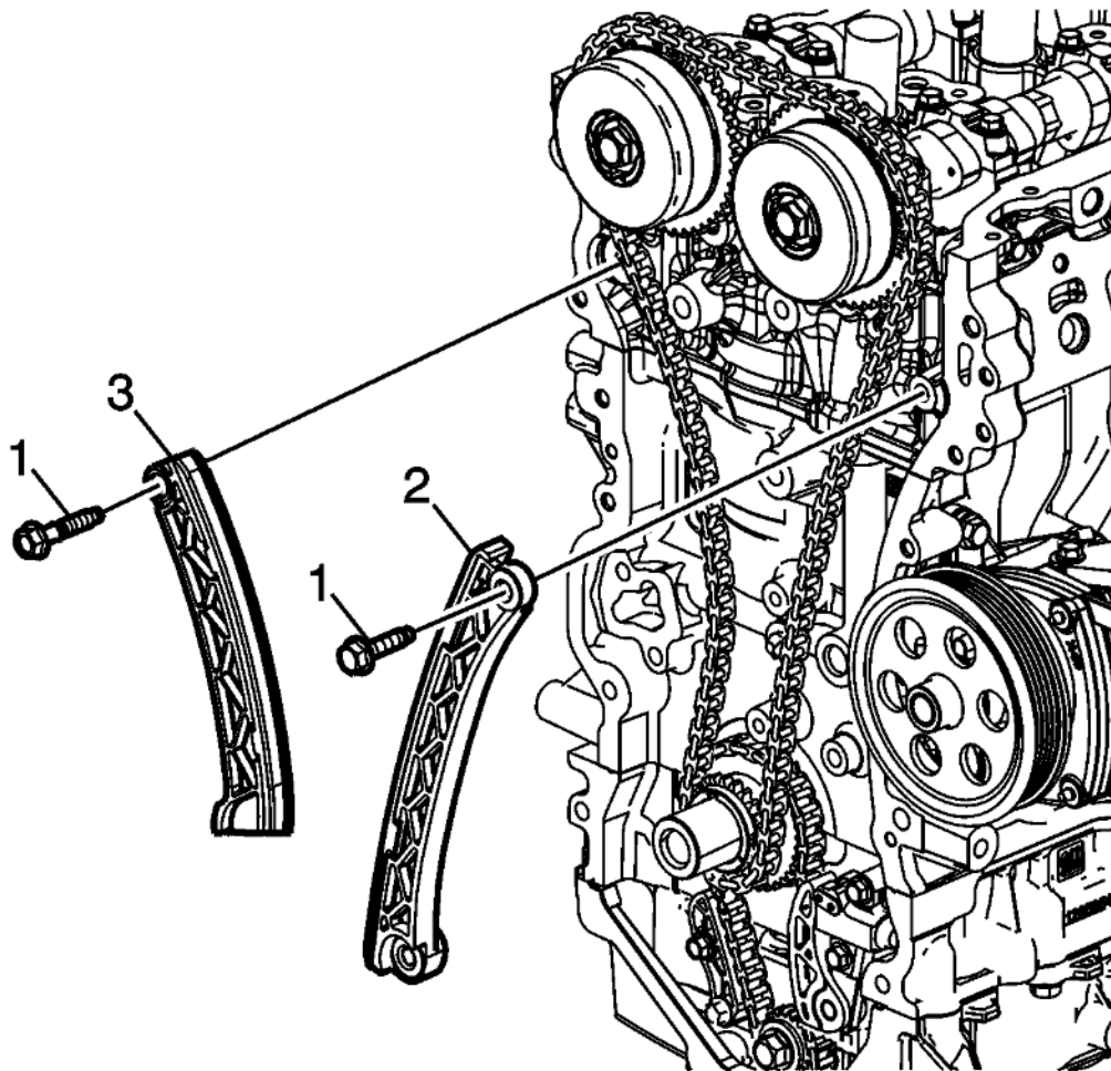
Fig. 102: Timing Chain Guide And Pivot Arm Bolt Courtesy of GENERAL MOTORS COMPANY
