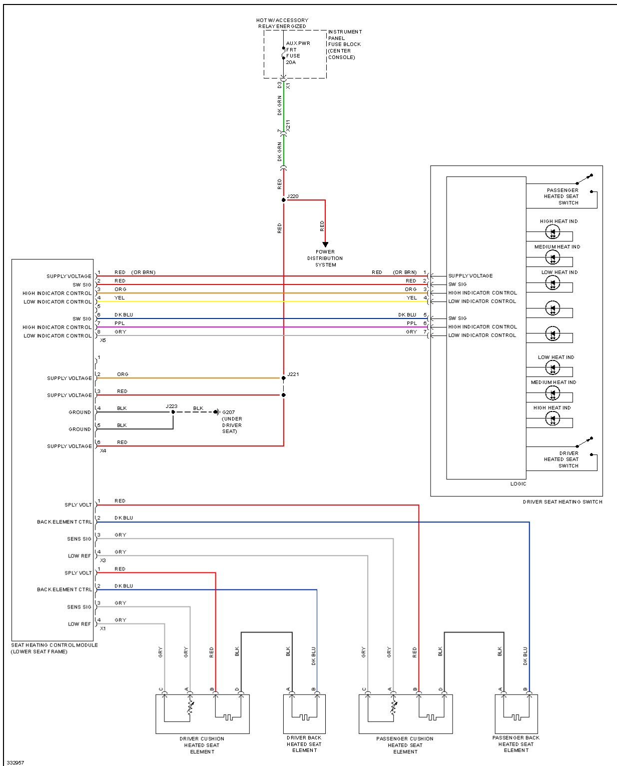
Fig. 59: Heated Seats Circuit, W/ SPO Heated Seats
