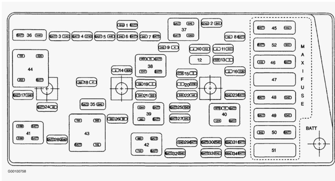
Fig. 1: Identifying Instrument Panel Electrical Center Components Courtesy of GENERAL MOTORS CORP.
