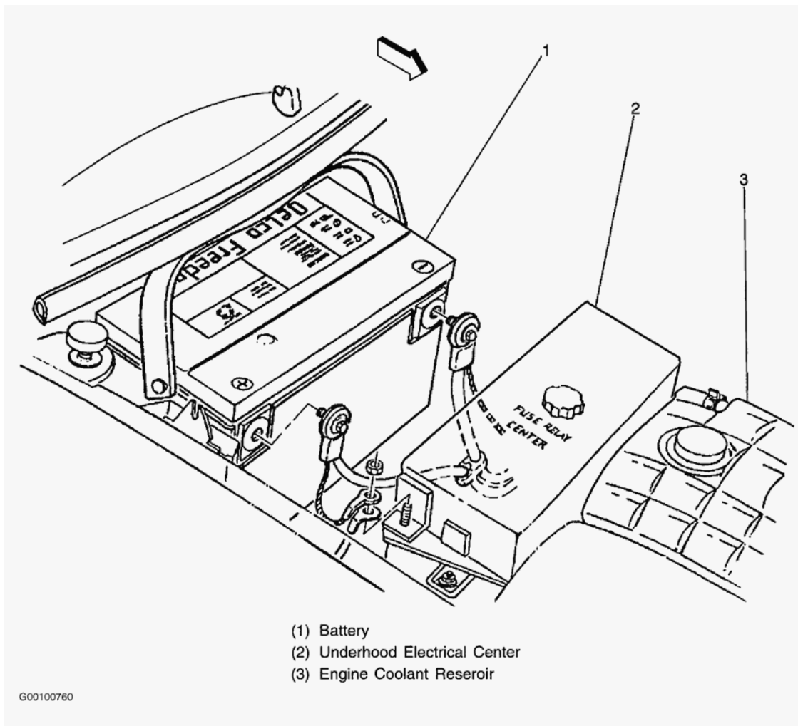
Fig. 3: Locating Underhood Electrical Center Courtesy of GENERAL MOTORS CORP.
