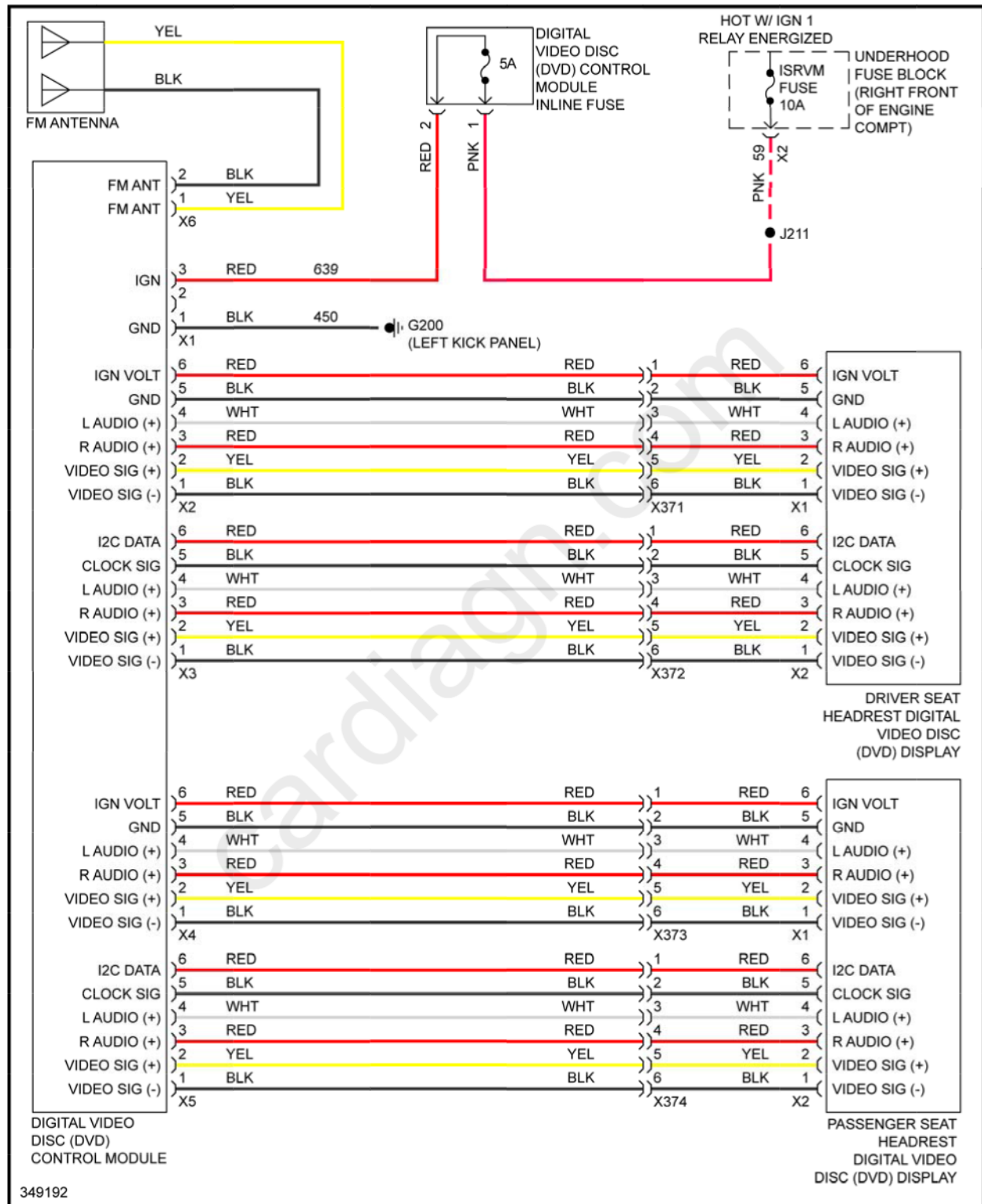
Fig. 107: Video System Circuit
