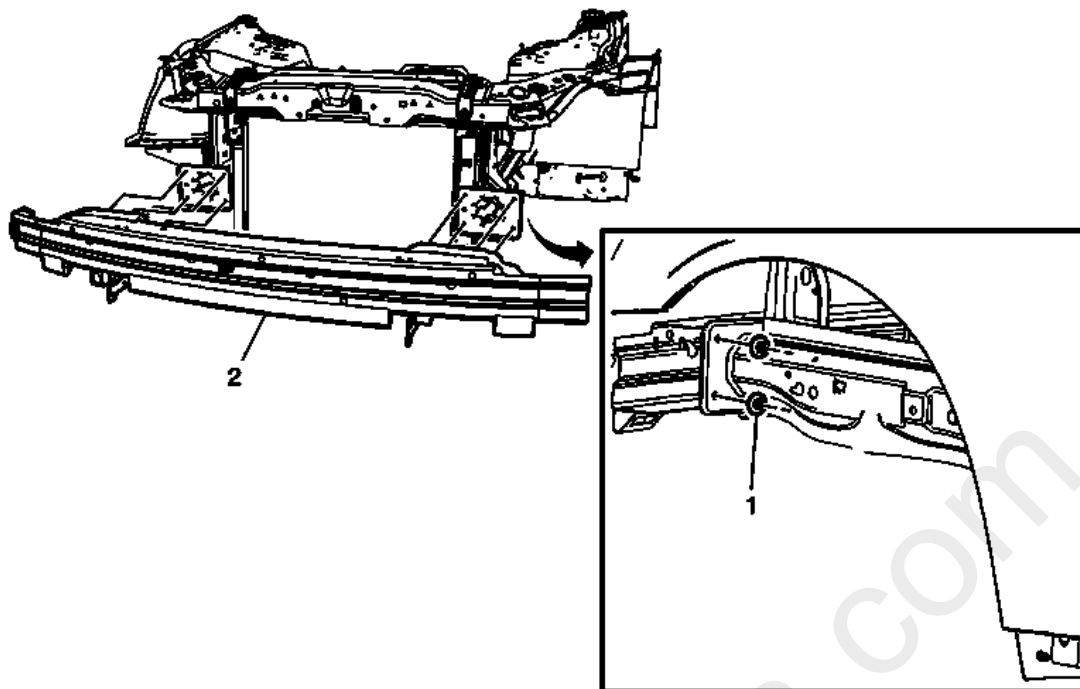
Fig. 3: View of Front Bumper Impact Bar Assembly Courtesy of GENERAL MOTORS COMPANY
