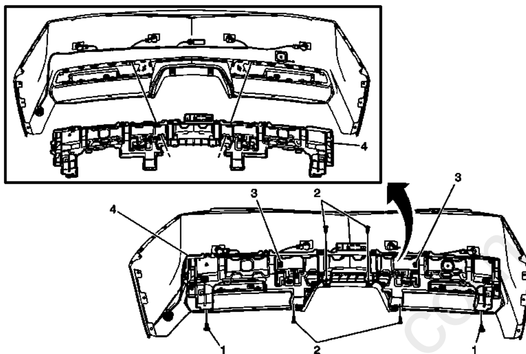
Fig. 15: Rear Bumper Fascia Energy Absorber (Coupe) Courtesy of GENERAL MOTORS COMPANY
