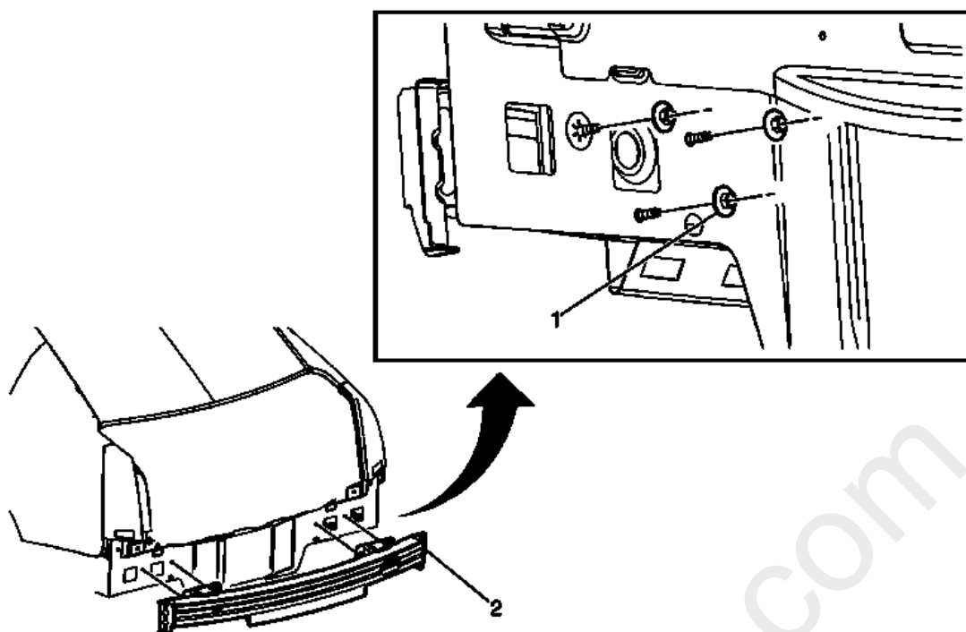
Fig. 18: Identifying Rear Bumper Impact Bar Courtesy of GENERAL MOTORS COMPANY
