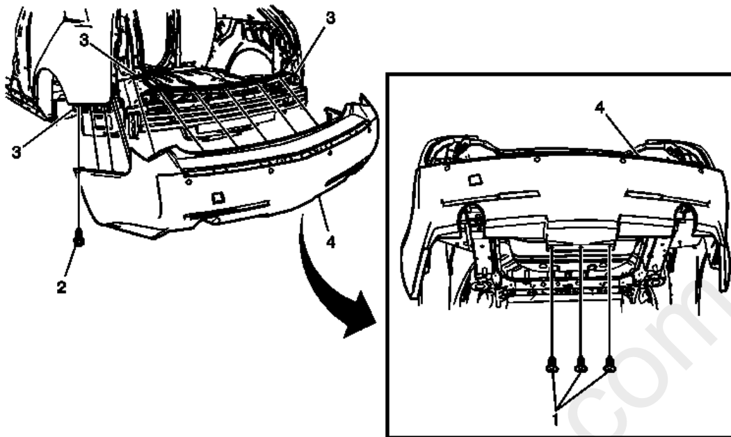
Fig. 9: Rear Bumper Fascia Components (Wagon)
