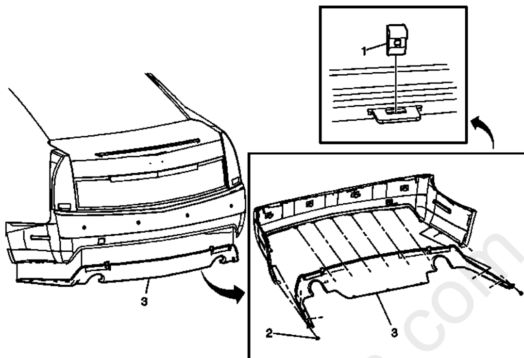
Fig. 22: View of Fascia Insert Assembly Rear Bumper Courtesy of GENERAL MOTORS COMPANY
