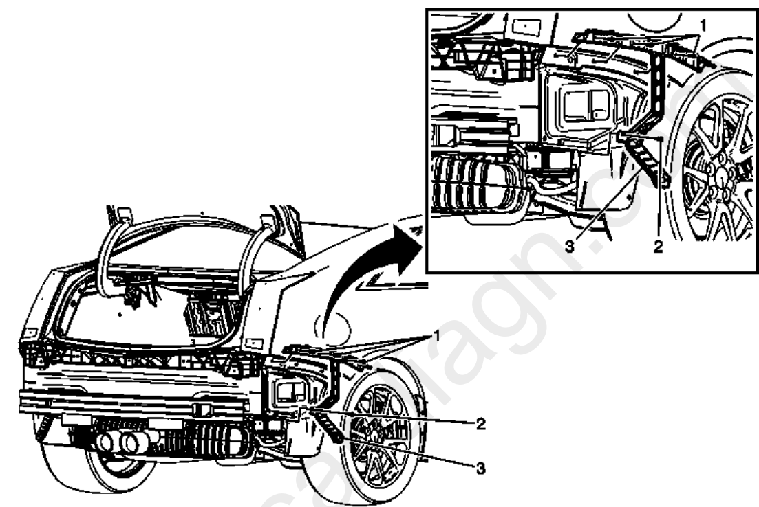
Fig. 11: Rear Bumper Fascia Bracket - Side (Coupe) Courtesy of GENERAL MOTORS COMPANY
