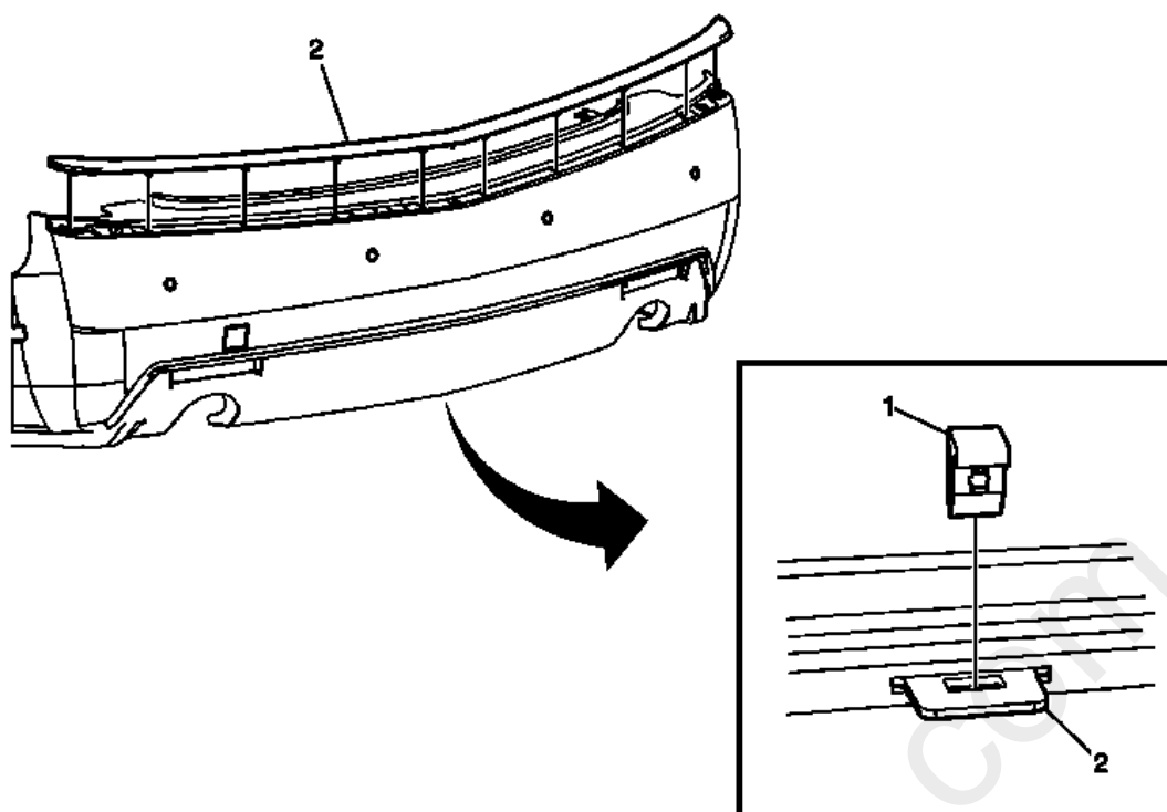
Fig. 8: View of Rear Bumper Fascia Molding Assembly Courtesy of GENERAL MOTORS COMPANY
