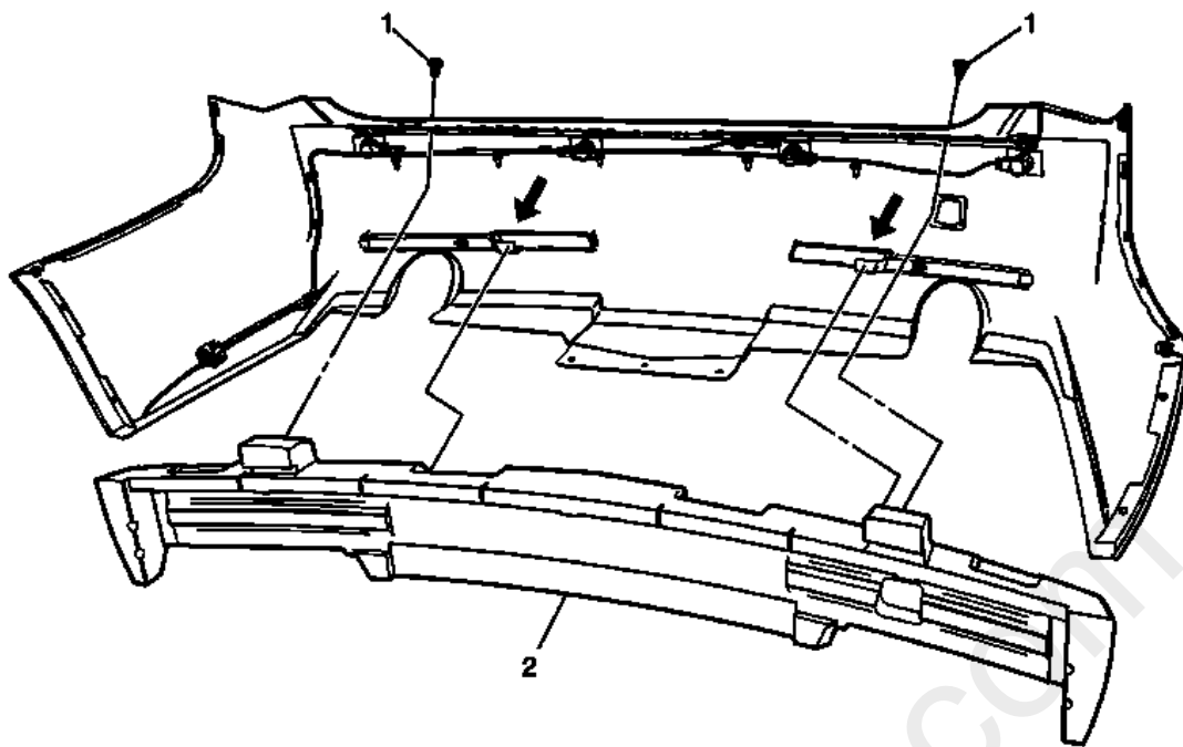
Fig. 16: Rear Bumper Fascia Energy Absorber & Retainers (Wagon) Courtesy of GENERAL MOTORS COMPANY
