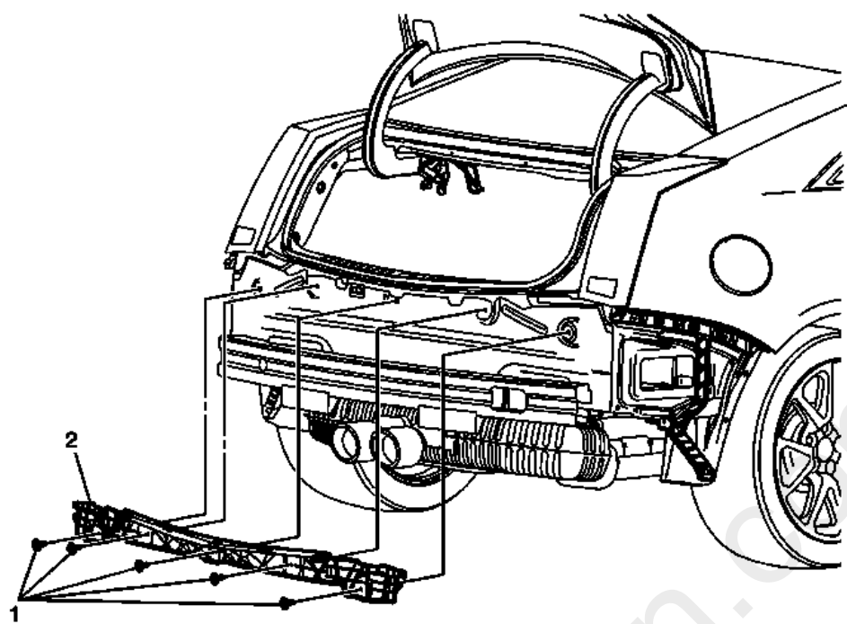
Fig. 13: Rear Bumper Fascia Center Support (Coupe) Courtesy of GENERAL MOTORS COMPANY
