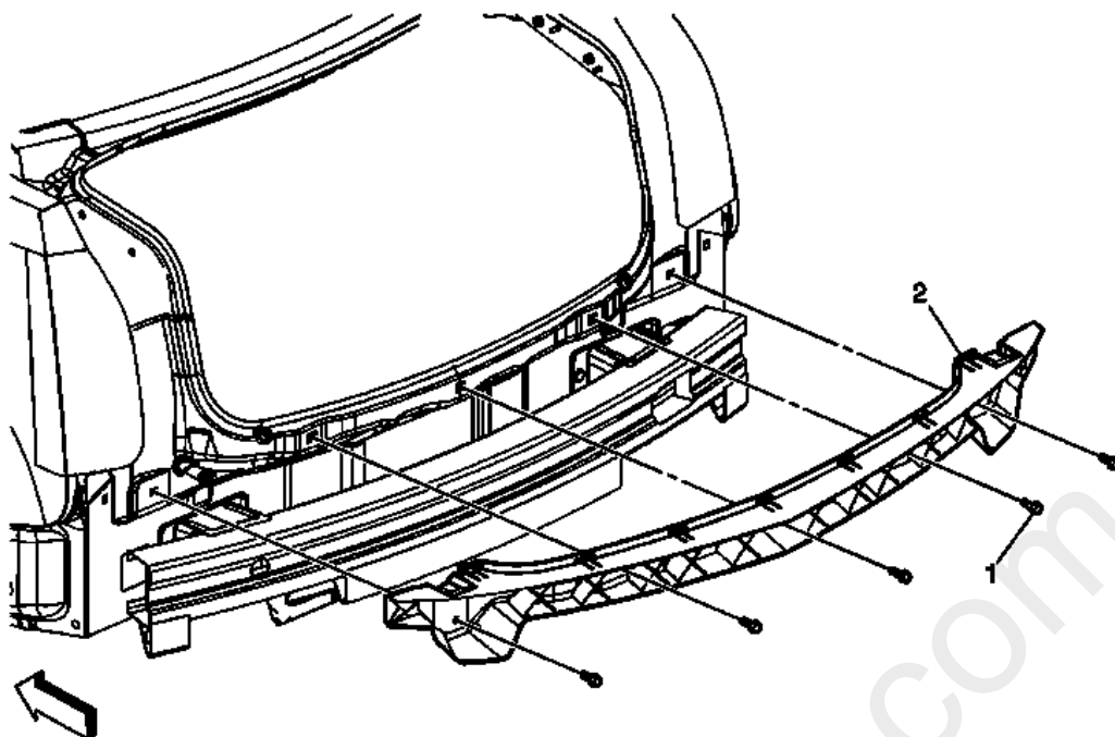
Fig. 14: View of Fascia Support Assembly Rear Bumper Courtesy of GENERAL MOTORS COMPANY
