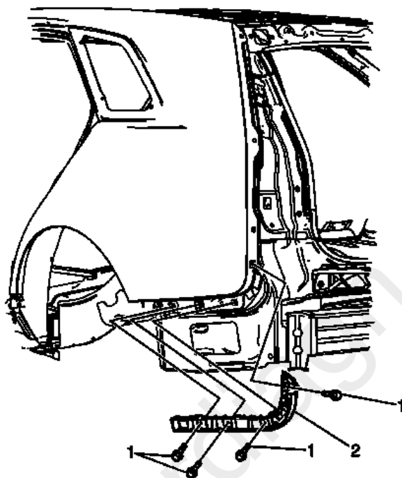
Fig. 12: Rear Bumper Fascia Bracket - Side (Wagon) Courtesy of GENERAL MOTORS COMPANY
