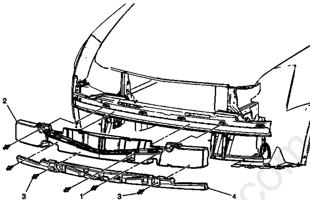
Fig. 1: View of Front Bumper Assembly Courtesy of GENERAL MOTORS COMPANY
