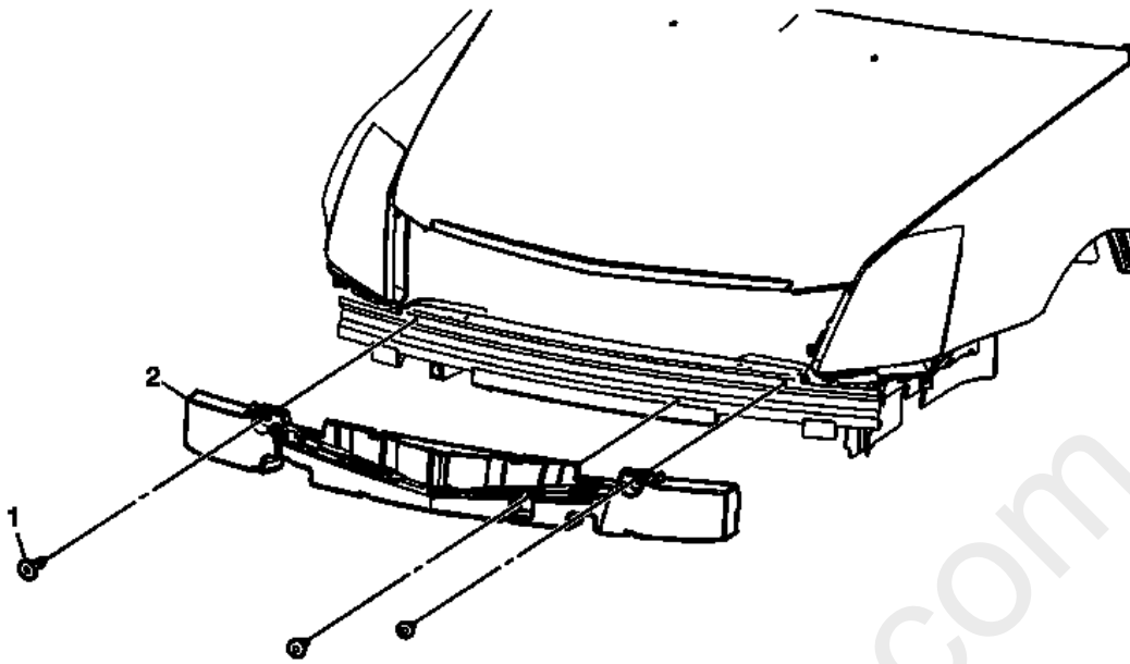
Fig. 2: Identifying Front Bumper Fascia Energy Absorber (Standard) Courtesy of GENERAL MOTORS COMPANY
