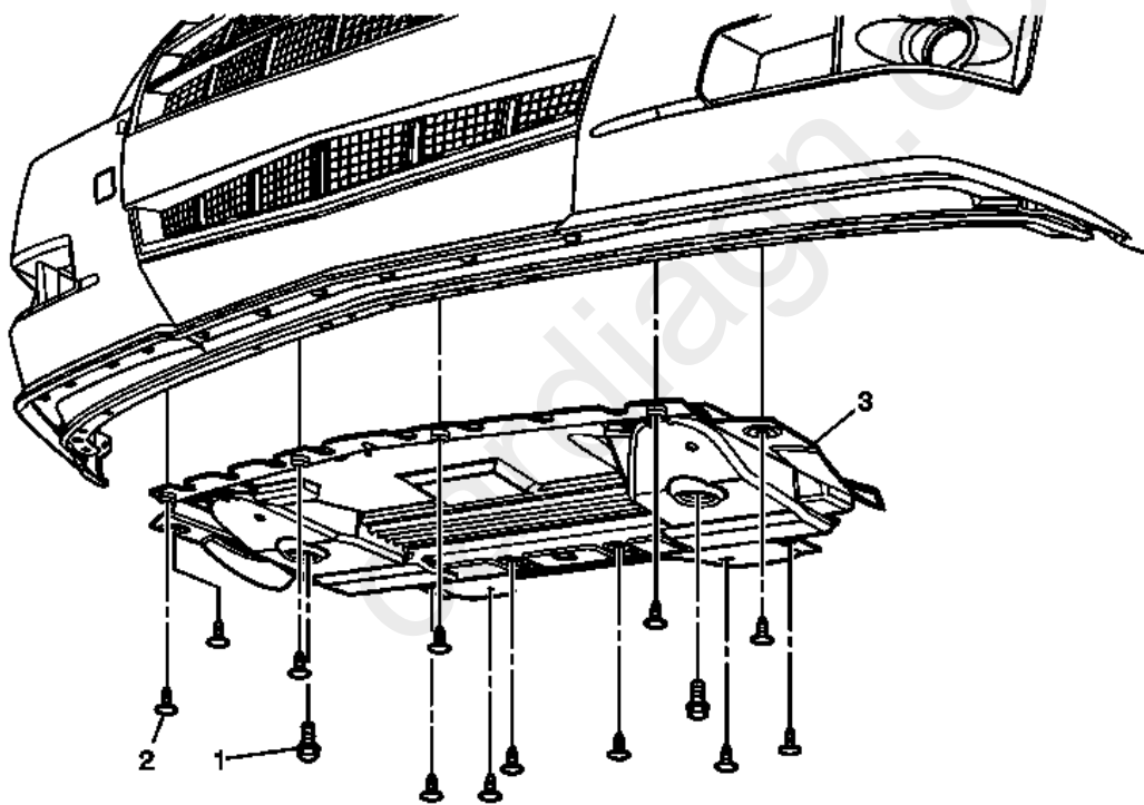
Fig. 6: Identifying Front Air Deflector Courtesy of GENERAL MOTORS COMPANY
