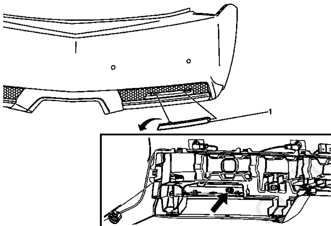
Fig. 19: Rear Bumper Fascia Reflector (Coupe) Courtesy of GENERAL MOTORS COMPANY
