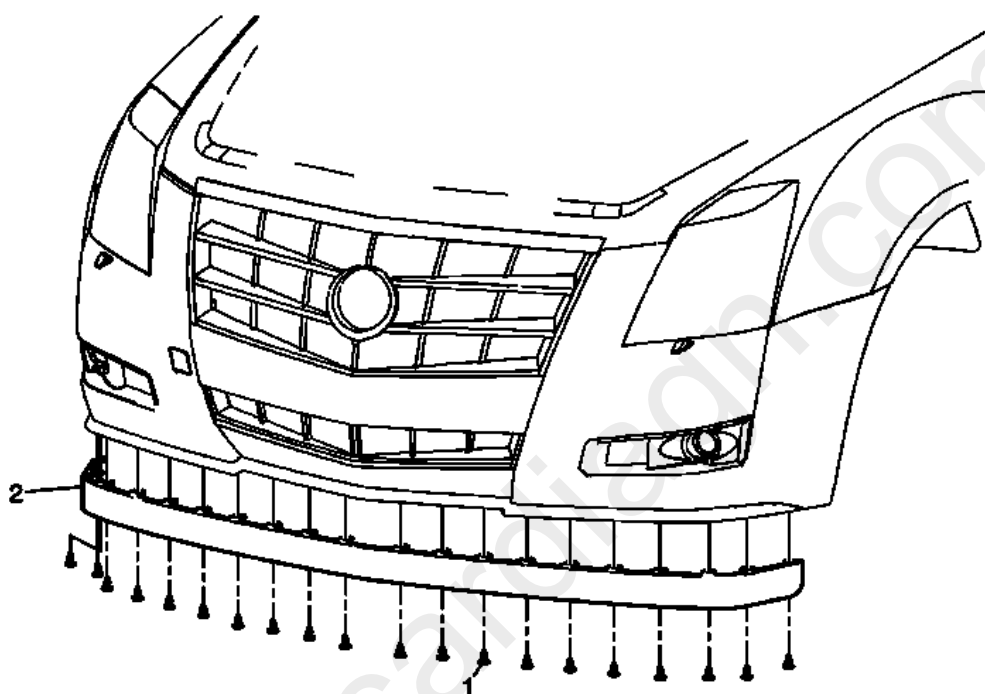
Fig. 7: View of Fascia Air Deflector Assembly Courtesy of GENERAL MOTORS COMPANY
