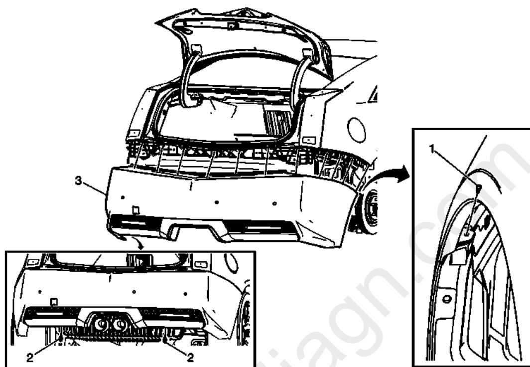
Fig. 10: Rear Bumper Fascia Components (Coupe)
