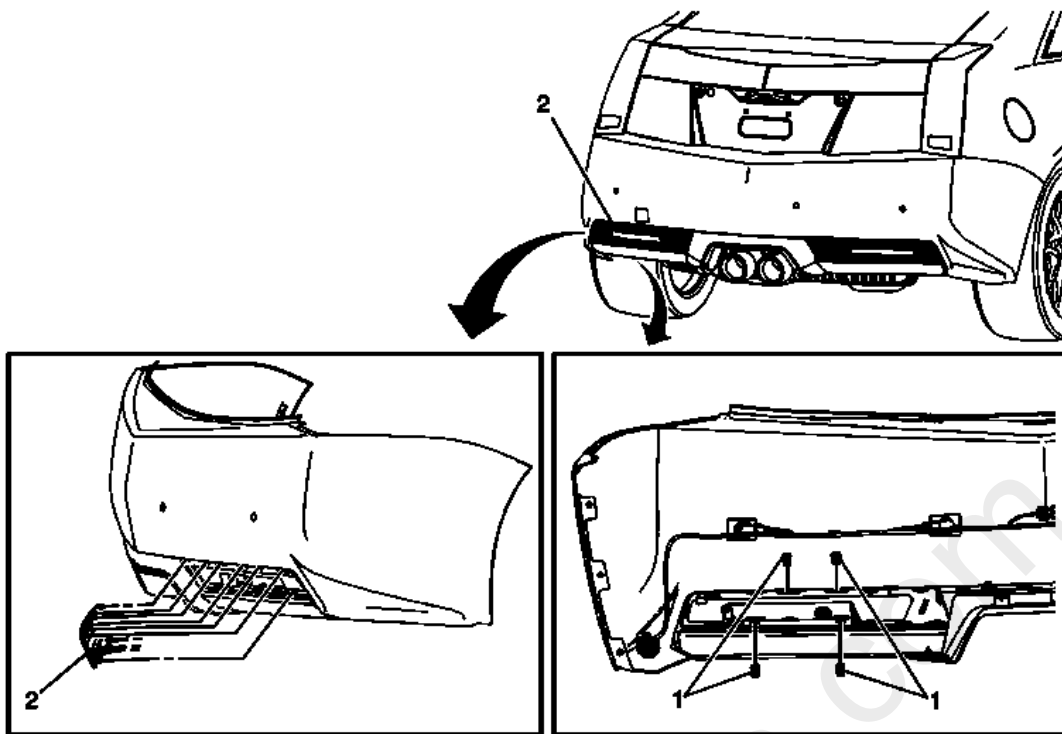
Fig. 21: Rear Bumper Fascia Insert & Clips (Coupe) Courtesy of GENERAL MOTORS COMPANY
