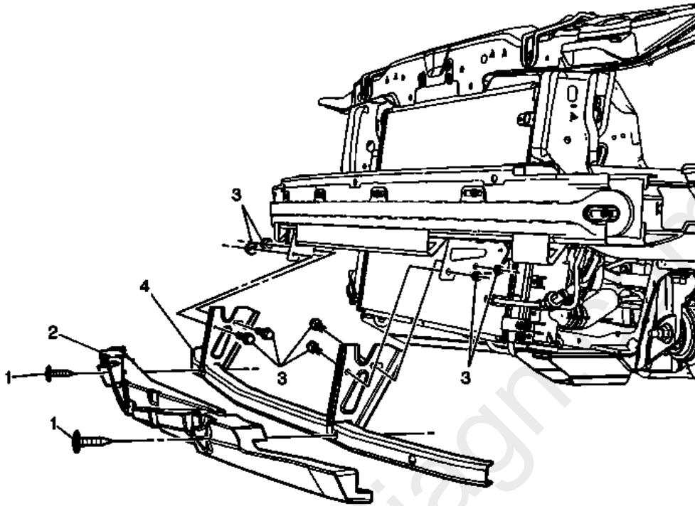
Fig. 4: Identifying Front Bumper Impact Bar Extension Courtesy of GENERAL MOTORS COMPANY
