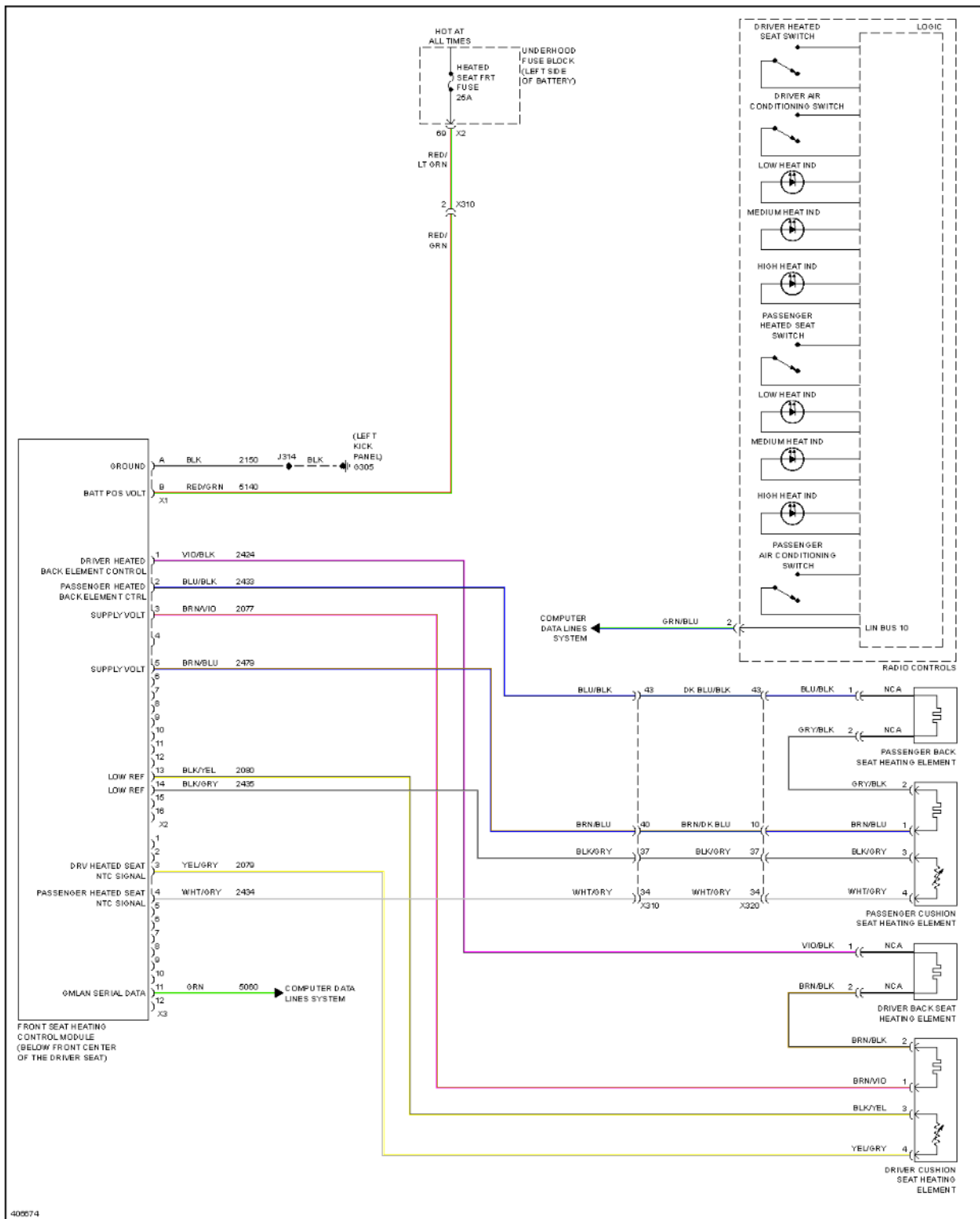
Fig. 106: Heated Seats Circuit, W/O Memory
