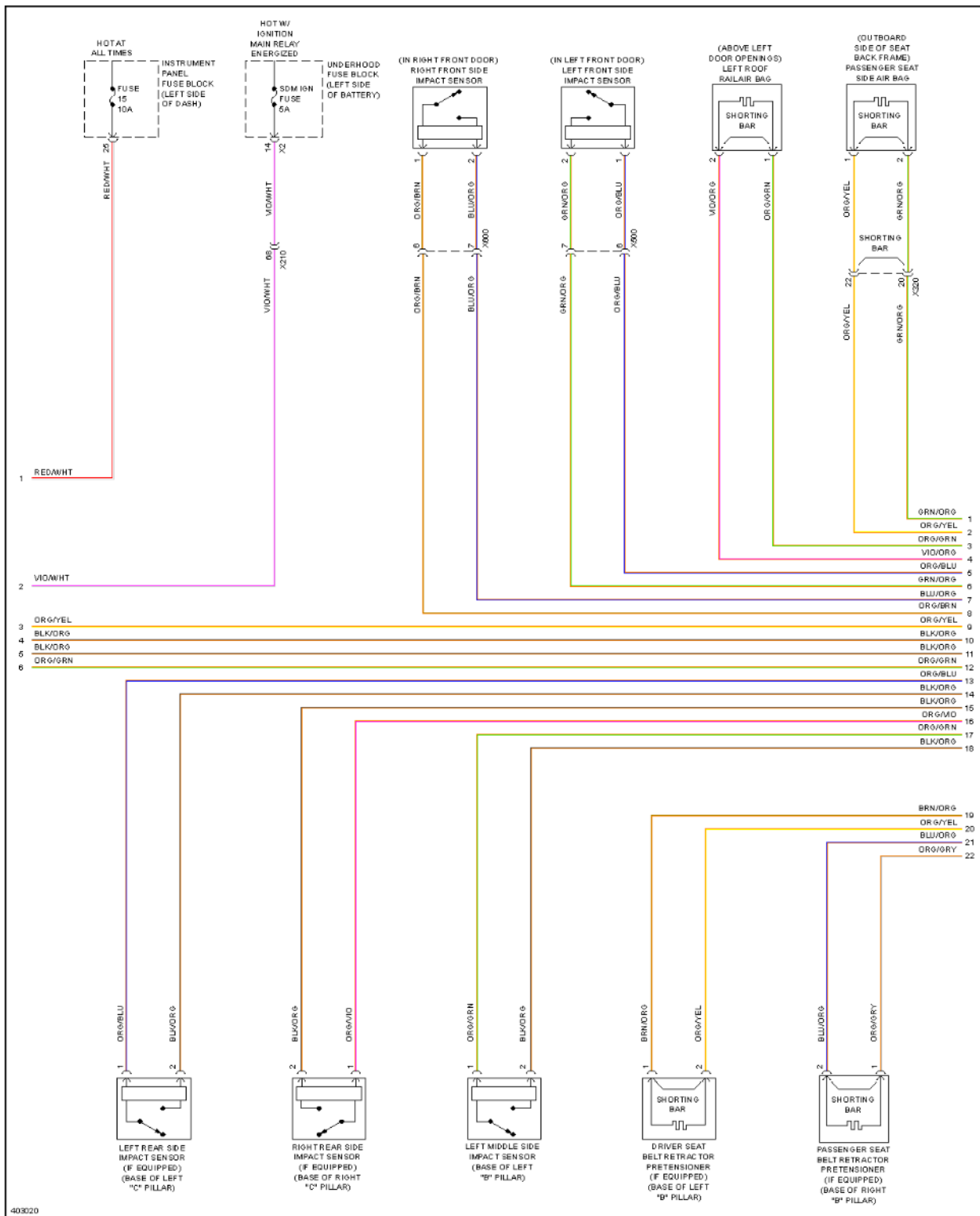
Fig. 128: Supplemental Restraints Circuit (2 of 3)
