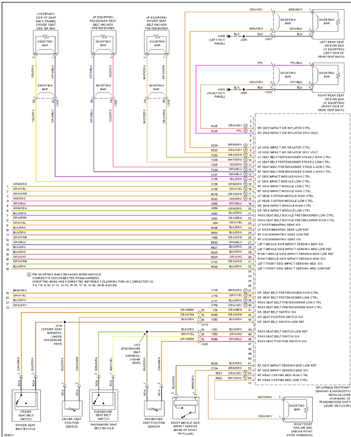
Fig. 129: Supplemental Restraints Circuit (3 of 3)
