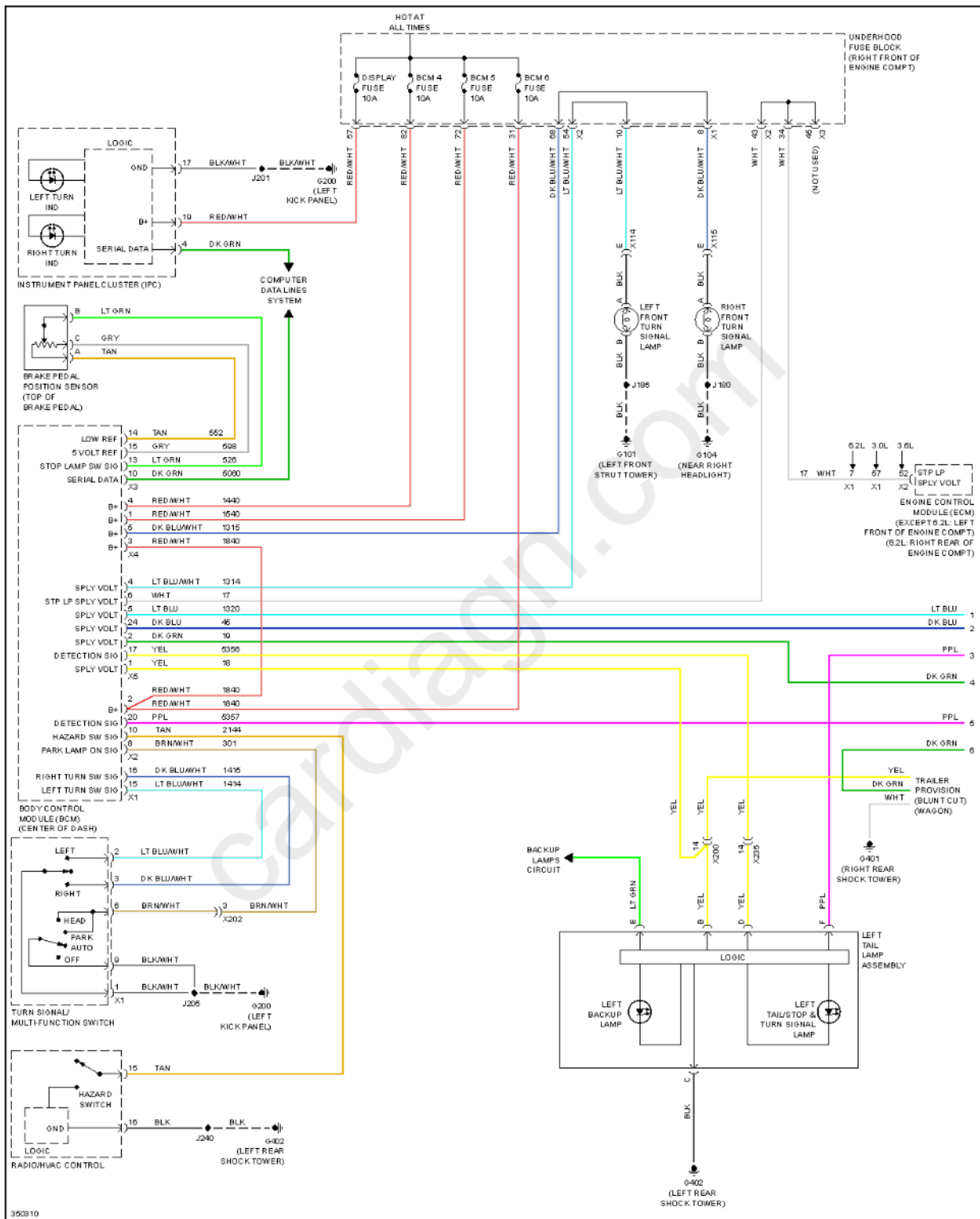
Fig. 43: Exterior Lamps Circuit (1 of 2)
