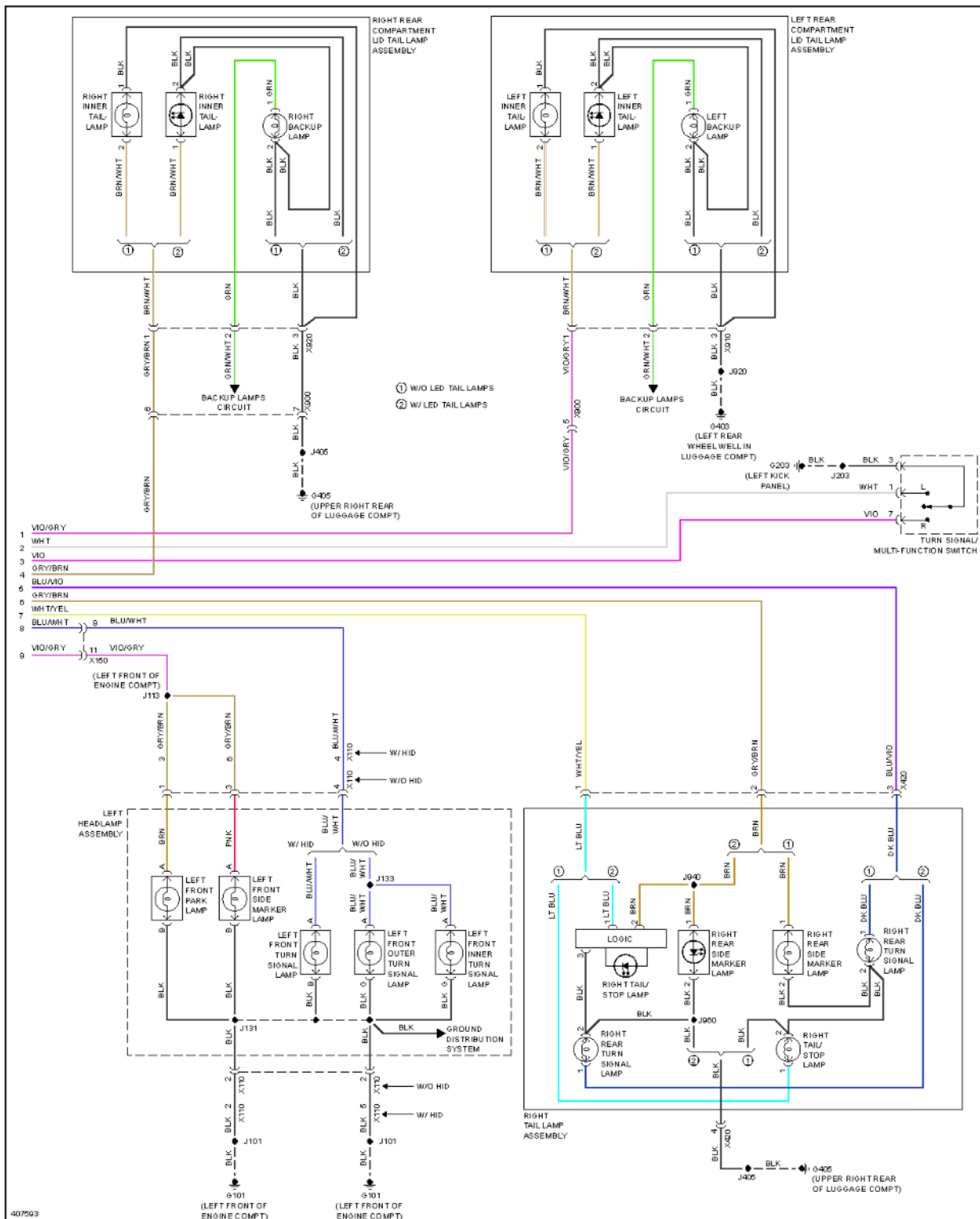
Fig. 54: Exterior Lamps Circuit (3 of 3)
