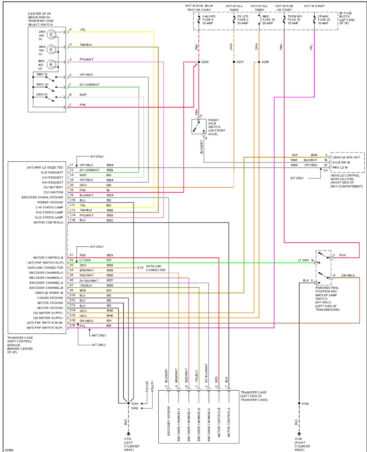
Fig. 38: Transfer Case Circuit
