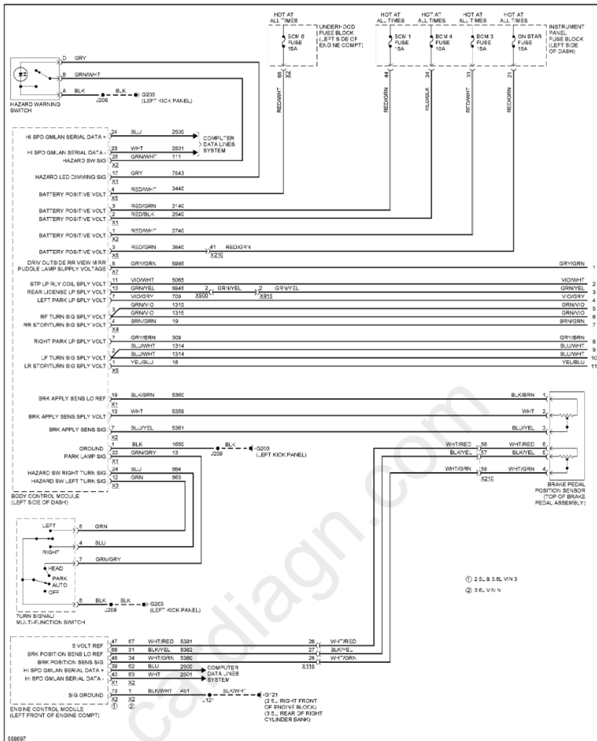
Fig. 48: Exterior Lamps Circuit (1 of 3)
