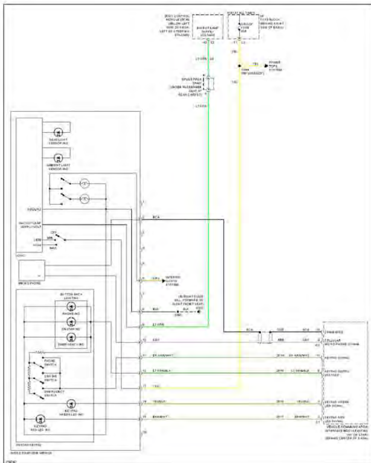
Fig. 49: Electrochromic Mirror Circuit
