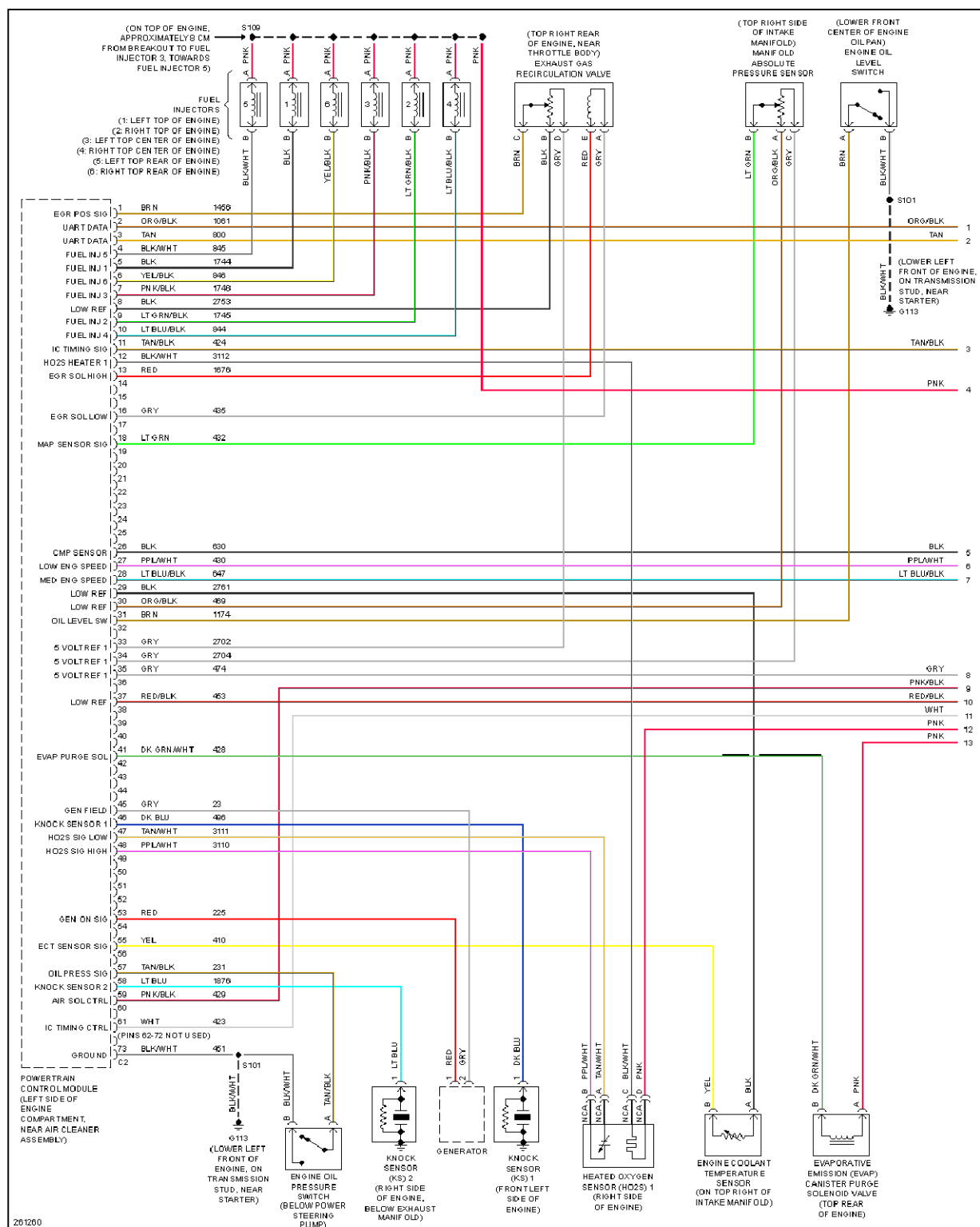
Fig. 24: 3.8L VIN 2, Engine Performance Circuit (1 of 5)
