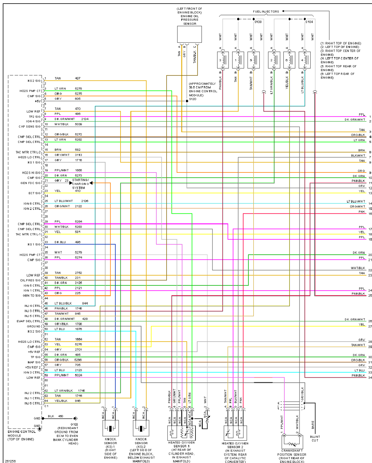
Fig. 20: 3.6L VIN 7, Engine Performance Circuit (1 of 4)
