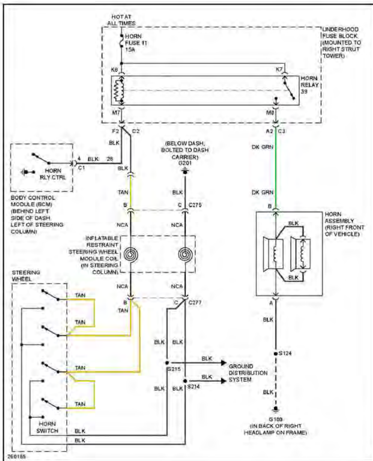
Fig. 36: Horn Circuit
