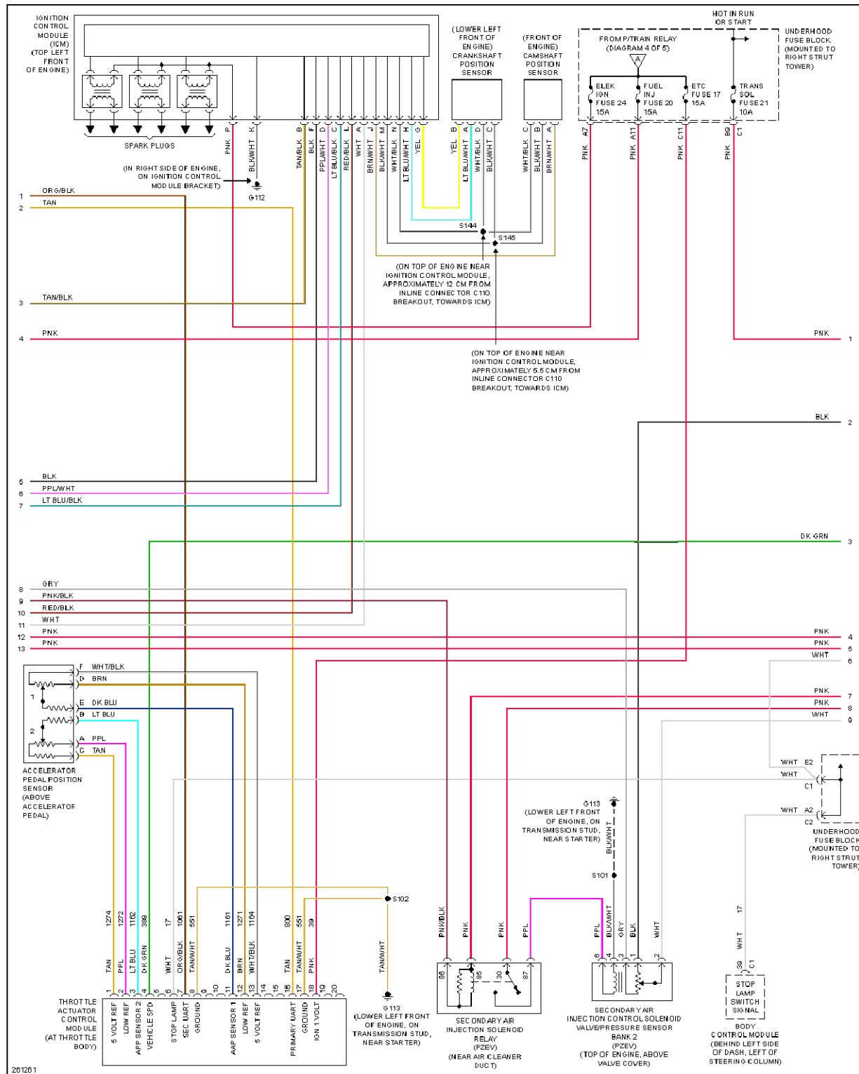
Fig. 25: 3.8L VIN 2, Engine Performance Circuit (2 of 5)
