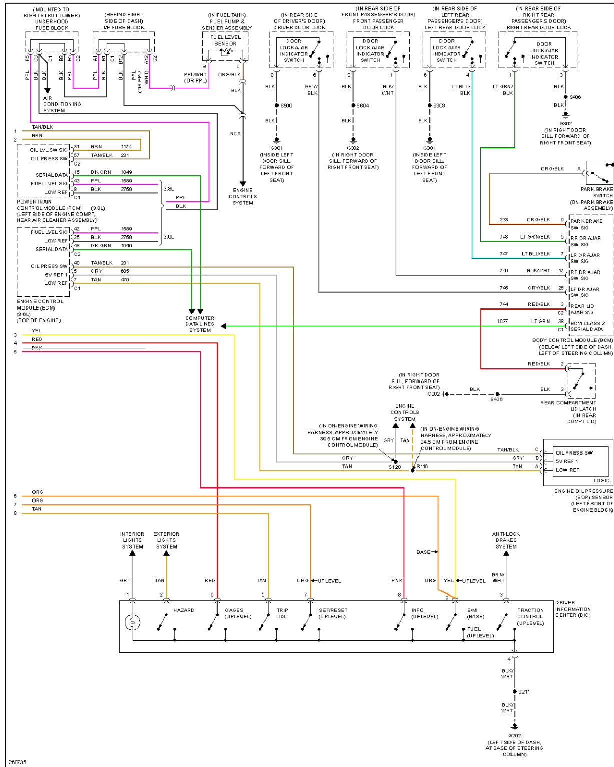
Fig. 38: Instrument Cluster Circuit, W/ Message Center (2 of 2)
