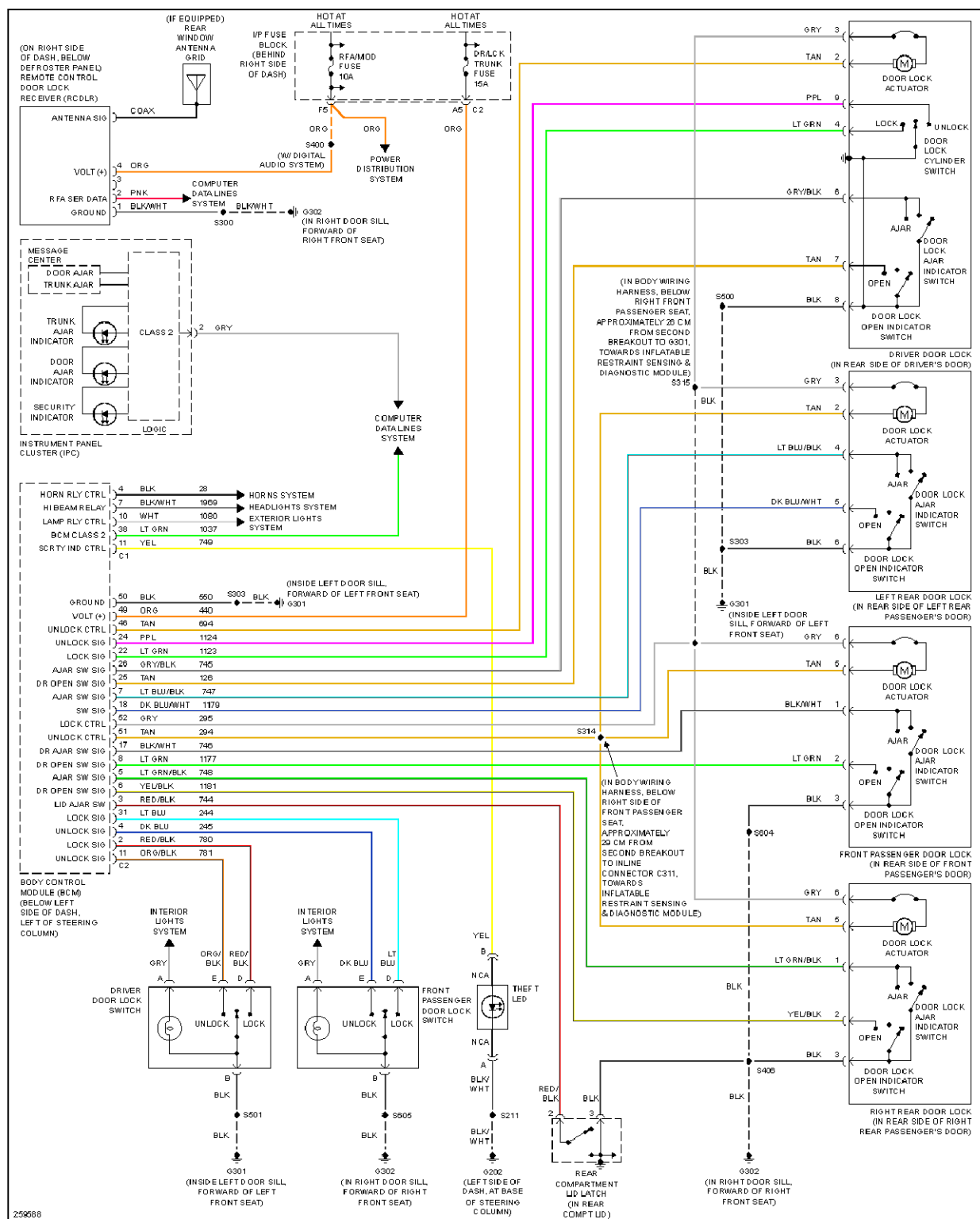
Fig. 10: Forced Entry Circuit
