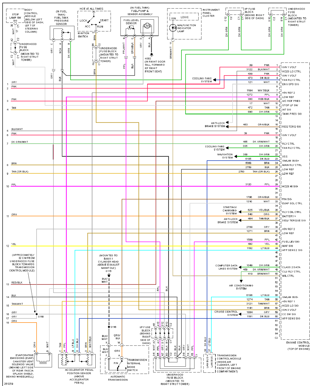
Fig. 23: 3.6L VIN 7, Engine Performance Circuit (4 of 4)
