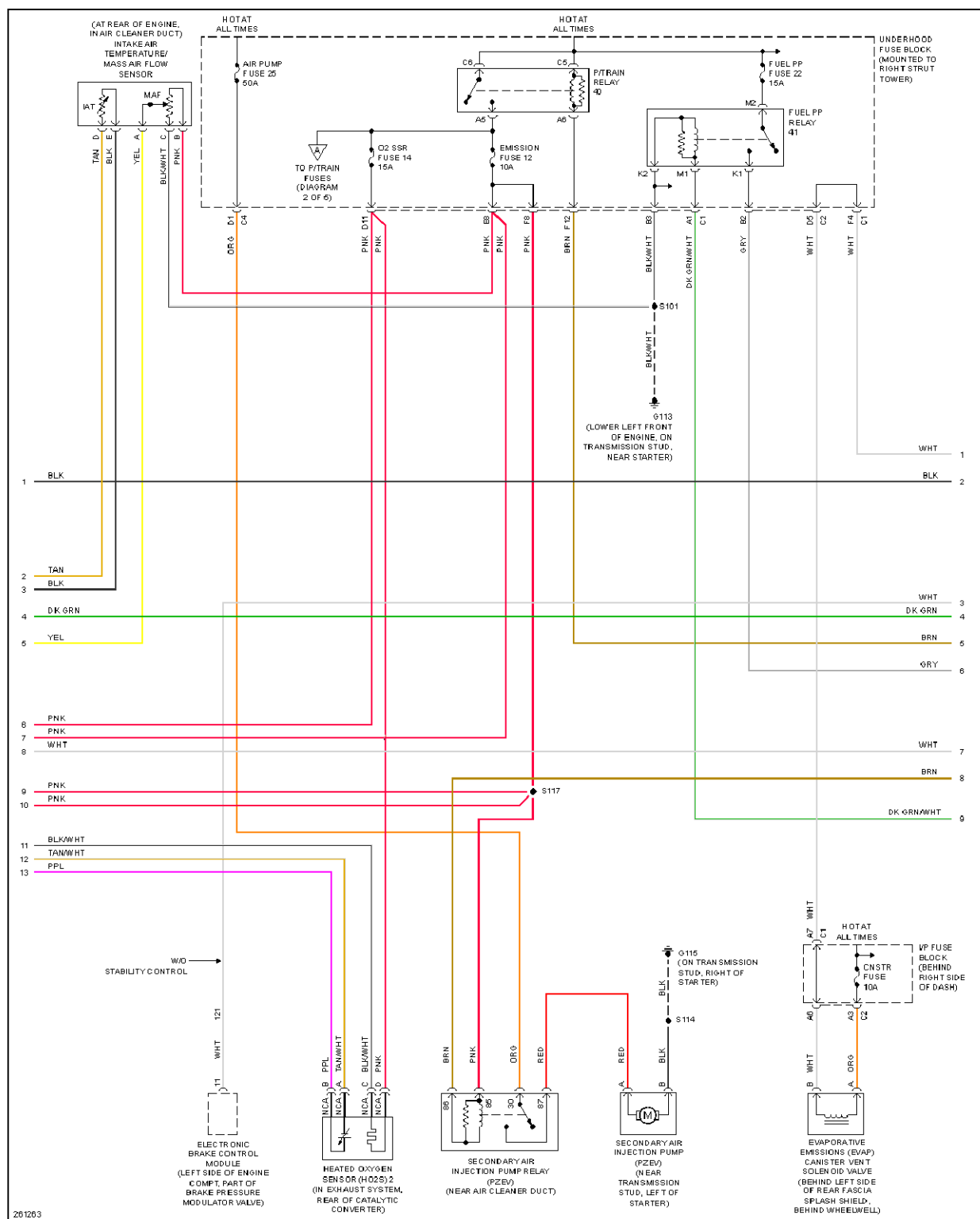
Fig. 27: 3.8L VIN 2, Engine Performance Circuit (4 of 5)
