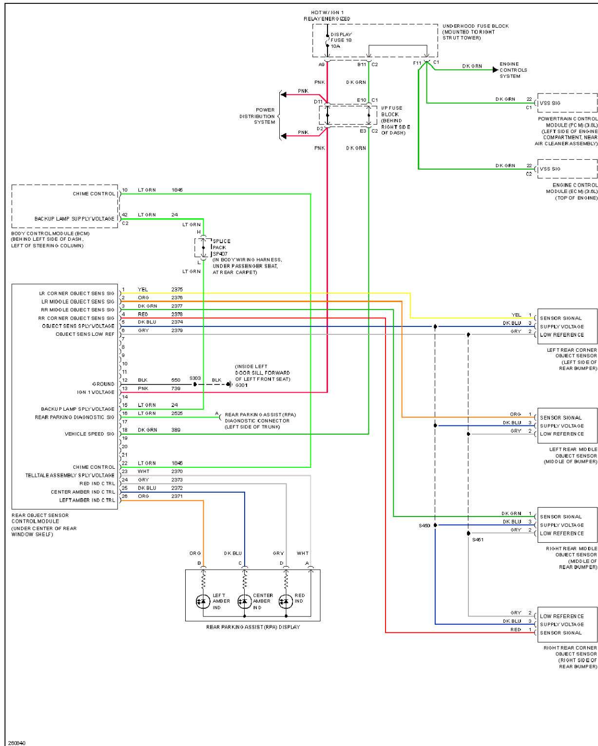
Fig. 43: Parking Assistant Circuit
