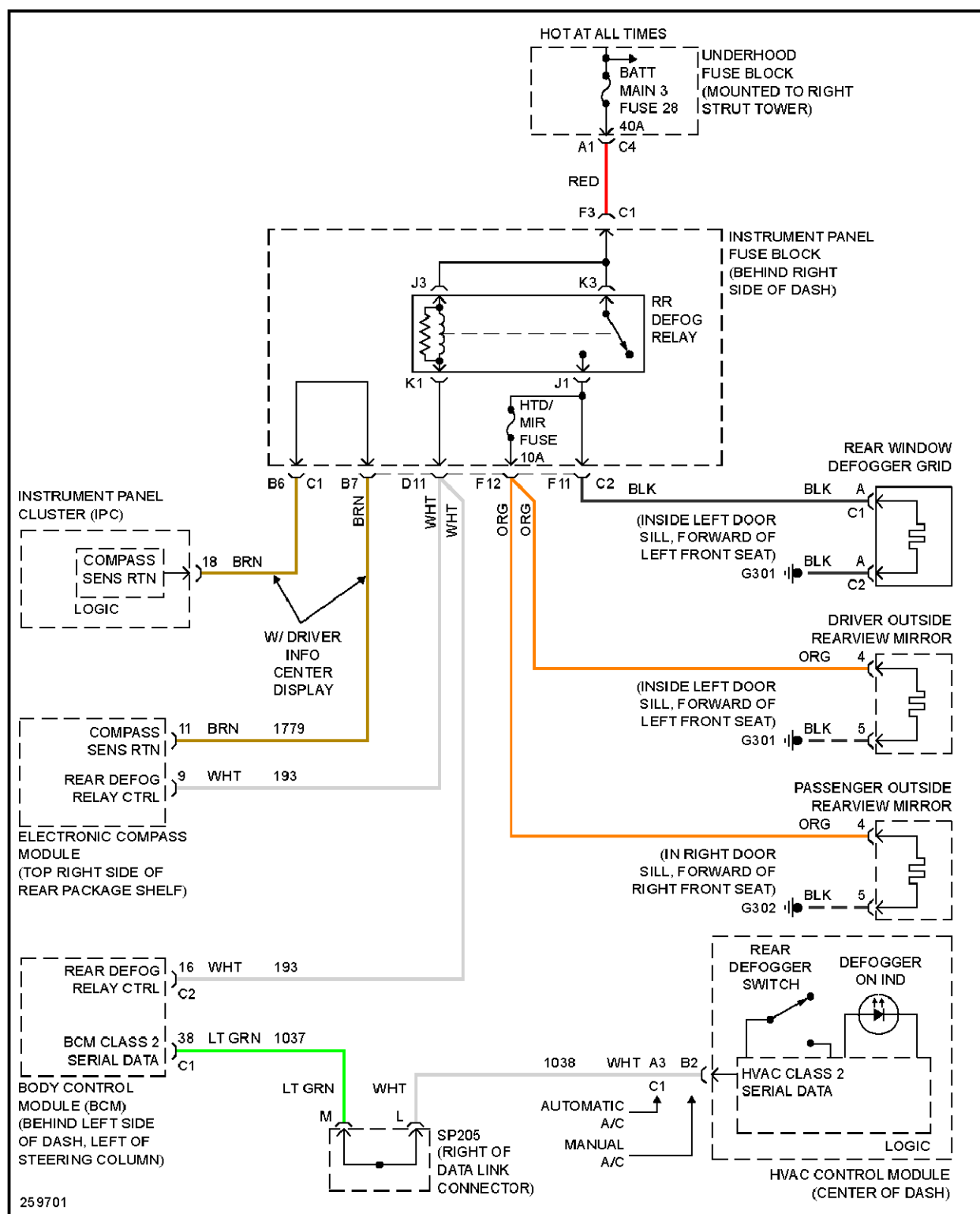
Fig. 18: Defoggers Circuit
