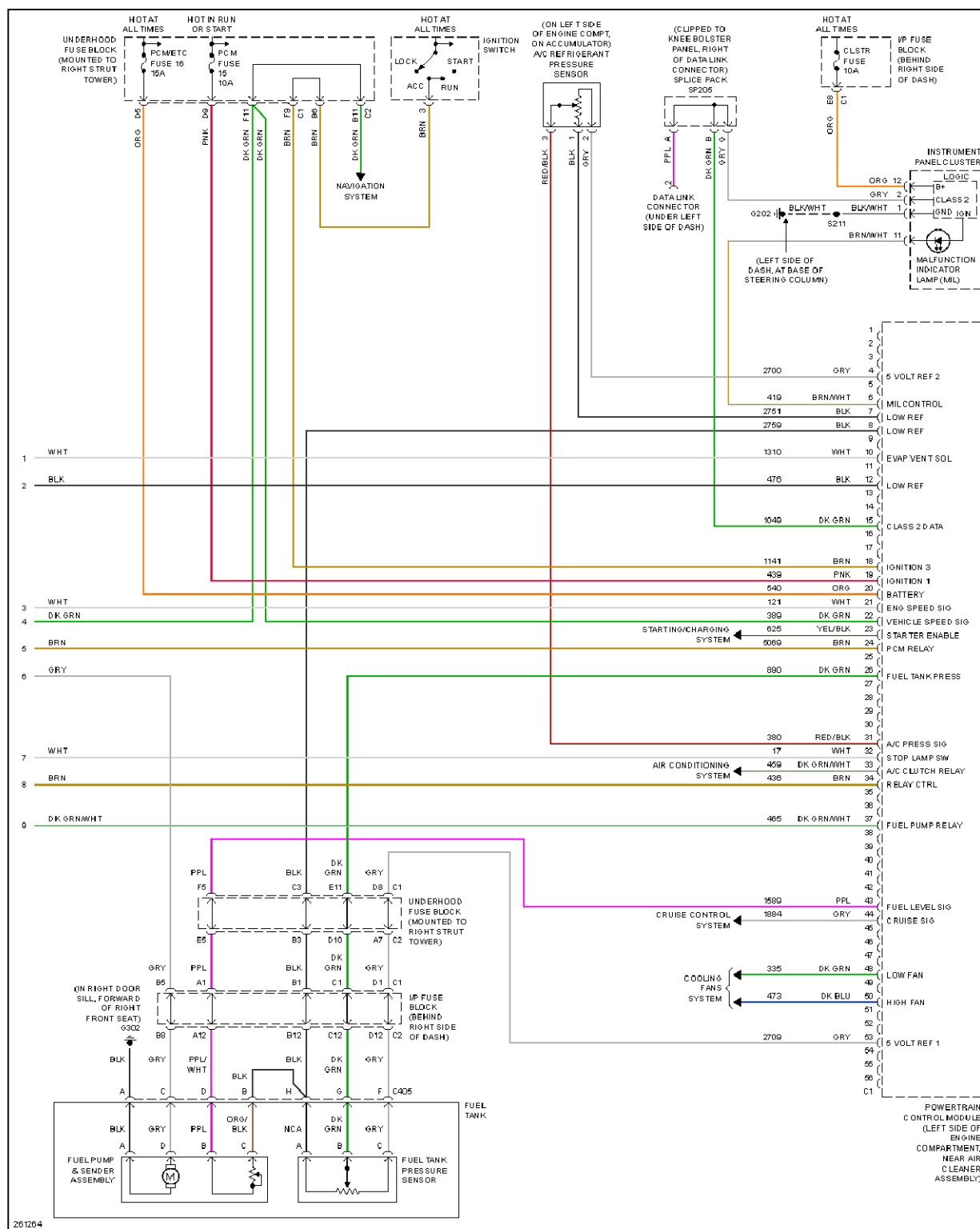
Fig. 28: 3.8L VIN 2, Engine Performance Circuit (5 of 5)
