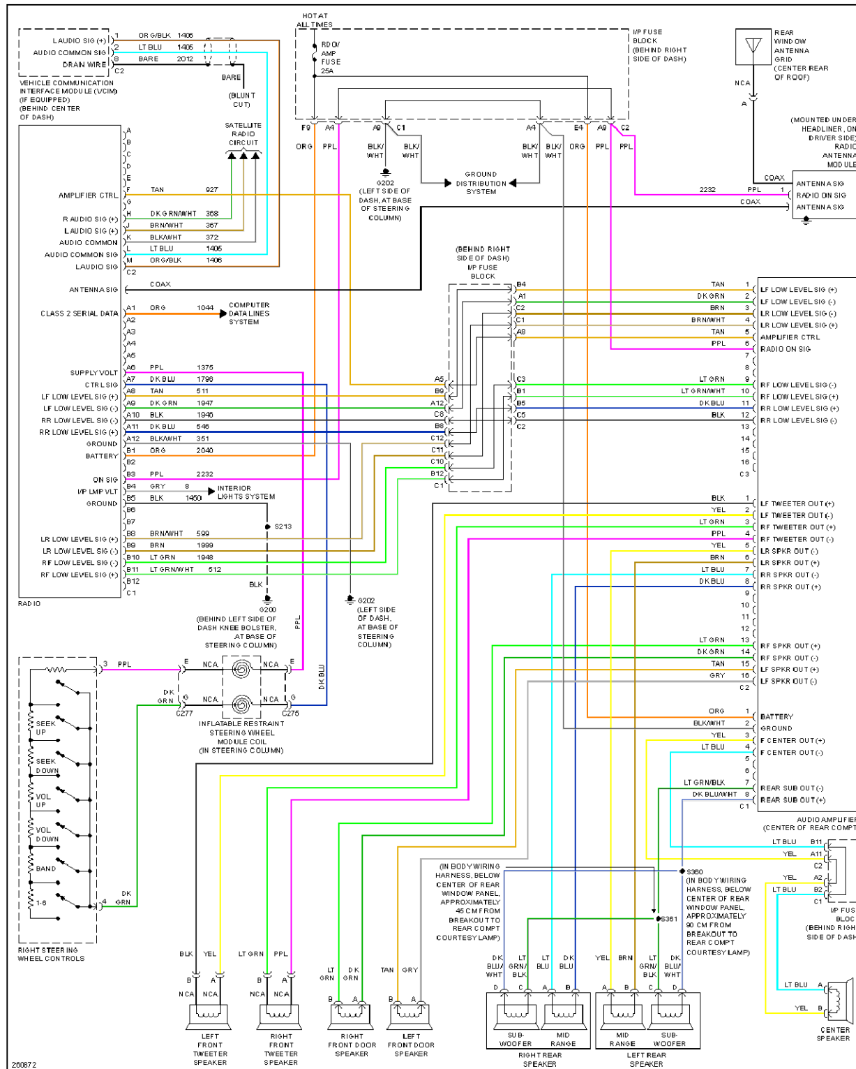
Fig. 57: Radio Circuit, W/ Amplifier
