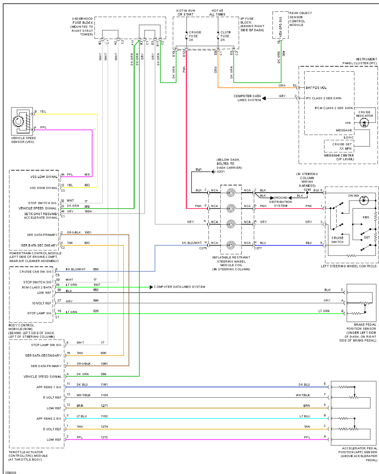
Fig. 17: 3.8L VIN 2, Cruise Control Circuit
