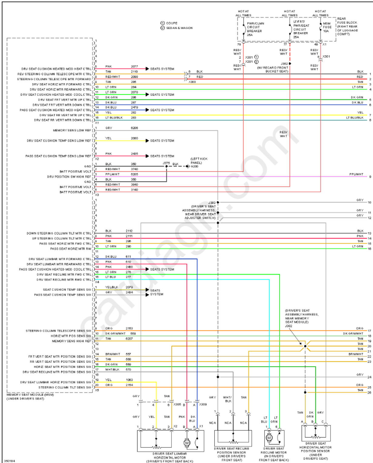
Fig. 60: Memory Seat Circuit (1 of 3)
