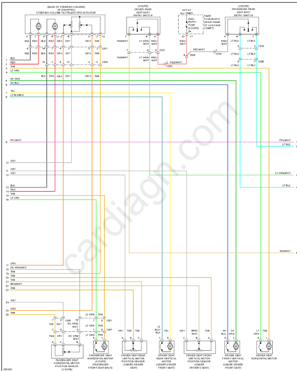
Fig. 61: Memory Seat Circuit (2 of 3)
