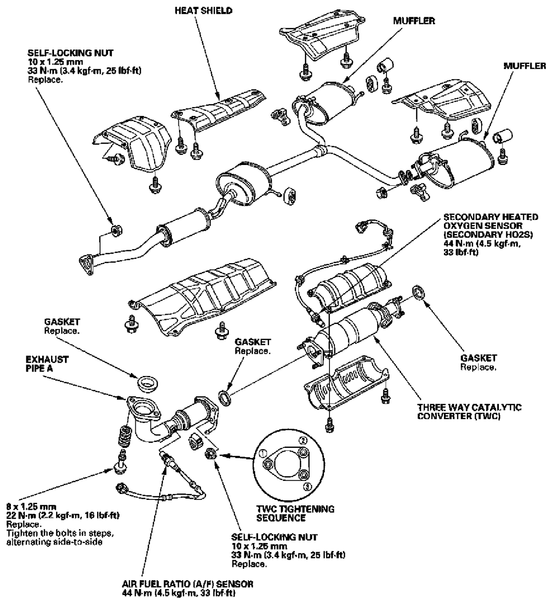
Fig. 1: Replacing Exhaust Pipe & Muffler
