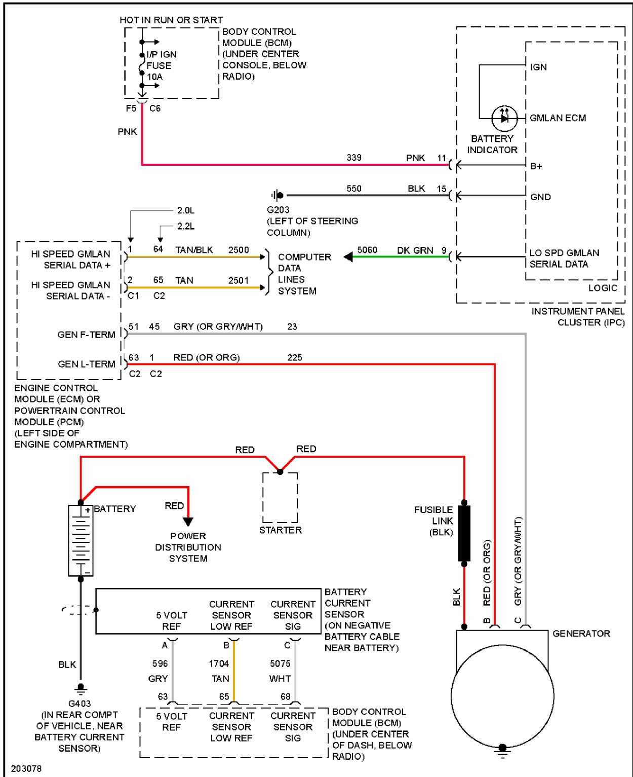
Fig. 54: Charging Circuit
