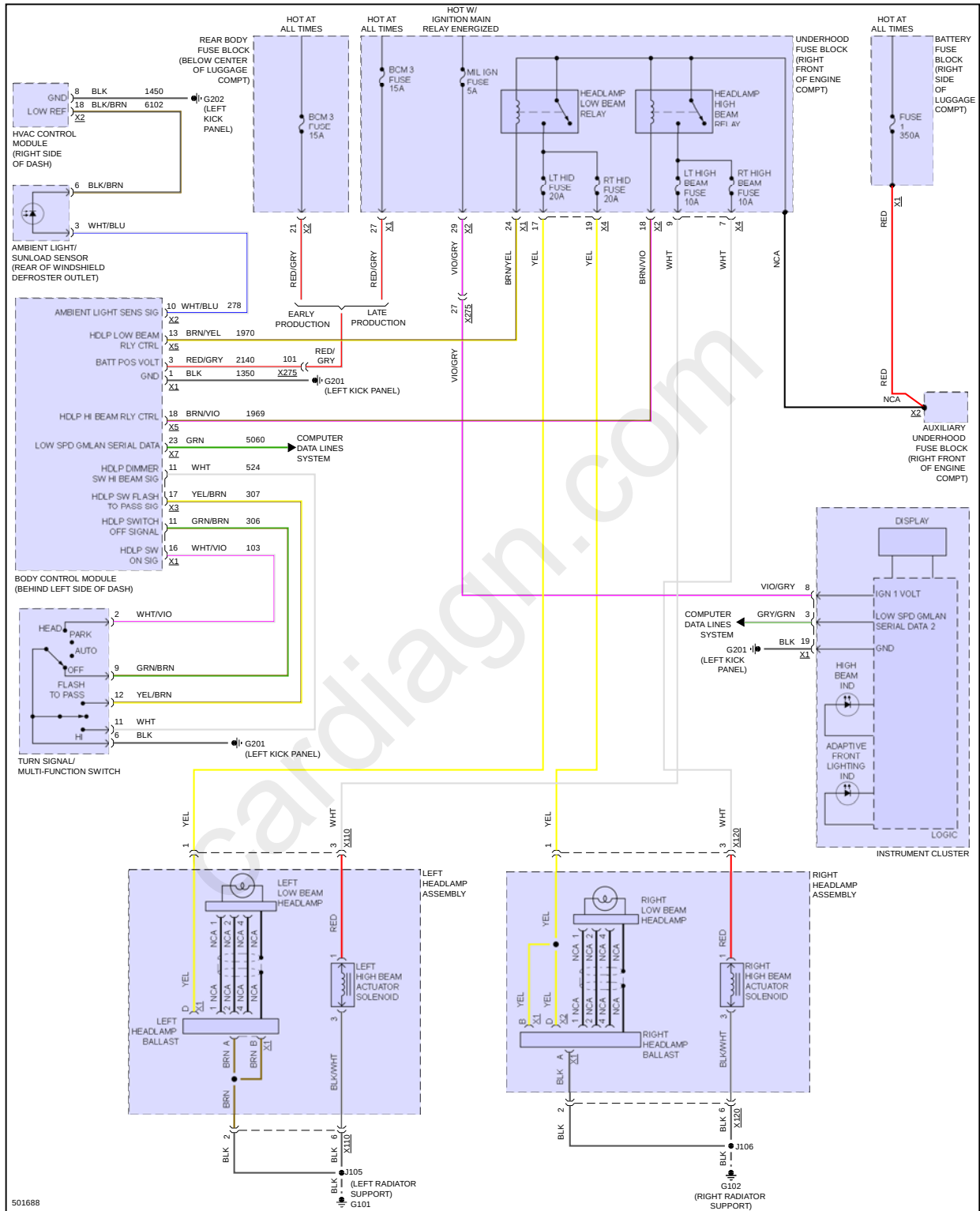
Fig 1: Headlights Circuit, W/ High Intensity Discharge
