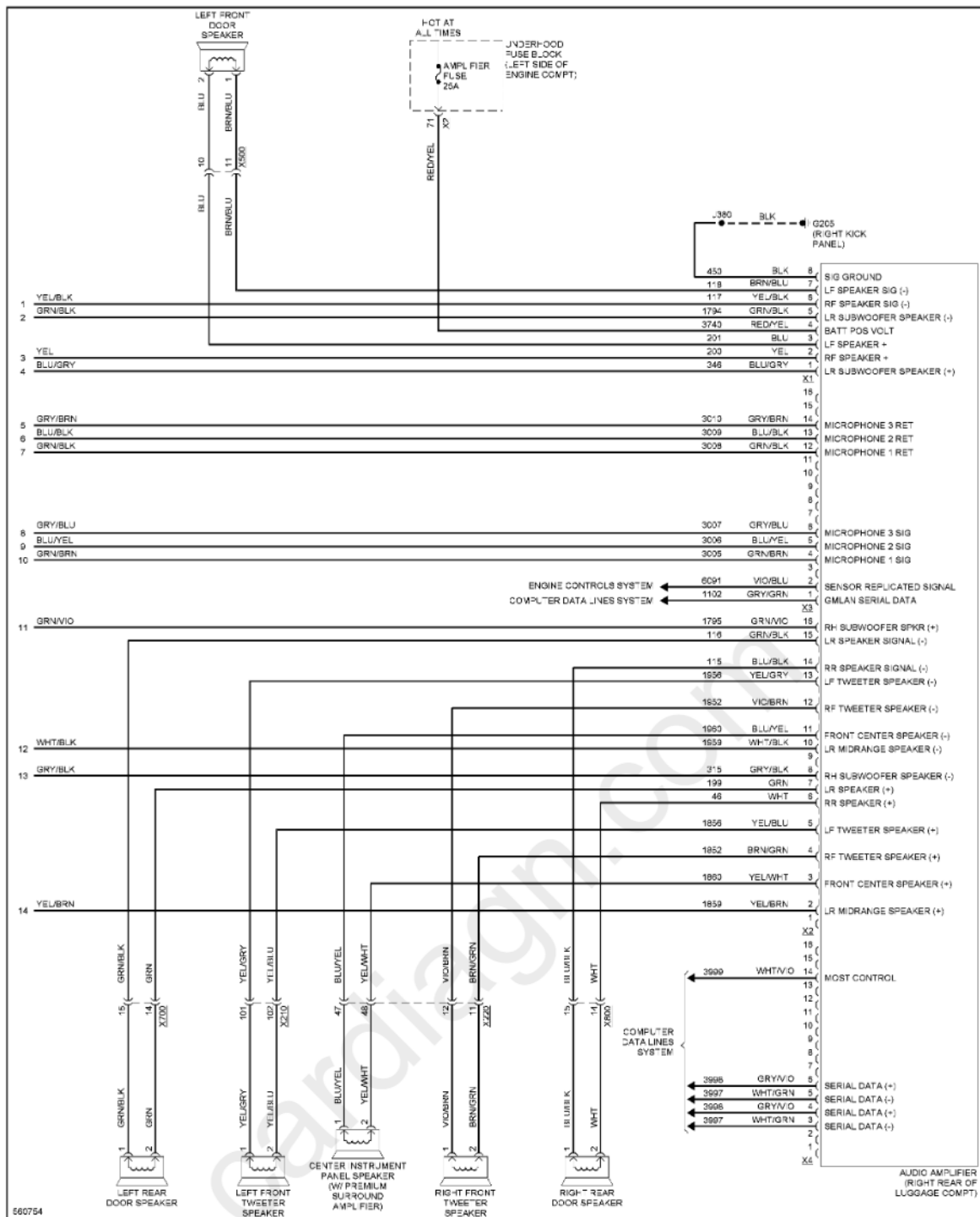
Fig. 81: Navigation Circuit (5 of 5)
