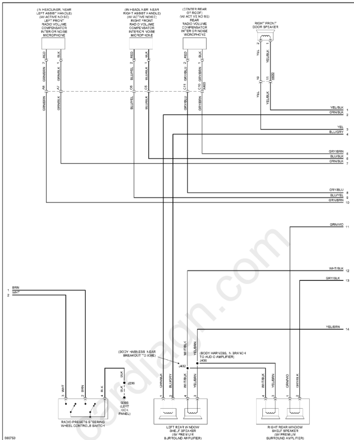
Fig. 80: Navigation Circuit (4 of 5)
