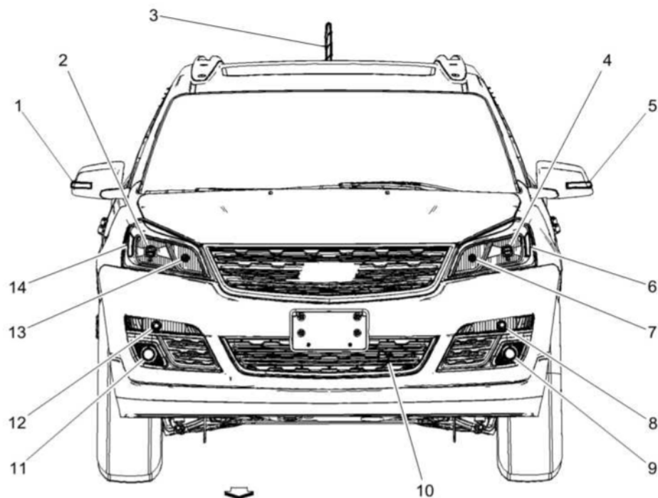
Fig. 2: Front Of Vehicle Components - Traverse Courtesy of GENERAL MOTORS COMPANY
