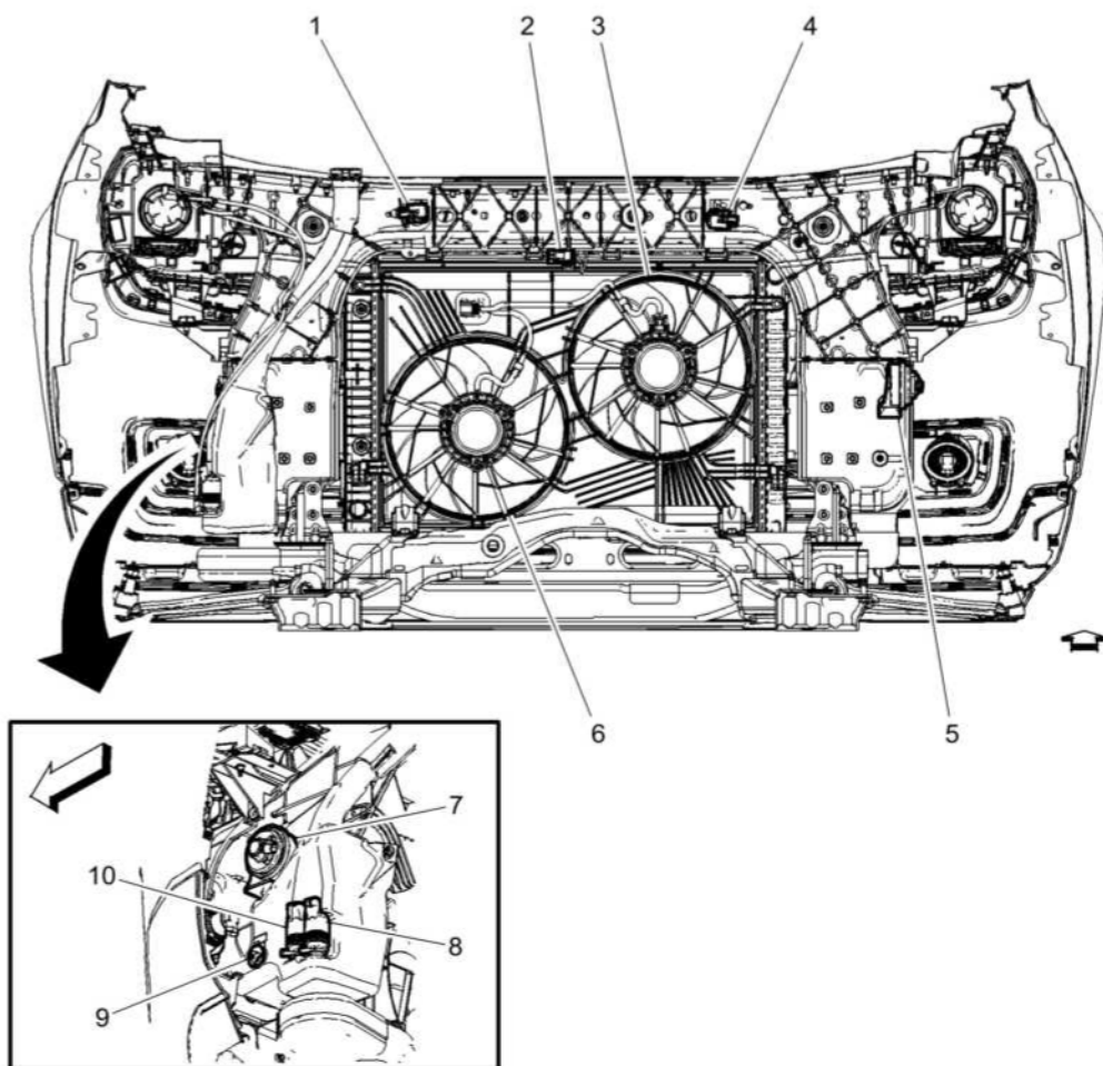
Fig. 4: Front Of Engine Compartment Components
