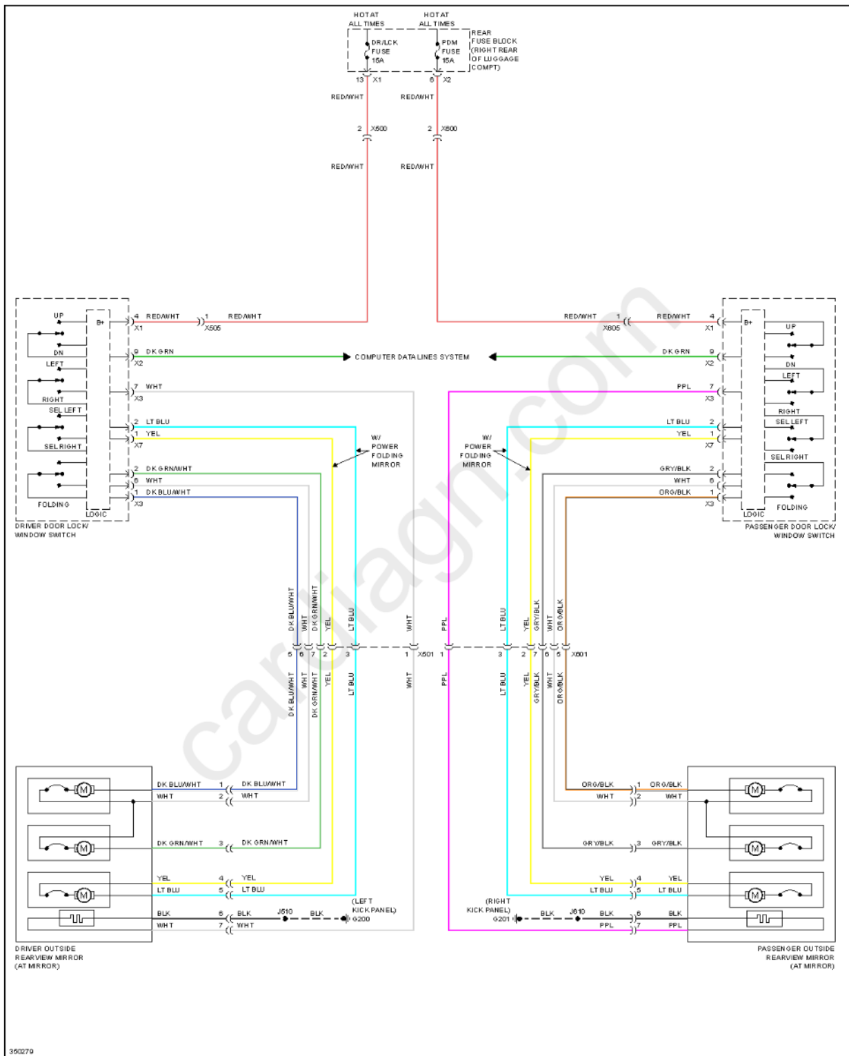
Fig. 87: Power Mirrors Circuit
