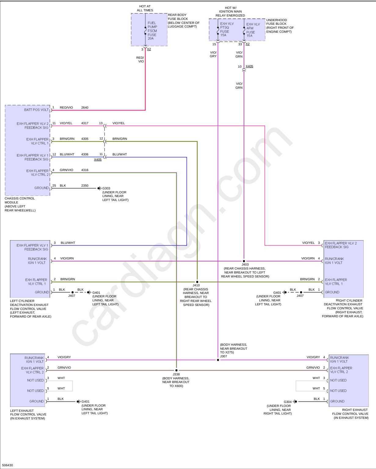
Fig 1: Electronic Muffler Circuit
